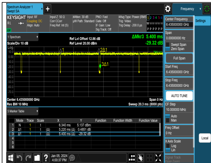
NTNV-11AX20SISO-Ant1-6435
