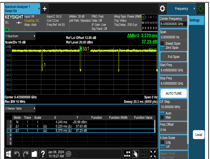
NTNV-11AX20SISO-Ant2-6435
