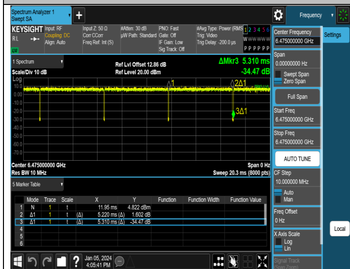
NTNV-11AX20SISO-Ant1-6475
