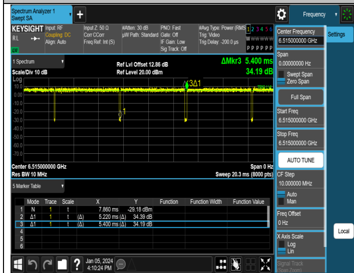
NTNV-11AX20SISO-Ant1-6515
