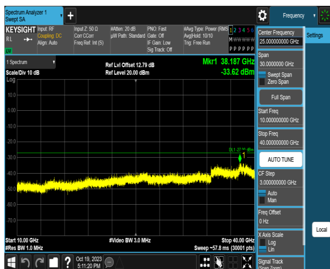
11AX160MIMO-Ant3-6825-10000~40000-PASS
