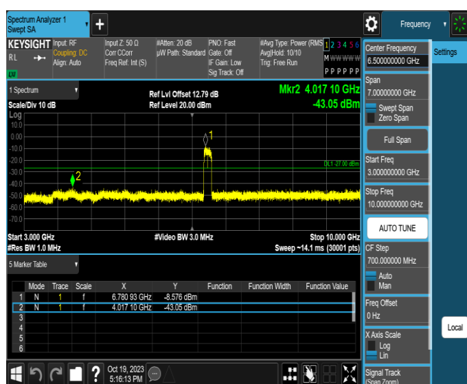
11AX160MIMO-Ant4-6825-3000~10000-PASS
