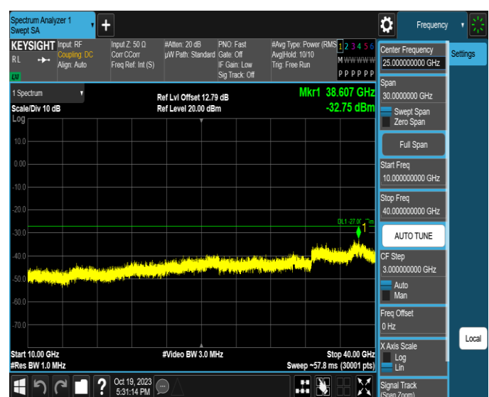
11AX160MIMO-Ant2-6985-10000~40000-PASS
