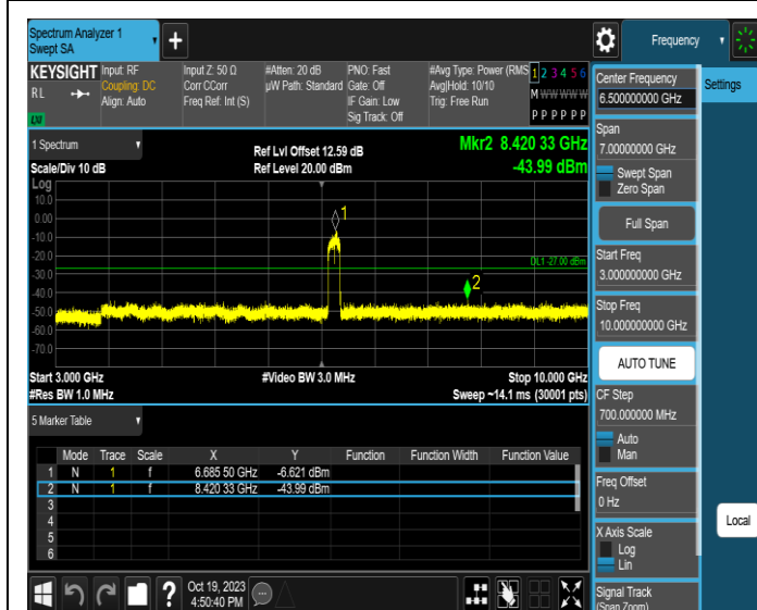
11AX160MIMO-Ant4-6665-3000~10000-PASS
