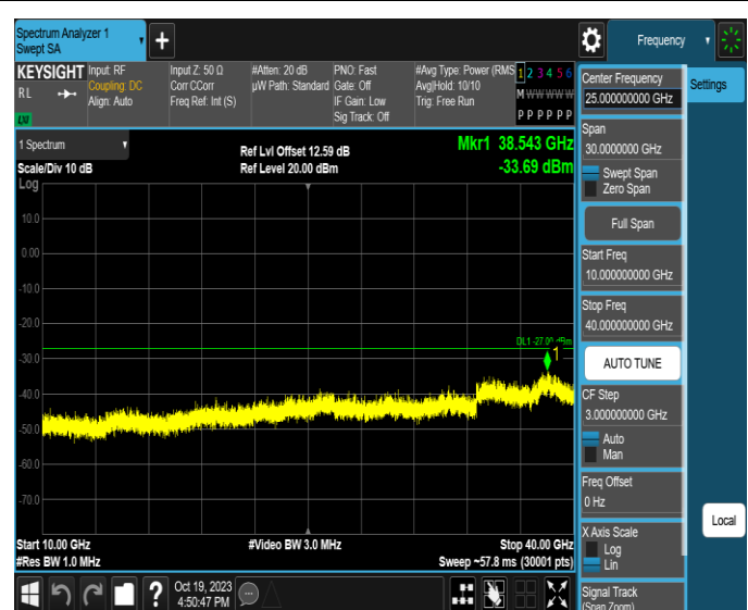
11AX160MIMO-Ant4-6665-10000~40000-PASS
