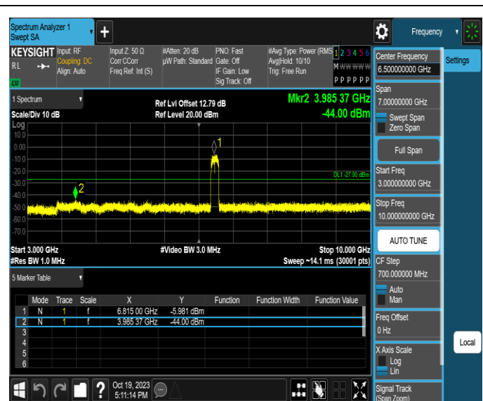
11AX160MIMO-Ant3-6825-3000~10000-PASS
