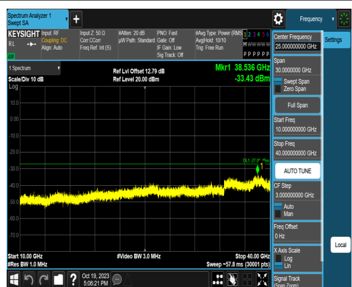
11AX160MIMO-Ant2-6825-10000~40000-PASS
