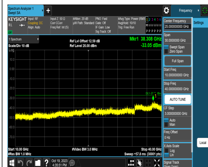
11AX160MIMO-Ant1-6665-10000~40000-PASS
