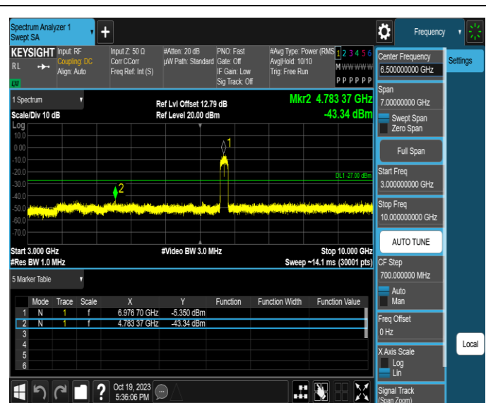
11AX160MIMO-Ant3-6985-3000~10000-PASS
