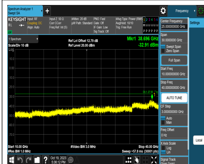
11AX160MIMO-Ant3-6985-10000~40000-PASS
