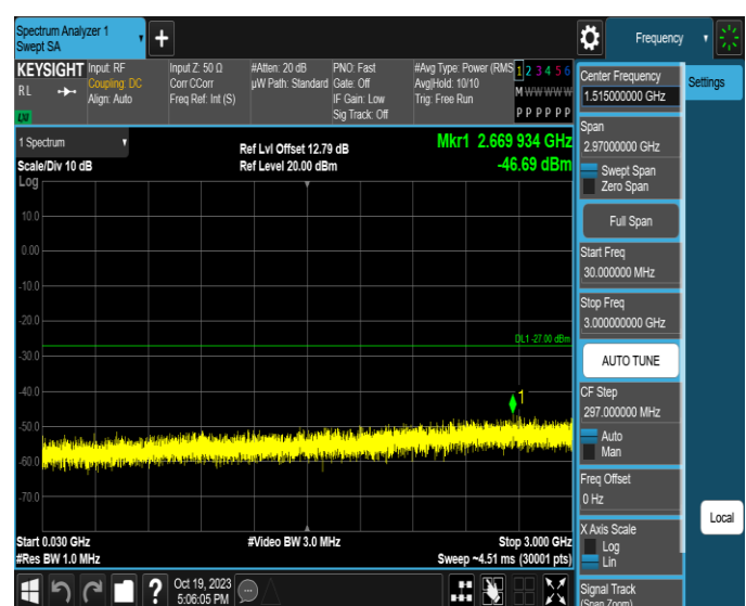
11AX160MIMO-Ant2-6825-30~3000-PASS
