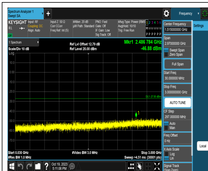
11AX160MIMO-Ant3-6825-30~3000-PASS
