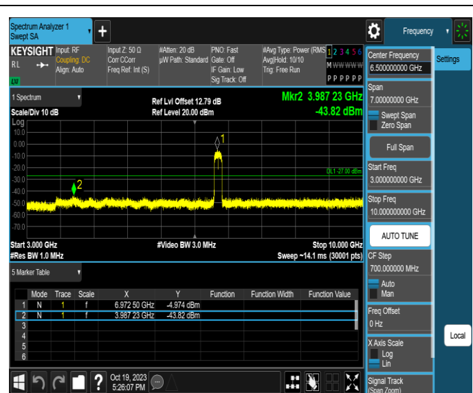
11AX160MIMO-Ant1-6985-3000~10000-PASS
