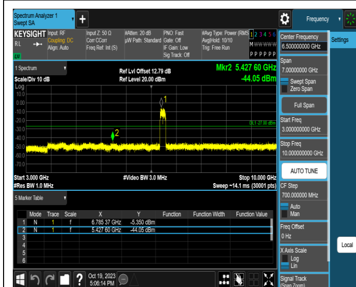
11AX160MIMO-Ant2-6825-3000~10000-PASS
