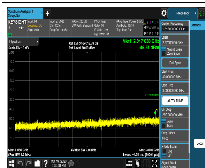
11AX160MIMO-Ant3-6985-30~3000-PASS
