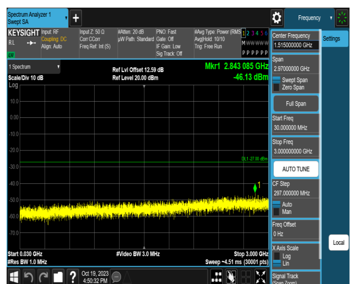
11AX160MIMO-Ant4-6665-30~3000-PASS
