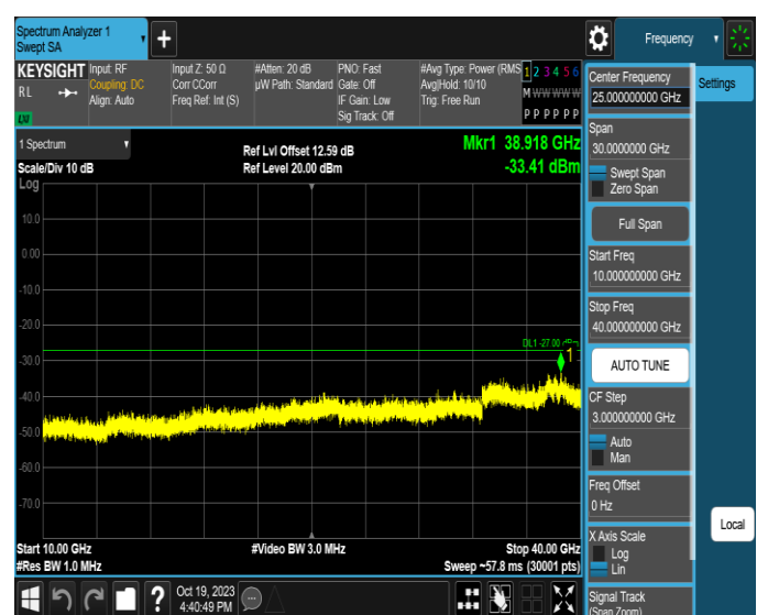
11AX160MIMO-Ant2-6665-10000~40000-PASS
