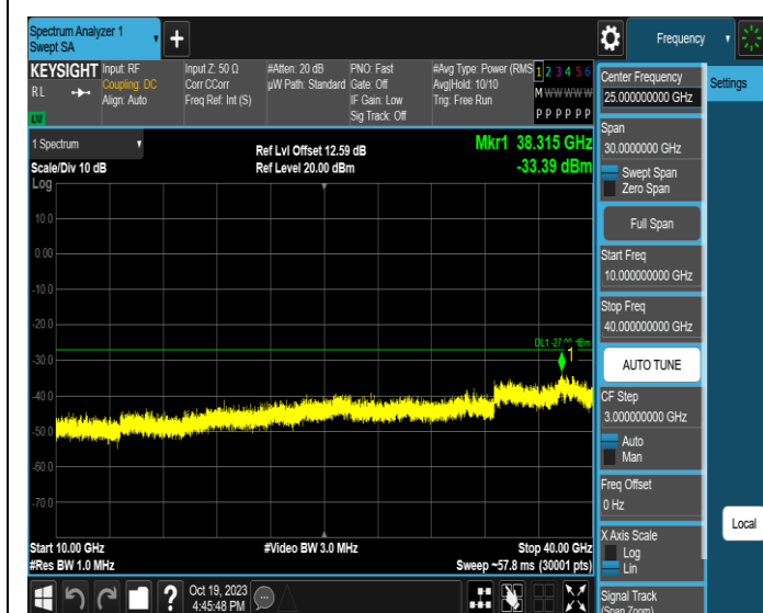
11AX160MIMO-Ant3-6665-10000~40000-PASS
