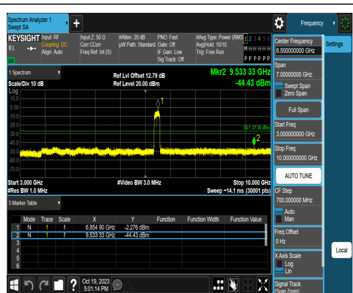
11AX160MIMO-Ant1-6825-3000~10000-PASS
