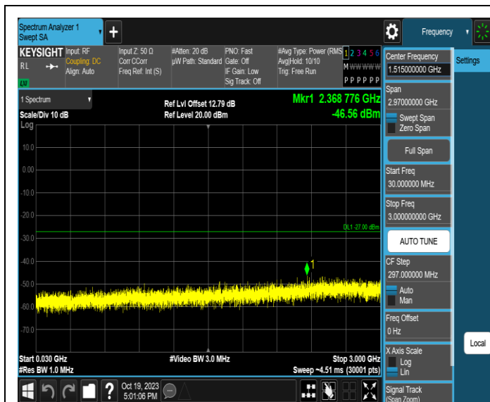
11AX160MIMO-Ant1-6825-30~3000-PASS
