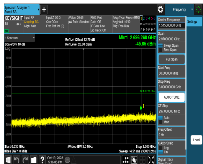
11AX160MIMO-Ant4-6825-30~3000-PASS
