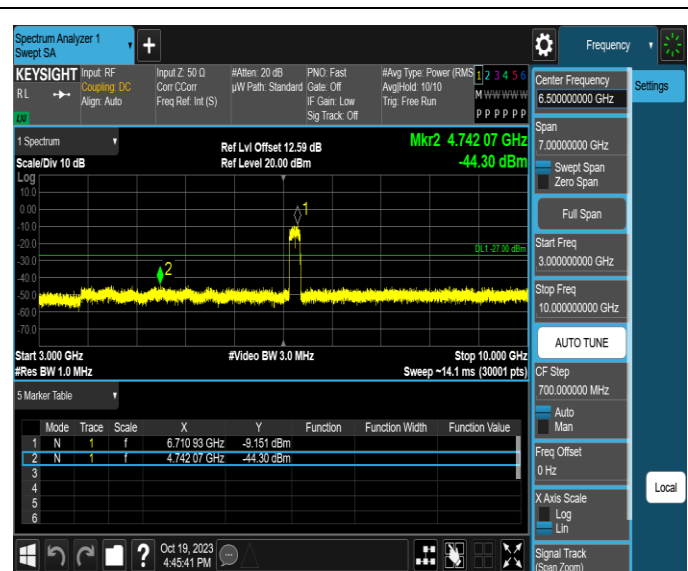
11AX160MIMO-Ant3-6665-3000~10000-PASS
