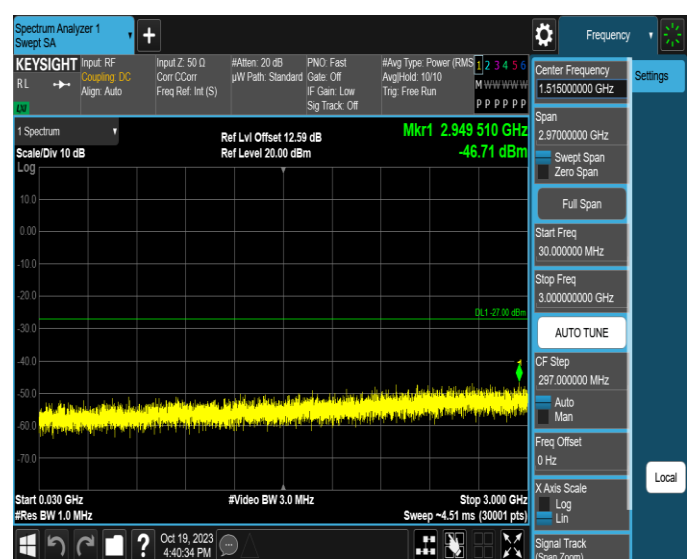
11AX160MIMO-Ant2-6665-30~3000-PASS
