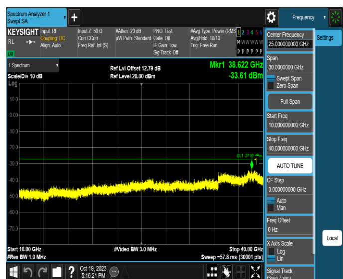
11AX160MIMO-Ant4-6825-10000~40000-PASS
