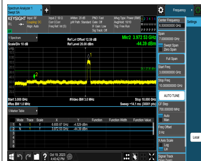
11AX160MIMO-Ant2-6665-3000~10000-PASS
