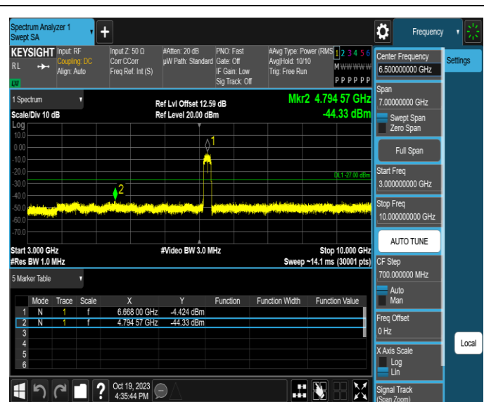
11AX160MIMO-Ant1-6665-3000~10000-PASS
