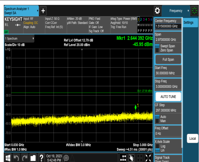
11AX160MIMO-Ant4-6985-30~3000-PASS
