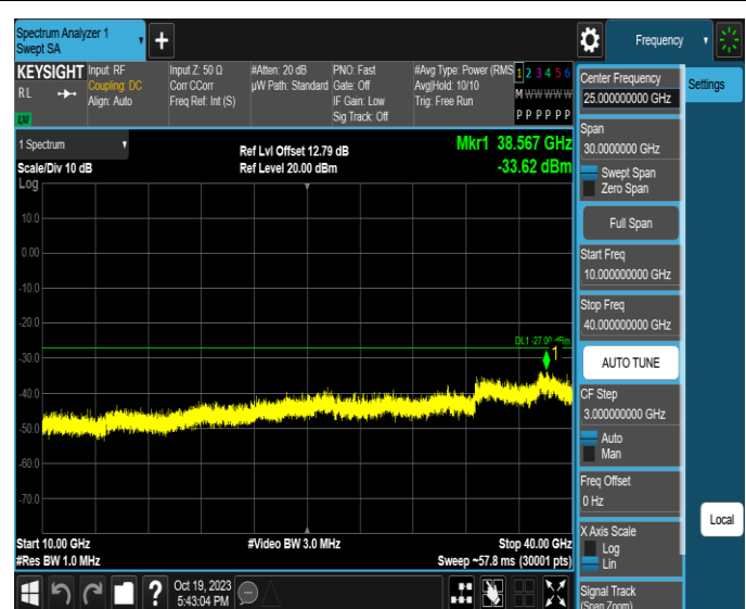
11AX160MIMO-Ant4-6985-10000~40000-PASS
