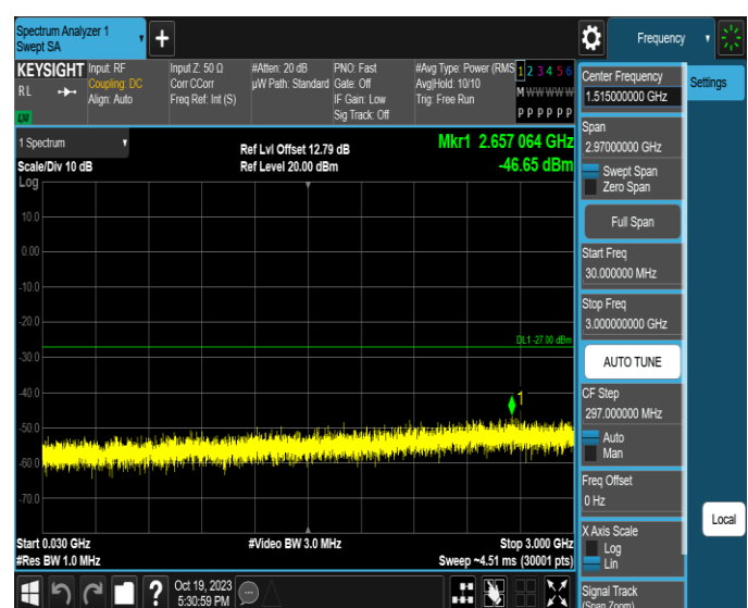
11AX160MIMO-Ant2-6985-30~3000-PASS
