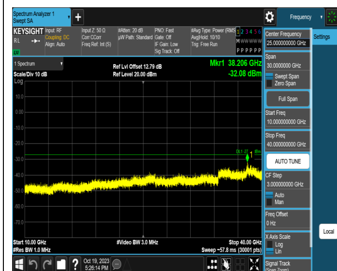
11AX160MIMO-Ant1-6985-10000~40000-PASS
