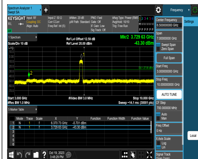
11AX160MIMO-Ant2-6345-3000~10000-PASS
