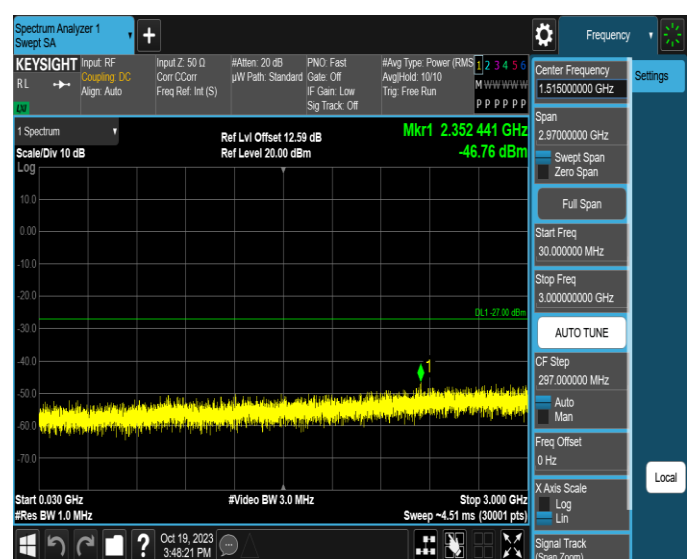
11AX160MIMO-Ant2-6345-30~3000-PASS
