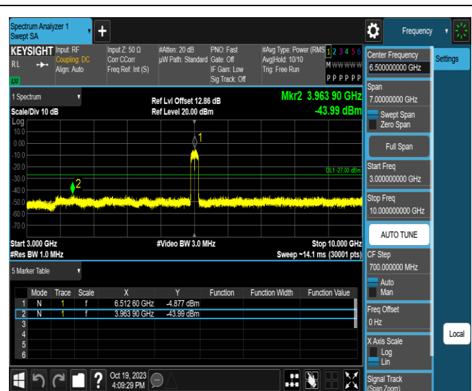
11AX160MIMO-Ant1-6505-3000~10000-PASS
