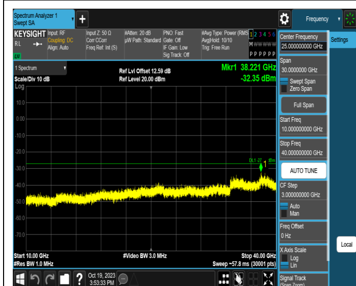
11AX160MIMO-Ant3-6345-10000~40000-PASS
