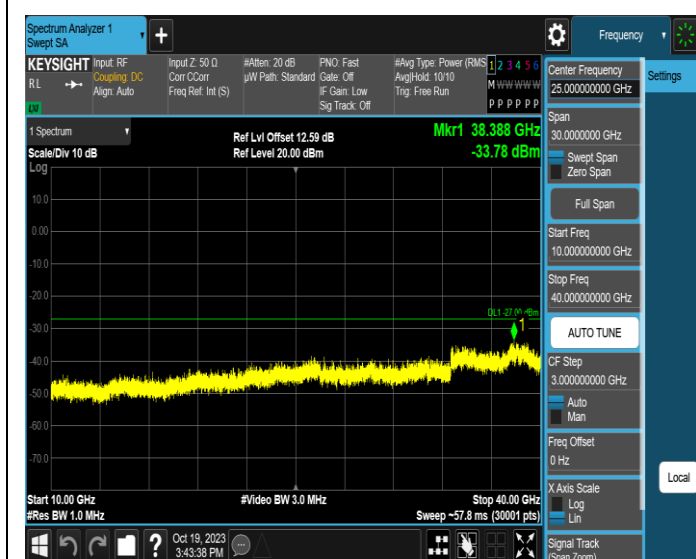
11AX160MIMO-Ant1-6345-10000~40000-PASS
