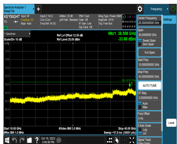
11AX160MIMO-Ant2-6345-10000~40000-PASS
