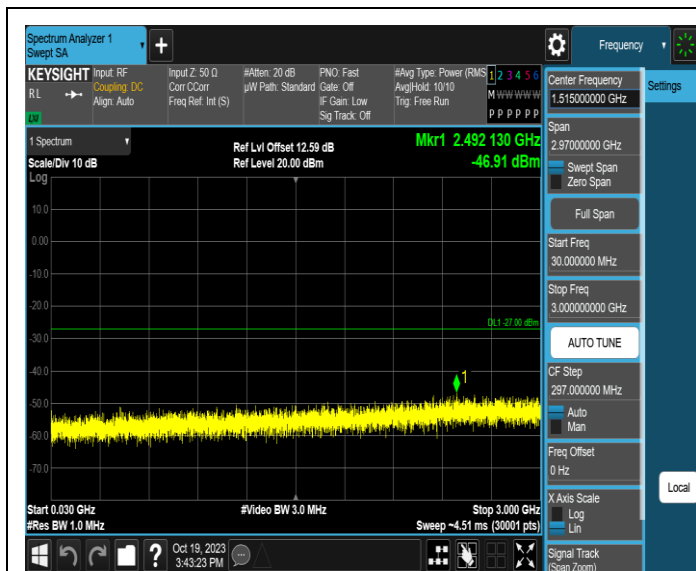
11AX160MIMO-Ant1-6345-30~3000-PASS
