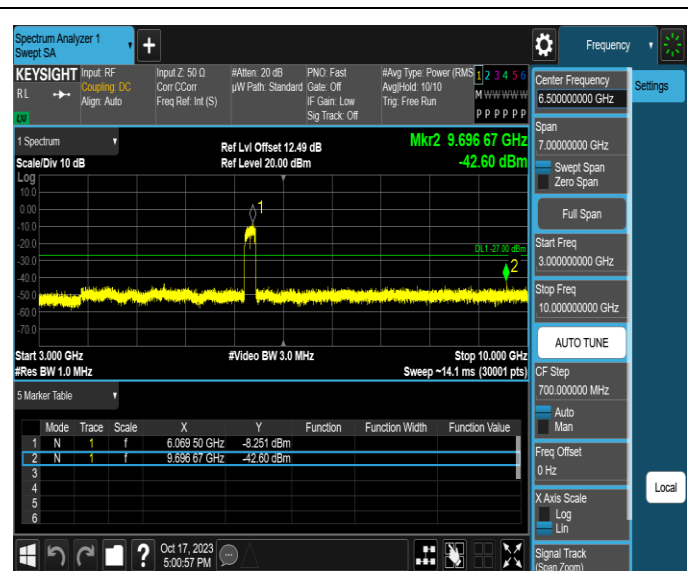
11AX160MIMO-Ant1-6025-3000~10000-PASS
