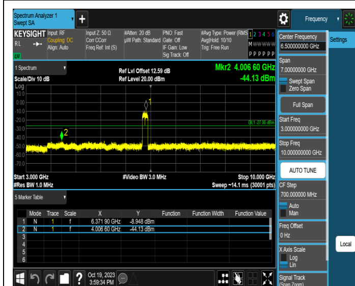
11AX160MIMO-Ant4-6345-3000~10000-PASS
