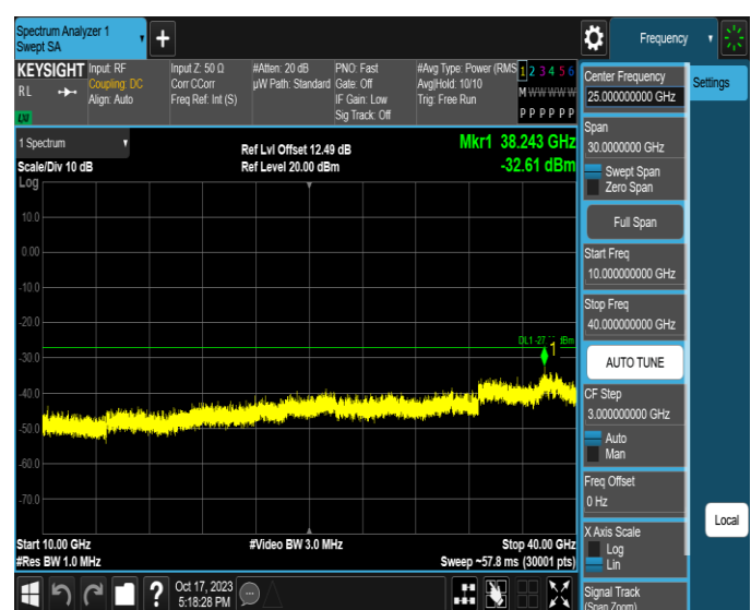
11AX160MIMO-Ant4-6025-10000~40000-PASS
