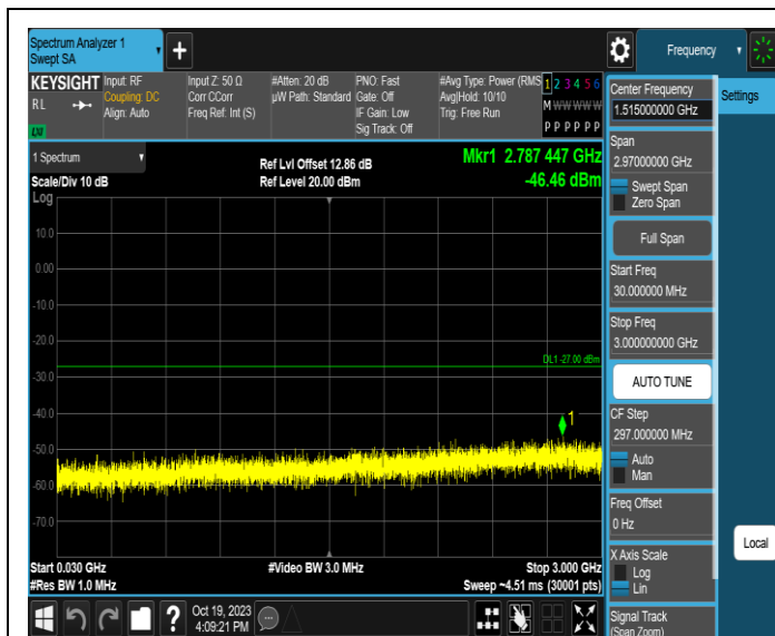
11AX160MIMO-Ant1-6505-30~3000-PASS
