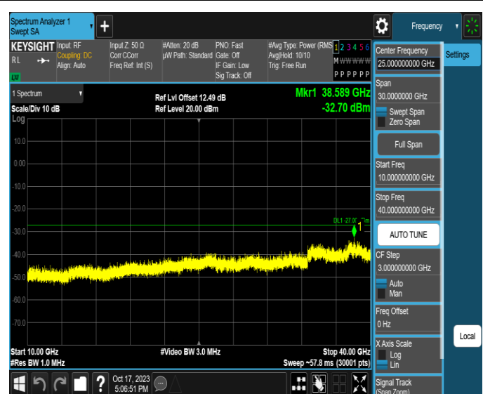
11AX160MIMO-Ant2-6025-10000~40000-PASS
