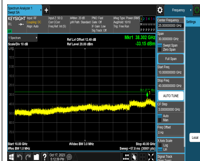
11AX160MIMO-Ant3-6025-10000~40000-PASS
