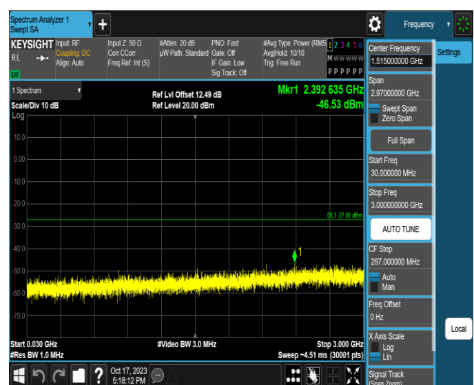
11AX160MIMO-Ant4-6025-30~3000-PASS
