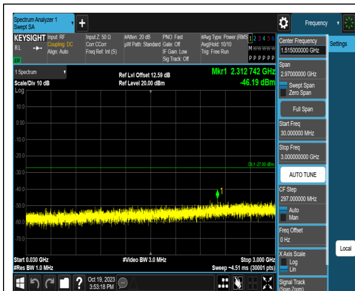
11AX160MIMO-Ant3-6345-30~3000-PASS
