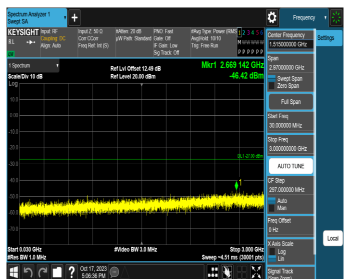
11AX160MIMO-Ant2-6025-30~3000-PASS
