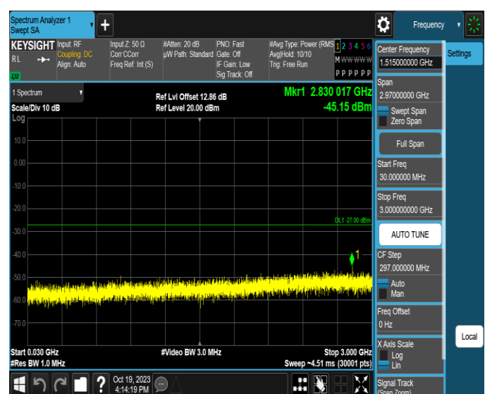
11AX160MIMO-Ant2-6505-30~3000-PASS
