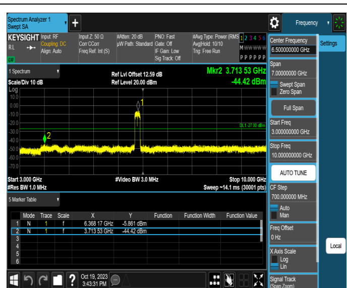
11AX160MIMO-Ant1-6345-3000~10000-PASS
