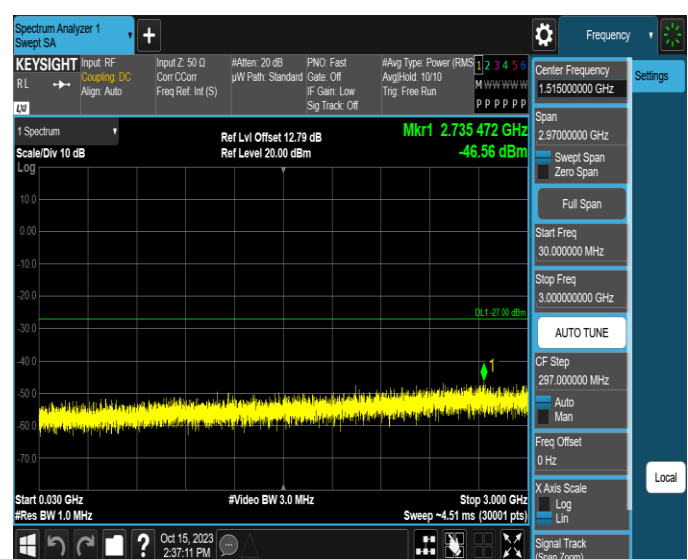
11AX160SISO-Ant4-6985-30~3000-PASS
