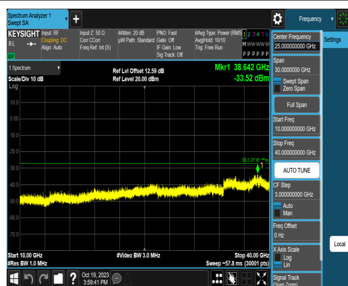
11AX160MIMO-Ant4-6345-10000~40000-PASS
