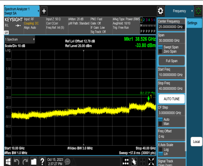
11AX160SISO-Ant4-6985-10000~40000-PASS
