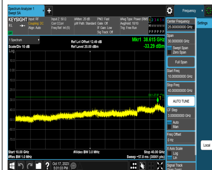
11AX160MIMO-Ant1-6025-10000~40000-PASS
