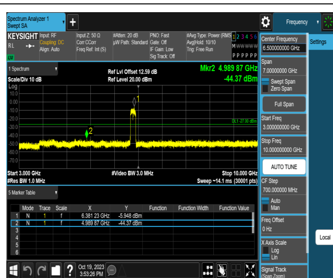
11AX160MIMO-Ant3-6345-3000~10000-PASS
