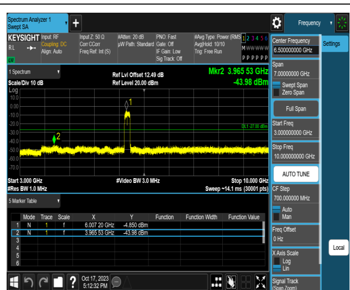
11AX160MIMO-Ant3-6025-3000~10000-PASS
