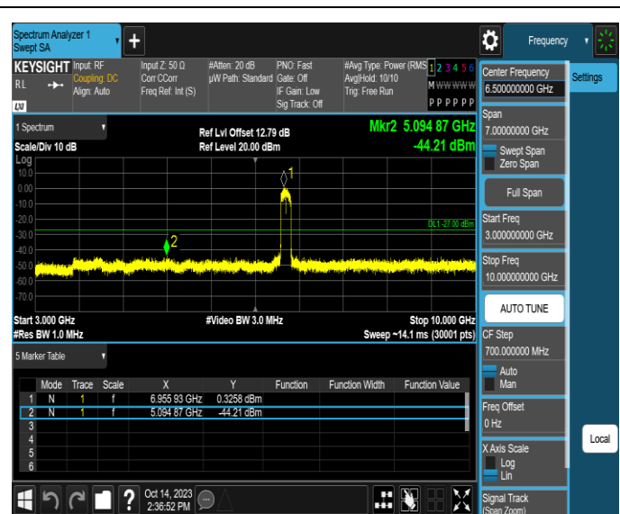
11AX160SISO-Ant3-6985-3000~10000-PASS
