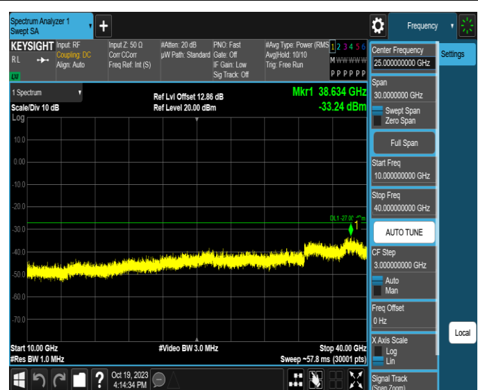
11AX160MIMO-Ant2-6505-10000~40000-PASS
