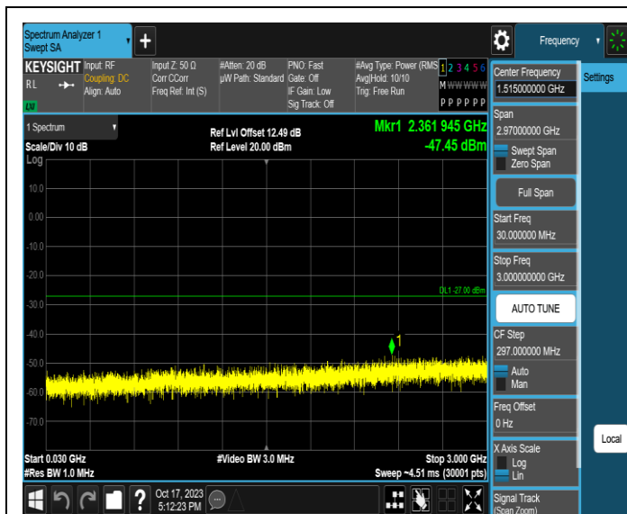
11AX160MIMO-Ant3-6025-30~3000-PASS
