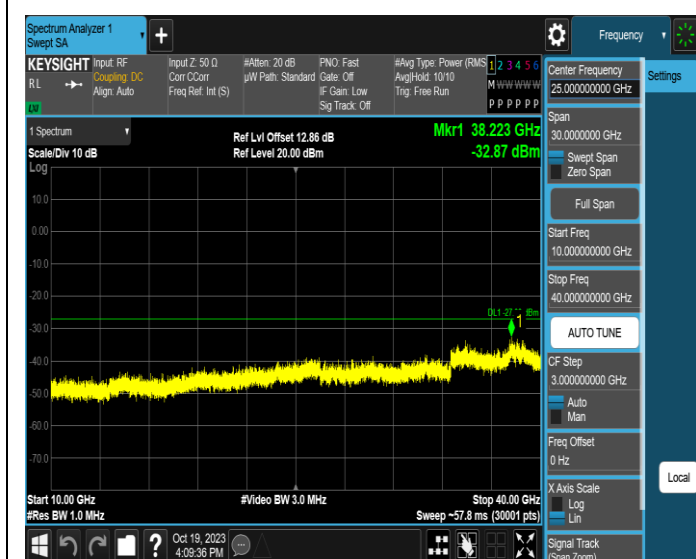
11AX160MIMO-Ant1-6505-10000~40000-PASS
