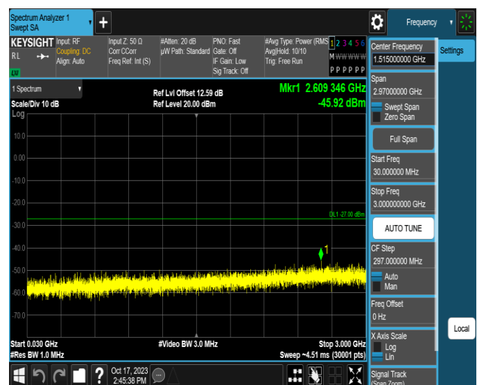
11AX80MIMO-Ant2-6705-30~3000-PASS
