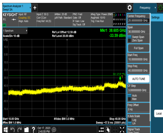
11AX80MIMO-Ant1-6705-10000~40000-PASS
