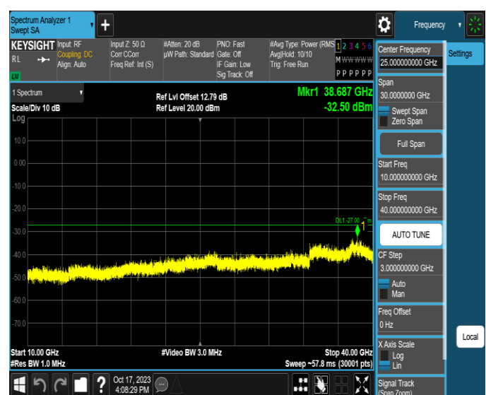
11AX80MIMO-Ant2-6945-10000~40000-PASS
