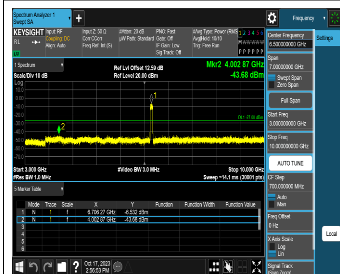
11AX80MIMO-Ant4-6705-3000~10000-PASS
