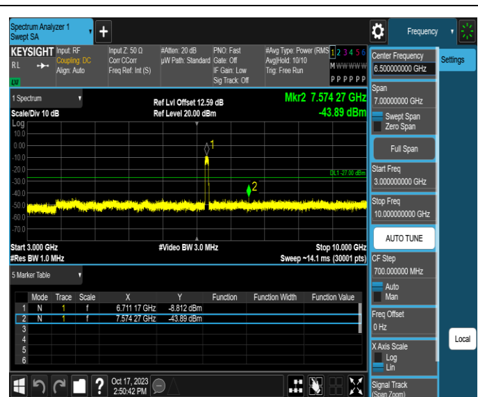
11AX80MIMO-Ant3-6705-3000~10000-PASS
