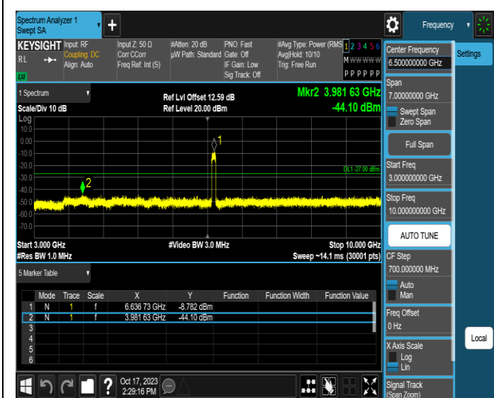
11AX80MIMO-Ant4-6625-3000~10000-PASS
