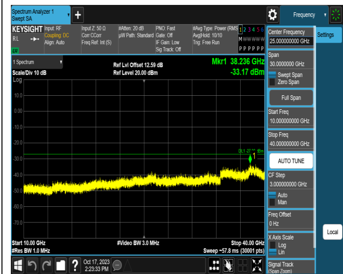
11AX80MIMO-Ant3-6625-10000~40000-PASS
