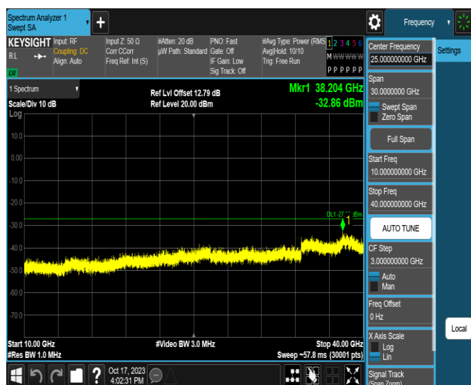
11AX80MIMO-Ant1-6945-10000~40000-PASS
