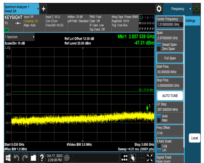
11AX80MIMO-Ant4-6625-30~3000-PASS
