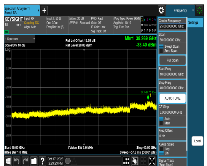
11AX80MIMO-Ant4-6625-10000~40000-PASS
