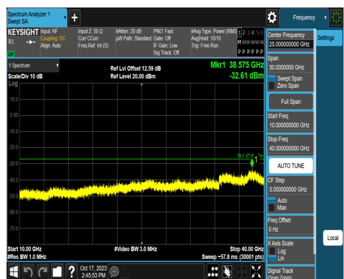
11AX80MIMO-Ant2-6705-10000~40000-PASS
