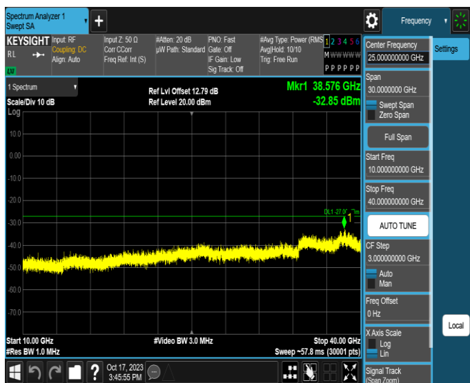
11AX80MIMO-Ant3-6865-10000~40000-PASS
