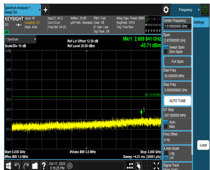
11AX80MIMO-Ant2-6785-30~3000-PASS
