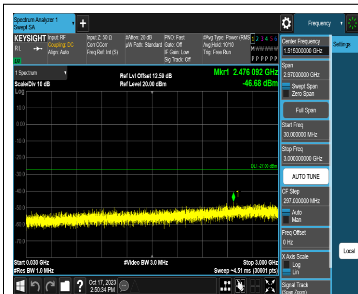
11AX80MIMO-Ant3-6705-30~3000-PASS
