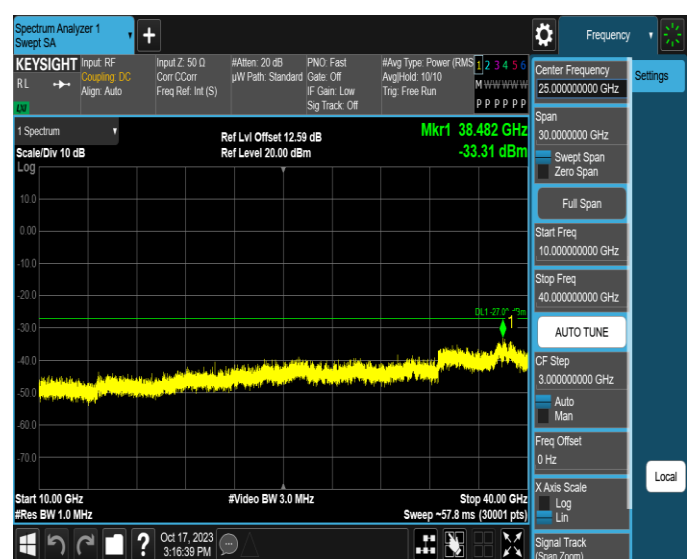
11AX80MIMO-Ant2-6785-10000~40000-PASS
