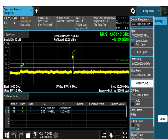
11AX80MIMO-Ant1-6705-3000~10000-PASS
