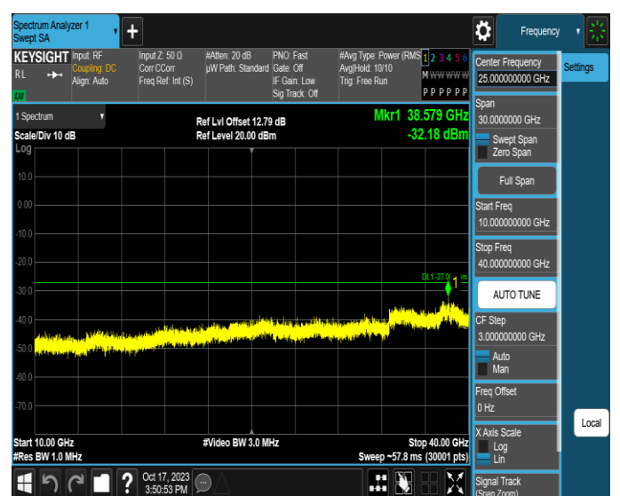
11AX80MIMO-Ant4-6865-10000~40000-PASS
