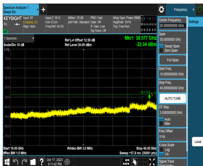
11AX80MIMO-Ant1-6785-10000~40000-PASS
