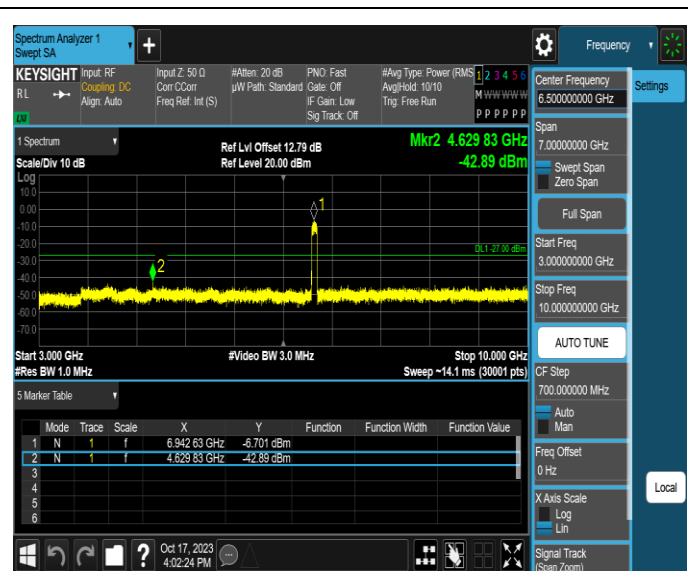
11AX80MIMO-Ant1-6945-3000~10000-PASS
