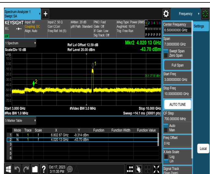
11AX80MIMO-Ant1-6785-3000~10000-PASS
