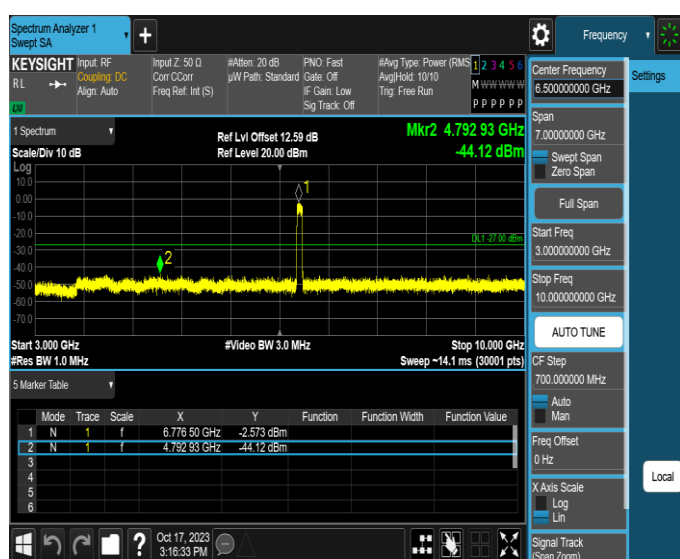
11AX80MIMO-Ant2-6785-3000~10000-PASS
