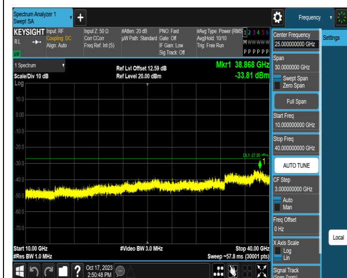
11AX80MIMO-Ant3-6705-10000~40000-PASS
