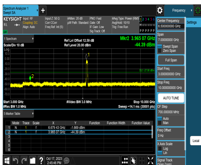
11AX80MIMO-Ant2-6705-3000~10000-PASS
