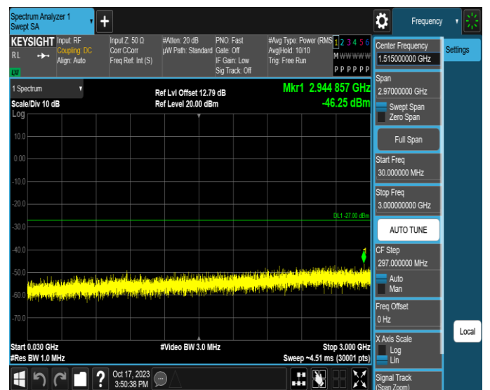
11AX80MIMO-Ant4-6865-30~3000-PASS
