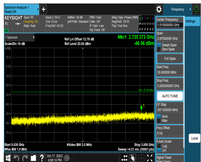
11AX80MIMO-Ant2-6945-30~3000-PASS
