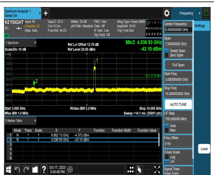
11AX80MIMO-Ant3-6865-3000~10000-PASS
