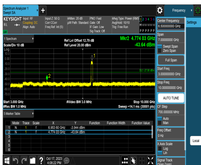
11AX80MIMO-Ant2-6945-3000~10000-PASS
