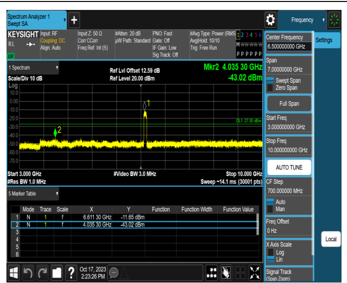
11AX80MIMO-Ant3-6625-3000~10000-PASS
