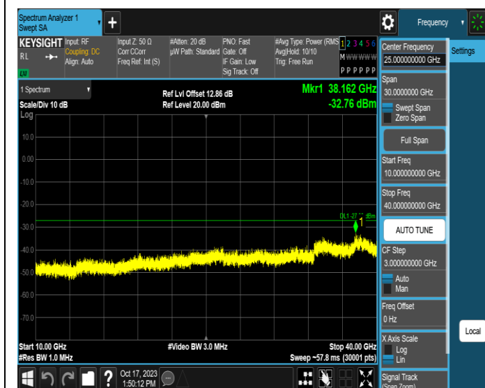
11AX80MIMO-Ant3-6545-10000~40000-PASS
