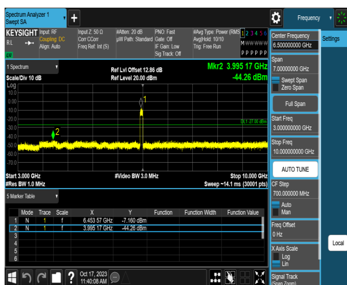
11AX80MIMO-Ant4-6465-3000~10000-PASS
