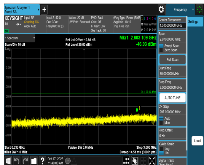
11AX80MIMO-Ant4-6465-30~3000-PASS
