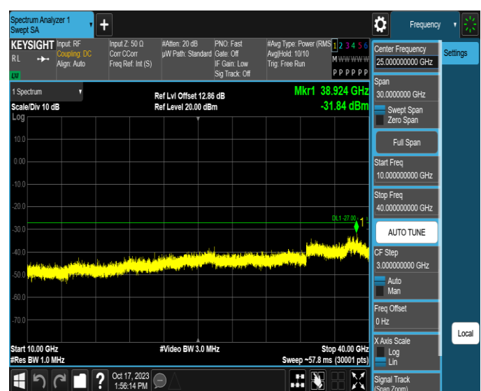
11AX80MIMO-Ant4-6545-10000~40000-PASS
