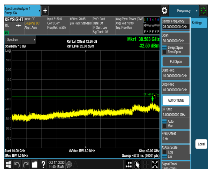
11AX80MIMO-Ant4-6465-10000~40000-PASS
