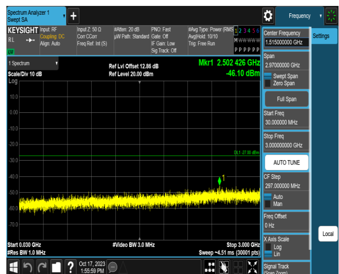
11AX80MIMO-Ant4-6545-30~3000-PASS
