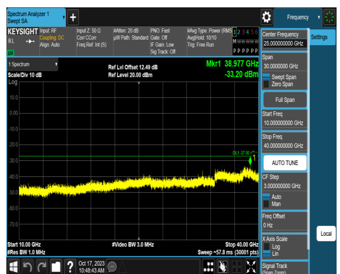
11AX80MIMO-Ant4-6145-10000~40000-PASS
