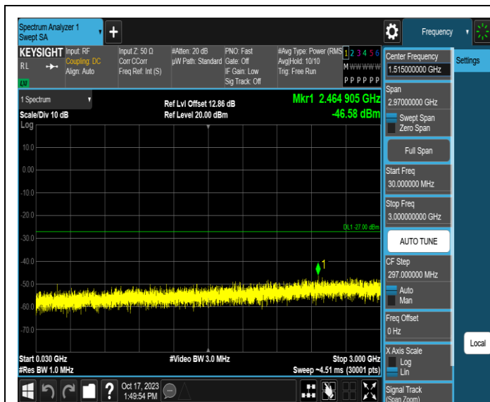
11AX80MIMO-Ant3-6545-30~3000-PASS
