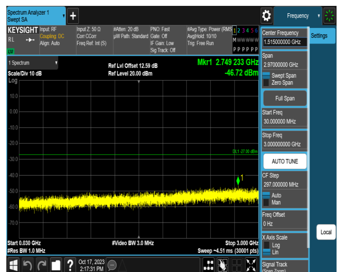
11AX80MIMO-Ant2-6625-30~3000-PASS
