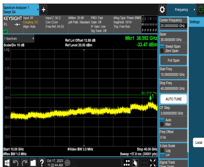
11AX80MIMO-Ant1-6465-10000~40000-PASS
