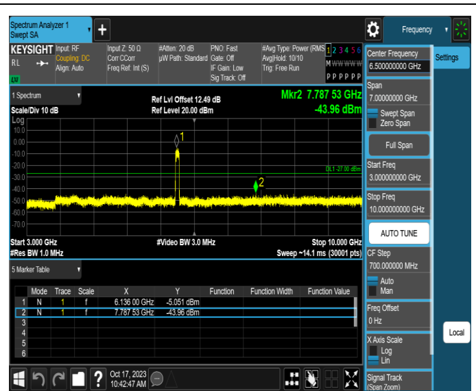
11AX80MIMO-Ant3-6145-3000~10000-PASS
