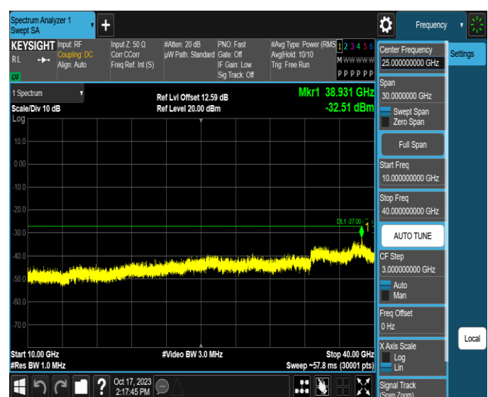
11AX80MIMO-Ant2-6625-10000~40000-PASS
