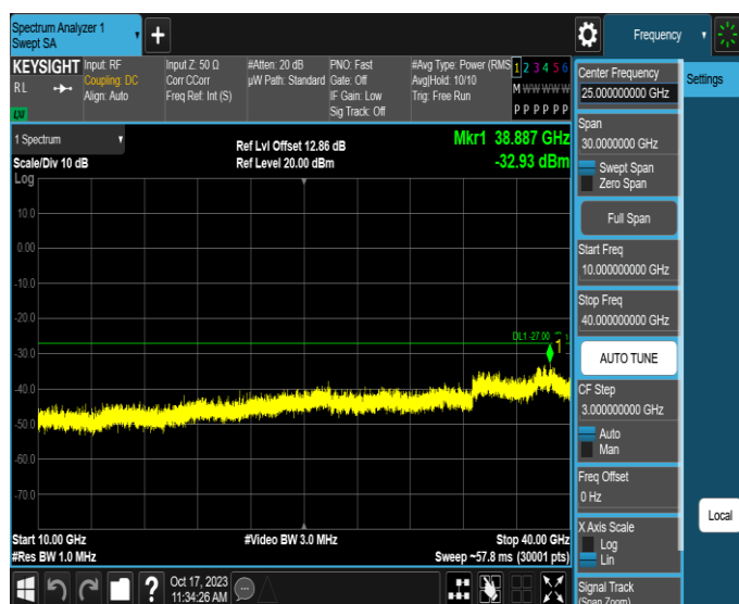
11AX80MIMO-Ant3-6465-10000~40000-PASS
