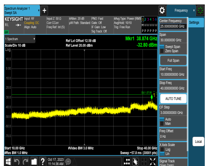
11AX80MIMO-Ant4-6385-10000~40000-PASS
