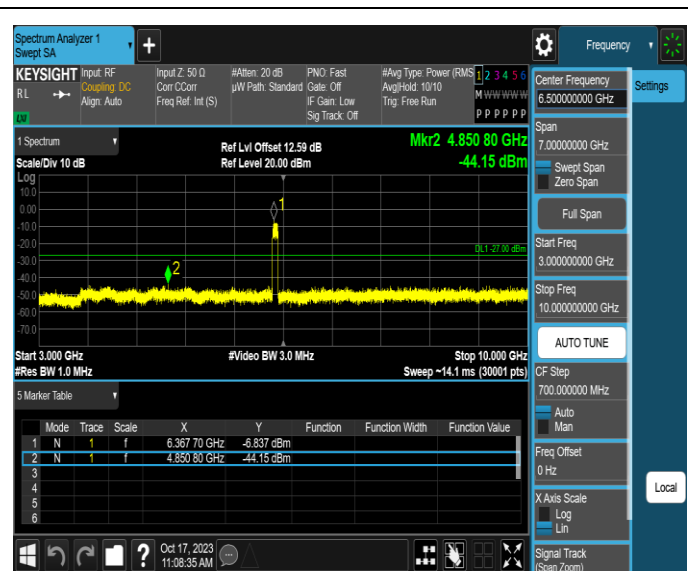
11AX80MIMO-Ant3-6385-3000~10000-PASS
