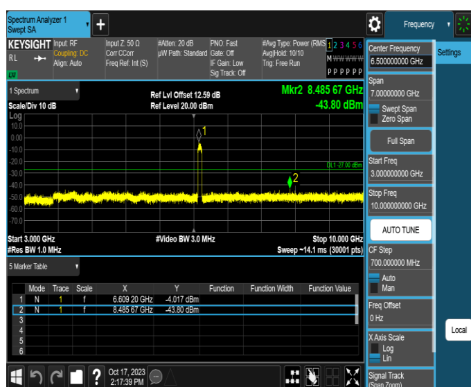
11AX80MIMO-Ant2-6625-3000~10000-PASS
