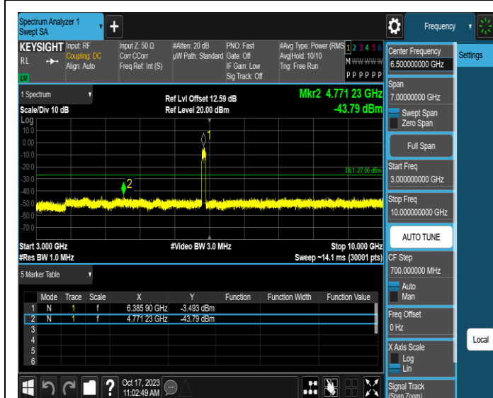
11AX80MIMO-Ant2-6385-3000~10000-PASS
