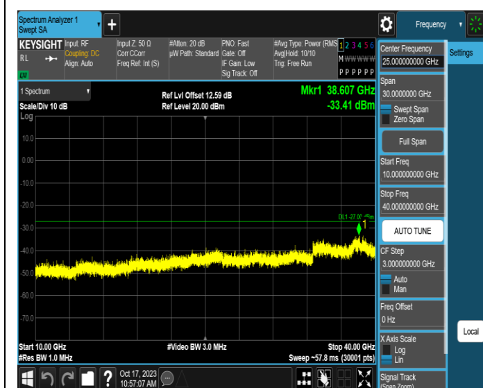
11AX80MIMO-Ant1-6385-10000~40000-PASS
