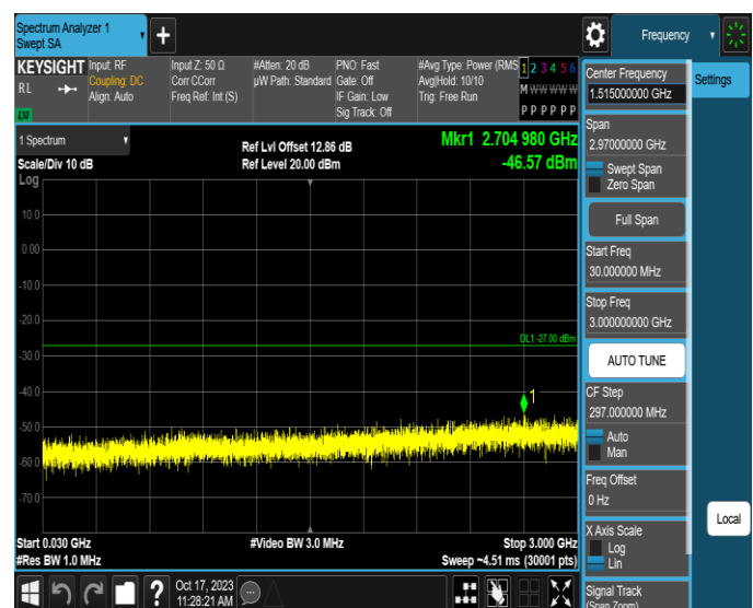
11AX80MIMO-Ant2-6465-30~3000-PASS
