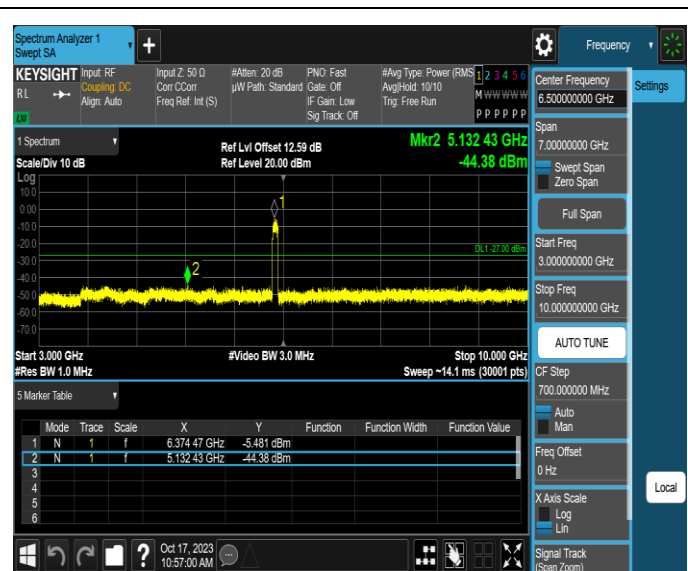
11AX80MIMO-Ant1-6385-3000~10000-PASS
