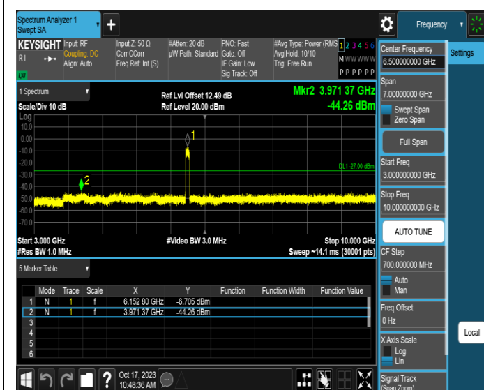
11AX80MIMO-Ant4-6145-3000~10000-PASS
