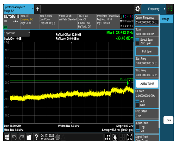
11AX80MIMO-Ant2-6465-10000~40000-PASS
