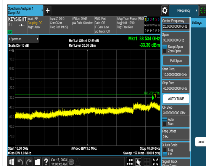
11AX80MIMO-Ant3-6385-10000~40000-PASS
