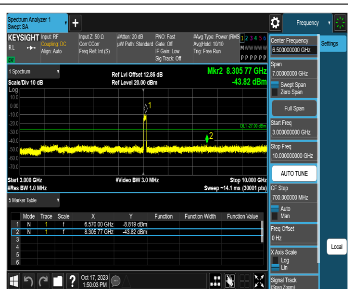
11AX80MIMO-Ant3-6545-3000~10000-PASS
