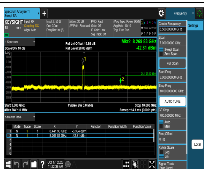
11AX80MIMO-Ant1-6465-3000~10000-PASS
