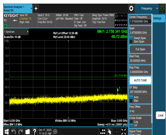
11AX80MIMO-Ant4-6385-30~3000-PASS
