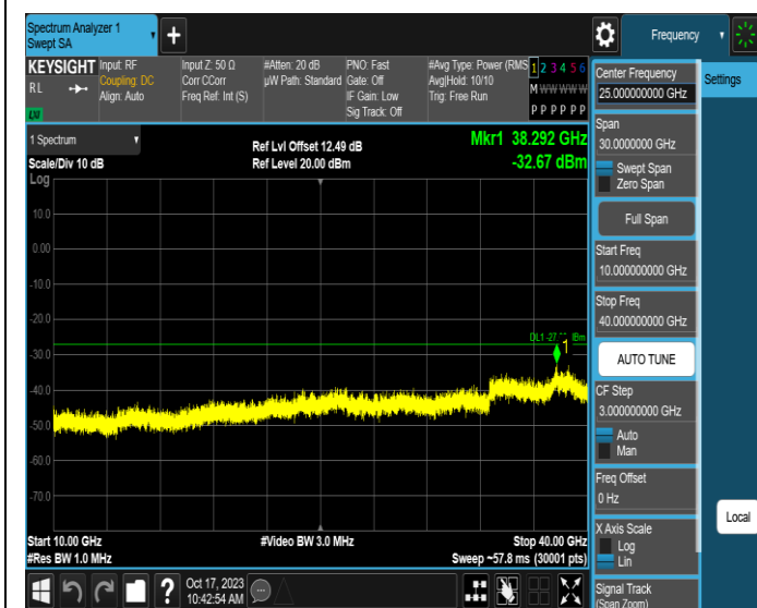
11AX80MIMO-Ant3-6145-10000~40000-PASS
