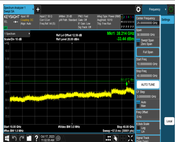
11AX80MIMO-Ant2-6385-10000~40000-PASS
