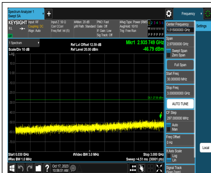
11AX80MIMO-Ant1-6385-30~3000-PASS
