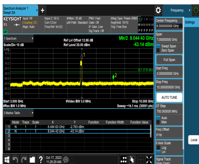
11AX80MIMO-Ant2-6465-3000~10000-PASS
