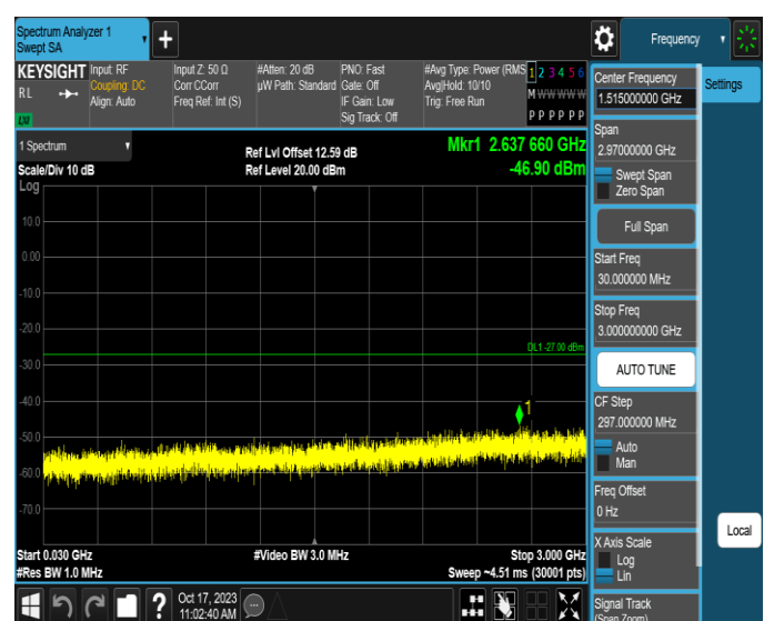
11AX80MIMO-Ant2-6385-30~3000-PASS
