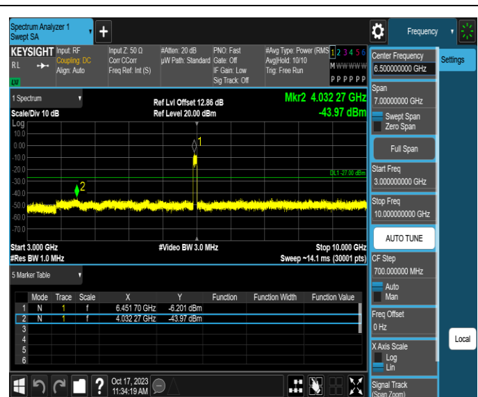
11AX80MIMO-Ant3-6465-3000~10000-PASS
