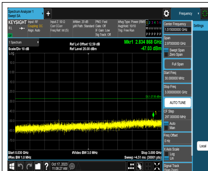
11AX80MIMO-Ant3-6385-30~3000-PASS
