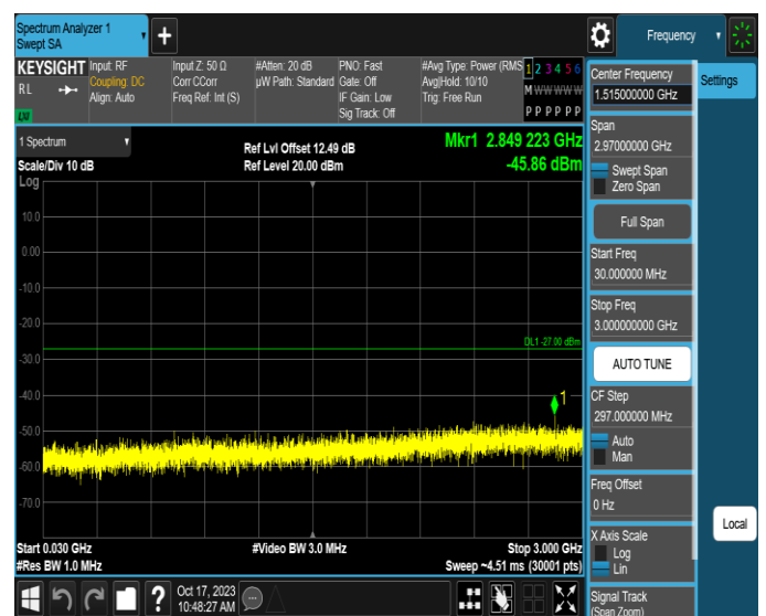
11AX80MIMO-Ant4-6145-30~3000-PASS
