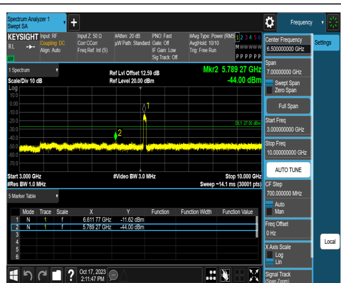
11AX80MIMO-Ant1-6625-3000~10000-PASS
