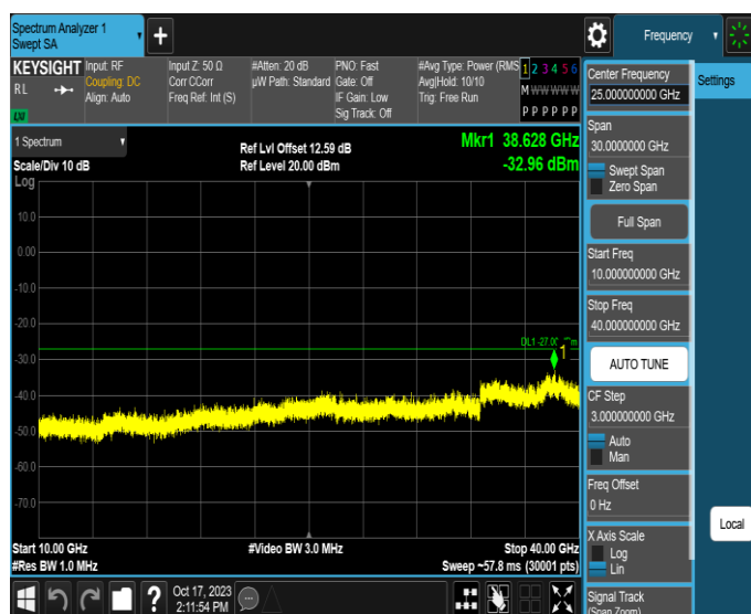
11AX80MIMO-Ant1-6625-10000~40000-PASS
