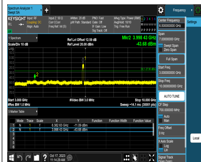
11AX80MIMO-Ant4-6385-3000~10000-PASS
