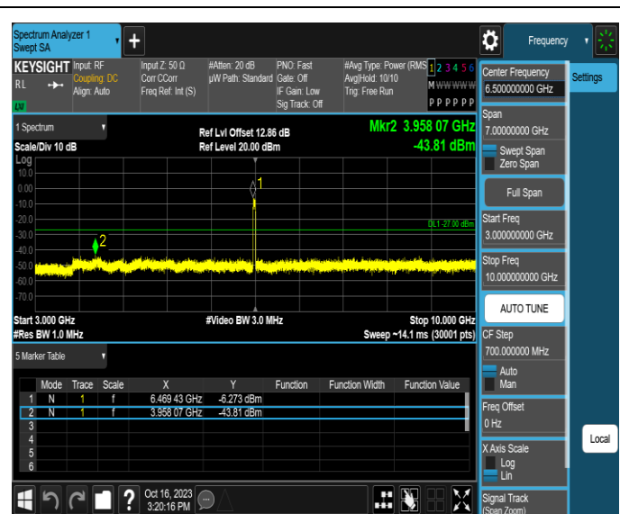
11AX40MIMO-Ant1-6485-3000~10000-PASS
