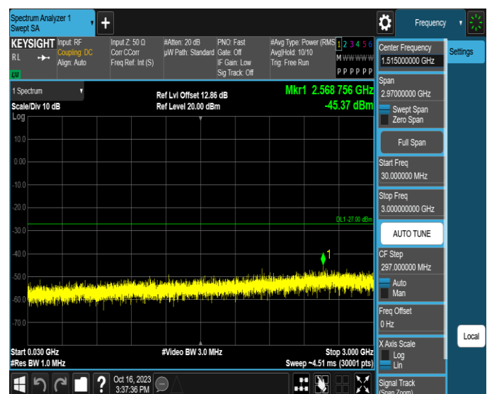
11AX40MIMO-Ant4-6485-30~3000-PASS
