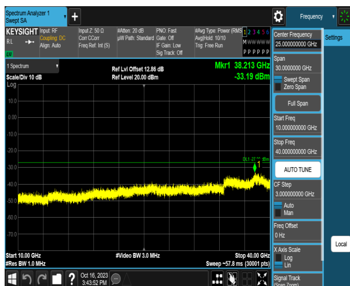
11AX40MIMO-Ant1-6525-10000~40000-PASS
