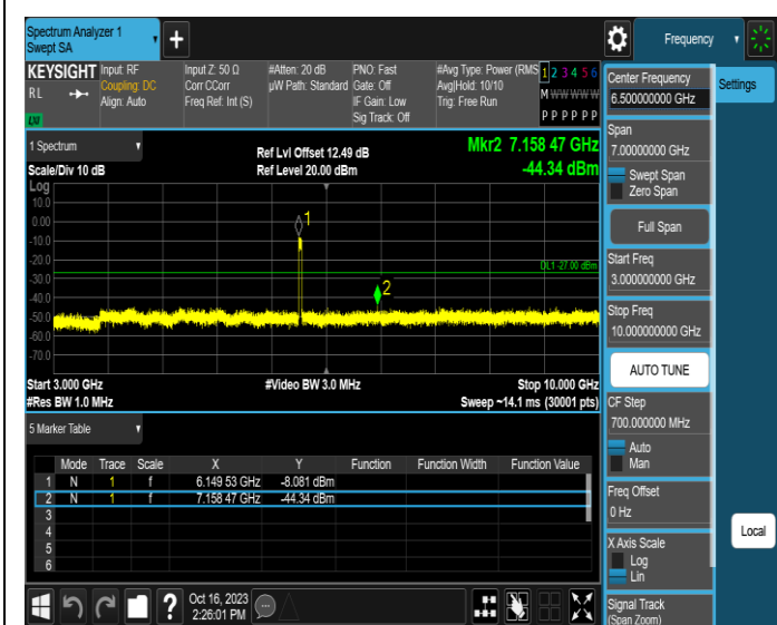
11AX40MIMO-Ant4-6165-3000~10000-PASS
