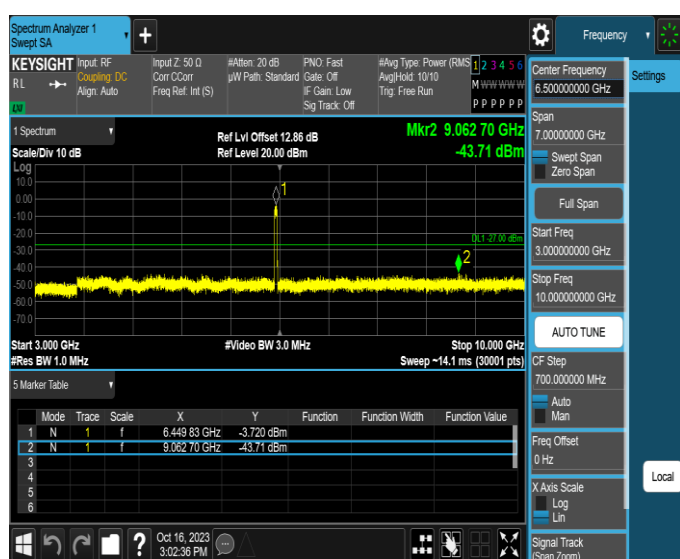
11AX40MIMO-Ant2-6445-3000~10000-PASS
