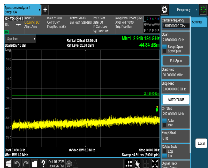
11AX40MIMO-Ant2-6525-30~3000-PASS
