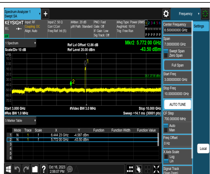
11AX40MIMO-Ant1-6445-3000~10000-PASS
