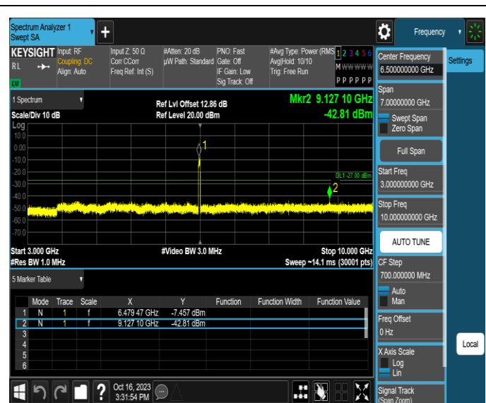
11AX40MIMO-Ant3-6485-3000~10000-PASS
