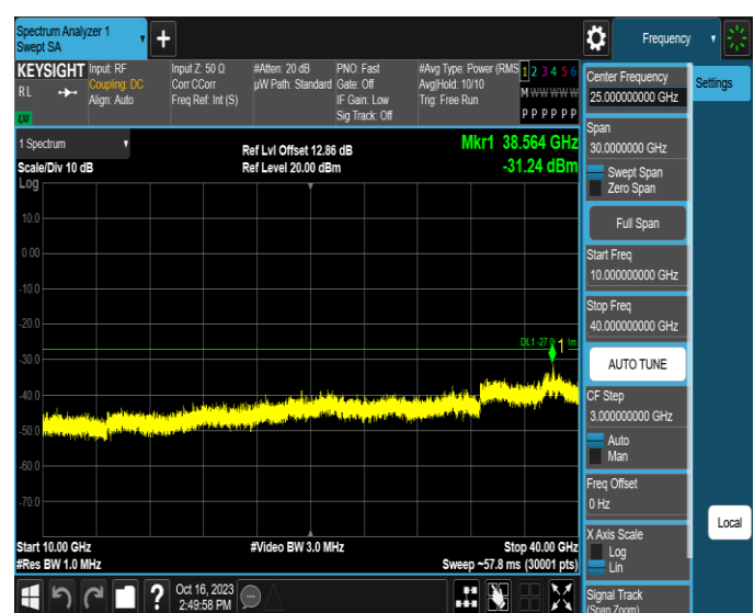
11AX40MIMO-Ant4-6405-10000~40000-PASS
