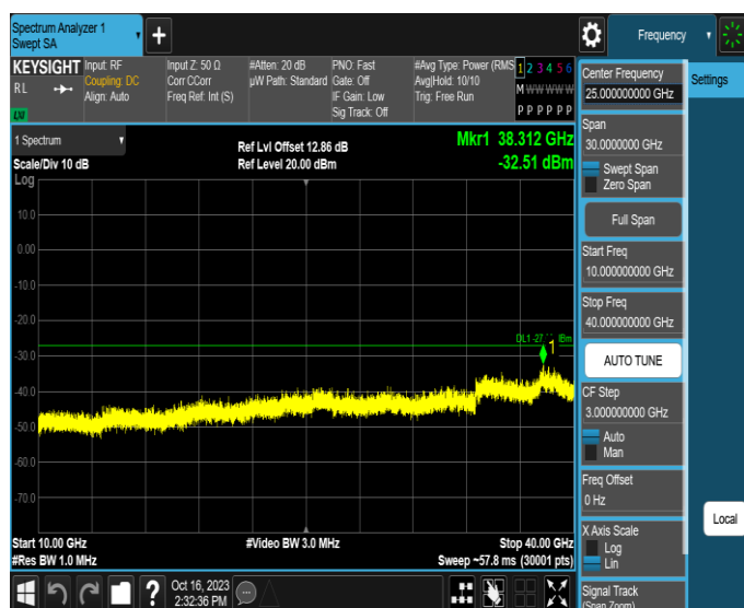
11AX40MIMO-Ant1-6405-10000~40000-PASS
