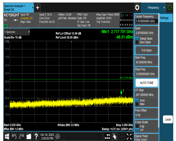
11AX40MIMO-Ant4-6165-30~3000-PASS
