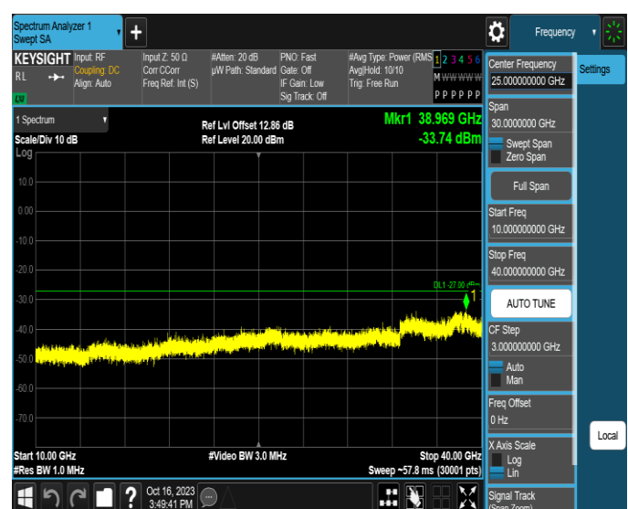
11AX40MIMO-Ant2-6525-10000~40000-PASS
