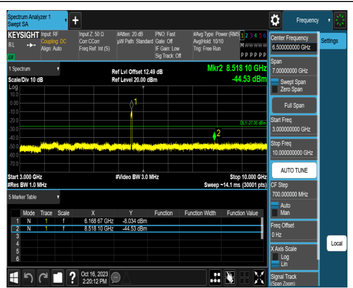
11AX40MIMO-Ant3-6165-3000~10000-PASS
