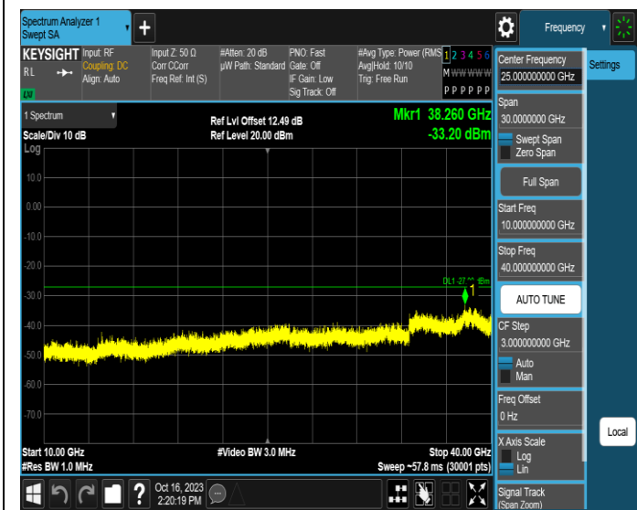
11AX40MIMO-Ant3-6165-10000~40000-PASS
