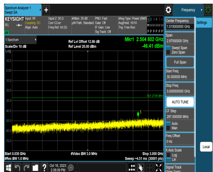
11AX40MIMO-Ant2-6405-30~3000-PASS
