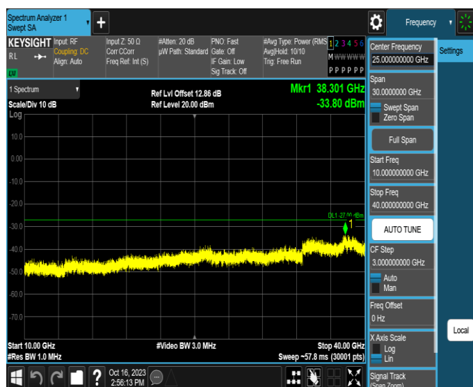
11AX40MIMO-Ant1-6445-10000~40000-PASS
