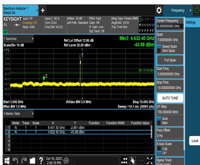
11AX40MIMO-Ant2-6405-3000~10000-PASS
