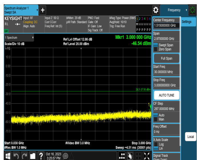
11AX40MIMO-Ant2-6485-30~3000-PASS
