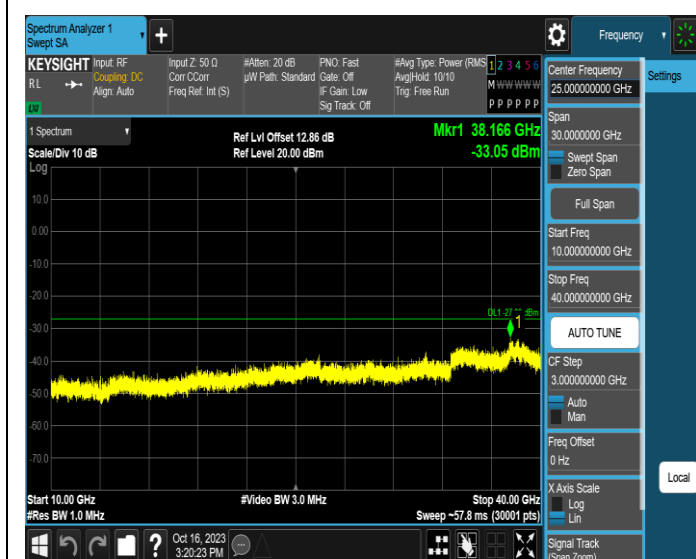
11AX40MIMO-Ant1-6485-10000~40000-PASS
