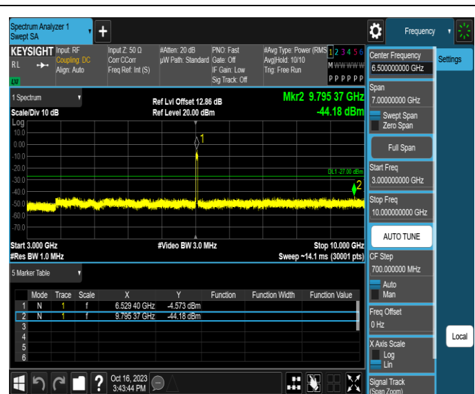
11AX40MIMO-Ant1-6525-3000~10000-PASS
