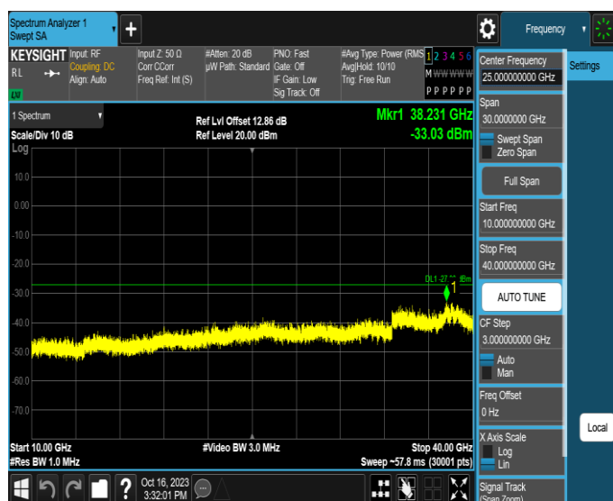
11AX40MIMO-Ant3-6485-10000~40000-PASS
