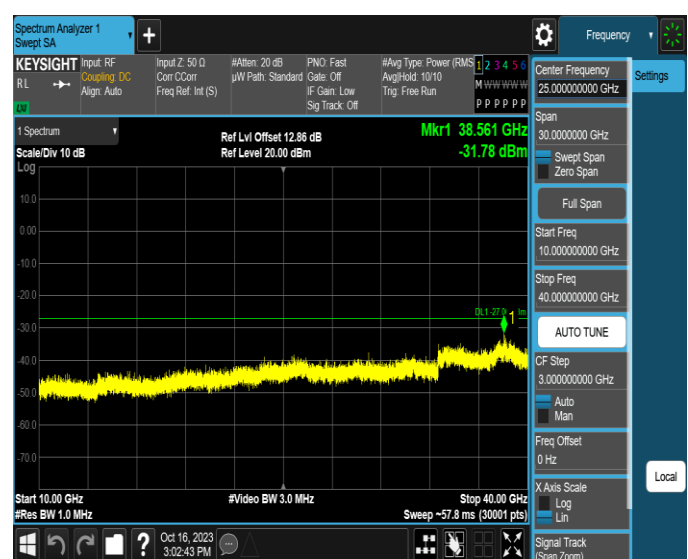
11AX40MIMO-Ant2-6445-10000~40000-PASS
