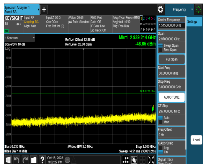
11AX40MIMO-Ant2-6445-30~3000-PASS
