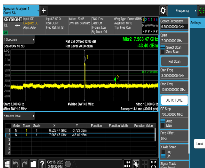
11AX40MIMO-Ant2-6525-3000~10000-PASS
