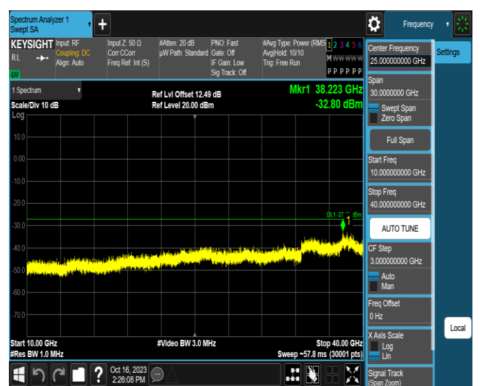
11AX40MIMO-Ant4-6165-10000~40000-PASS
