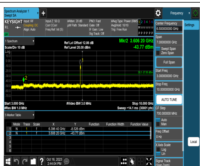
11AX40MIMO-Ant3-6405-3000~10000-PASS
