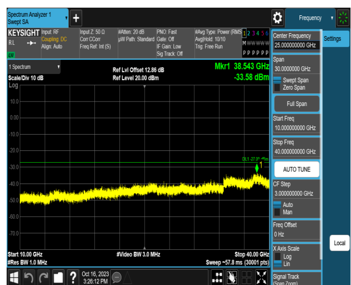
11AX40MIMO-Ant2-6485-10000~40000-PASS
