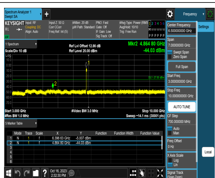
11AX40MIMO-Ant1-6405-3000~10000-PASS
