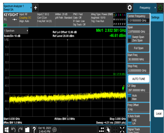
11AX40MIMO-Ant4-6405-30~3000-PASS
