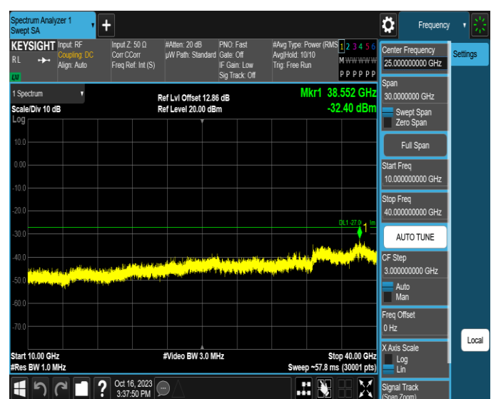
11AX40MIMO-Ant4-6485-10000~40000-PASS
