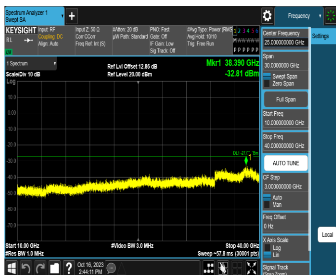
11AX40MIMO-Ant3-6405-10000~40000-PASS
