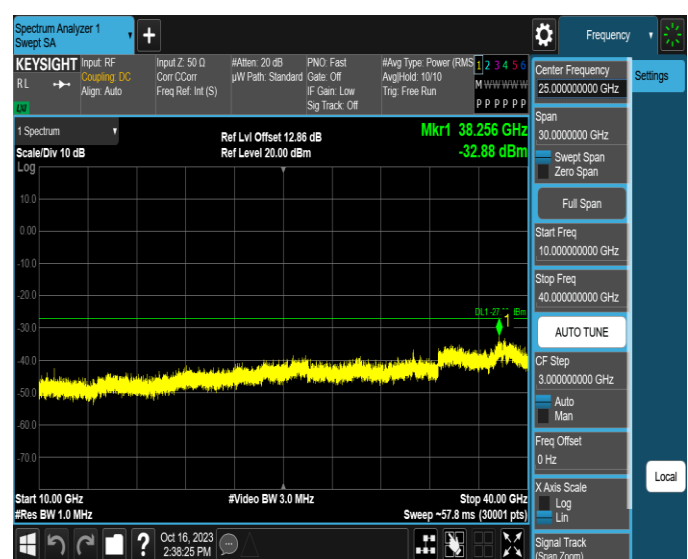
11AX40MIMO-Ant2-6405-10000~40000-PASS
