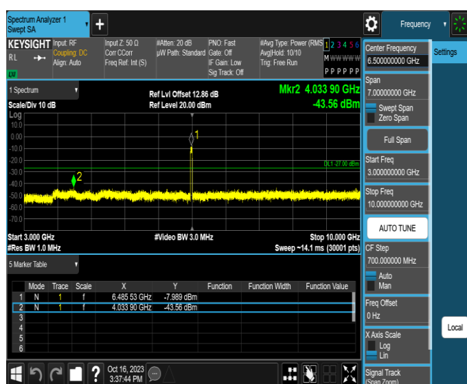
11AX40MIMO-Ant4-6485-3000~10000-PASS
