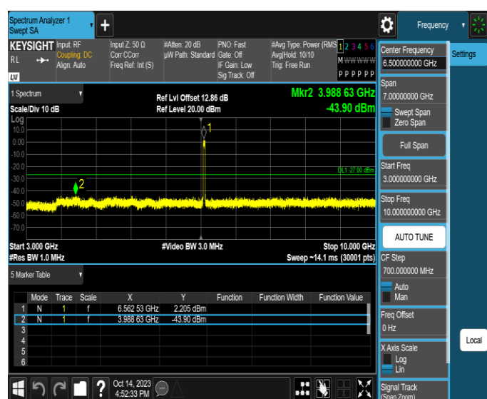
11AX40SISO-Ant4-6565-3000~10000-PASS
