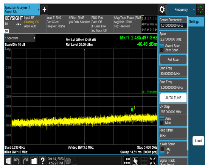
11AX40SISO-Ant4-6565-30~3000-PASS
