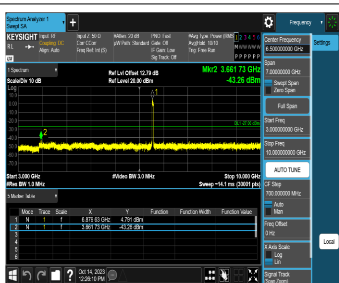
11AX40SISO-Ant3-6885-3000~10000-PASS
