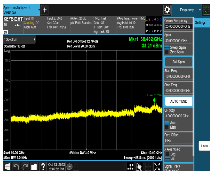
11AX40SISO-Ant1-6885-10000~40000-PASS
