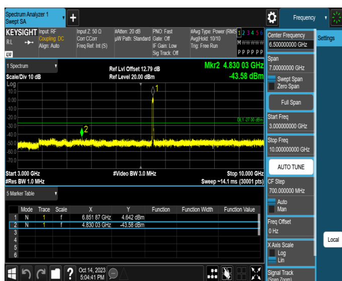
11AX40SISO-Ant4-6845-3000~10000-PASS
