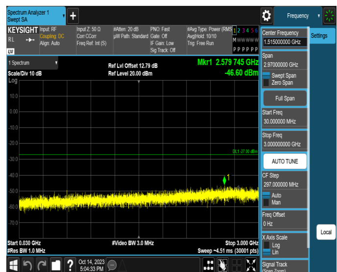
11AX40SISO-Ant4-6845-30~3000-PASS
