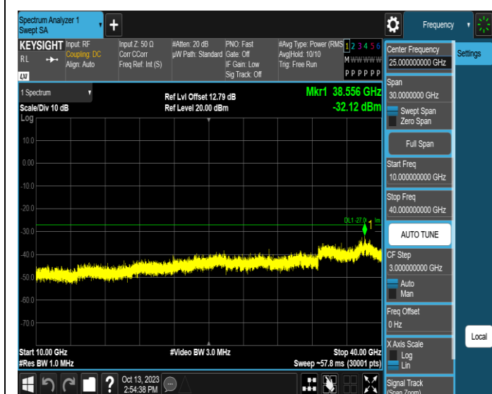
11AX40SISO-Ant1-6925-10000~40000-PASS
