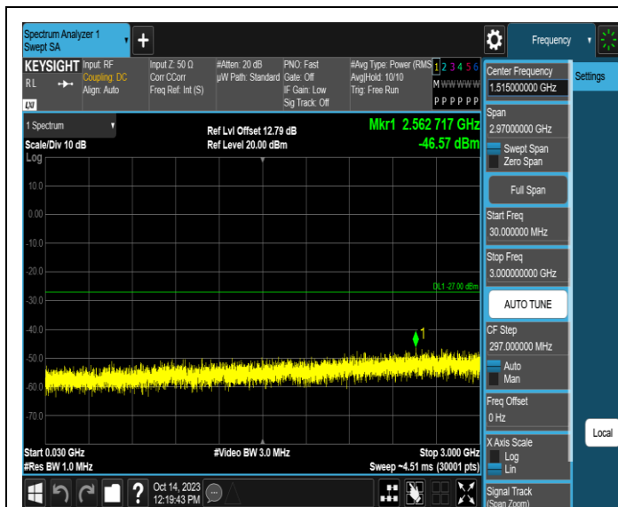
11AX40SISO-Ant3-6845-30~3000-PASS
