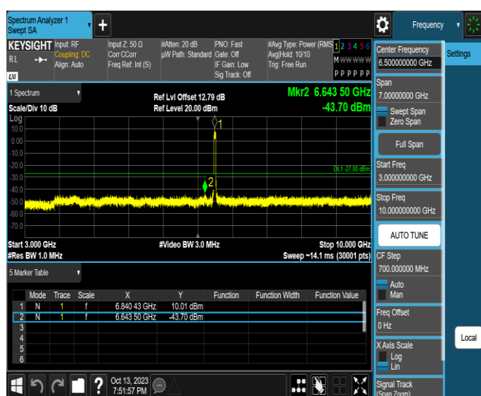
11AX40SISO-Ant2-6845-3000~10000-PASS
