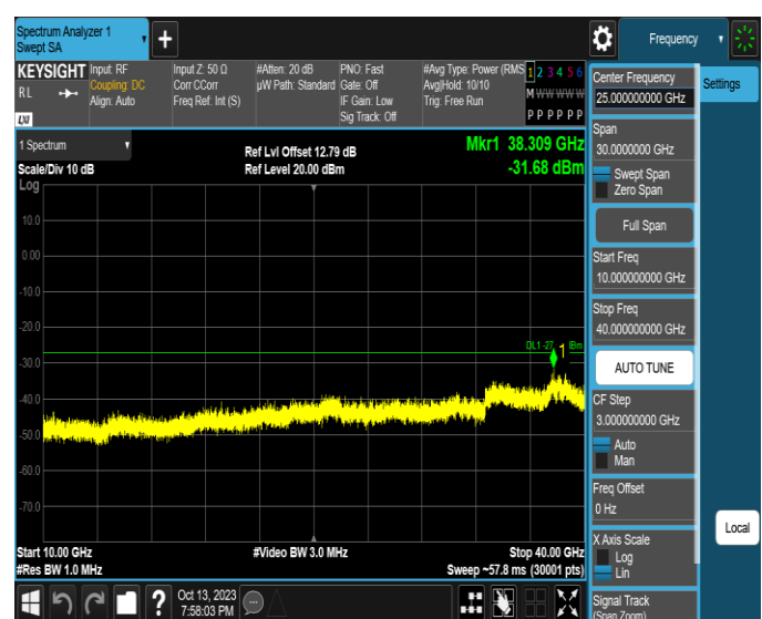
11AX40SISO-Ant2-6885-10000~40000-PASS
