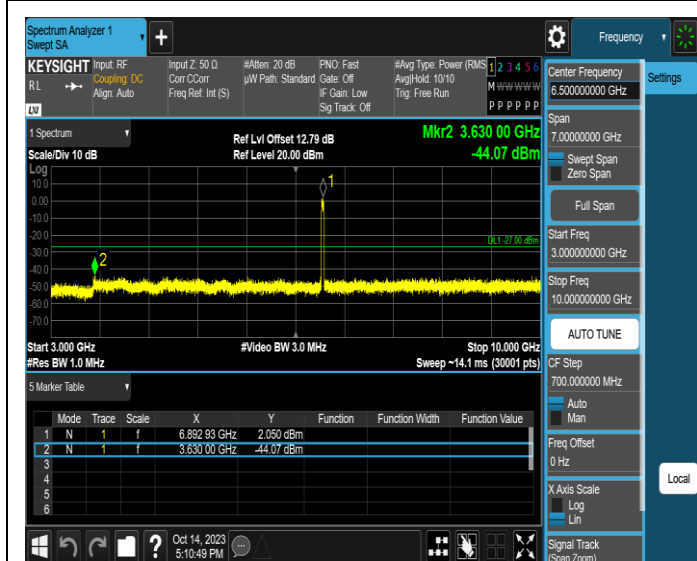
11AX40SISO-Ant4-6885-3000~10000-PASS
