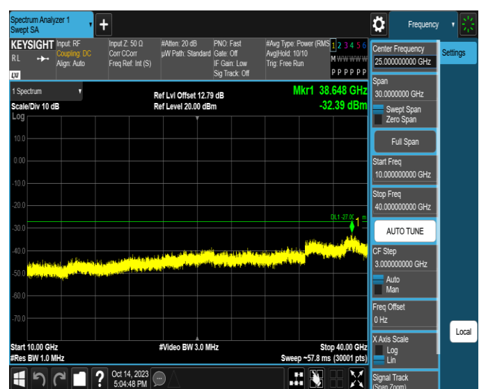
11AX40SISO-Ant4-6845-10000~40000-PASS
