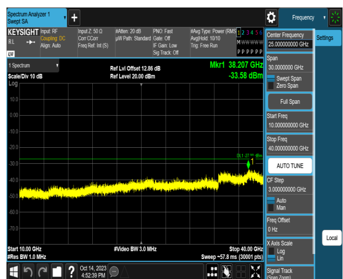
11AX40SISO-Ant4-6565-10000~40000-PASS
