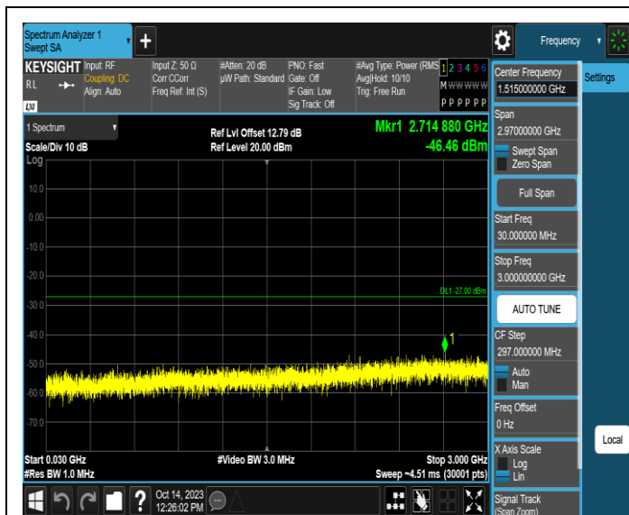
11AX40SISO-Ant3-6885-30~3000-PASS
