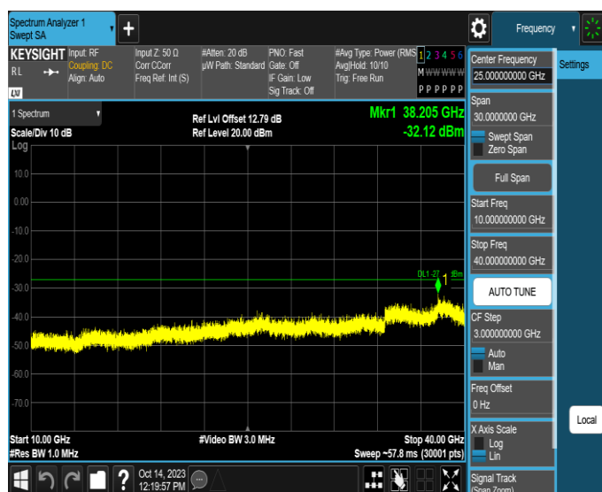
11AX40SISO-Ant3-6845-10000~40000-PASS
