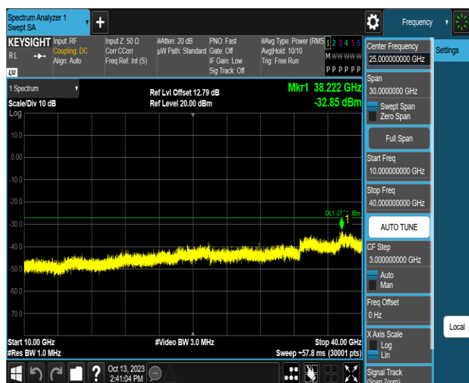
11AX40SISO-Ant1-6845-10000~40000-PASS
