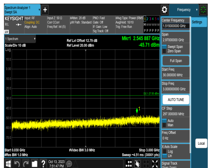
11AX40SISO-Ant2-6845-30~3000-PASS
