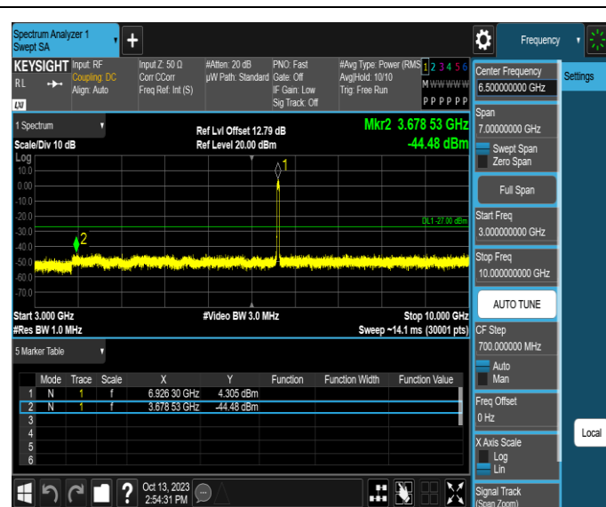
11AX40SISO-Ant1-6925-3000~10000-PASS
