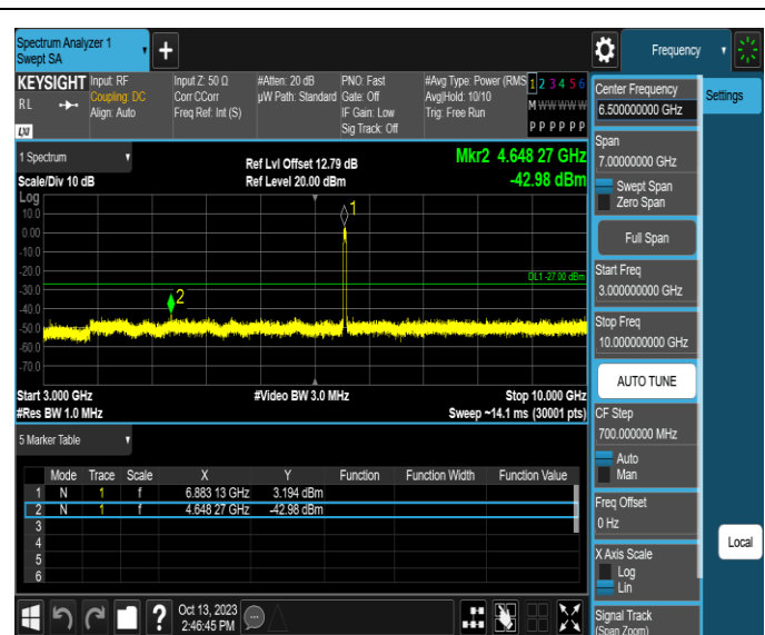
11AX40SISO-Ant1-6885-3000~10000-PASS
