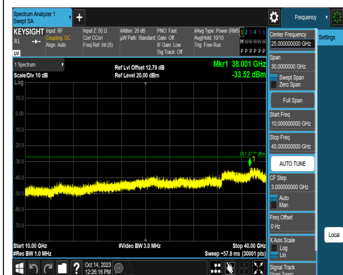
11AX40SISO-Ant3-6885-10000~40000-PASS
