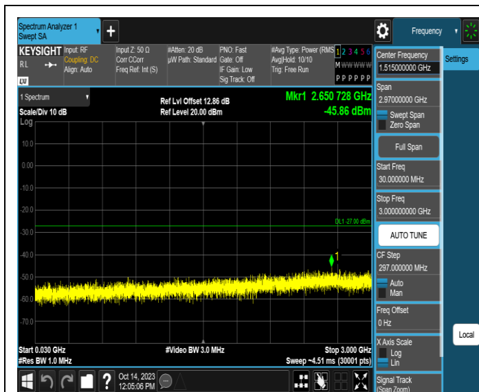
11AX40SISO-Ant3-6565-30~3000-PASS
