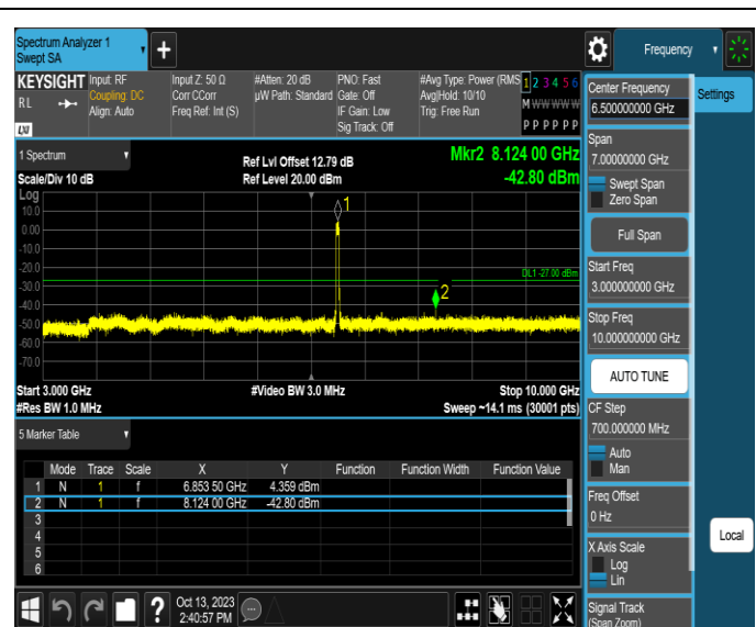
11AX40SISO-Ant1-6845-3000~10000-PASS
