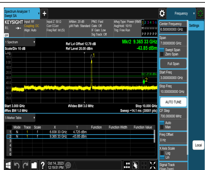
11AX40SISO-Ant3-6845-3000~10000-PASS
