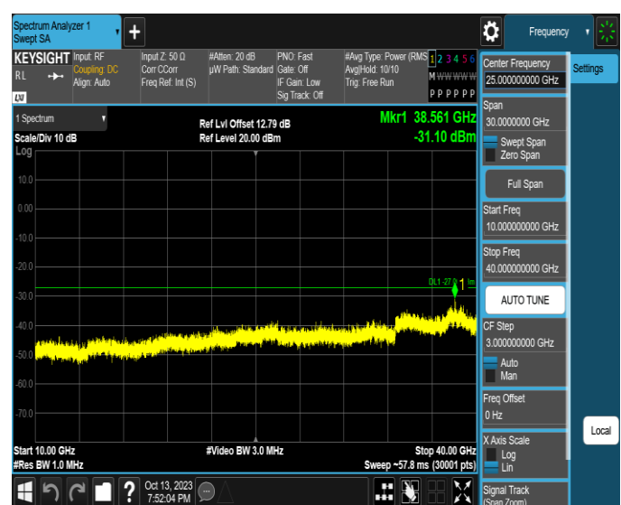
11AX40SISO-Ant2-6845-10000~40000-PASS
