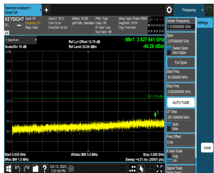
11AX40SISO-Ant2-6885-30~3000-PASS
