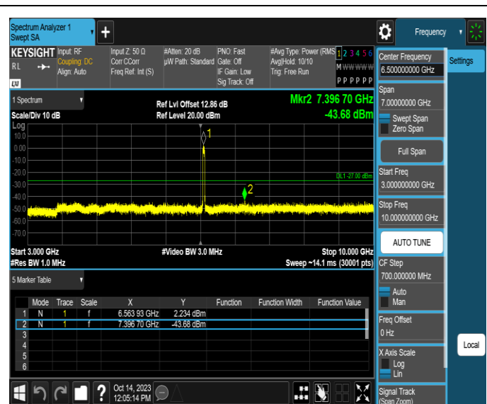
11AX40SISO-Ant3-6565-3000~10000-PASS
