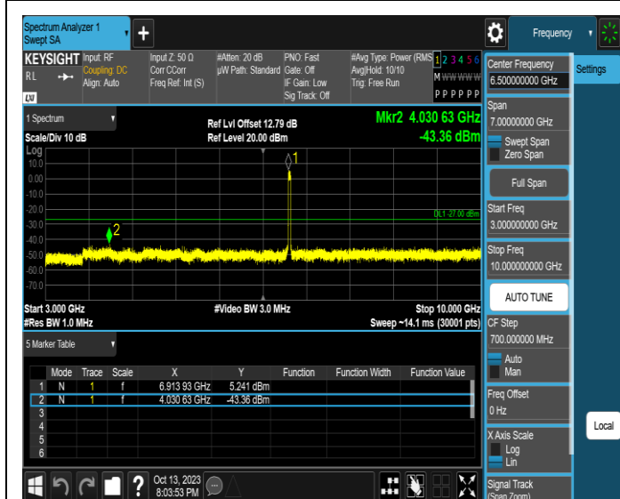
11AX40SISO-Ant2-6925-3000~10000-PASS
