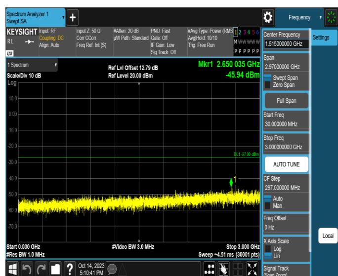
11AX40SISO-Ant4-6885-30~3000-PASS
