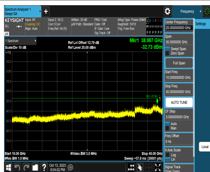
11AX40SISO-Ant2-6925-10000~40000-PASS
