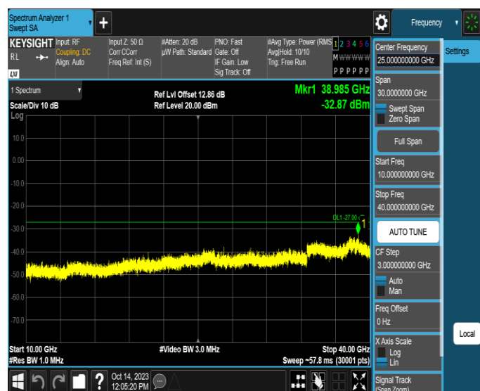
11AX40SISO-Ant3-6565-10000~40000-PASS
