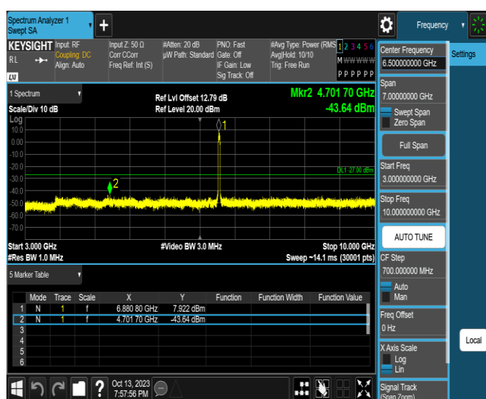
11AX40SISO-Ant2-6885-3000~10000-PASS
