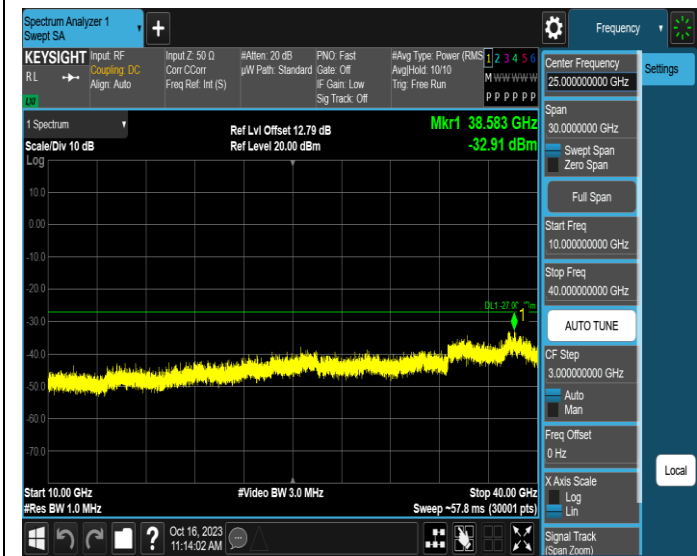
11AX20MIMO-Ant3-6995-10000~40000-PASS
