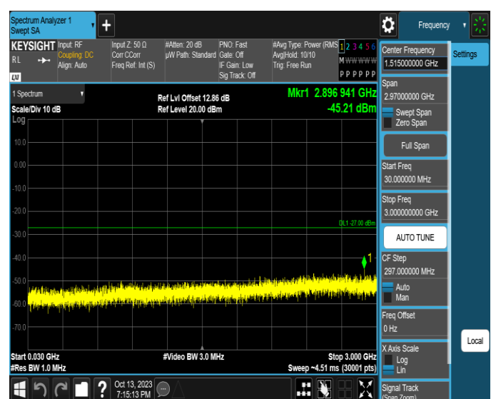
11AX40SISO-Ant2-6405-30~3000-PASS
