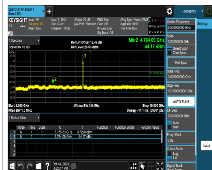
11AX40SISO-Ant4-6165-3000~10000-PASS
