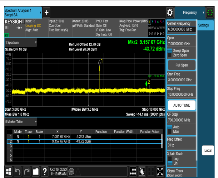
11AX20MIMO-Ant3-6995-3000~10000-PASS
