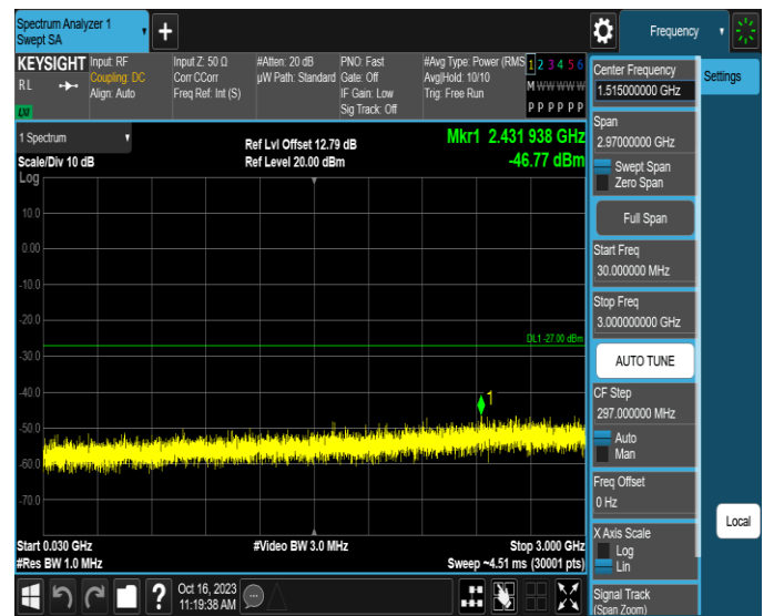
11AX20MIMO-Ant4-6995-30~3000-PASS
