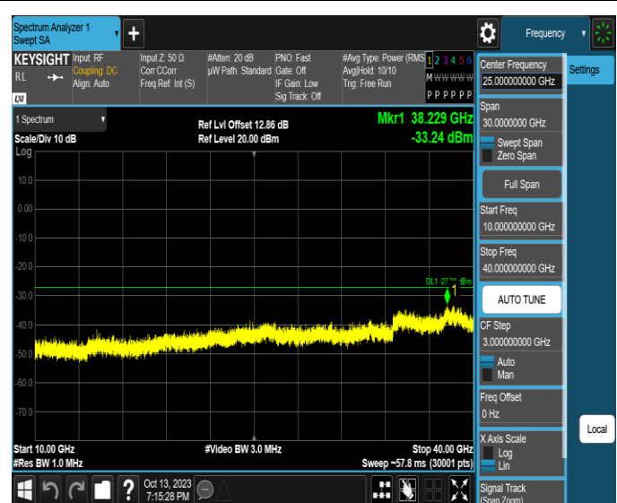
11AX40SISO-Ant2-6405-10000~40000-PASS
