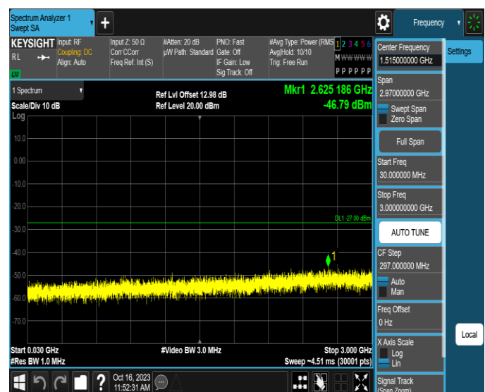
11AX20MIMO-Ant4-7115-30~3000-PASS
