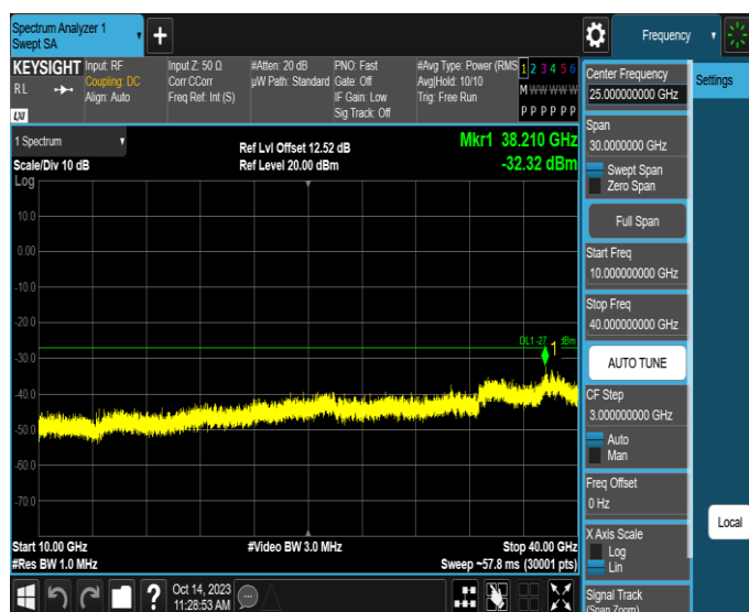
11AX40SISO-Ant3-5965-10000~40000-PASS
