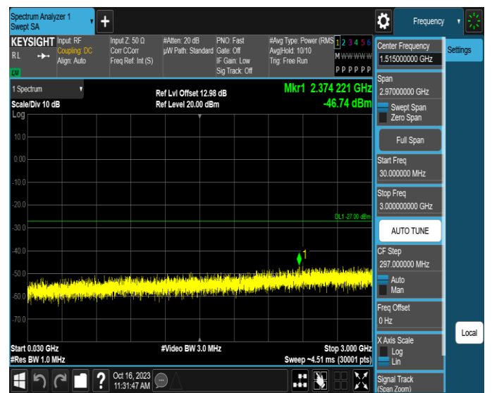
11AX20MIMO-Ant2-7115-30~3000-PASS
