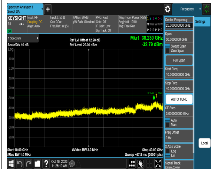
11AX20MIMO-Ant1-7115-10000~40000-PASS
