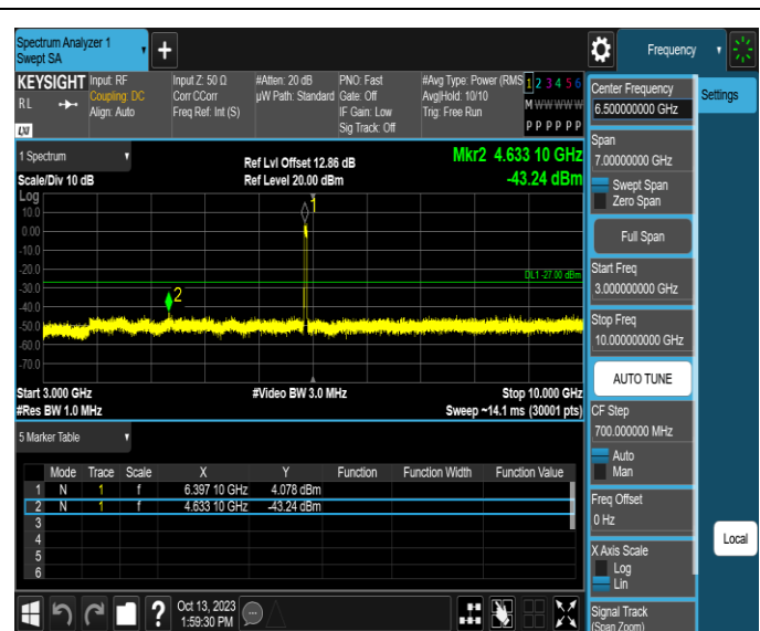
11AX40SISO-Ant1-6405-3000~10000-PASS
