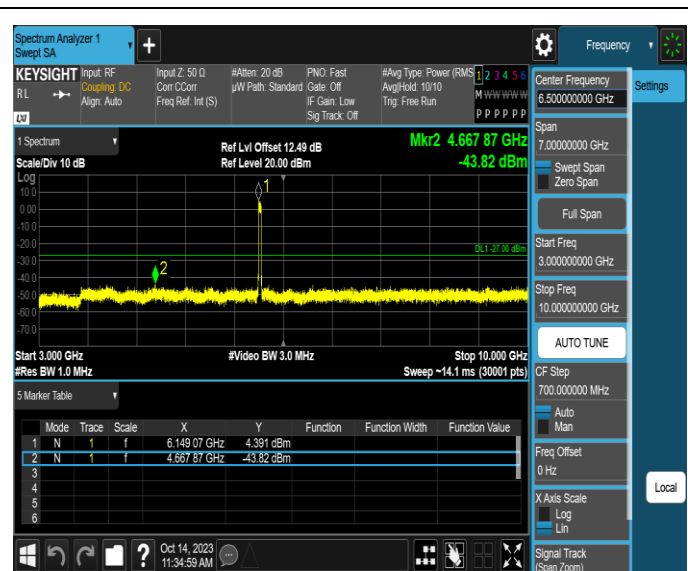
11AX40SISO-Ant3-6165-3000~10000-PASS
