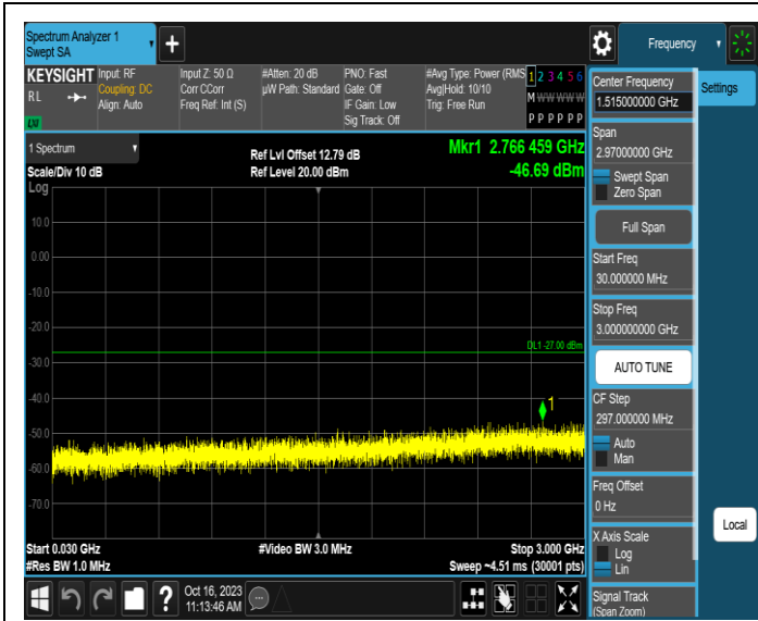
11AX20MIMO-Ant3-6995-30~3000-PASS
