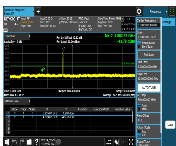
11AX40SISO-Ant3-5965-3000~10000-PASS
