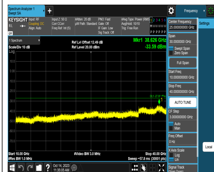
11AX40SISO-Ant3-6165-10000~40000-PASS
