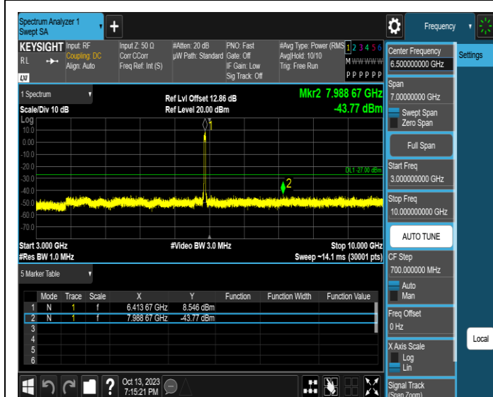
11AX40SISO-Ant2-6405-3000~10000-PASS
