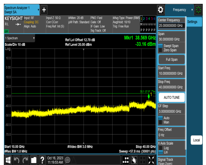
11AX20MIMO-Ant4-6995-10000~40000-PASS
