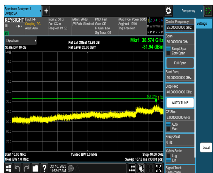
11AX20MIMO-Ant4-7115-10000~40000-PASS
