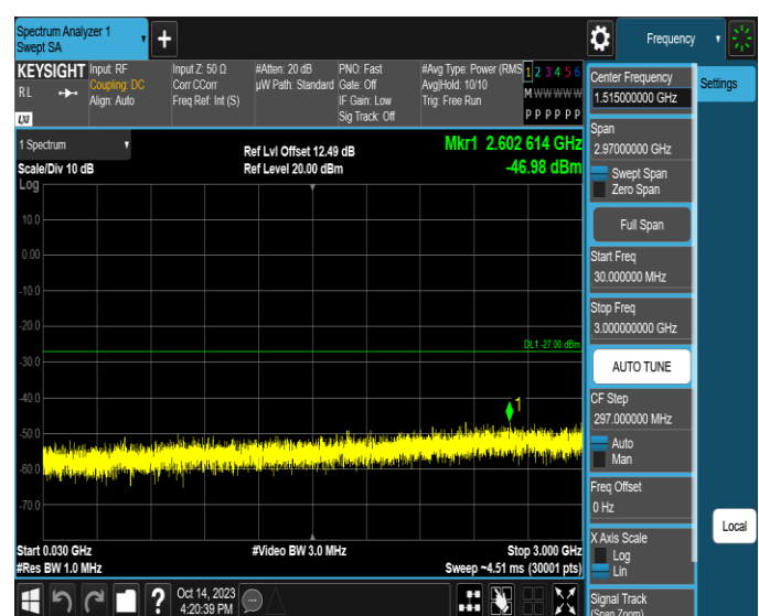
11AX40SISO-Ant4-6165-30~3000-PASS
