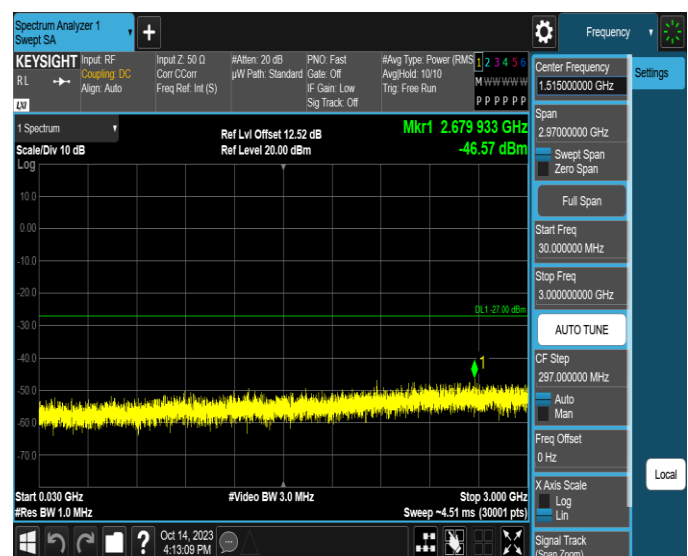
11AX40SISO-Ant4-5965-30~3000-PASS
