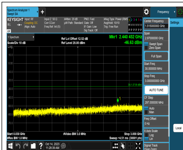
11AX40SISO-Ant3-5965-30~3000-PASS
