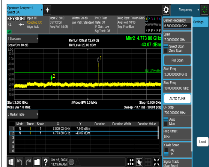
11AX20MIMO-Ant4-6995-3000~10000-PASS
