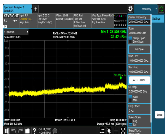
11AX40SISO-Ant4-6165-10000~40000-PASS
