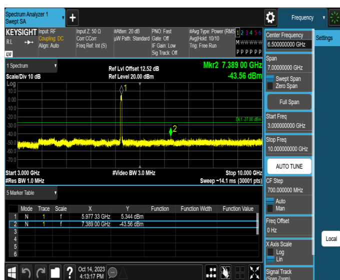
11AX40SISO-Ant4-5965-3000~10000-PASS
