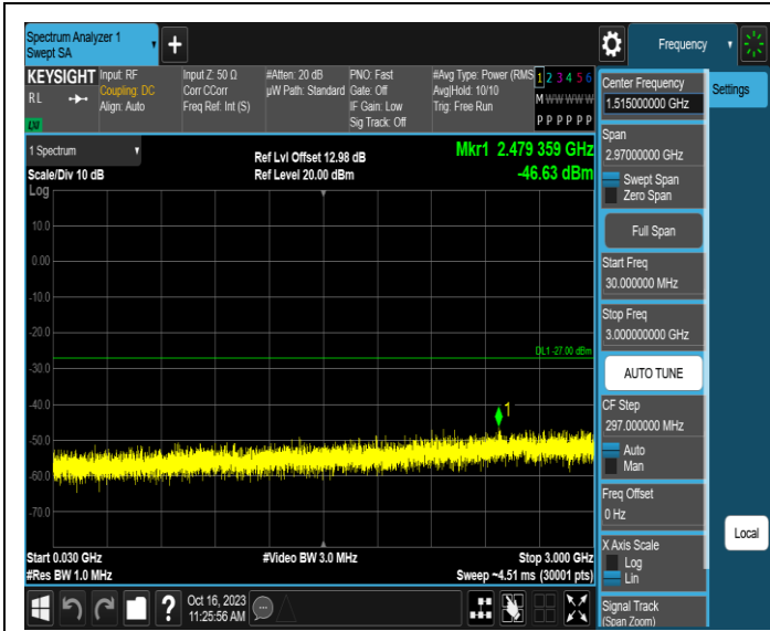
11AX20MIMO-Ant1-7115-30~3000-PASS
