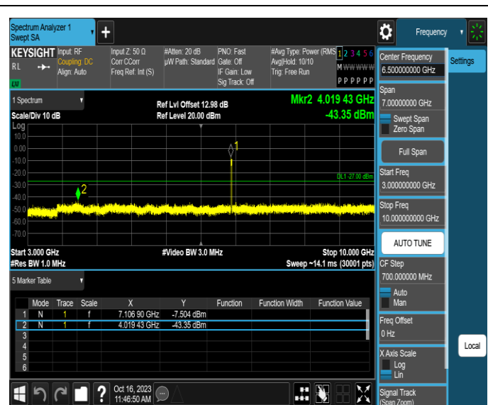
11AX20MIMO-Ant3-7115-3000~10000-PASS
