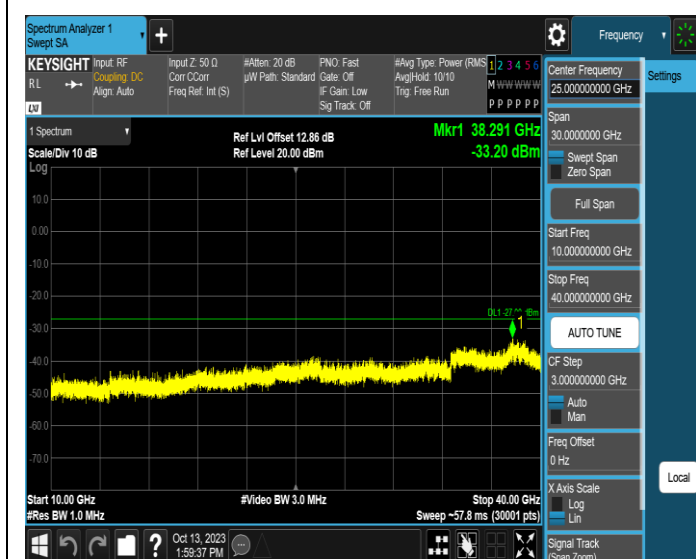
11AX40SISO-Ant1-6405-10000~40000-PASS
