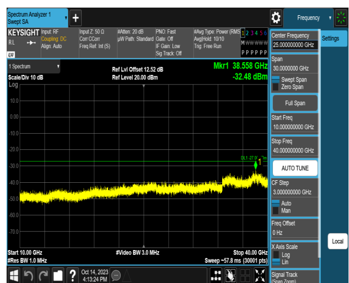
11AX40SISO-Ant4-5965-10000~40000-PASS
