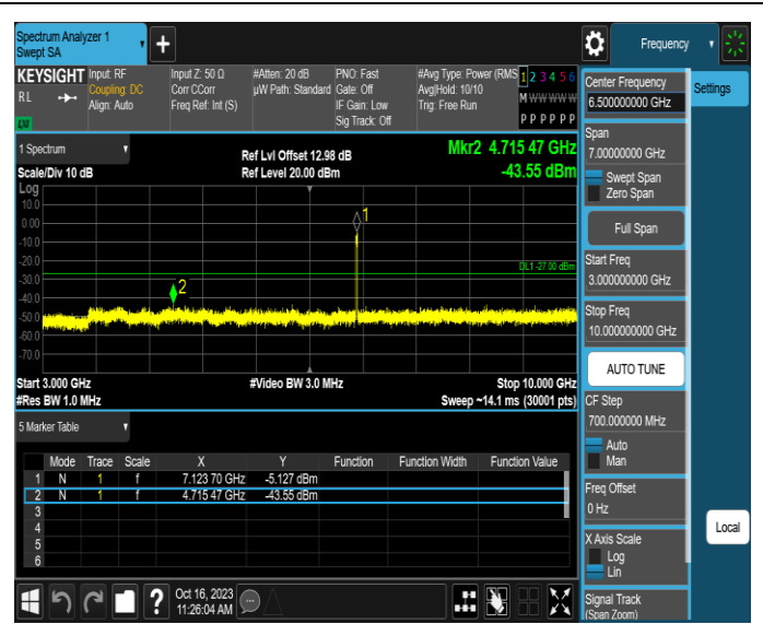
11AX20MIMO-Ant1-7115-3000~10000-PASS
