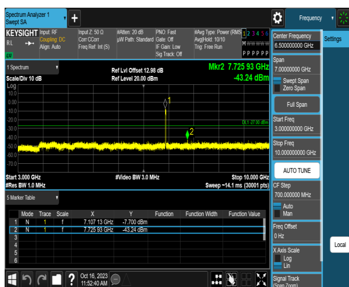
11AX20MIMO-Ant4-7115-3000~10000-PASS
