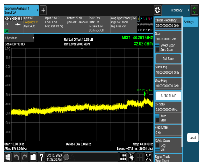
11AX20MIMO-Ant2-7115-10000~40000-PASS
