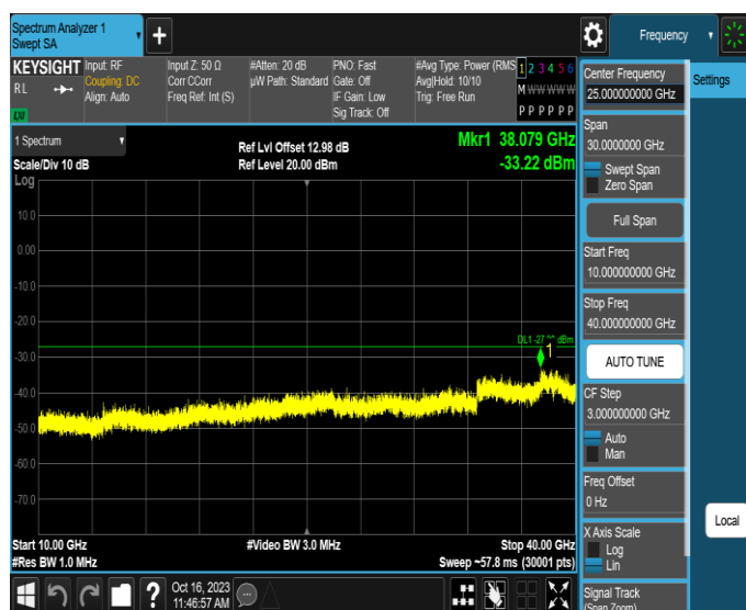
11AX20MIMO-Ant3-7115-10000~40000-PASS
