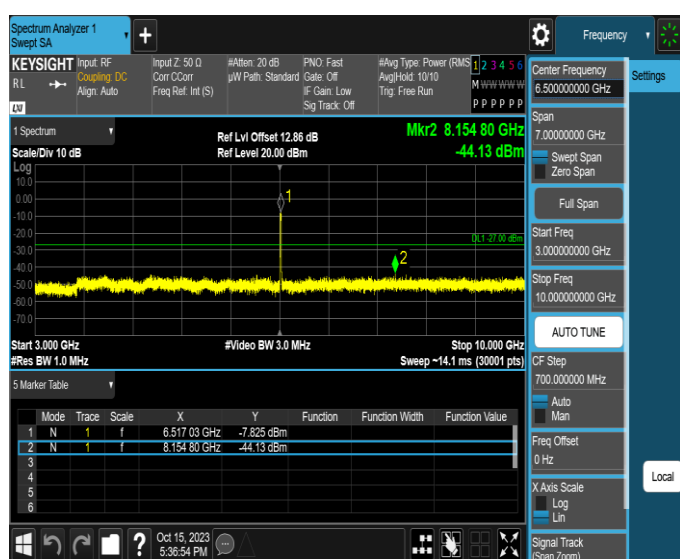
11AX20MIMO-Ant4-6515-3000~10000-PASS
