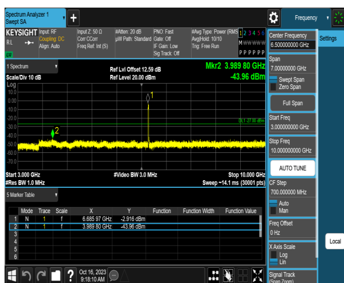
11AX20MIMO-Ant2-6695-3000~10000-PASS
