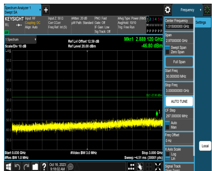
11AX20MIMO-Ant2-6695-30~3000-PASS
