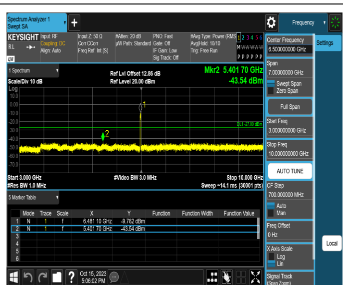
11AX20MIMO-Ant3-6475-3000~10000-PASS
