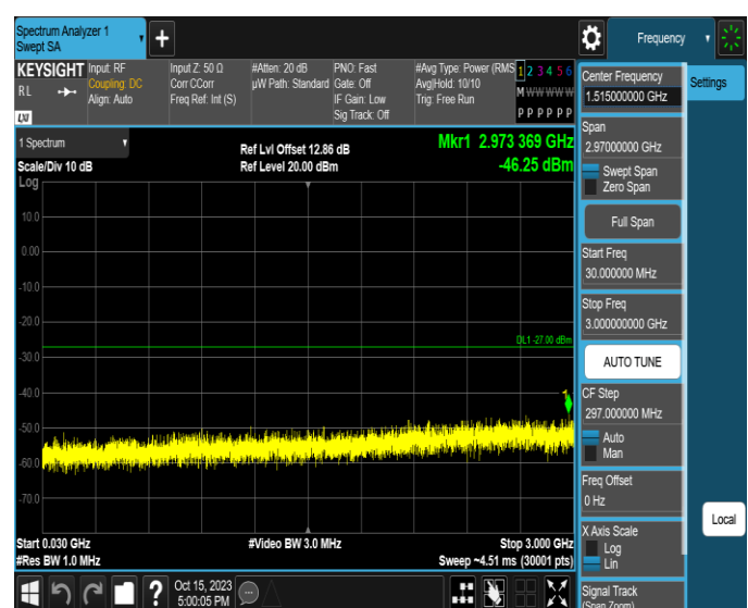
11AX20MIMO-Ant2-6475-30~3000-PASS
