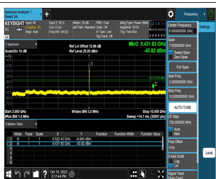
11AX20MIMO-Ant1-6515-3000~10000-PASS
