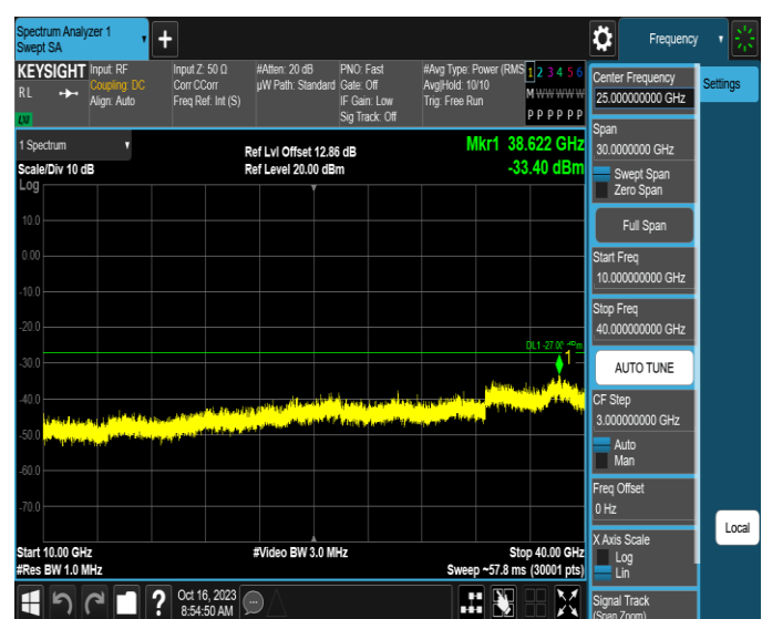
11AX20MIMO-Ant2-6535-10000~40000-PASS
