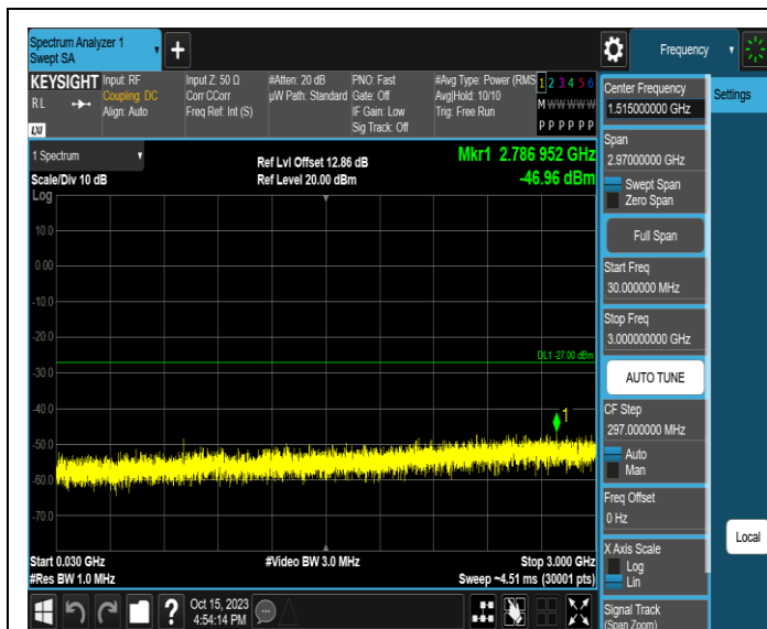
11AX20MIMO-Ant1-6475-30~3000-PASS
