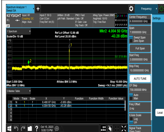
11AX20MIMO-Ant2-6475-3000~10000-PASS
