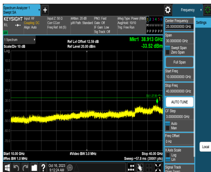
11AX20MIMO-Ant1-6695-10000~40000-PASS
