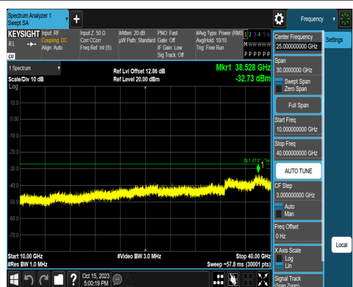
11AX20MIMO-Ant2-6475-10000~40000-PASS
