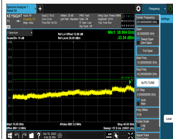
11AX20MIMO-Ant1-6475-10000~40000-PASS
