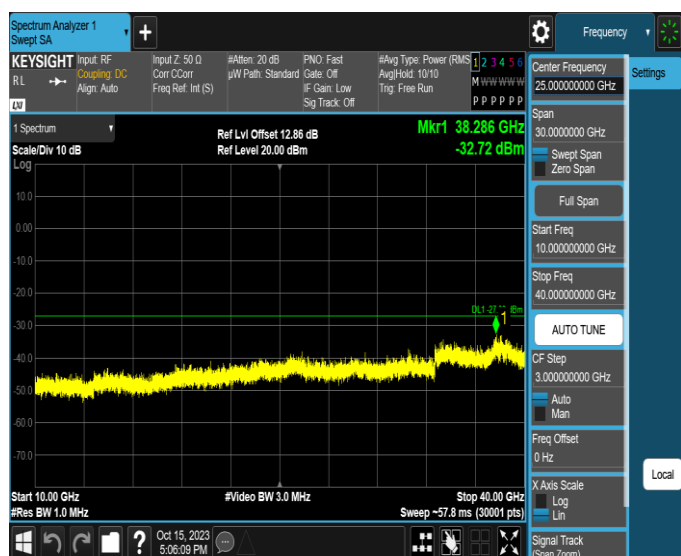
11AX20MIMO-Ant3-6475-10000~40000-PASS
