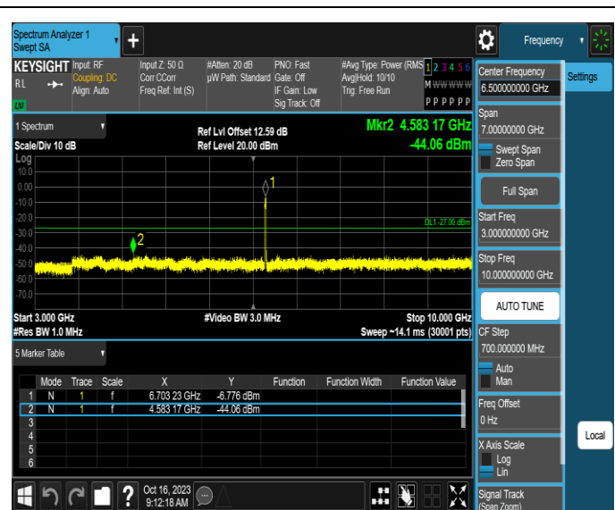
11AX20MIMO-Ant1-6695-3000~10000-PASS
