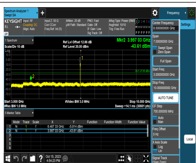
11AX20MIMO-Ant1-6475-3000~10000-PASS
