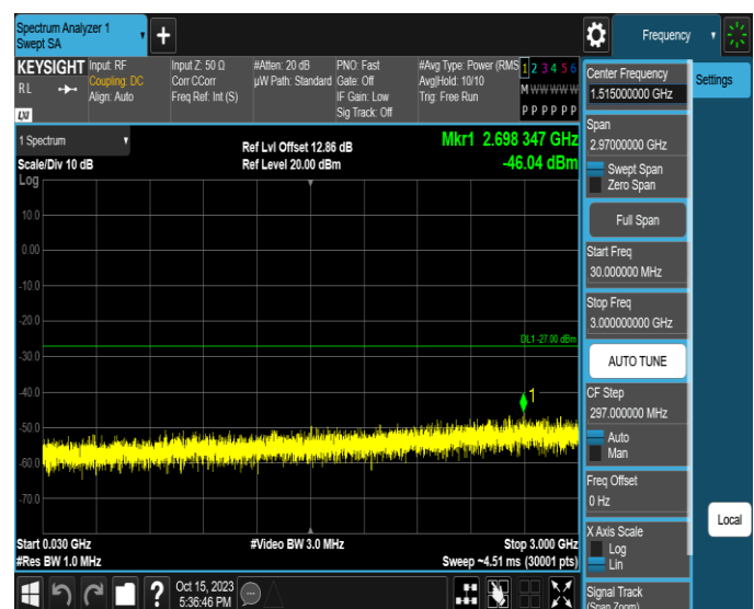
11AX20MIMO-Ant4-6515-30~3000-PASS
