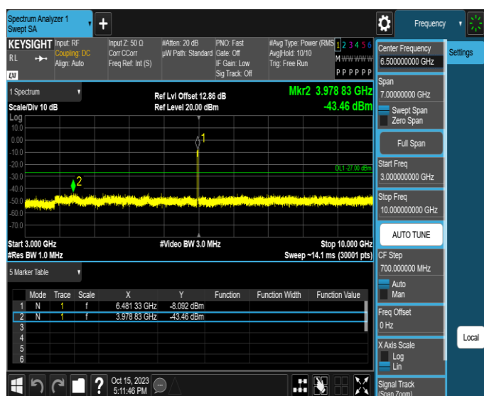
11AX20MIMO-Ant4-6475-3000~10000-PASS
