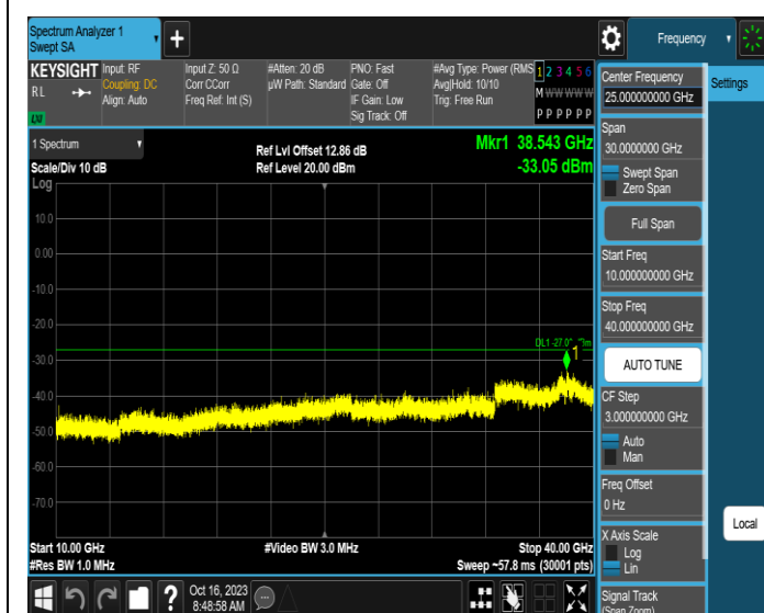
11AX20MIMO-Ant1-6535-10000~40000-PASS
