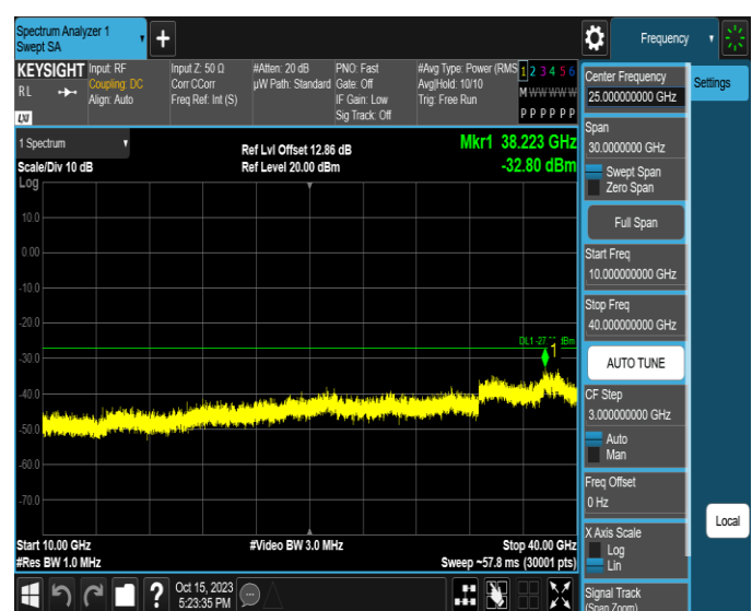
11AX20MIMO-Ant2-6515-10000~40000-PASS
