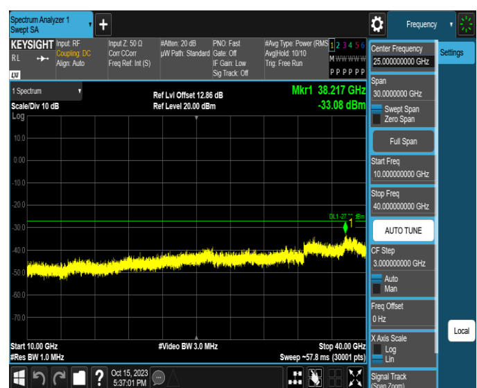
11AX20MIMO-Ant4-6515-10000~40000-PASS
