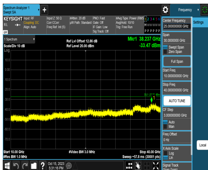
11AX20MIMO-Ant3-6515-10000~40000-PASS
