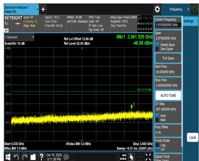
11AX20MIMO-Ant4-6475-30~3000-PASS
