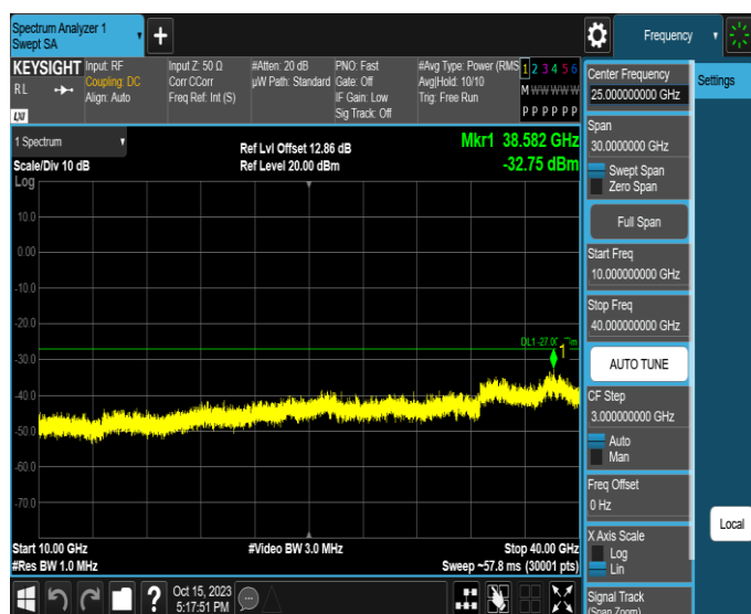
11AX20MIMO-Ant1-6515-10000~40000-PASS
