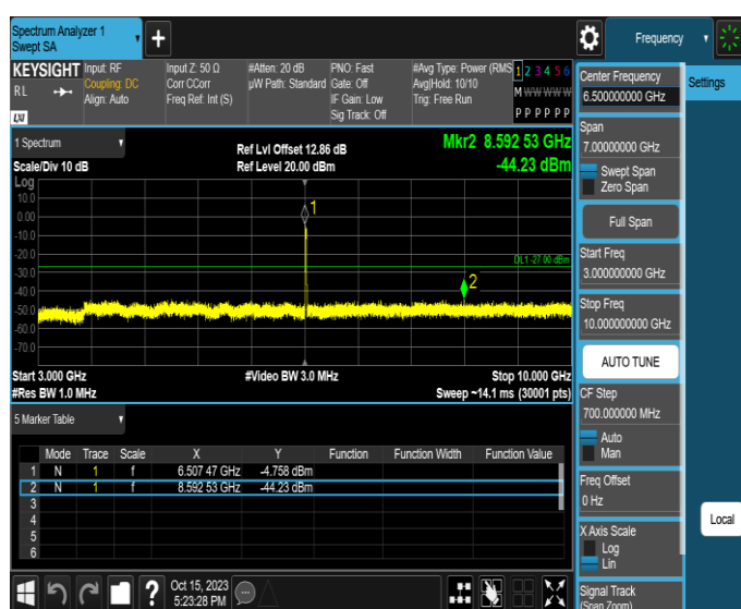
11AX20MIMO-Ant2-6515-3000~10000-PASS
