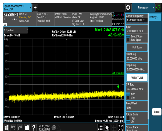
11AX20MIMO-Ant2-6515-30~3000-PASS
