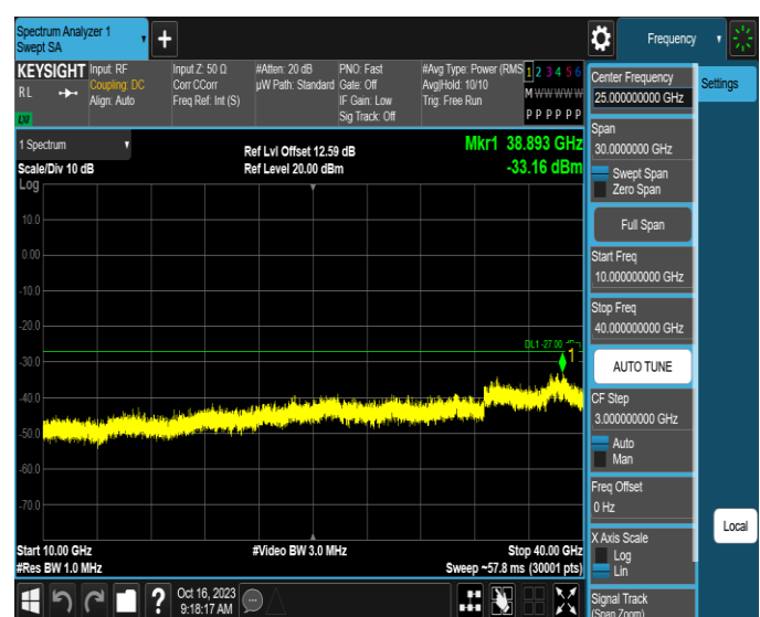
11AX20MIMO-Ant2-6695-10000~40000-PASS
