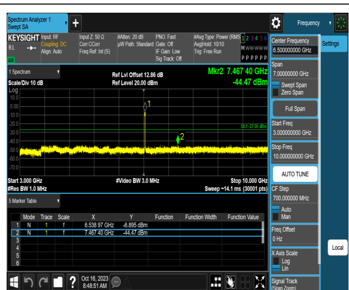
11AX20MIMO-Ant1-6535-3000~10000-PASS
