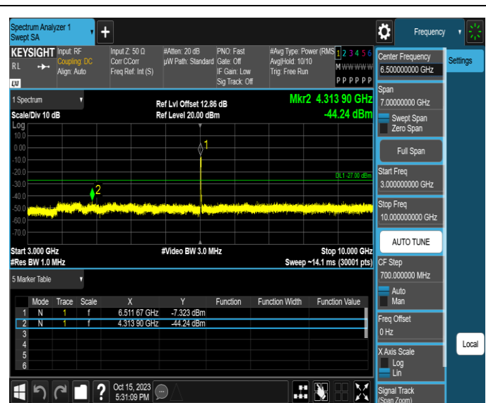
11AX20MIMO-Ant3-6515-3000~10000-PASS
