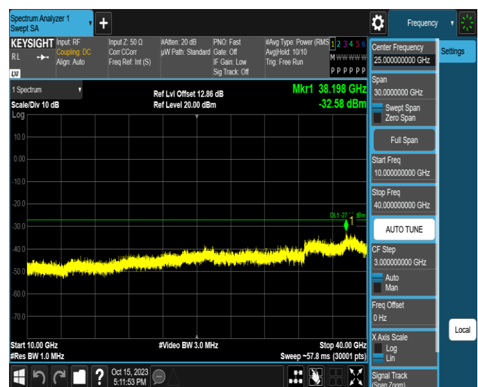
11AX20MIMO-Ant4-6475-10000~40000-PASS
