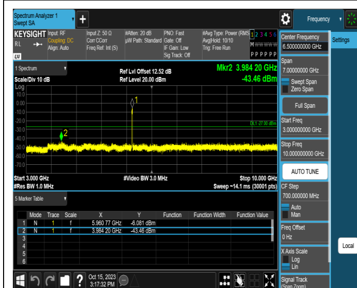
11AX20MIMO-Ant4-5955-3000~10000-PASS
