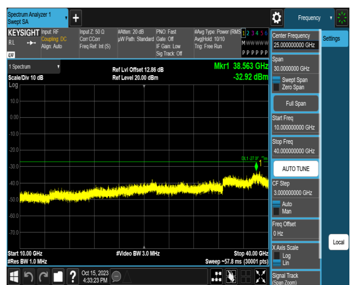
11AX20MIMO-Ant2-6435-10000~40000-PASS
