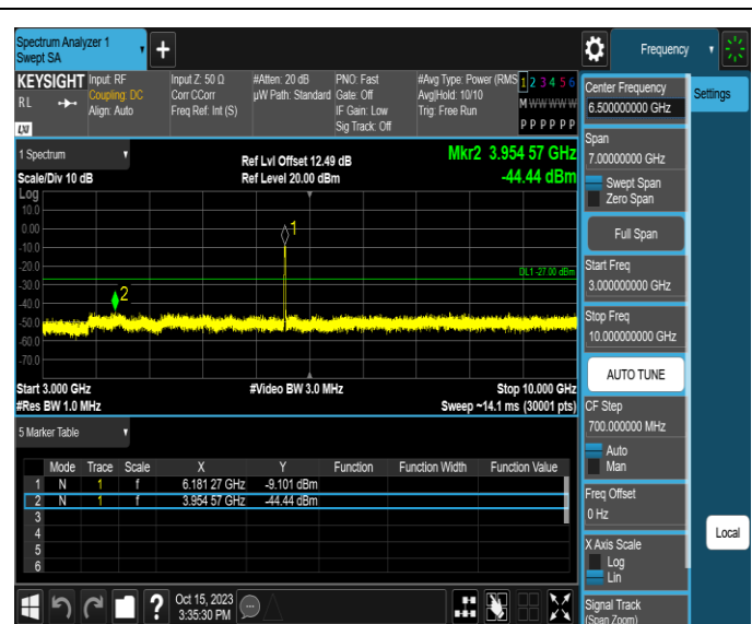
11AX20MIMO-Ant3-6175-3000~10000-PASS
