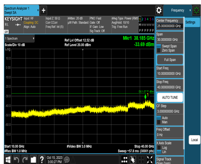
11AX20MIMO-Ant2-5955-10000~40000-PASS
