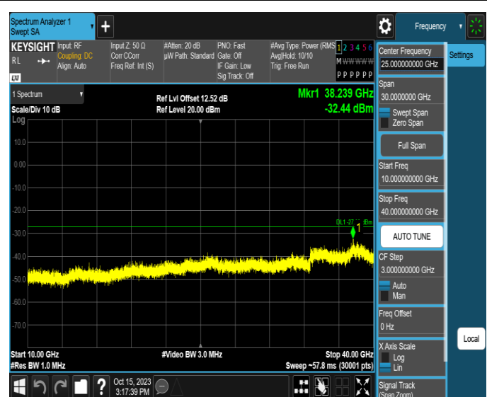
11AX20MIMO-Ant4-5955-10000~40000-PASS
