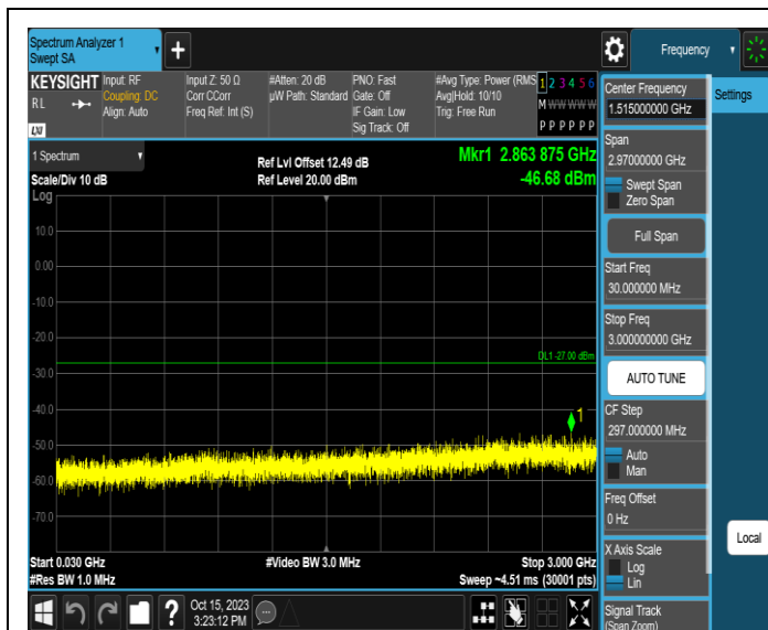
11AX20MIMO-Ant1-6175-30~3000-PASS
