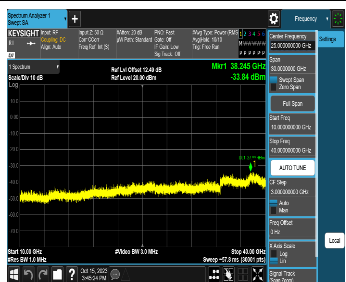
11AX20MIMO-Ant4-6175-10000~40000-PASS
