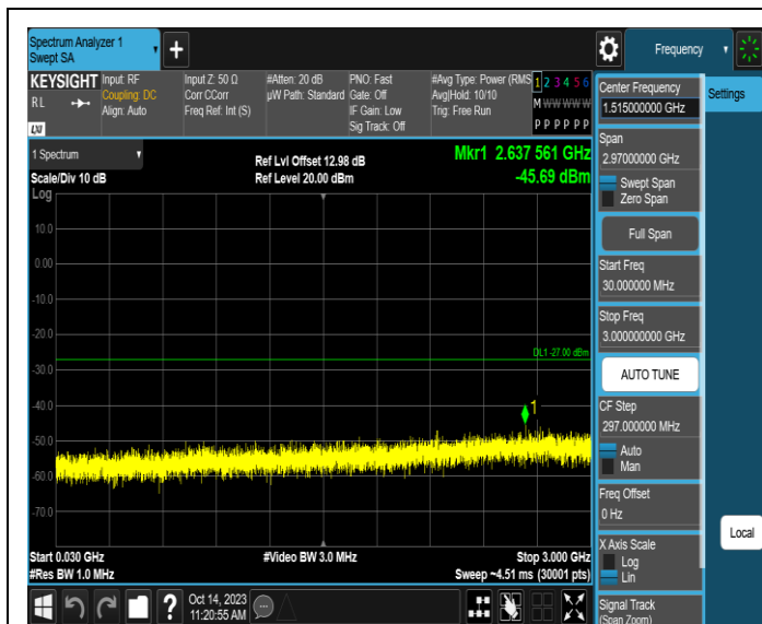
11AX20SISO-Ant3-7115-30~3000-PASS
