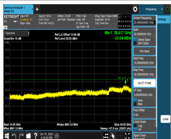
11AX20MIMO-Ant4-6415-10000~40000-PASS
