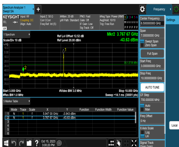
11AX20MIMO-Ant2-5955-3000~10000-PASS
