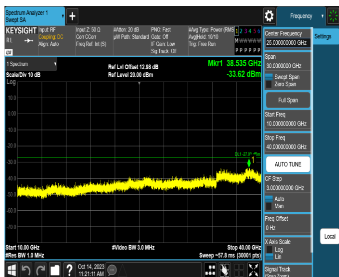
11AX20SISO-Ant3-7115-10000~40000-PASS
