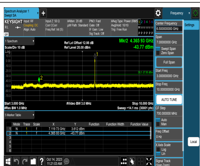
11AX20SISO-Ant3-7115-3000~10000-PASS
