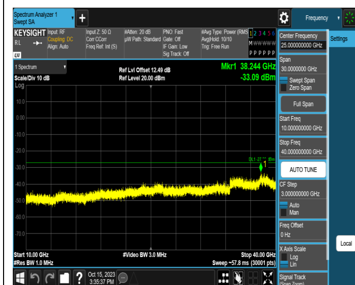
11AX20MIMO-Ant3-6175-10000~40000-PASS
