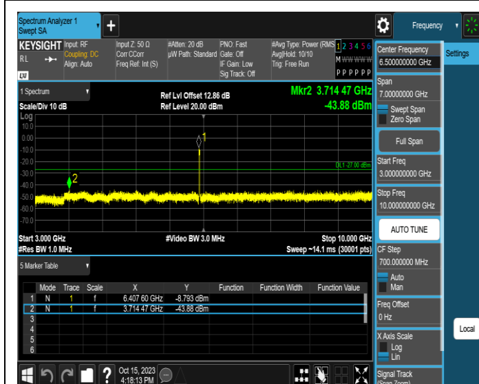
11AX20MIMO-Ant4-6415-3000~10000-PASS
