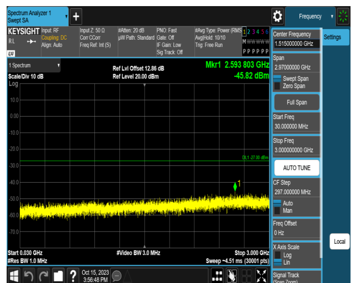
11AX20MIMO-Ant2-6415-30~3000-PASS
