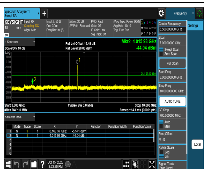
11AX20MIMO-Ant1-6175-3000~10000-PASS
