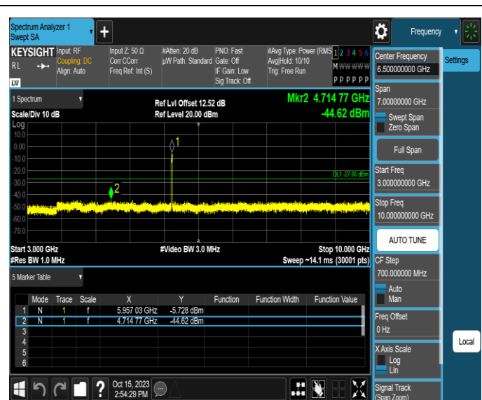
11AX20MIMO-Ant1-5955-3000~10000-PASS
