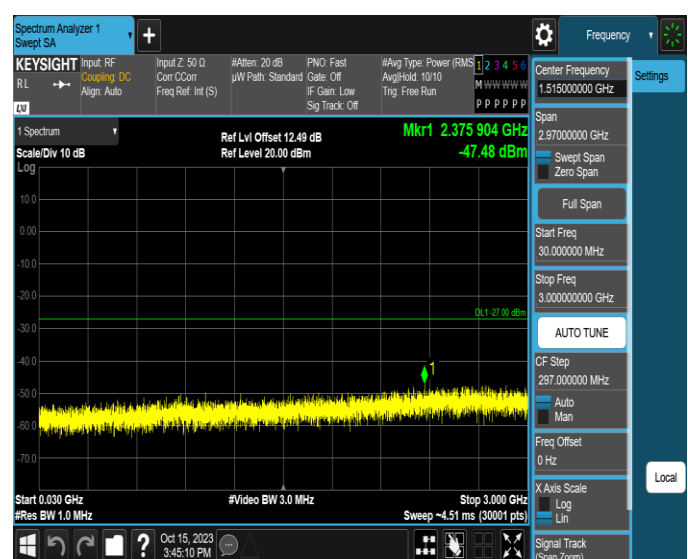
11AX20MIMO-Ant4-6175-30~3000-PASS
