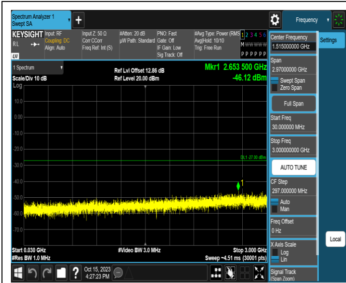
11AX20MIMO-Ant1-6435-30~3000-PASS
