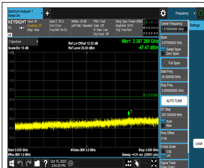
11AX20MIMO-Ant1-5955-30~3000-PASS
