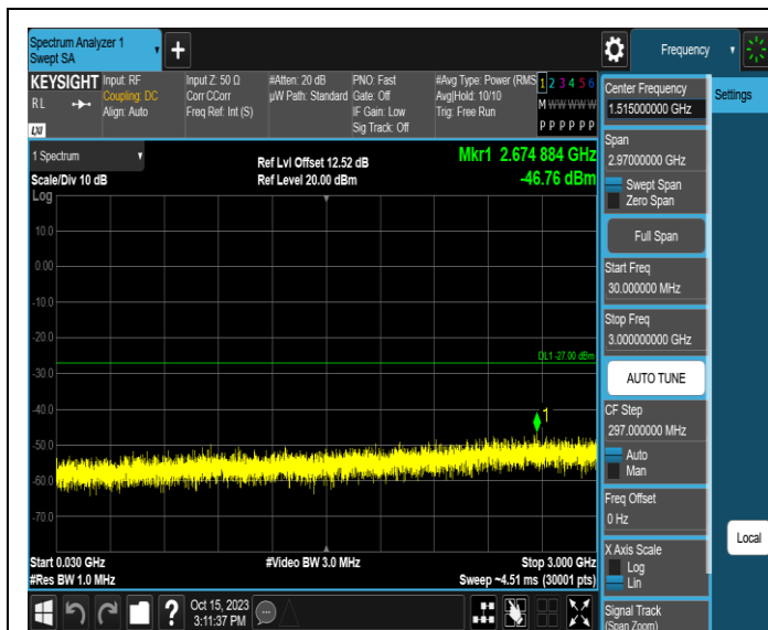
11AX20MIMO-Ant3-5955-30~3000-PASS
