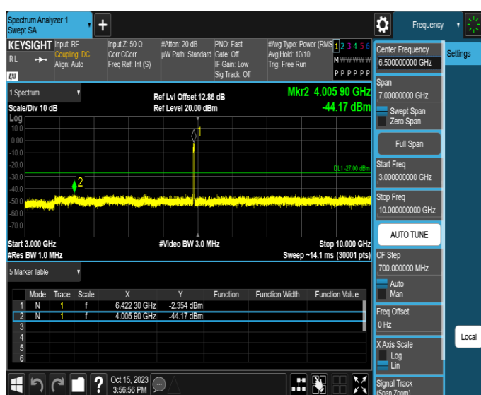
11AX20MIMO-Ant2-6415-3000~10000-PASS
