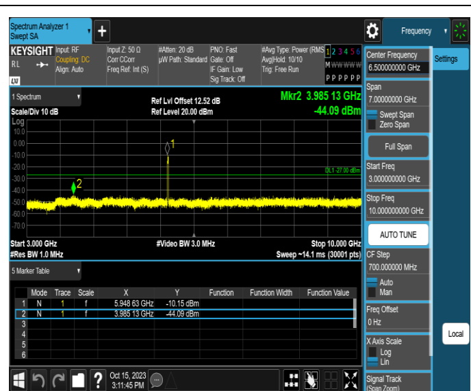
11AX20MIMO-Ant3-5955-3000~10000-PASS
