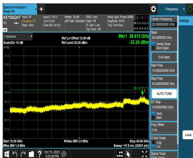
11AX20MIMO-Ant1-6175-10000~40000-PASS
