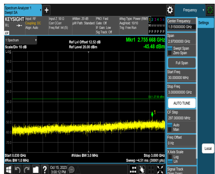
11AX20MIMO-Ant2-5955-30~3000-PASS
