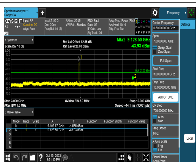
11AX20MIMO-Ant1-6415-3000~10000-PASS
