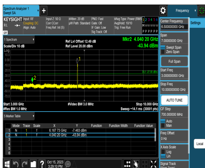
11AX20MIMO-Ant2-6175-3000~10000-PASS
