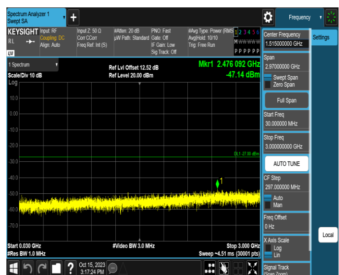
11AX20MIMO-Ant4-5955-30~3000-PASS
