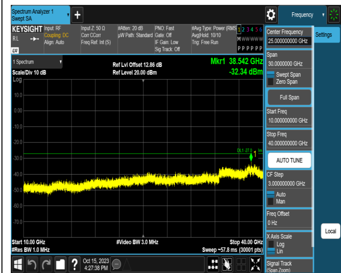
11AX20MIMO-Ant1-6435-10000~40000-PASS
