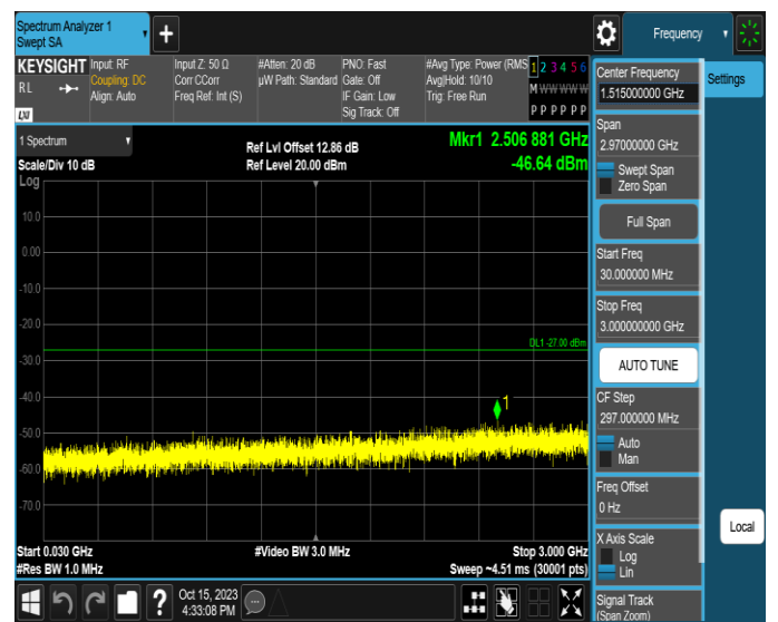
11AX20MIMO-Ant2-6435-30~3000-PASS
