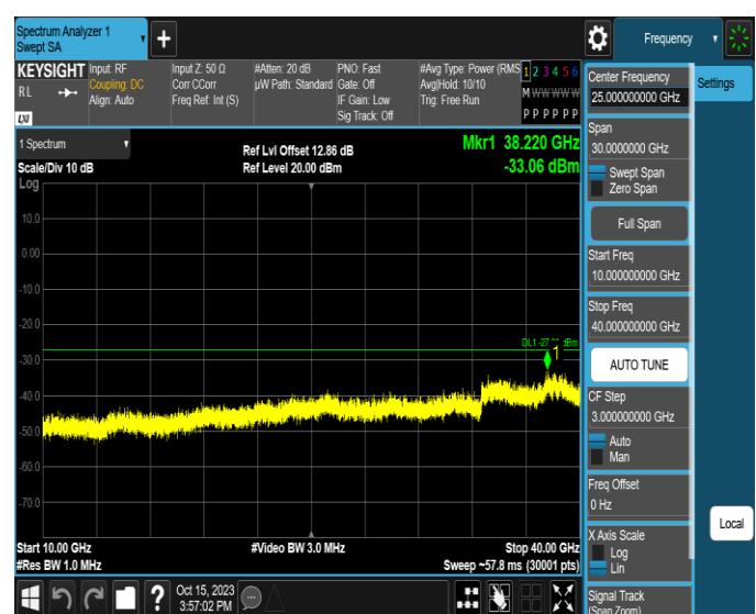
11AX20MIMO-Ant2-6415-10000~40000-PASS
