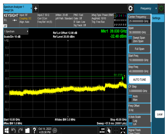
11AX20SISO-Ant4-7115-10000~40000-PASS
