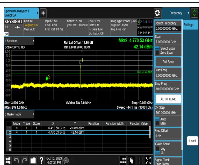
11AX20MIMO-Ant3-6415-3000~10000-PASS
