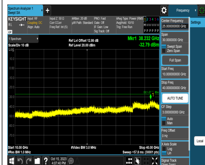
11AX20MIMO-Ant3-6415-10000~40000-PASS
