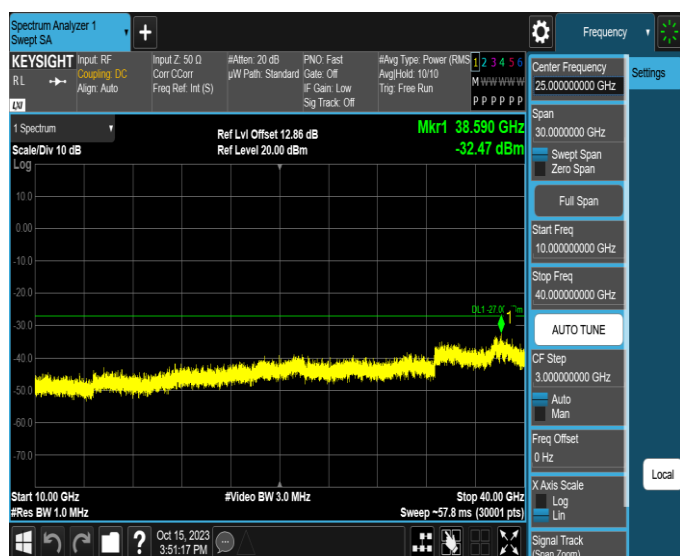
11AX20MIMO-Ant1-6415-10000~40000-PASS
