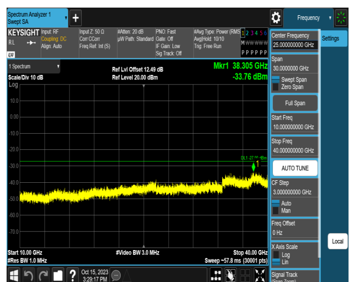
11AX20MIMO-Ant2-6175-10000~40000-PASS
