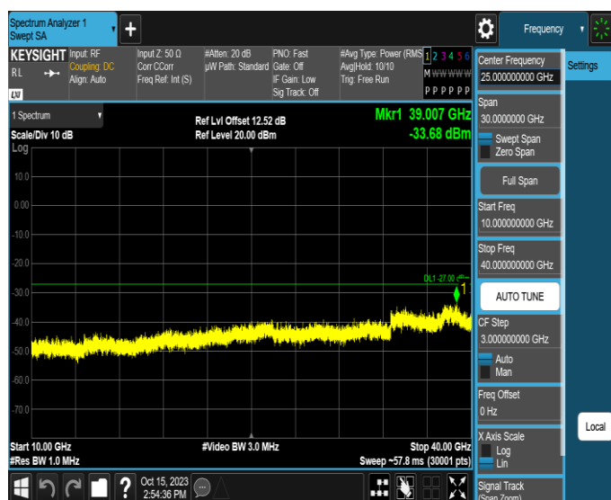
11AX20MIMO-Ant1-5955-10000~40000-PASS
