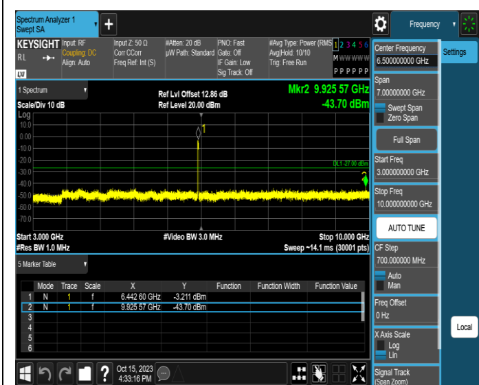
11AX20MIMO-Ant2-6435-3000~10000-PASS
