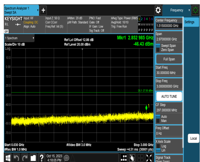
11AX20MIMO-Ant4-6415-30~3000-PASS
