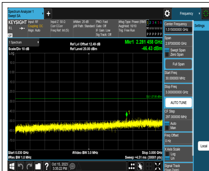
11AX20MIMO-Ant3-6175-30~3000-PASS
