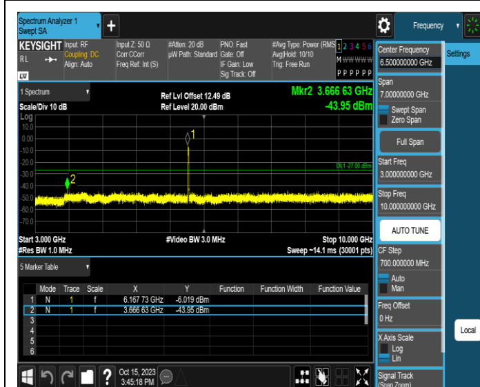
11AX20MIMO-Ant4-6175-3000~10000-PASS
