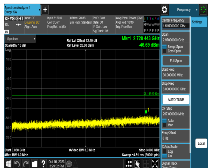
11AX20MIMO-Ant2-6175-30~3000-PASS
