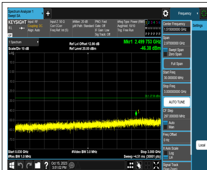
11AX20MIMO-Ant1-6415-30~3000-PASS
