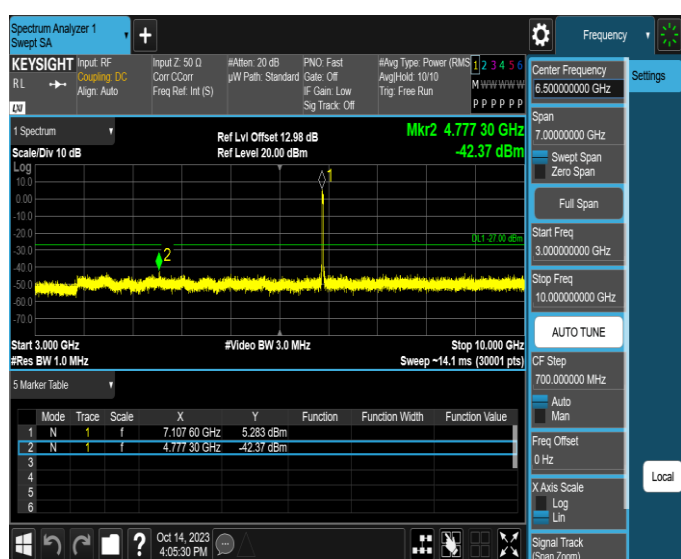
11AX20SISO-Ant4-7115-3000~10000-PASS
