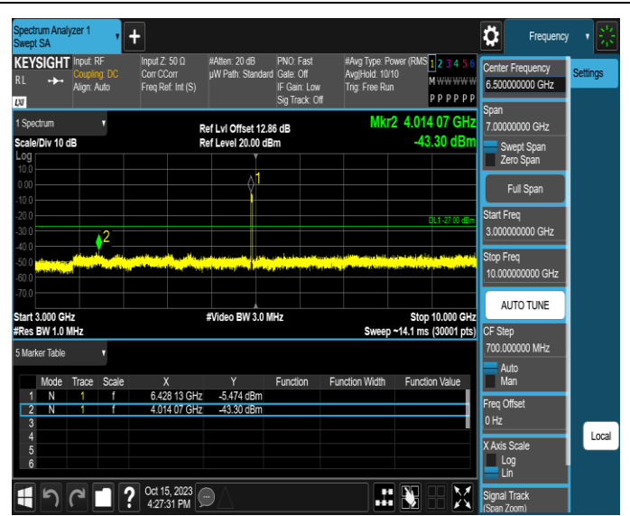
11AX20MIMO-Ant1-6435-3000~10000-PASS
