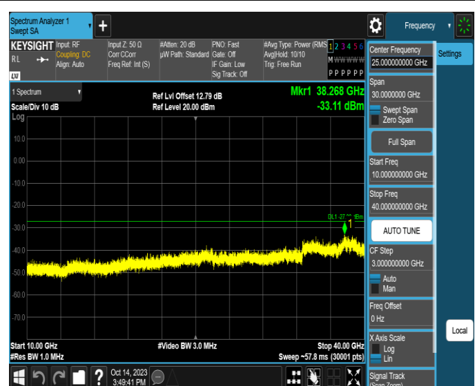
11AX20SISO-Ant4-6895-10000~40000-PASS
