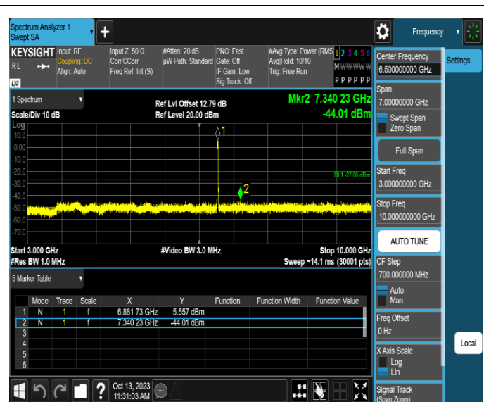
11AX20SISO-Ant1-6875-3000~10000-PASS
