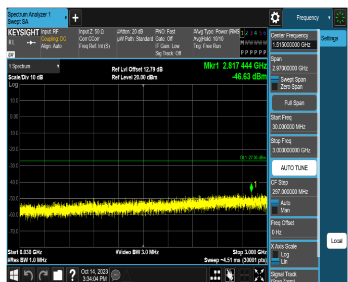
11AX20SISO-Ant4-6855-30~3000-PASS
