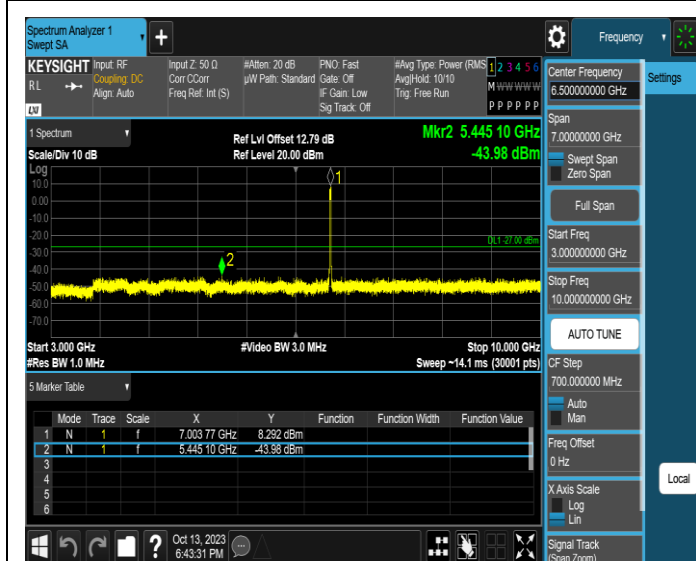
11AX20SISO-Ant2-6995-3000~10000-PASS
