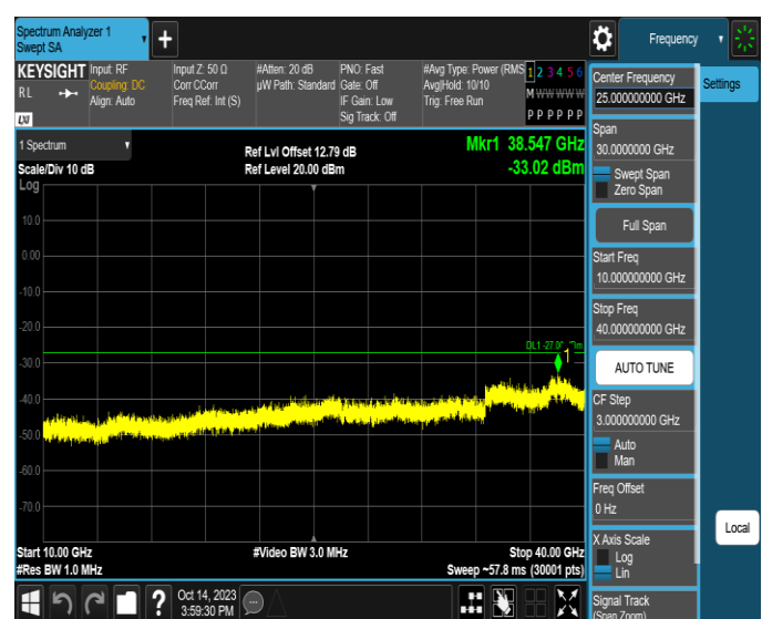
11AX20SISO-Ant4-6995-10000~40000-PASS
