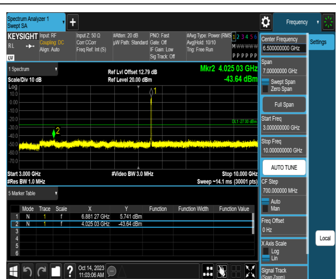
11AX20SISO-Ant3-6875-3000~10000-PASS
