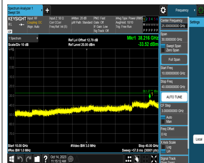
11AX20SISO-Ant3-6995-10000~40000-PASS
