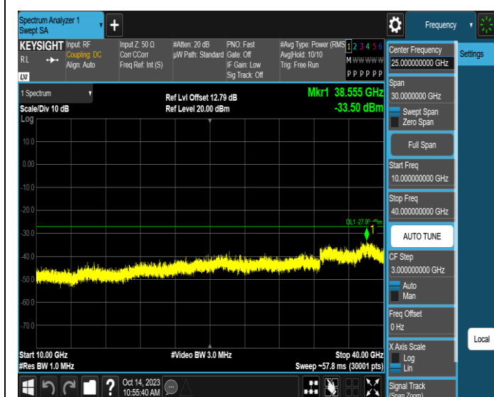
11AX20SISO-Ant3-6855-10000~40000-PASS
