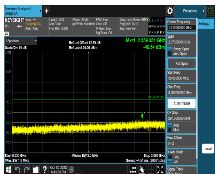
11AX20SISO-Ant2-6995-30~3000-PASS
