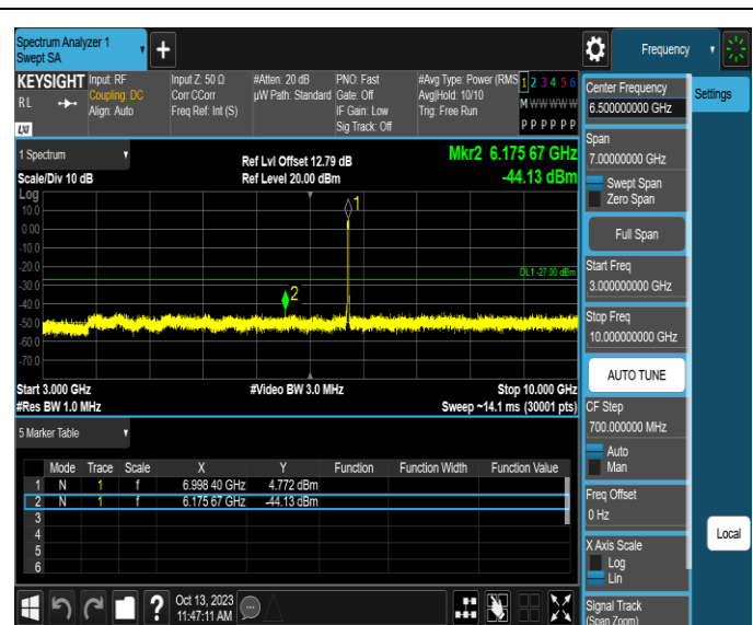
11AX20SISO-Ant1-6995-3000~10000-PASS
