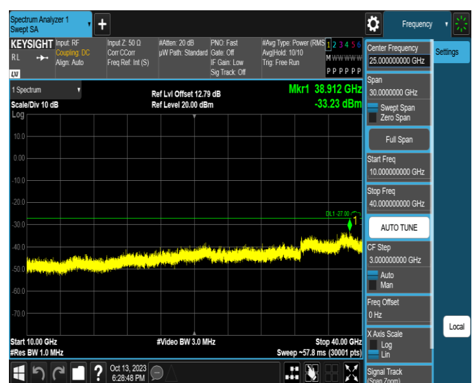
11AX20SISO-Ant2-6875-10000~40000-PASS
