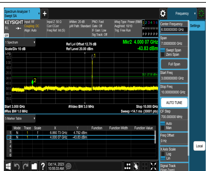
11AX20SISO-Ant3-6855-3000~10000-PASS
