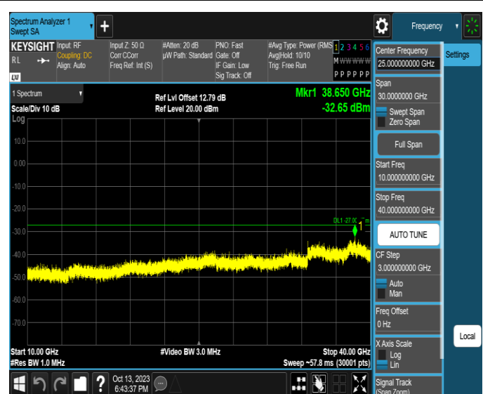
11AX20SISO-Ant2-6995-10000~40000-PASS
