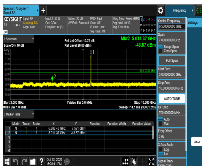
11AX20SISO-Ant2-6875-3000~10000-PASS
