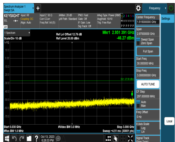
11AX20SISO-Ant2-6875-30~3000-PASS
