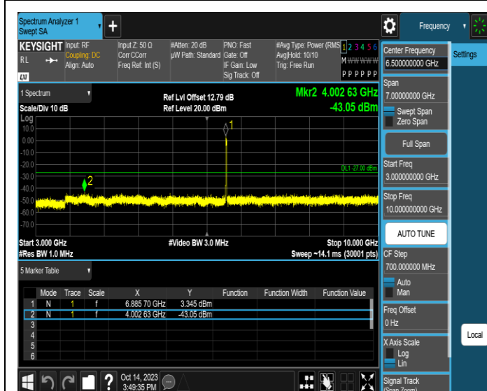
11AX20SISO-Ant4-6895-3000~10000-PASS
