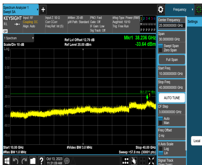
11AX20SISO-Ant1-6875-10000~40000-PASS
