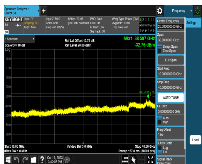
11AX20SISO-Ant4-6875-10000~40000-PASS
