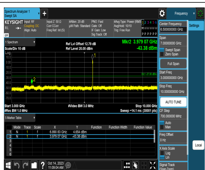
11AX20SISO-Ant3-6895-3000~10000-PASS
