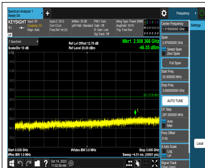
11AX20SISO-Ant3-6875-30~3000-PASS
