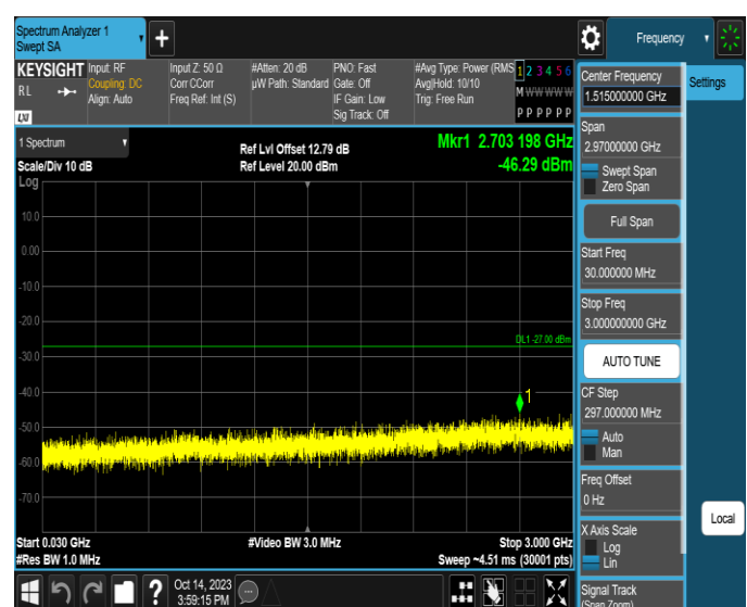
11AX20SISO-Ant4-6995-30~3000-PASS
