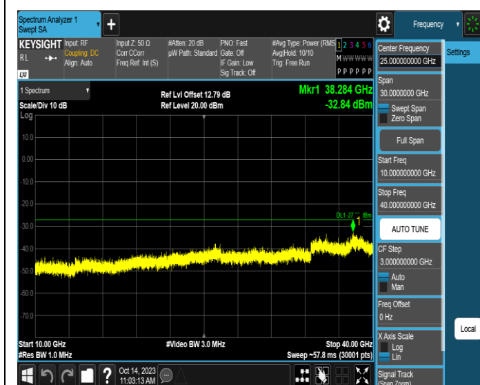
11AX20SISO-Ant3-6875-10000~40000-PASS
