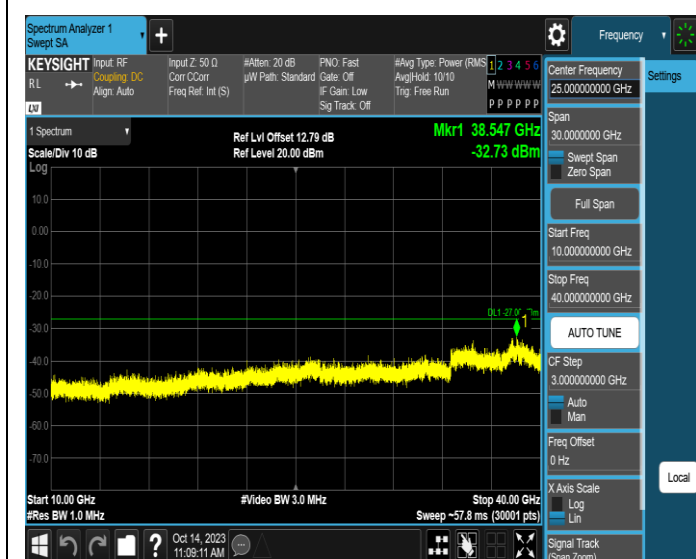
11AX20SISO-Ant3-6895-10000~40000-PASS
