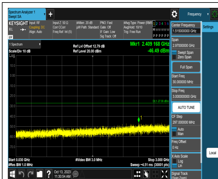
11AX20SISO-Ant1-6875-30~3000-PASS
