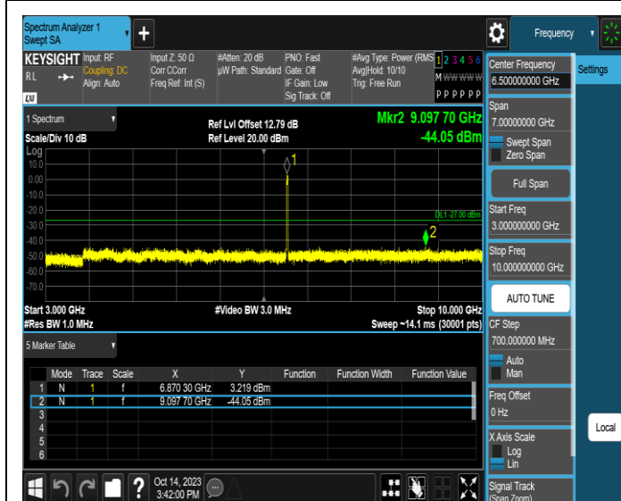
11AX20SISO-Ant4-6875-3000~10000-PASS
