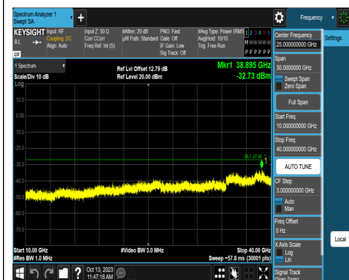
11AX20SISO-Ant1-6995-10000~40000-PASS
