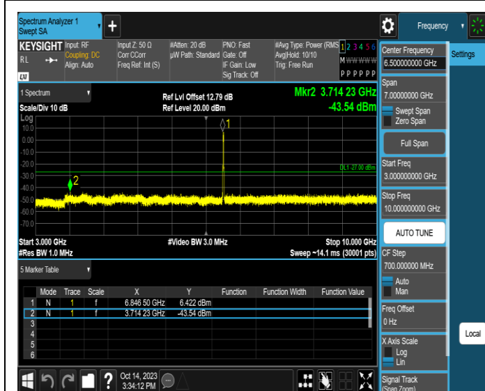
11AX20SISO-Ant4-6855-3000~10000-PASS
