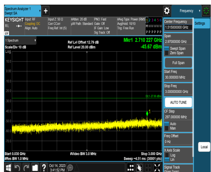
11AX20SISO-Ant4-6875-30~3000-PASS
