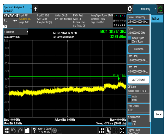
11AX20SISO-Ant4-6855-10000~40000-PASS
