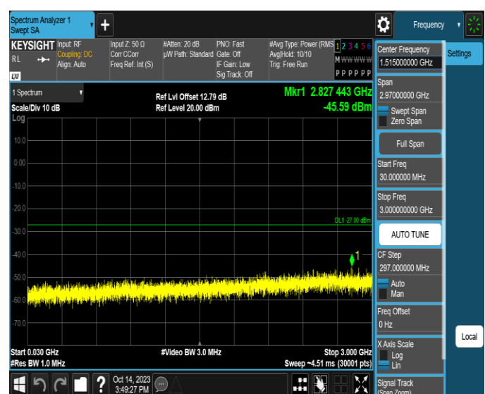
11AX20SISO-Ant4-6895-30~3000-PASS
