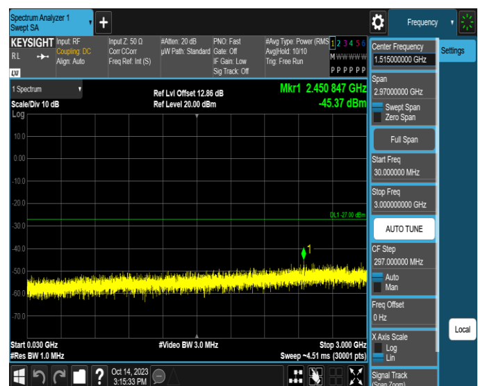
11AX20SISO-Ant4-6515-30~3000-PASS
