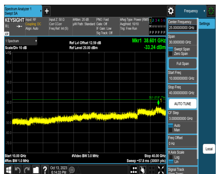
11AX20SISO-Ant2-6695-10000~40000-PASS
