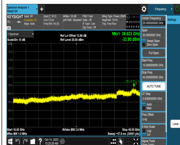
11AX20SISO-Ant3-6475-10000~40000-PASS
