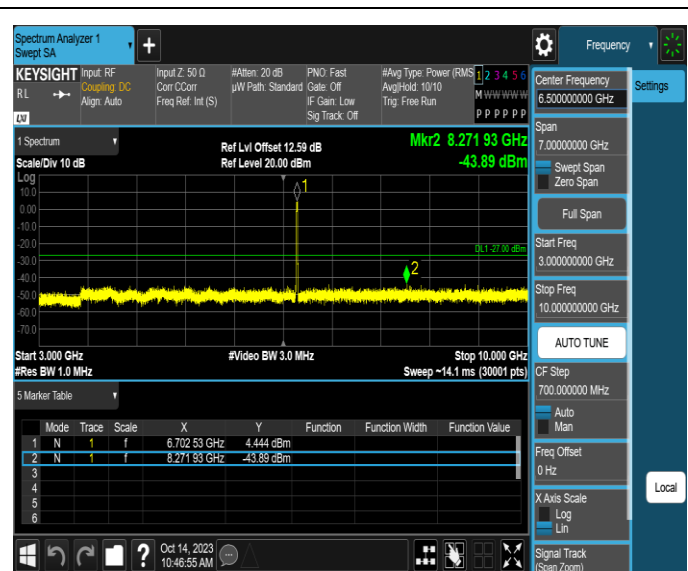
11AX20SISO-Ant3-6695-3000~10000-PASS
