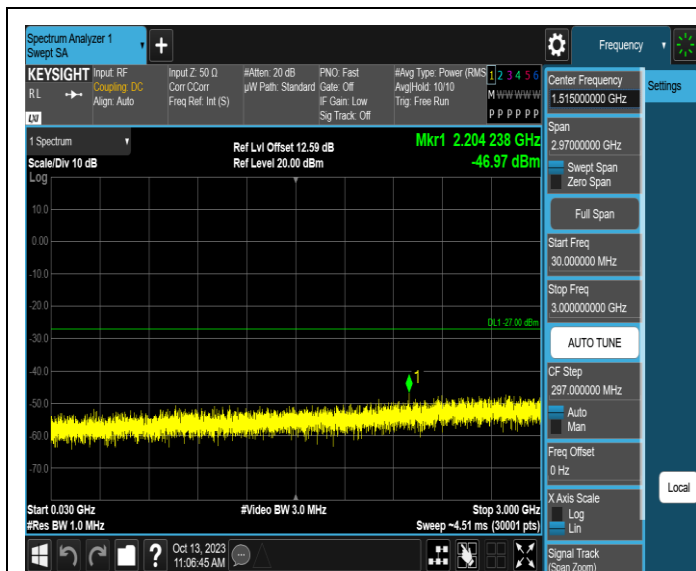
11AX20SISO-Ant1-6695-30~3000-PASS
