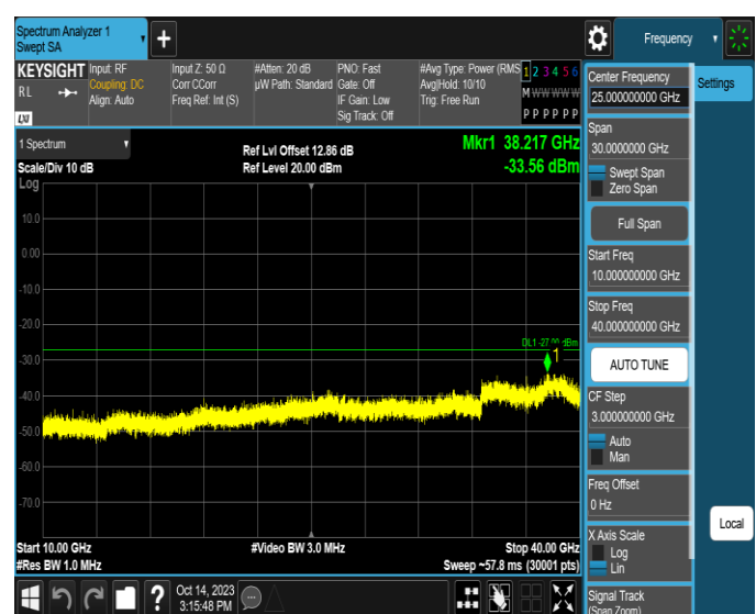
11AX20SISO-Ant4-6515-10000~40000-PASS
