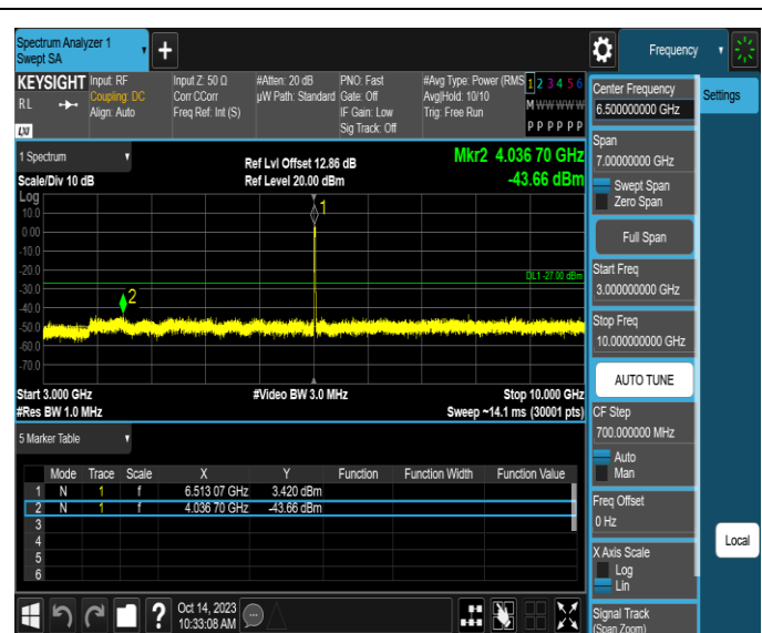
11AX20SISO-Ant3-6515-3000~10000-PASS
