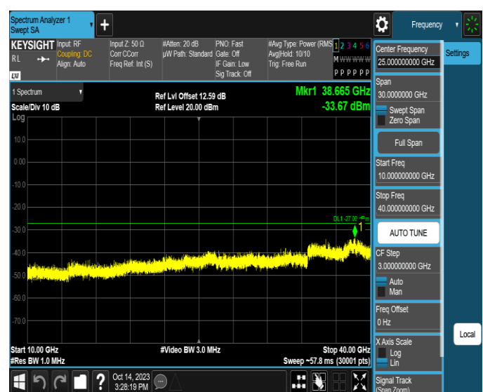
11AX20SISO-Ant4-6695-10000~40000-PASS
