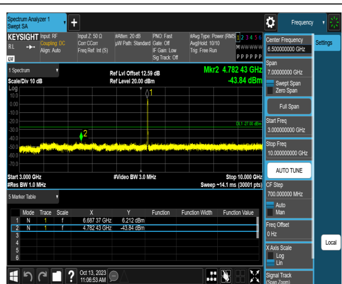
11AX20SISO-Ant1-6695-3000~10000-PASS
