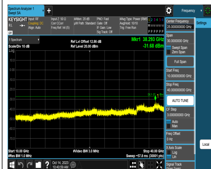
11AX20SISO-Ant3-6535-10000~40000-PASS
