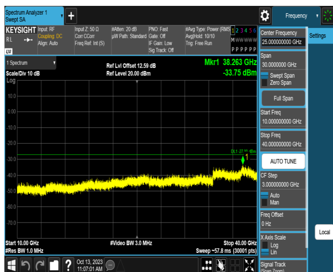
11AX20SISO-Ant1-6695-10000~40000-PASS
