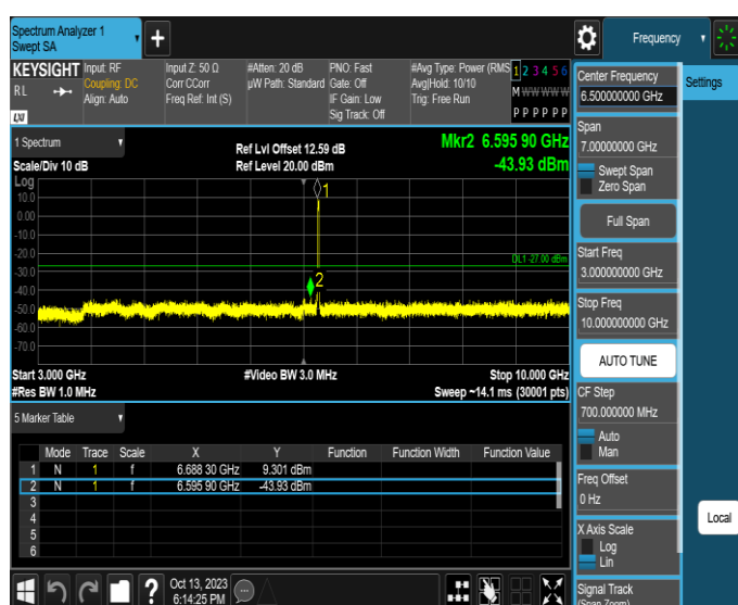
11AX20SISO-Ant2-6695-3000~10000-PASS
