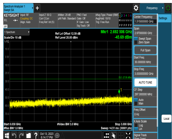
11AX20SISO-Ant2-6695-30~3000-PASS
