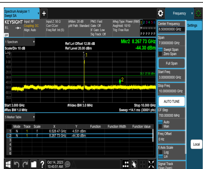
11AX20SISO-Ant3-6535-3000~10000-PASS
