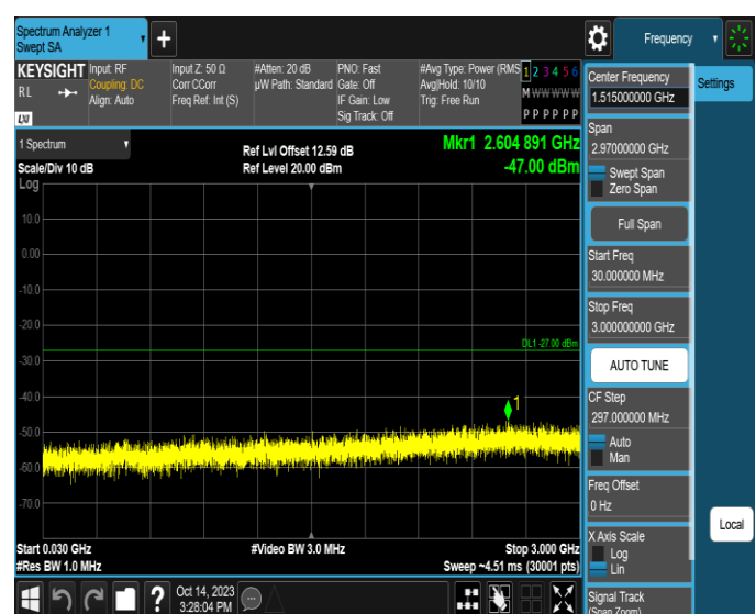
11AX20SISO-Ant4-6695-30~3000-PASS
