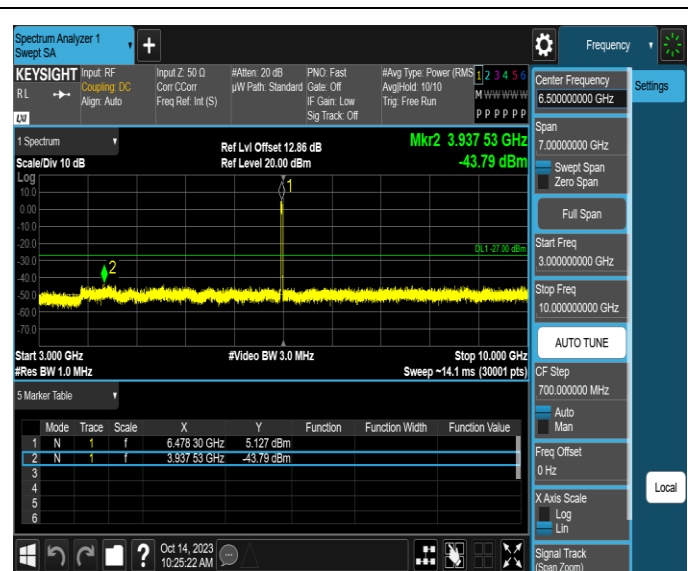
11AX20SISO-Ant3-6475-3000~10000-PASS
