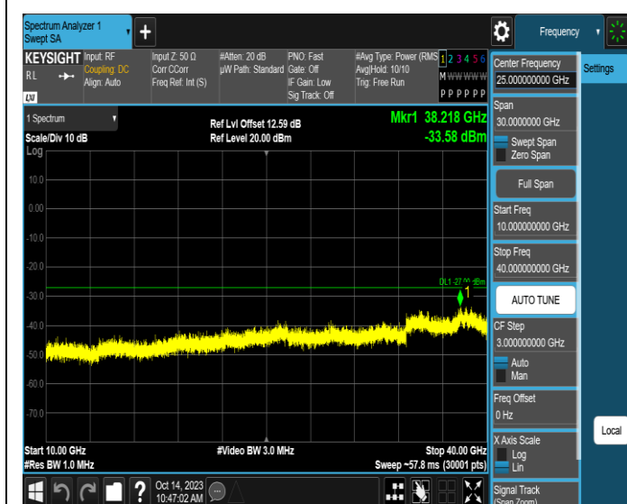
11AX20SISO-Ant3-6695-10000~40000-PASS
