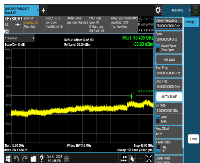
11AX20SISO-Ant4-6535-10000~40000-PASS
