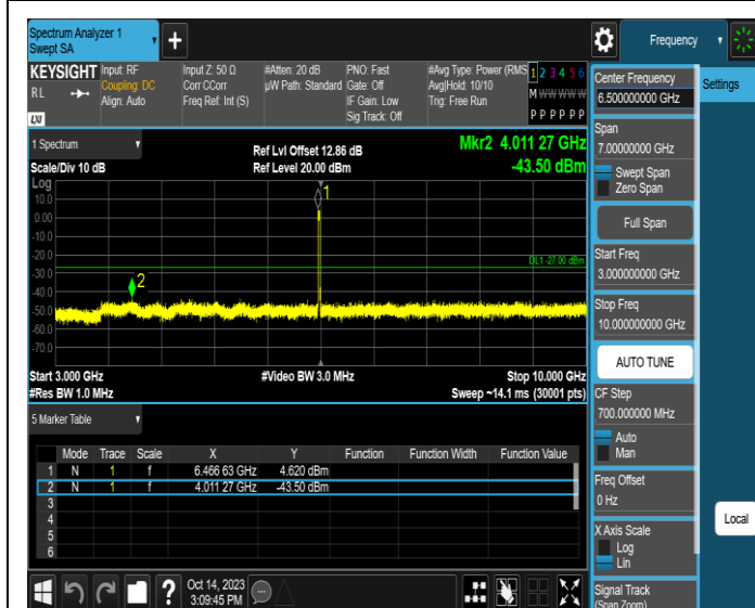
11AX20SISO-Ant4-6475-3000~10000-PASS
