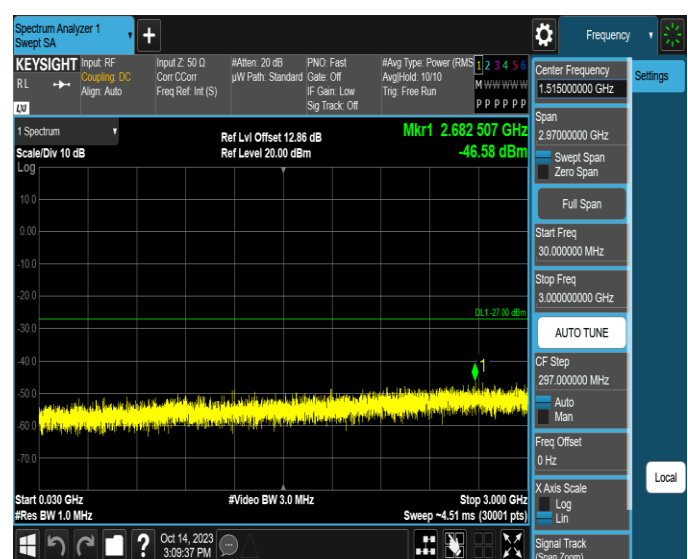
11AX20SISO-Ant4-6475-30~3000-PASS
