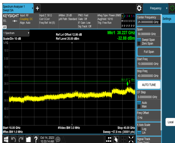
11AX20SISO-Ant3-6515-10000~40000-PASS
