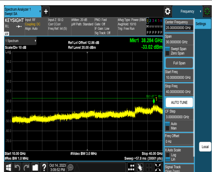
11AX20SISO-Ant4-6475-10000~40000-PASS
