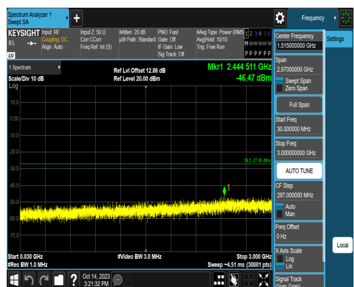
11AX20SISO-Ant4-6535-30~3000-PASS
