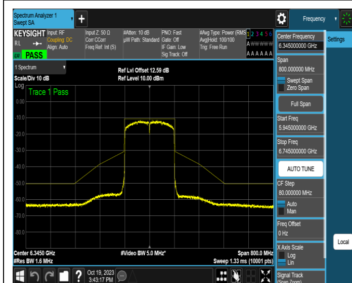
NTNV-11AX160MIMO-Ant1-6345-PASS
