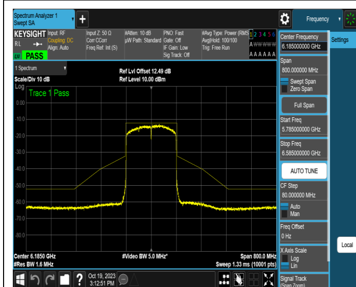
NTNV-11AX160MIMO-Ant1-6185-PASS
