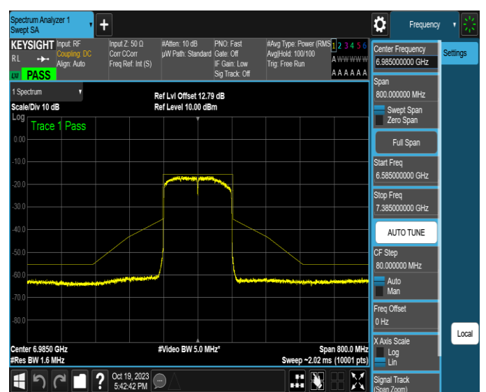
NTNV-11AX160MIMO-Ant4-6985-PASS
