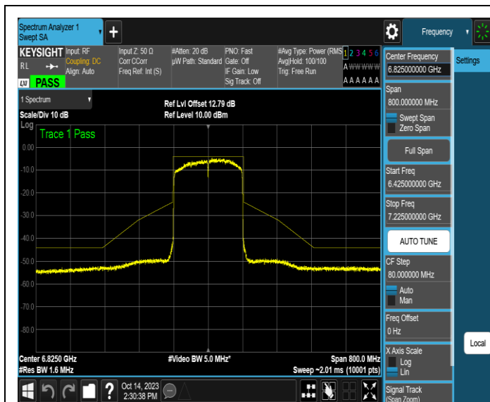
NTNV-11AX160SISO-Ant3-6825-PASS
