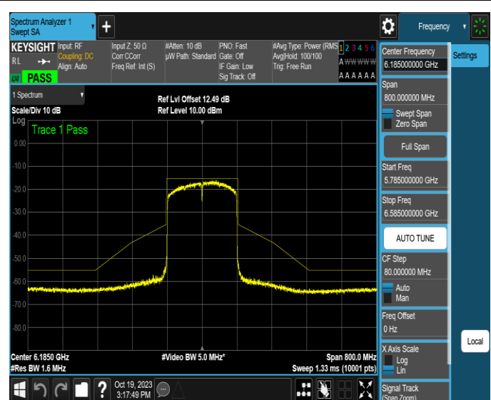
NTNV-11AX160MIMO-Ant2-6185-PASS
