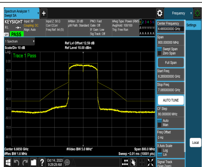
NTNV-11AX160SISO-Ant2-6665-PASS
