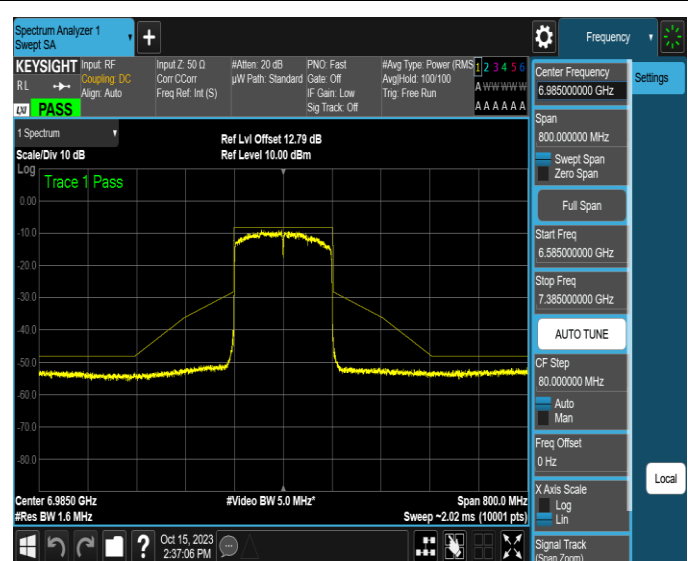
NTNV-11AX160SISO-Ant4-6985-PASS
