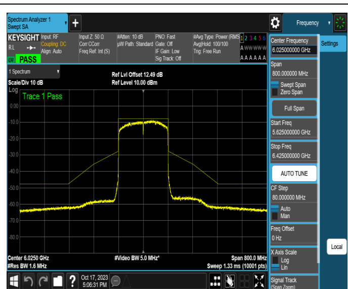
NTNV-11AX160MIMO-Ant2-6025-PASS
