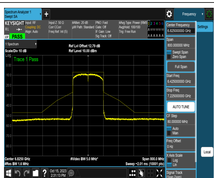
NTNV-11AX160SISO-Ant4-6825-PASS
