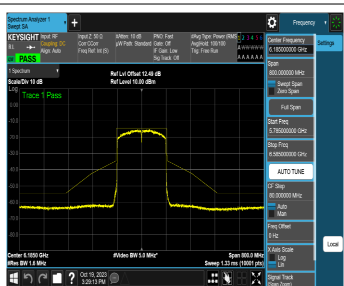
NTNV-11AX160MIMO-Ant4-6185-PASS
