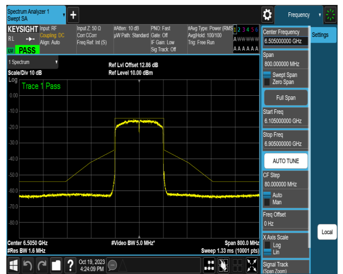
NTNV-11AX160MIMO-Ant4-6505-PASS
