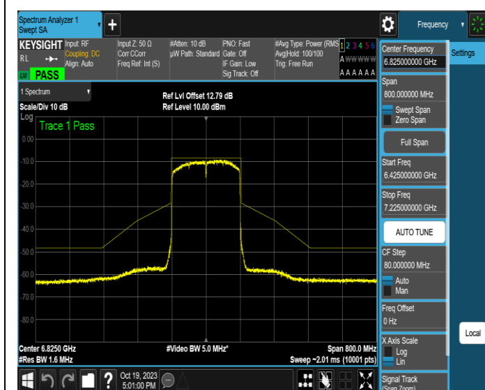
NTNV-11AX160MIMO-Ant1-6825-PASS
