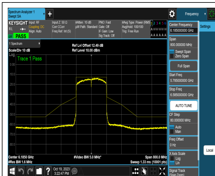
NTNV-11AX160MIMO-Ant3-6185-PASS
