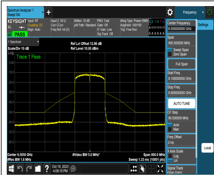
NTNV-11AX160MIMO-Ant1-6505-PASS
