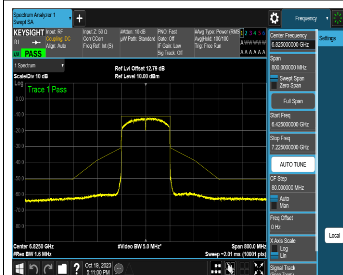
NTNV-11AX160MIMO-Ant3-6825-PASS
