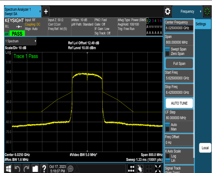
NTNV-11AX160MIMO-Ant4-6025-PASS
