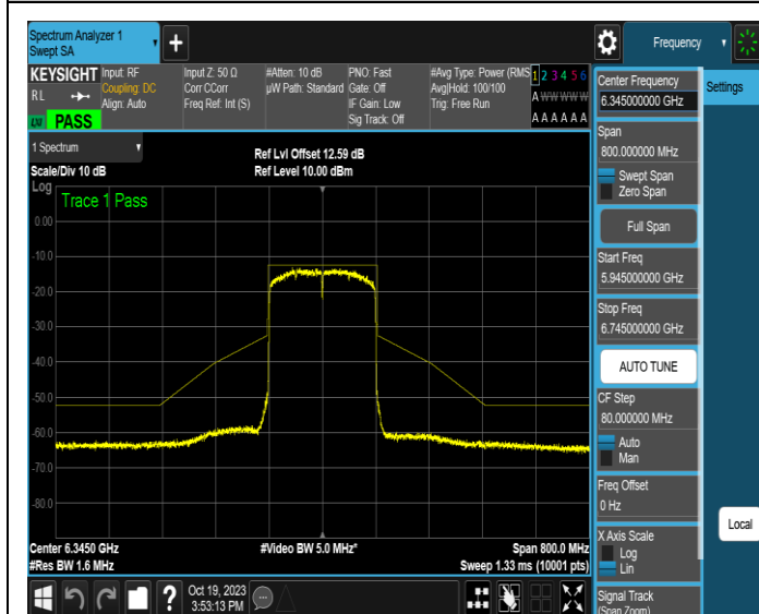
NTNV-11AX160MIMO-Ant3-6345-PASS
