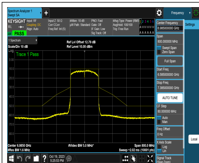
NTNV-11AX160MIMO-Ant1-6985-PASS
