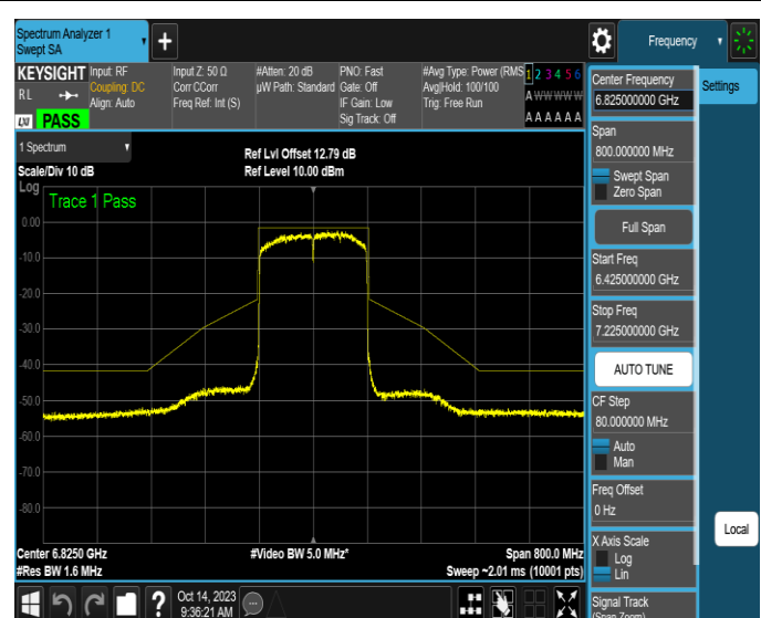
NTNV-11AX160SISO-Ant2-6825-PASS
