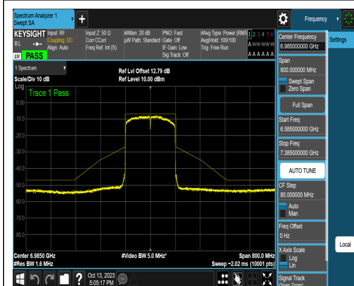
NTNV-11AX160SISO-Ant1-6985-PASS
