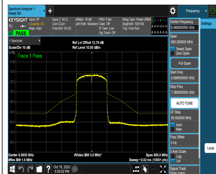
NTNV-11AX160MIMO-Ant3-6985-PASS
