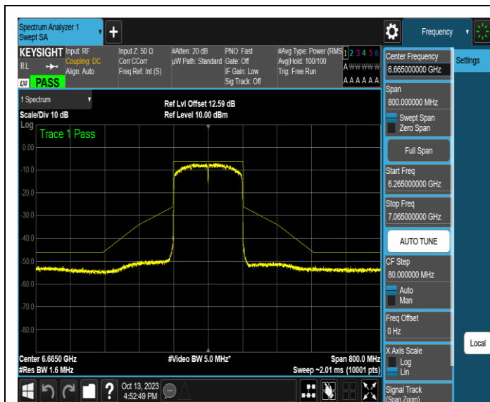
NTNV-11AX160SISO-Ant1-6665-PASS
