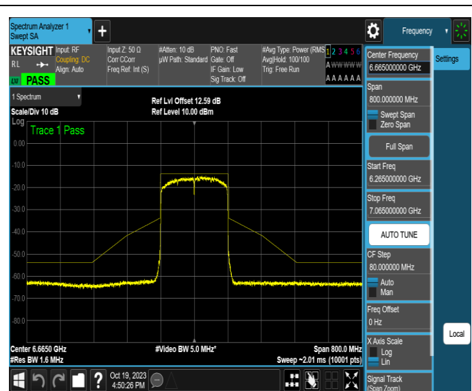
NTNV-11AX160MIMO-Ant4-6665-PASS
