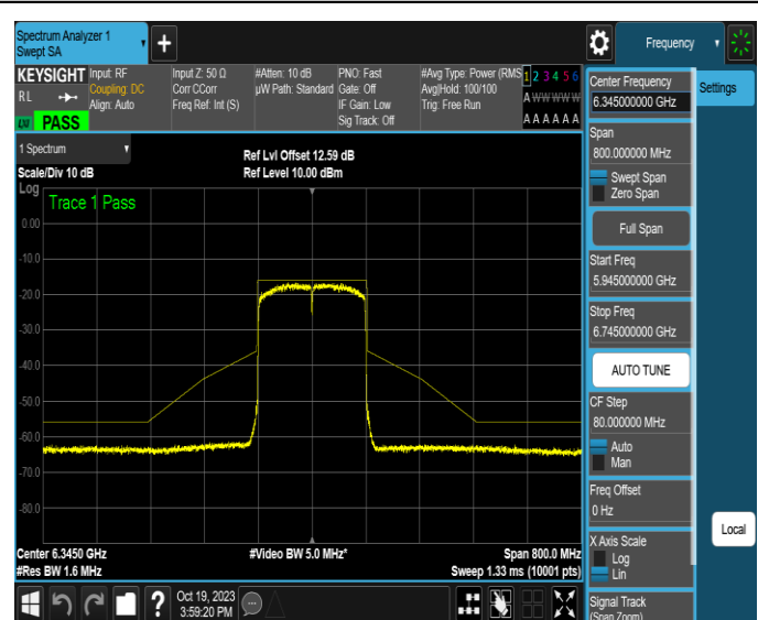
NTNV-11AX160MIMO-Ant4-6345-PASS
