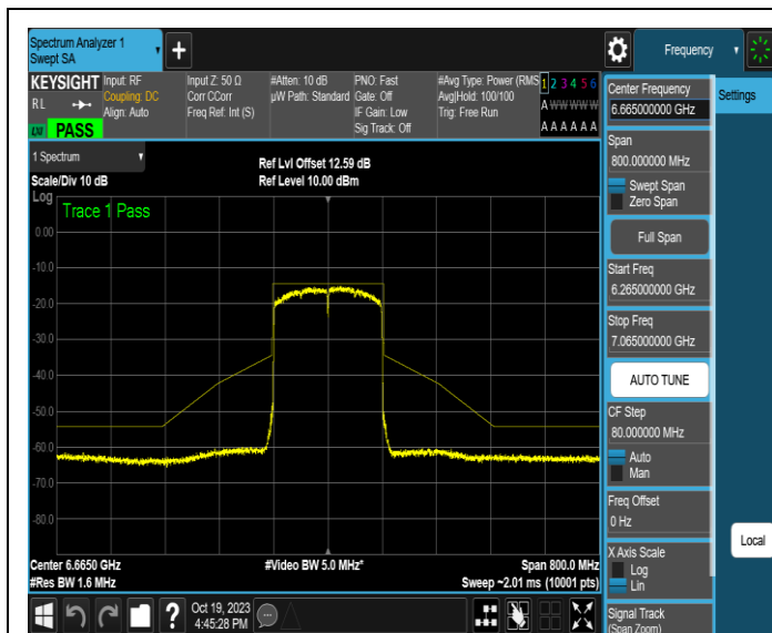
NTNV-11AX160MIMO-Ant3-6665-PASS
