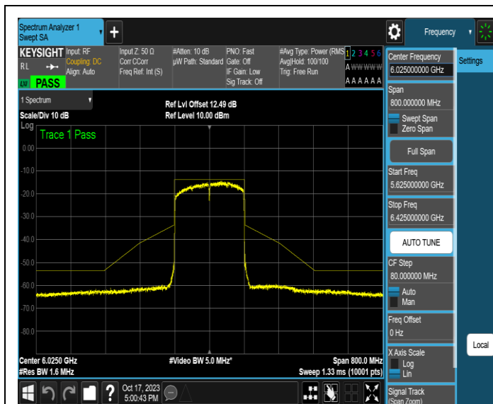
NTNV-11AX160MIMO-Ant1-6025-PASS
