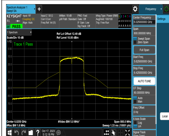
NTNV-11AX160MIMO-Ant3-6025-PASS
