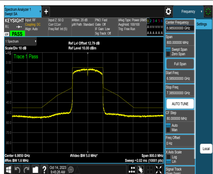
NTNV-11AX160SISO-Ant2-6985-PASS
