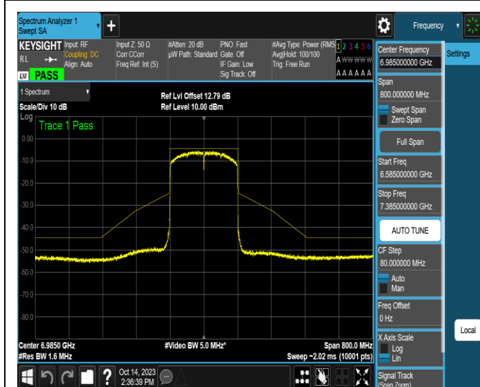
NTNV-11AX160SISO-Ant3-6985-PASS
