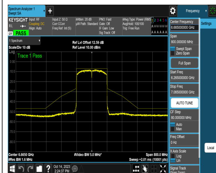
NTNV-11AX160SISO-Ant3-6665-PASS
