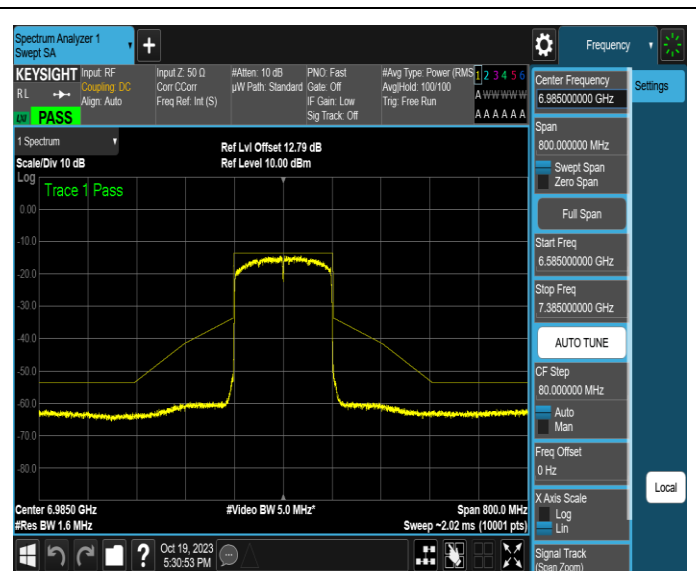
NTNV-11AX160MIMO-Ant2-6985-PASS
