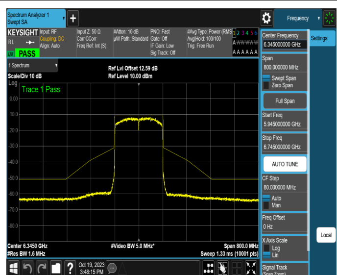
NTNV-11AX160MIMO-Ant2-6345-PASS
