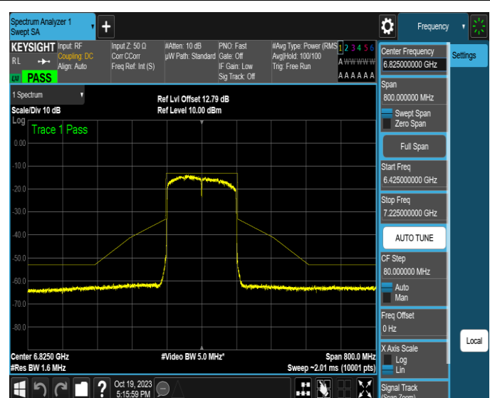
NTNV-11AX160MIMO-Ant4-6825-PASS
