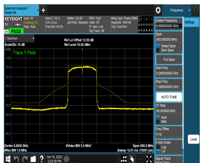
NTNV-11AX160SISO-Ant4-6665-PASS
