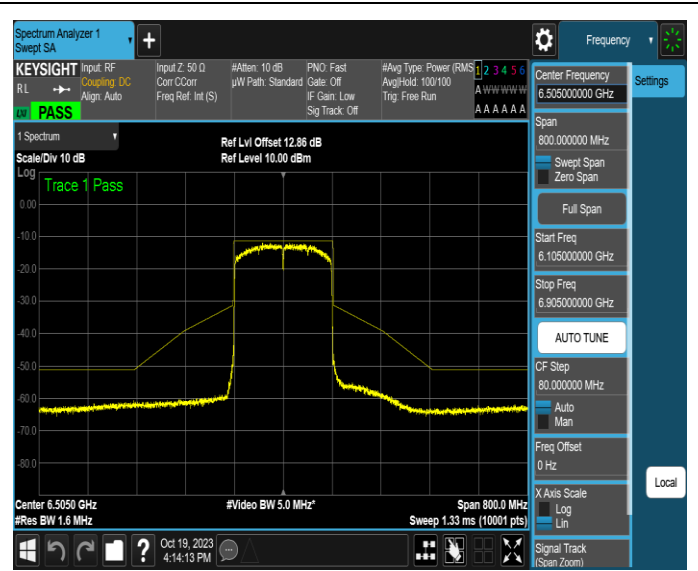
NTNV-11AX160MIMO-Ant2-6505-PASS
