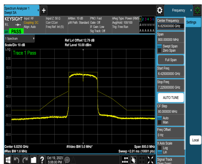
NTNV-11AX160MIMO-Ant2-6825-PASS
