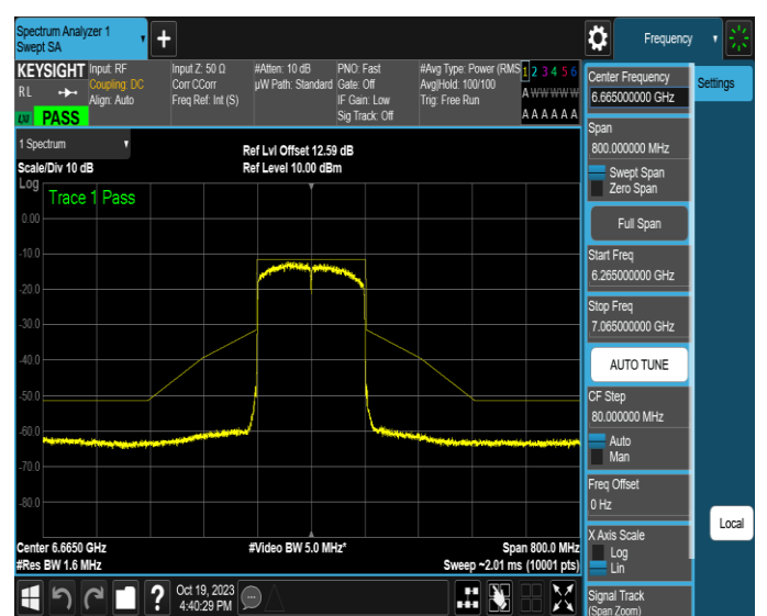
NTNV-11AX160MIMO-Ant2-6665-PASS
