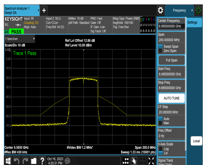
NTNV-11AX40MIMO-Ant4-6565-PASS
