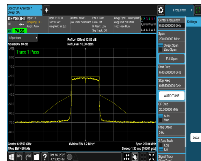
NTNV-11AX40MIMO-Ant3-6565-PASS
