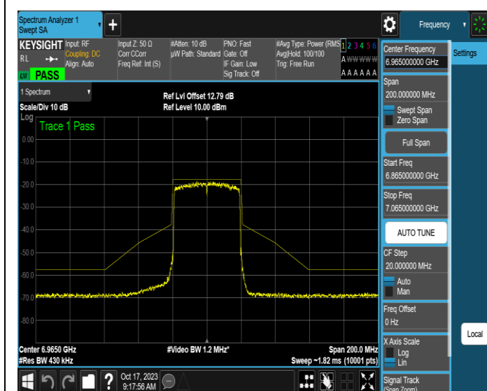
NTNV-11AX40MIMO-Ant1-6965-PASS
