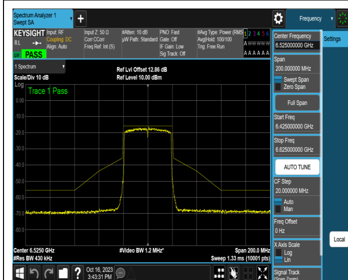
NTNV-11AX40MIMO-Ant1-6525-PASS
