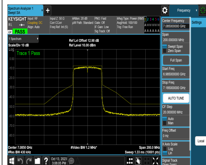
NTNV-11AX40SISO-Ant1-7085-PASS
