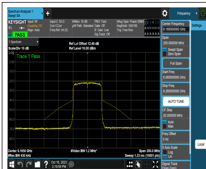
NTNV-11AX40MIMO-Ant3-6165-PASS
