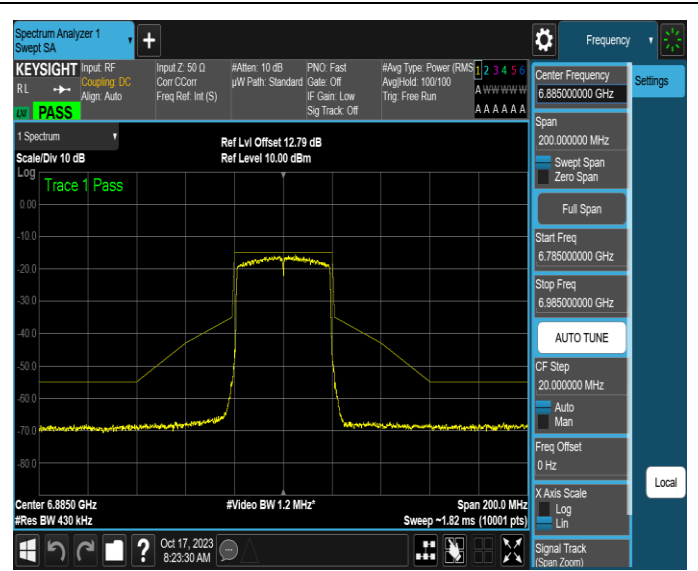
NTNV-11AX40MIMO-Ant2-6885-PASS
