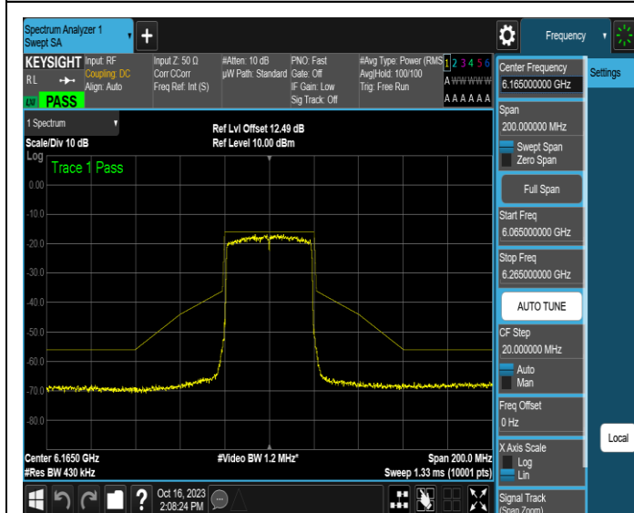
NTNV-11AX40MIMO-Ant1-6165-PASS
