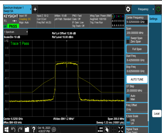
NTNV-11AX40MIMO-Ant4-6525-PASS
