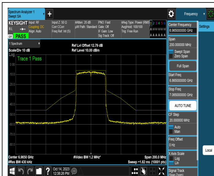
NTNV-11AX40SISO-Ant3-6965-PASS
