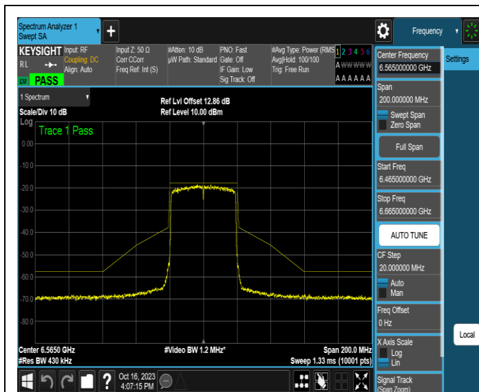
NTNV-11AX40MIMO-Ant1-6565-PASS
