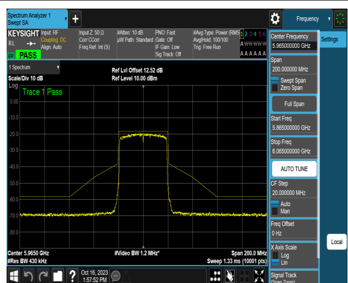
NTNV-11AX40MIMO-Ant4-5965-PASS
