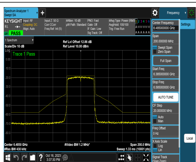
NTNV-11AX40MIMO-Ant4-6485-PASS
