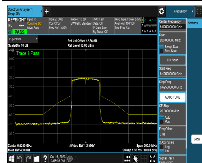
NTNV-11AX40MIMO-Ant3-6525-PASS
