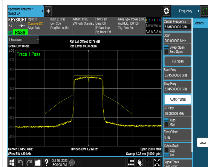
NTNV-11AX40MIMO-Ant3-6845-PASS
