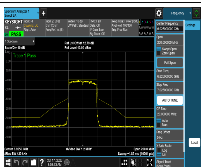
NTNV-11AX40MIMO-Ant4-6925-PASS
