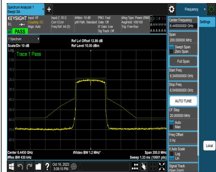
NTNV-11AX40MIMO-Ant3-6445-PASS
