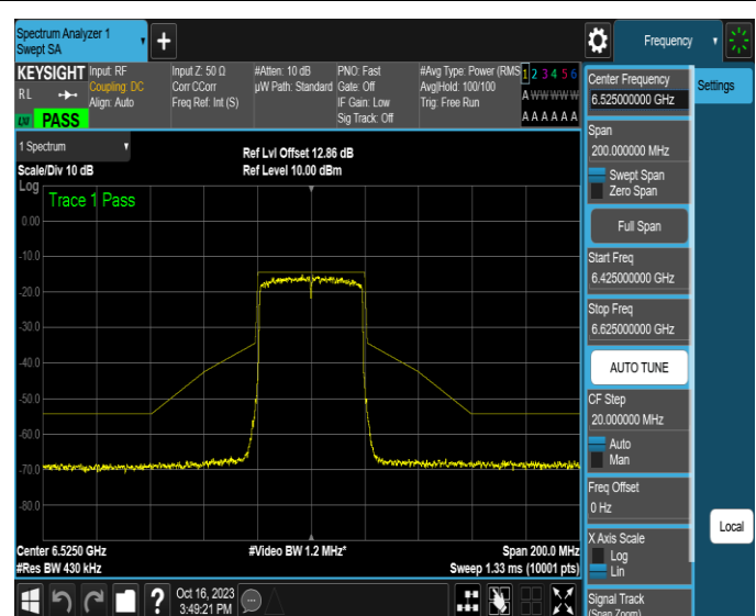
NTNV-11AX40MIMO-Ant2-6525-PASS
