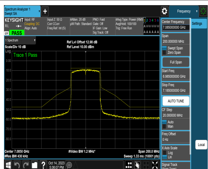
NTNV-11AX40SISO-Ant4-7085-PASS
