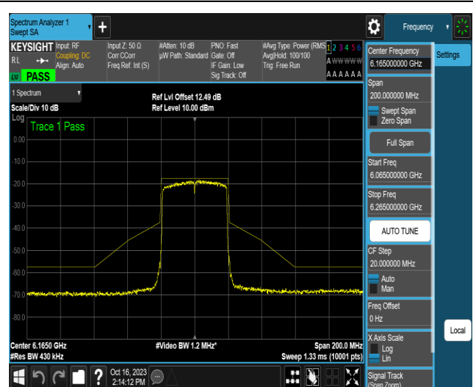
NTNV-11AX40MIMO-Ant2-6165-PASS
