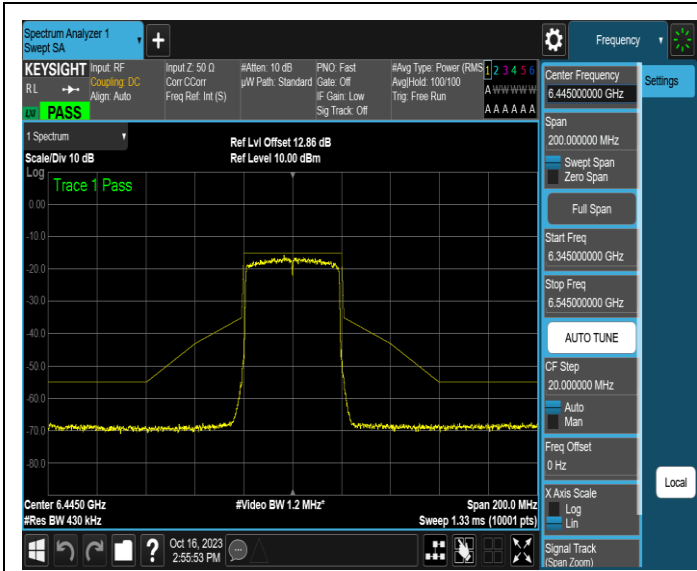
NTNV-11AX40MIMO-Ant1-6445-PASS
