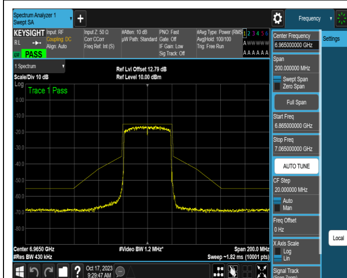
NTNV-11AX40MIMO-Ant3-6965-PASS
