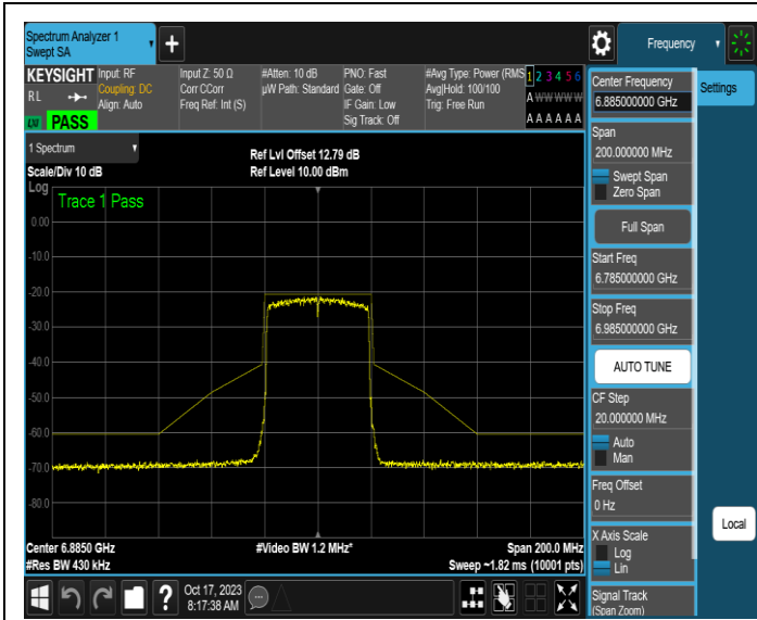
NTNV-11AX40MIMO-Ant1-6885-PASS
