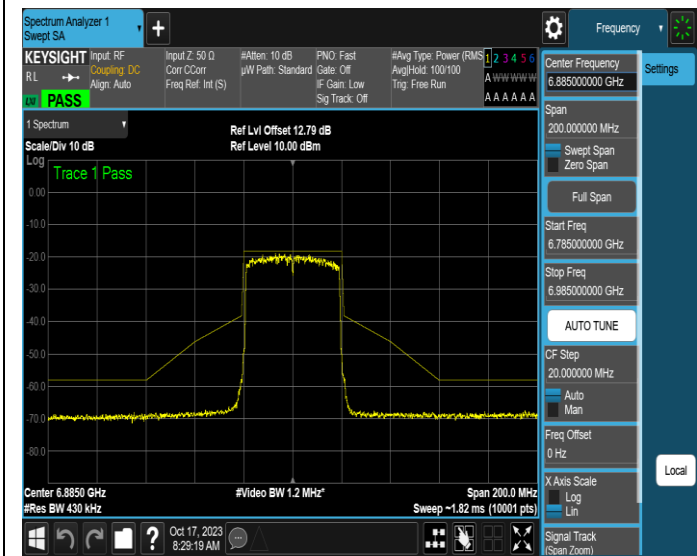
NTNV-11AX40MIMO-Ant3-6885-PASS
