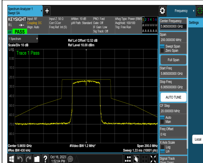
NTNV-11AX40MIMO-Ant3-5965-PASS
