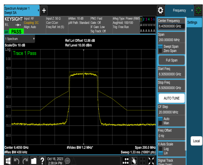
NTNV-11AX40MIMO-Ant2-6405-PASS
