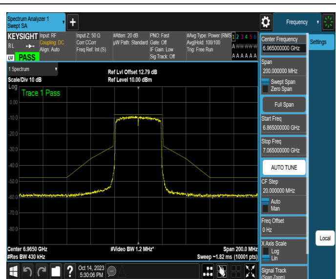
NTNV-11AX40SISO-Ant4-6965-PASS
