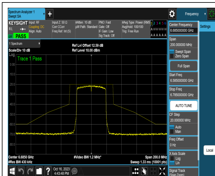
NTNV-11AX40MIMO-Ant3-6685-PASS
