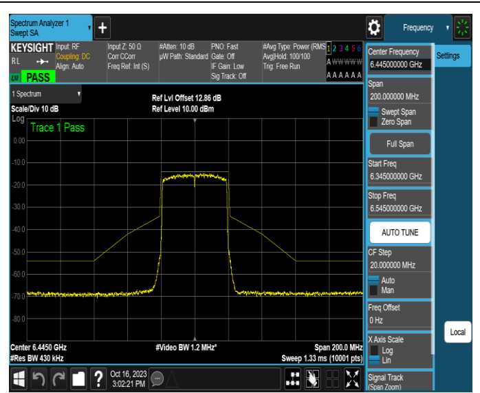
NTNV-11AX40MIMO-Ant2-6445-PASS
