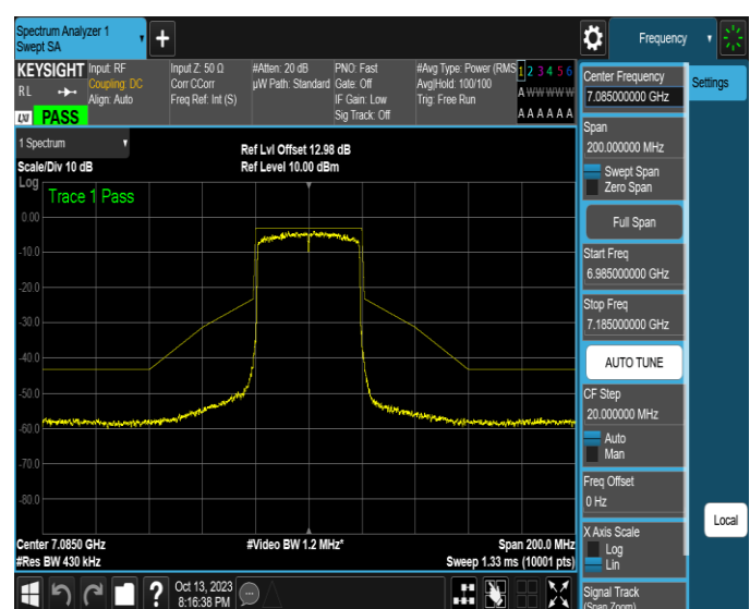
NTNV-11AX40SISO-Ant2-7085-PASS
