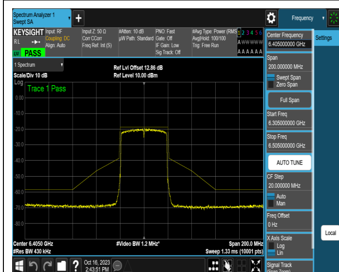
NTNV-11AX40MIMO-Ant3-6405-PASS
