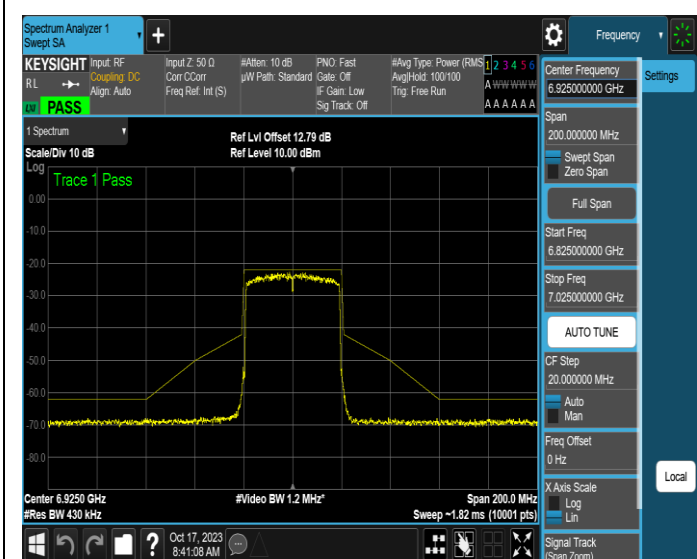
NTNV-11AX40MIMO-Ant1-6925-PASS
