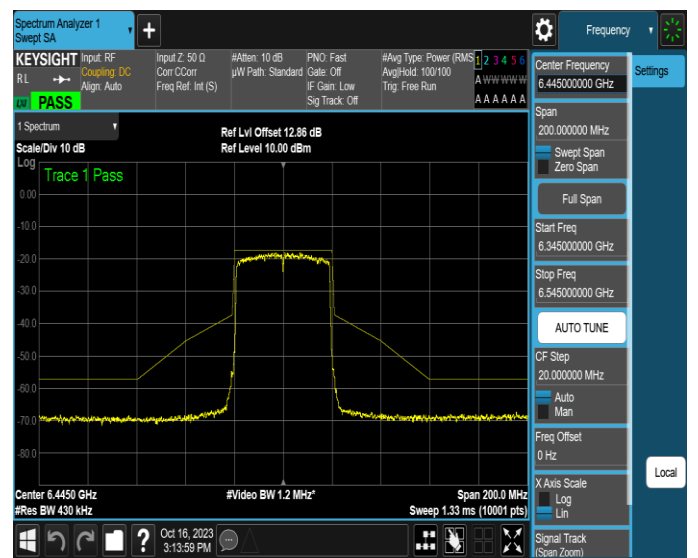
NTNV-11AX40MIMO-Ant4-6445-PASS
