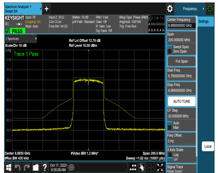
NTNV-11AX40MIMO-Ant4-6885-PASS
