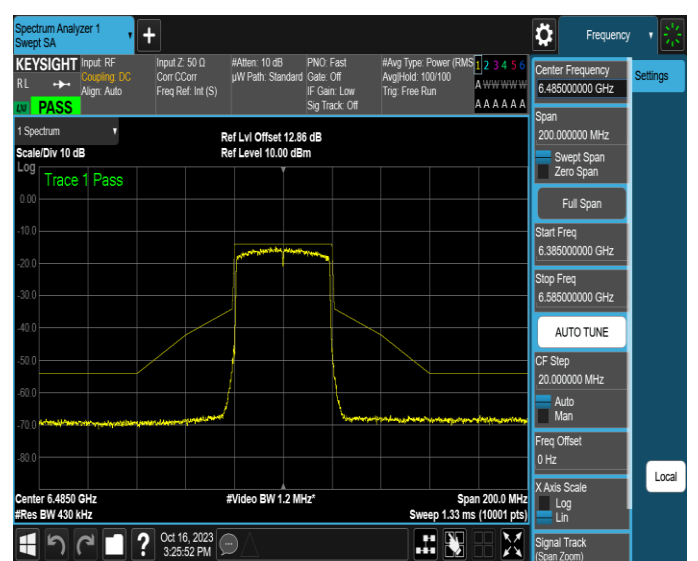
NTNV-11AX40MIMO-Ant2-6485-PASS
