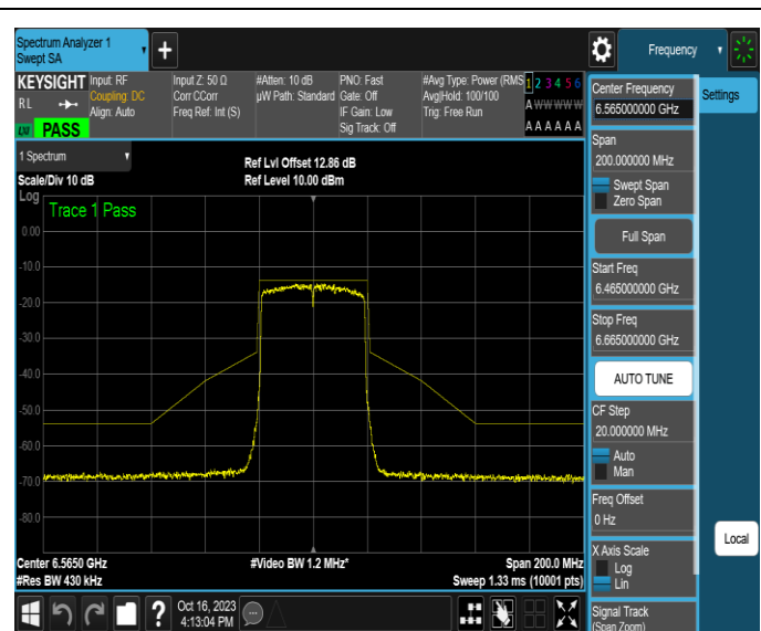
NTNV-11AX40MIMO-Ant2-6565-PASS
