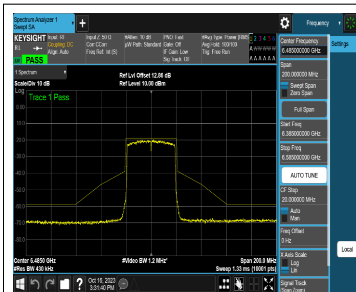
NTNV-11AX40MIMO-Ant3-6485-PASS
