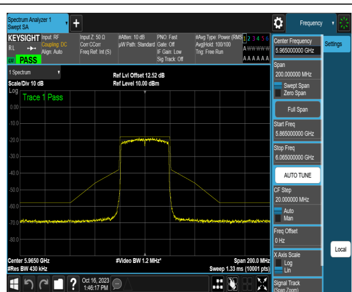
NTNV-11AX40MIMO-Ant2-5965-PASS
