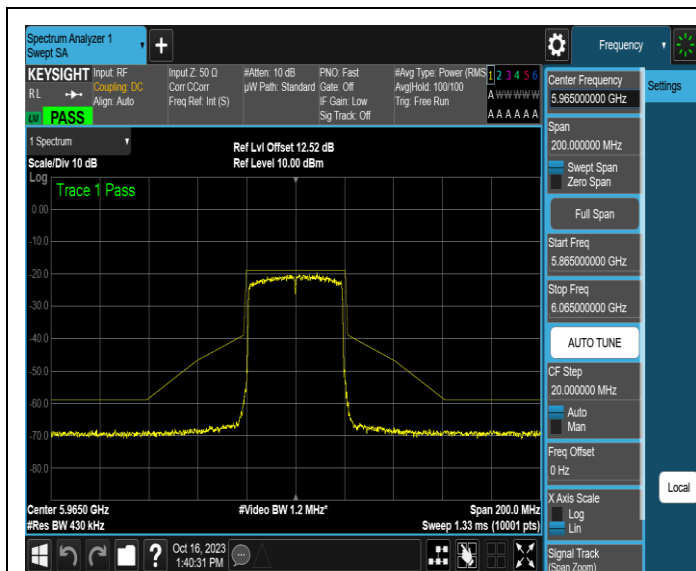
NTNV-11AX40MIMO-Ant1-5965-PASS
