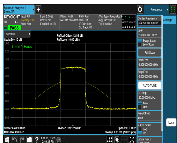
NTNV-11AX40MIMO-Ant4-6405-PASS
