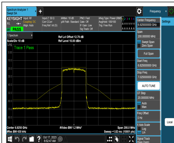
NTNV-11AX40MIMO-Ant3-6925-PASS
