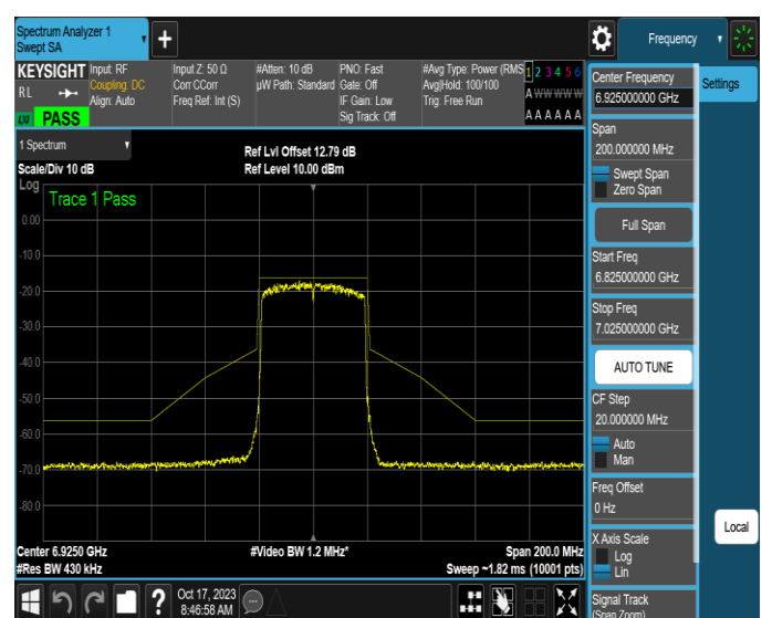
NTNV-11AX40MIMO-Ant2-6925-PASS
