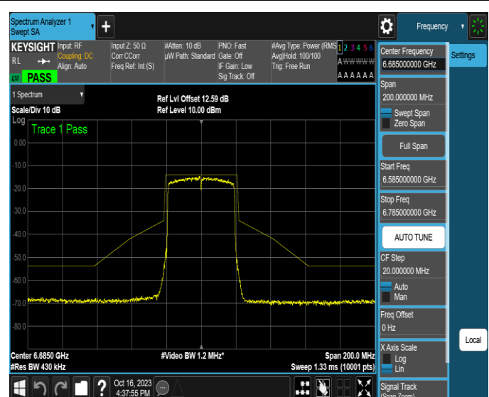
NTNV-11AX40MIMO-Ant2-6685-PASS
