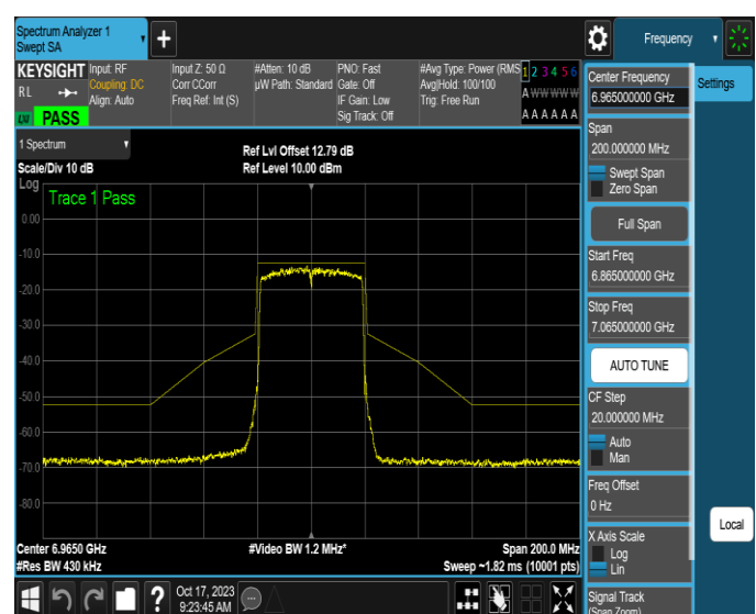
NTNV-11AX40MIMO-Ant2-6965-PASS
