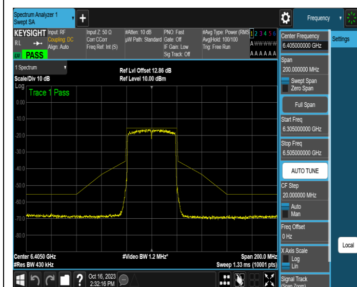
NTNV-11AX40MIMO-Ant1-6405-PASS
