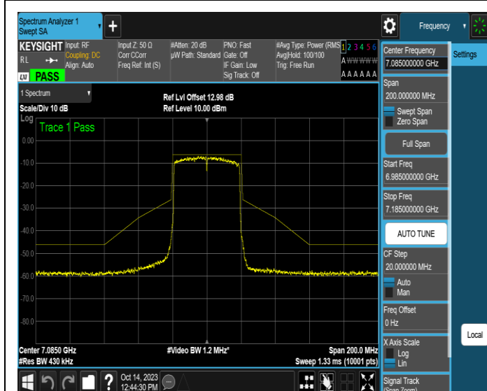
NTNV-11AX40SISO-Ant3-7085-PASS
