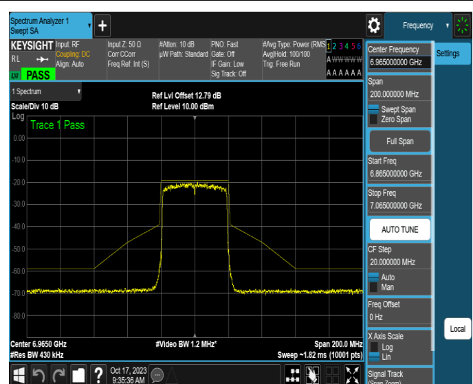
NTNV-11AX40MIMO-Ant4-6965-PASS
