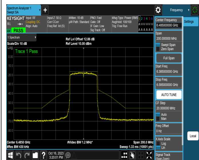
NTNV-11AX40MIMO-Ant1-6485-PASS
