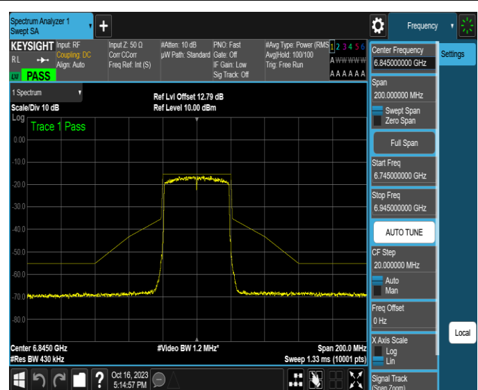
NTNV-11AX40MIMO-Ant4-6845-PASS
