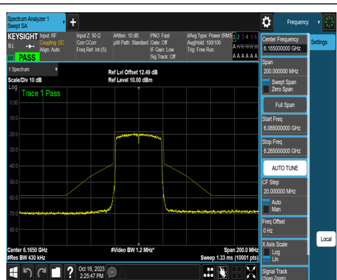
NTNV-11AX40MIMO-Ant4-6165-PASS
