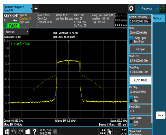
NTNV-11AX40MIMO-Ant2-6845-PASS
