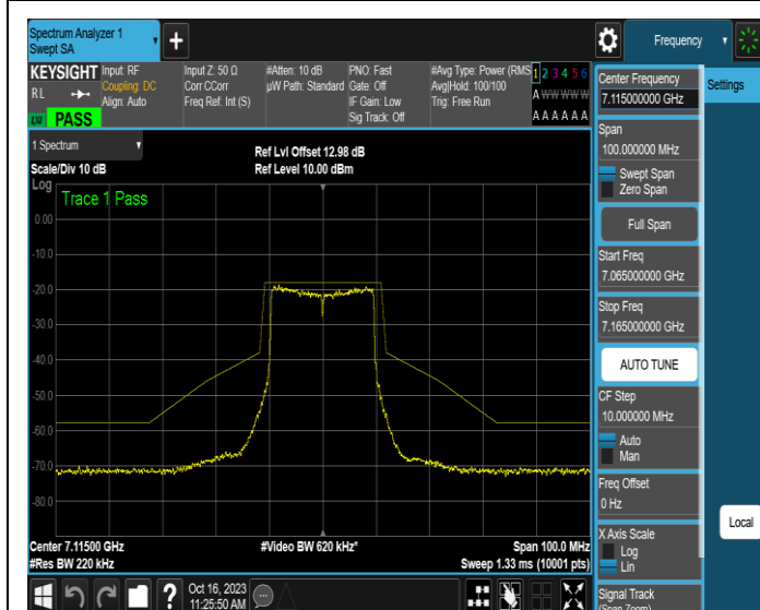
NTNV-11AX20MIMO-Ant1-7115-PASS
