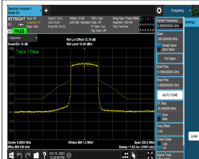
NTNV-11AX40SISO-Ant3-6885-PASS
