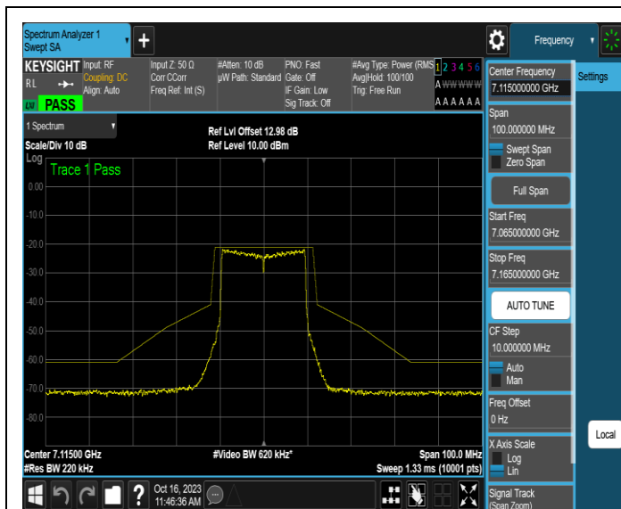
NTNV-11AX20MIMO-Ant3-7115-PASS
