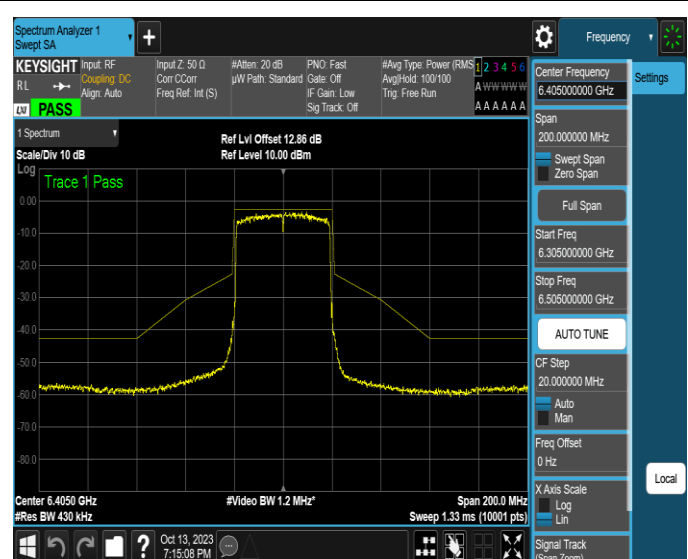
NTNV-11AX40SISO-Ant2-6405-PASS
