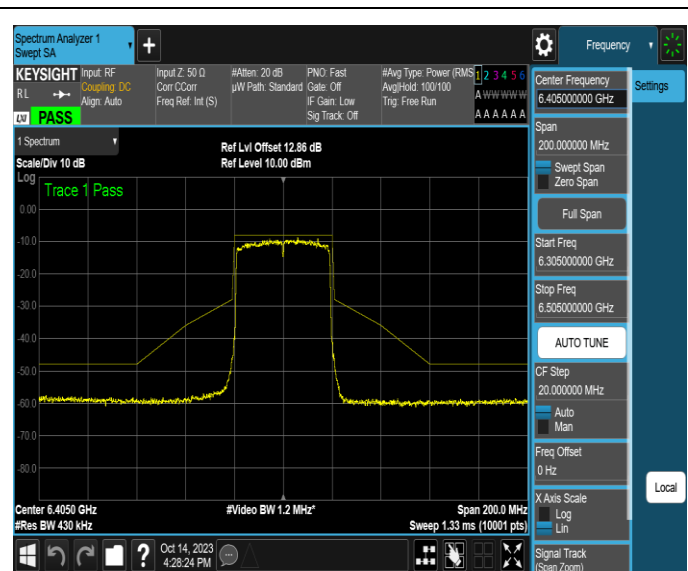
NTNV-11AX40SISO-Ant4-6405-PASS
