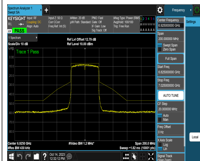
NTNV-11AX40SISO-Ant3-6925-PASS
