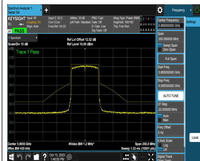
NTNV-11AX40SISO-Ant1-5965-PASS
