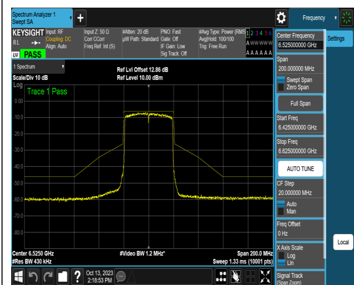
NTNV-11AX40SISO-Ant1-6525-PASS
