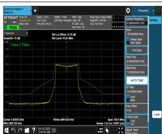
NTNV-11AX20MIMO-Ant2-6995-PASS
