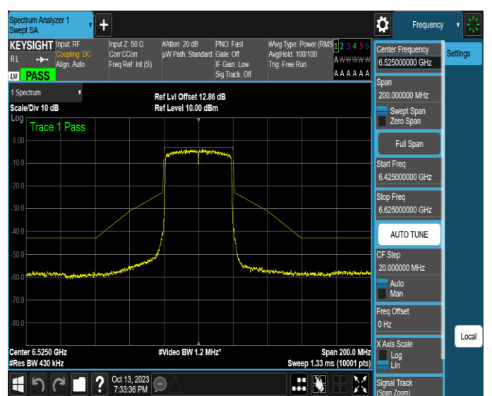
NTNV-11AX40SISO-Ant2-6525-PASS
