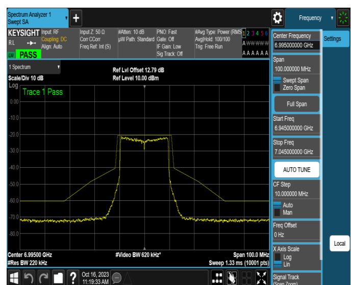
NTNV-11AX20MIMO-Ant4-6995-PASS
