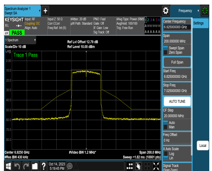
NTNV-11AX40SISO-Ant4-6925-PASS
