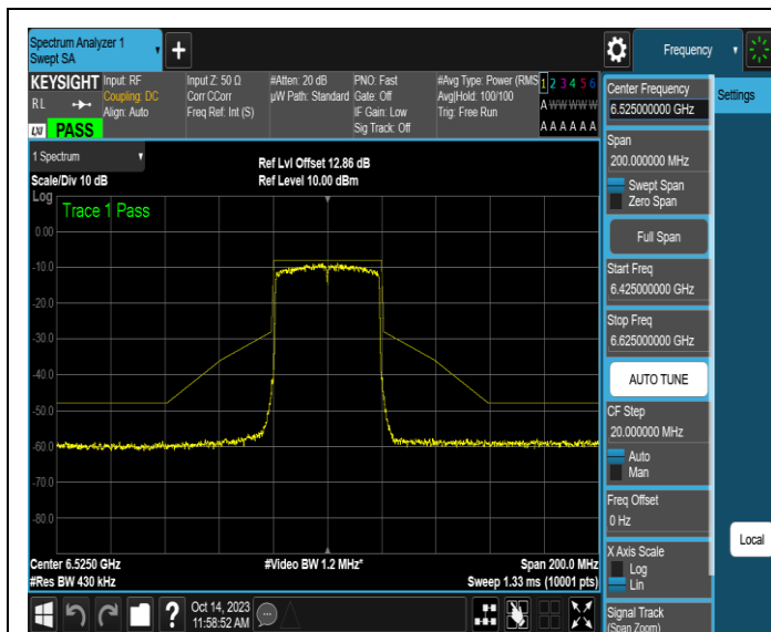
NTNV-11AX40SISO-Ant3-6525-PASS
