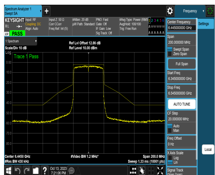
NTNV-11AX40SISO-Ant2-6445-PASS
