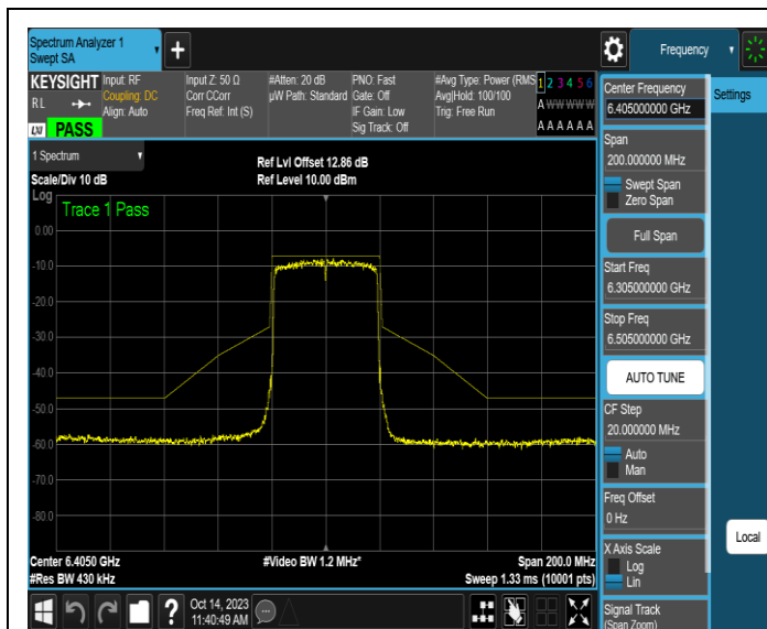
NTNV-11AX40SISO-Ant3-6405-PASS
