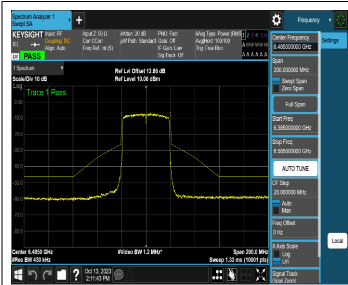
NTNV-11AX40SISO-Ant1-6485-PASS
