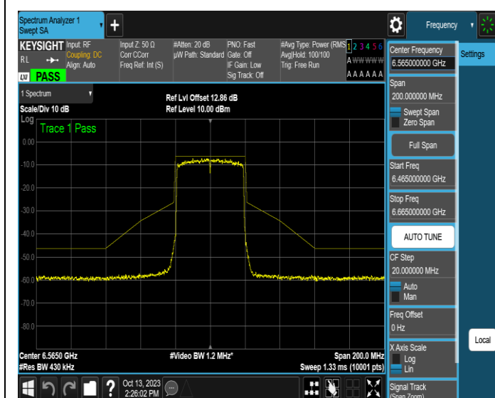
NTNV-11AX40SISO-Ant1-6565-PASS
