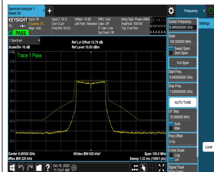
NTNV-11AX20MIMO-Ant3-6995-PASS
