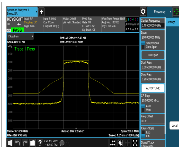
NTNV-11AX40SISO-Ant1-6165-PASS
