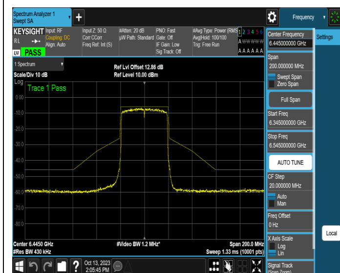
NTNV-11AX40SISO-Ant1-6445-PASS
