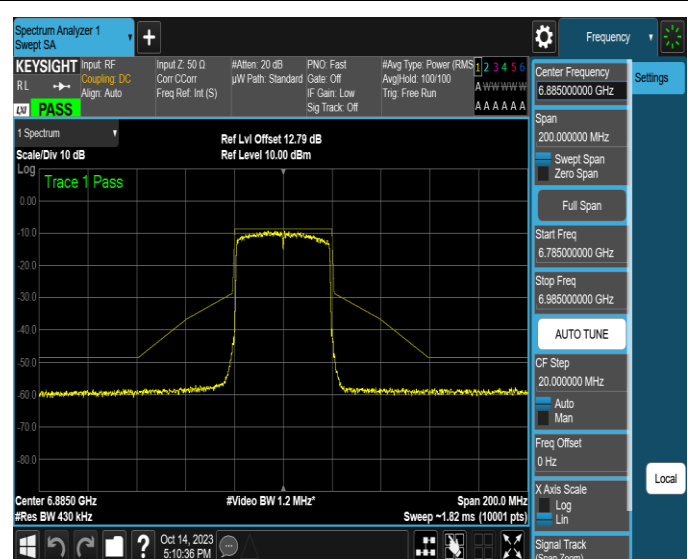
NTNV-11AX40SISO-Ant4-6885-PASS
