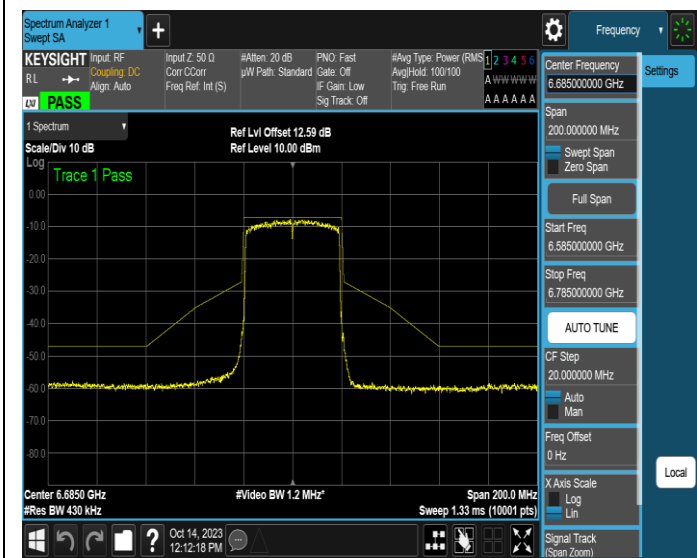
NTNV-11AX40SISO-Ant3-6685-PASS
