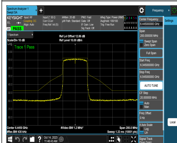
NTNV-11AX40SISO-Ant3-6445-PASS
