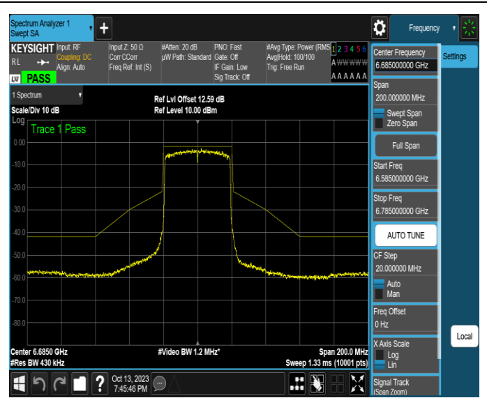
NTNV-11AX40SISO-Ant2-6685-PASS
