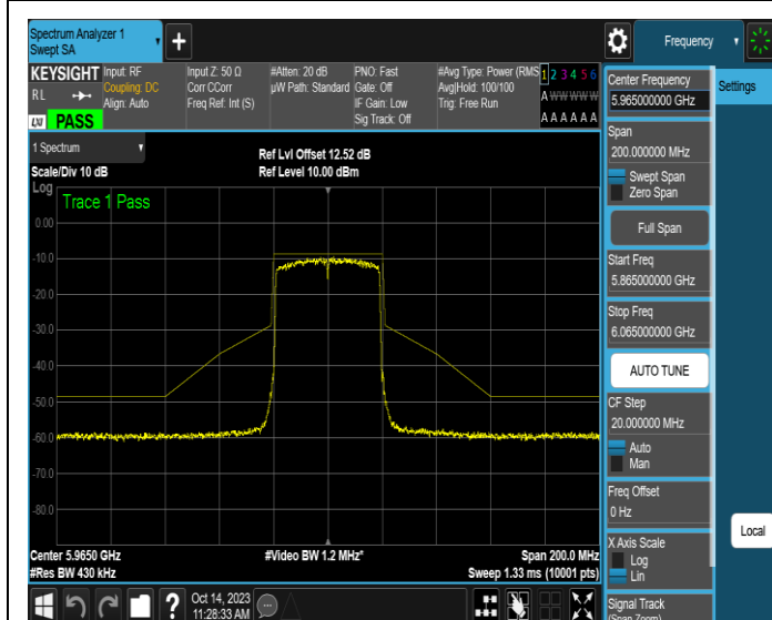
NTNV-11AX40SISO-Ant3-5965-PASS
