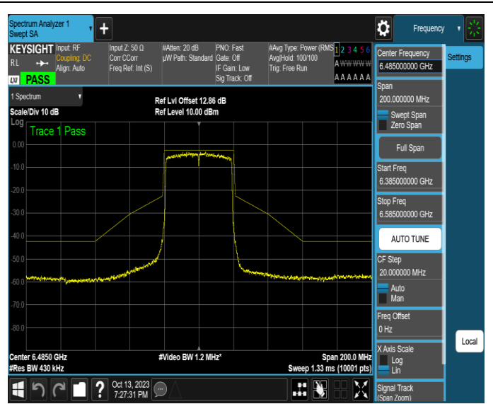
NTNV-11AX40SISO-Ant2-6485-PASS
