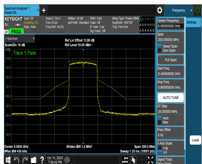
NTNV-11AX40SISO-Ant2-6565-PASS
