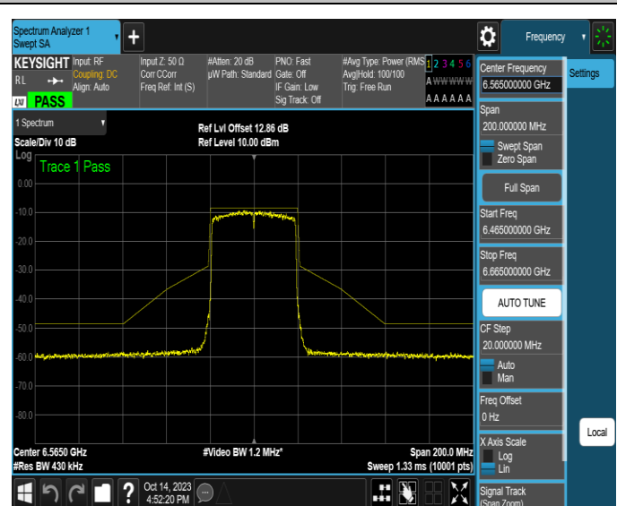
NTNV-11AX40SISO-Ant4-6565-PASS
