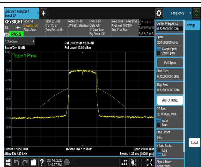
NTNV-11AX40SISO-Ant4-6525-PASS
