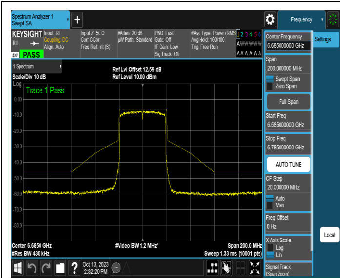
NTNV-11AX40SISO-Ant1-6685-PASS
