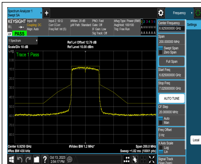
NTNV-11AX40SISO-Ant1-6925-PASS
