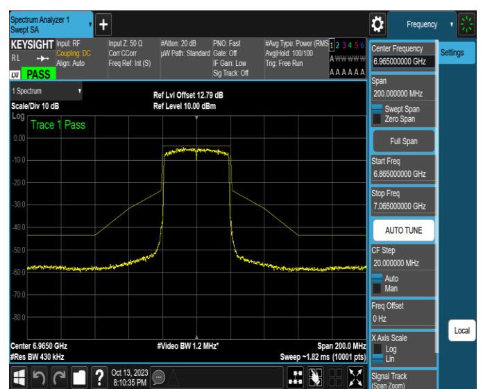
NTNV-11AX40SISO-Ant2-6965-PASS
