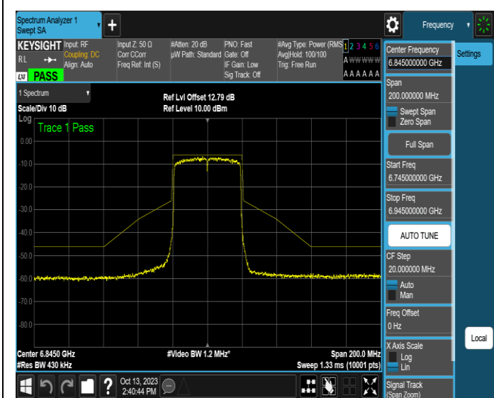
NTNV-11AX40SISO-Ant1-6845-PASS
