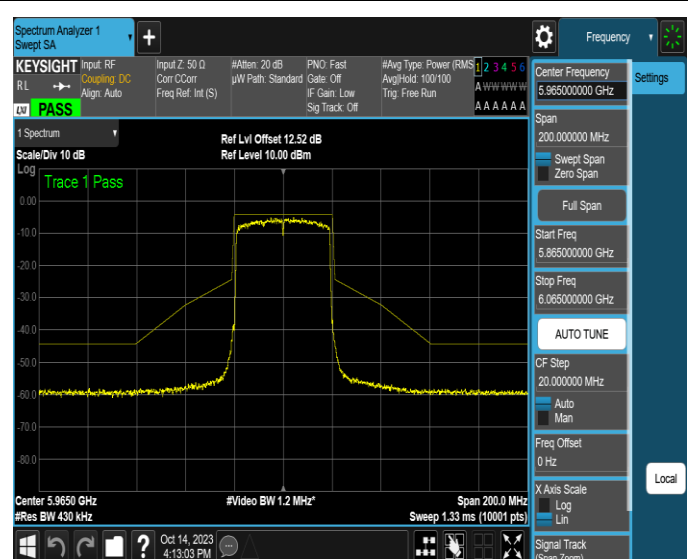
NTNV-11AX40SISO-Ant4-5965-PASS
