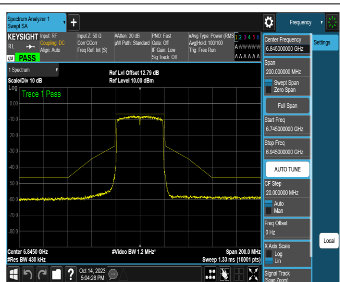
NTNV-11AX40SISO-Ant4-6845-PASS
