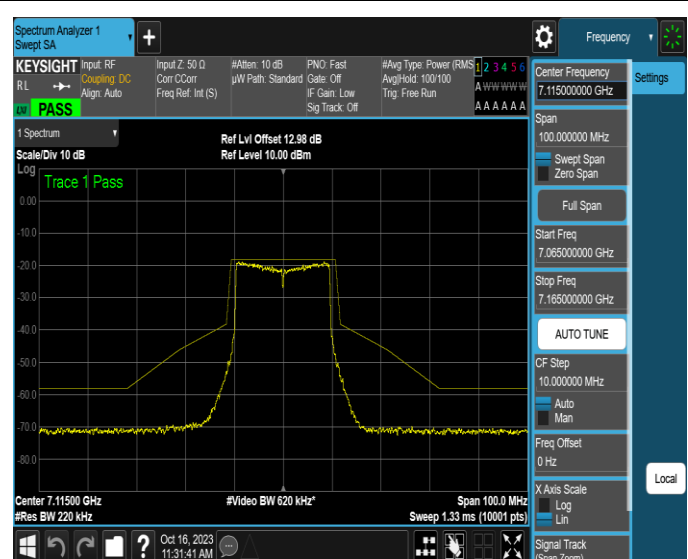
NTNV-11AX20MIMO-Ant2-7115-PASS
