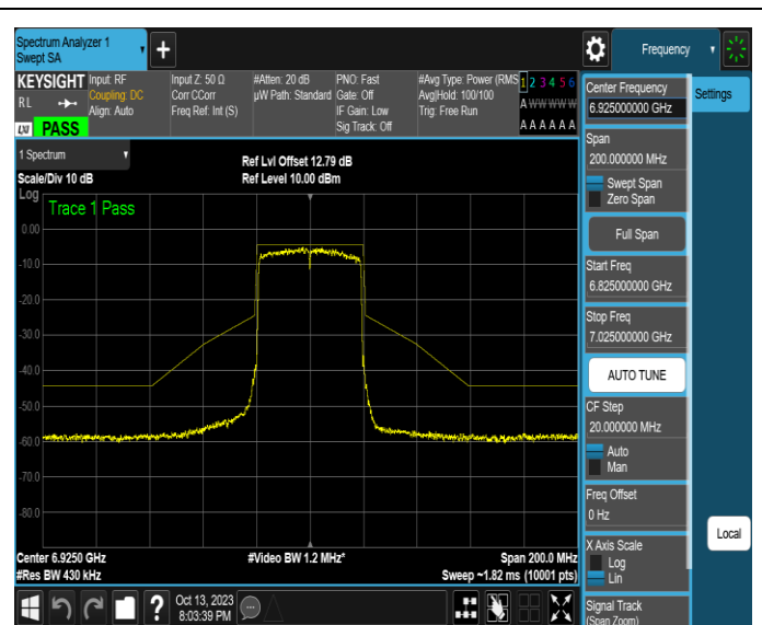
NTNV-11AX40SISO-Ant2-6925-PASS
