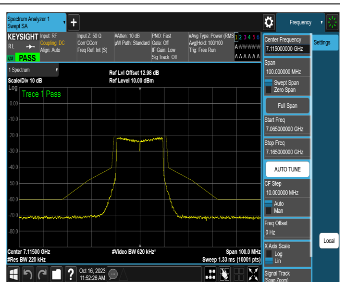
NTNV-11AX20MIMO-Ant4-7115-PASS
