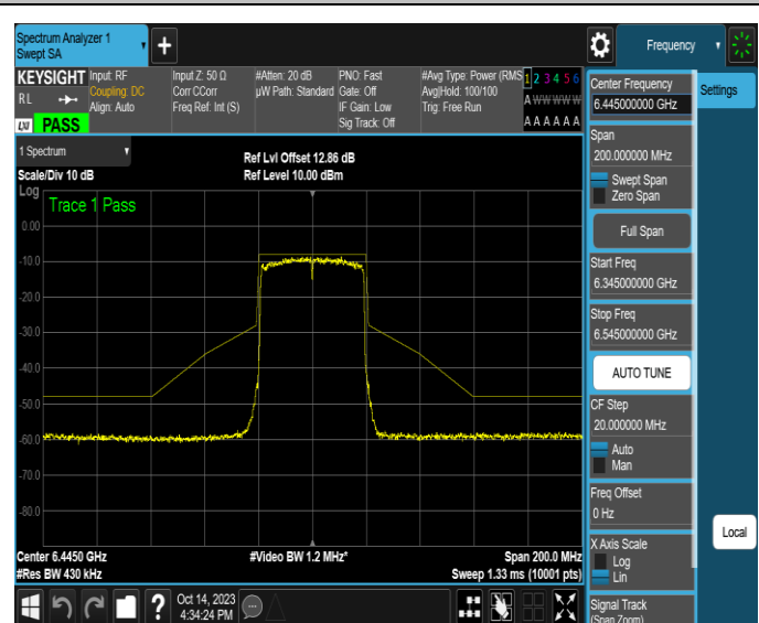
NTNV-11AX40SISO-Ant4-6445-PASS
