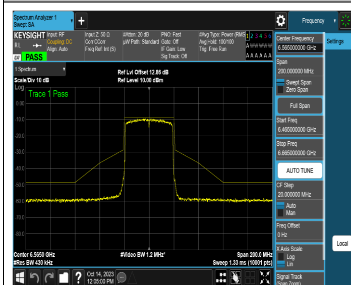
NTNV-11AX40SISO-Ant3-6565-PASS
