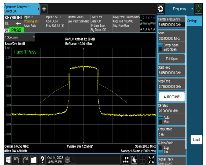
NTNV-11AX40SISO-Ant4-6685-PASS
