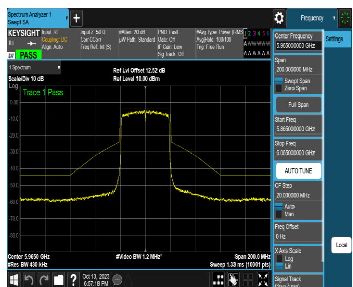
NTNV-11AX40SISO-Ant2-5965-PASS
