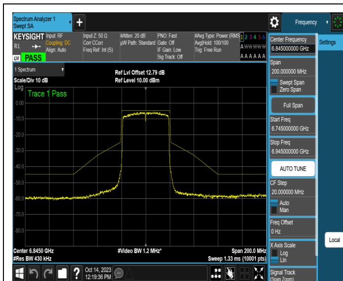
NTNV-11AX40SISO-Ant3-6845-PASS
