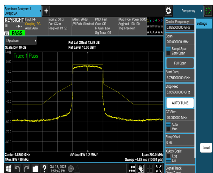
NTNV-11AX40SISO-Ant2-6885-PASS
