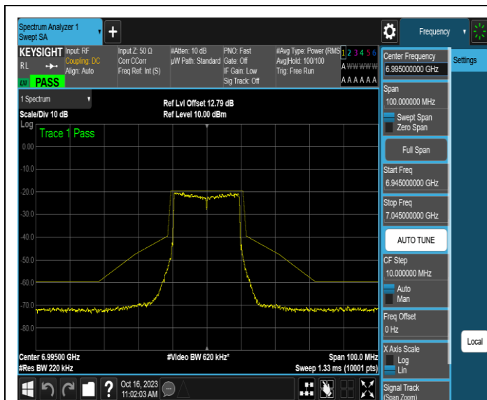
NTNV-11AX20MIMO-Ant1-6995-PASS
