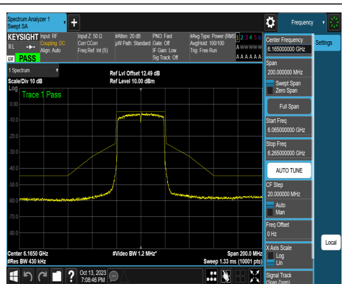
NTNV-11AX40SISO-Ant2-6165-PASS
