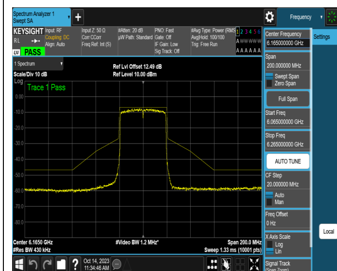
NTNV-11AX40SISO-Ant3-6165-PASS
