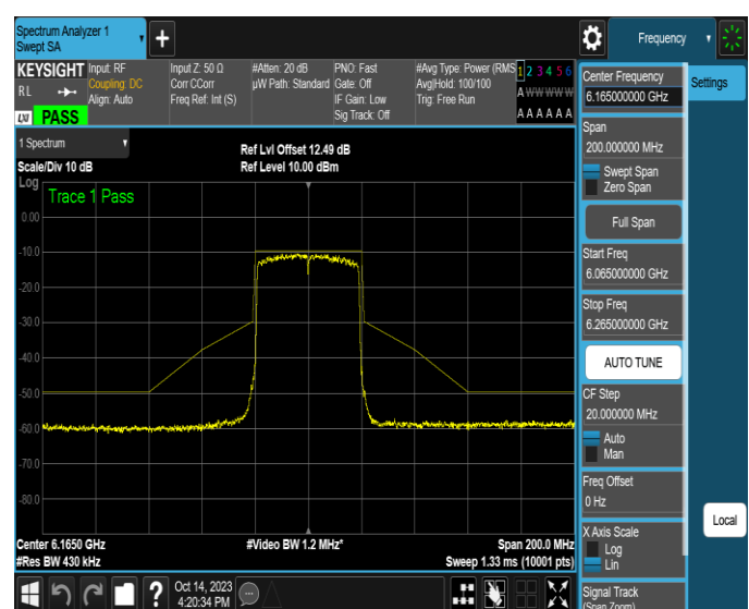
NTNV-11AX40SISO-Ant4-6165-PASS
