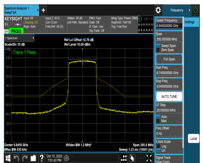
NTNV-11AX40SISO-Ant2-6845-PASS
