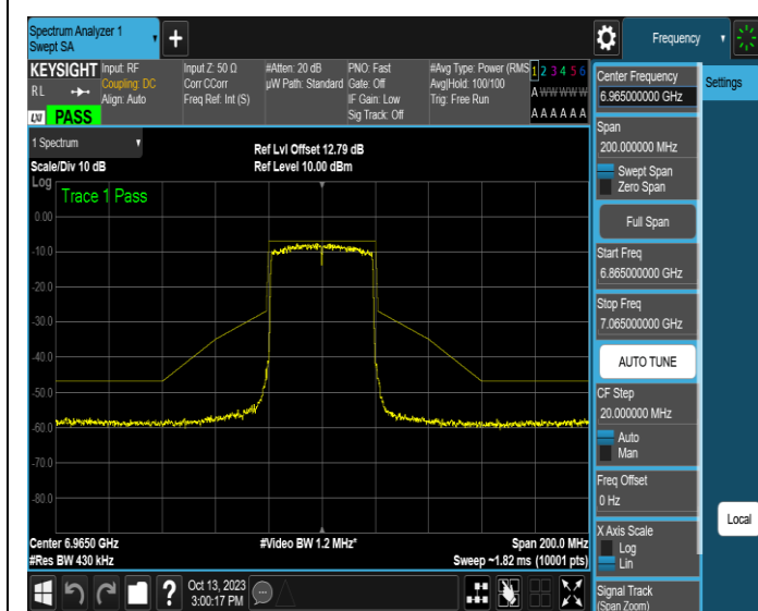
NTNV-11AX40SISO-Ant1-6965-PASS
