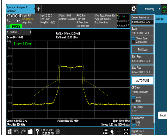
NTNV-11AX20MIMO-Ant1-6895-PASS
