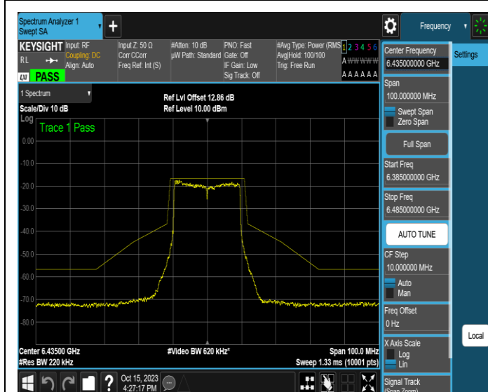
NTNV-11AX20MIMO-Ant1-6435-PASS
