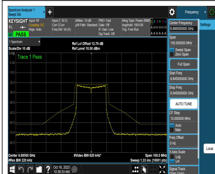
NTNV-11AX20MIMO-Ant3-6895-PASS
