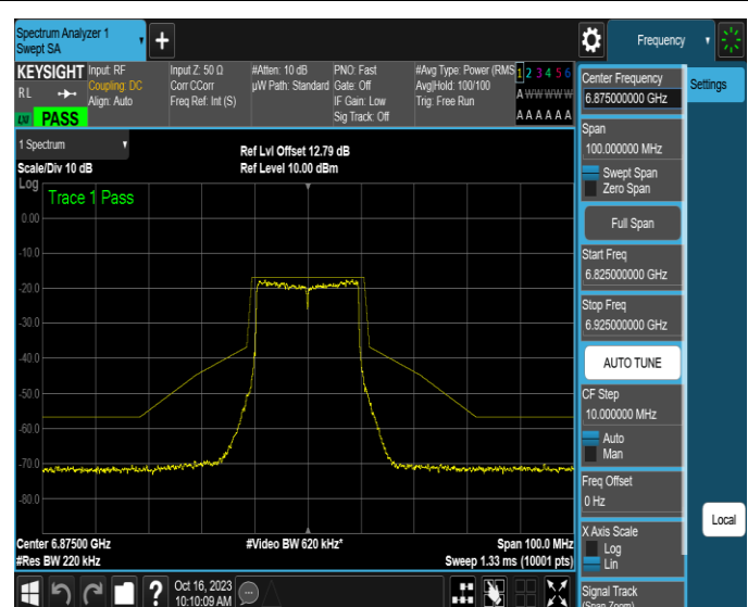
NTNV-11AX20MIMO-Ant2-6875-PASS
