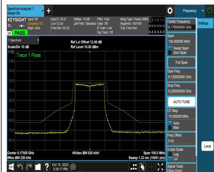
NTNV-11AX20MIMO-Ant3-6175-PASS
