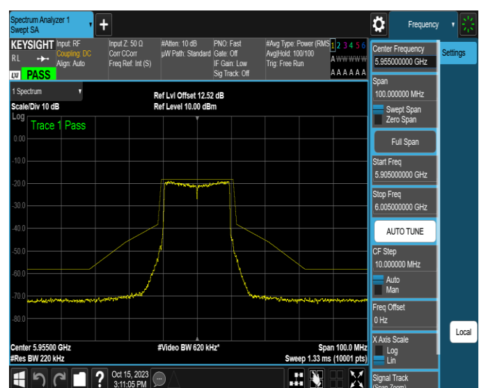
NTNV-11AX20MIMO-Ant2-5955-PASS
