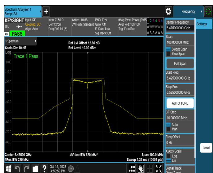
NTNV-11AX20MIMO-Ant2-6475-PASS
