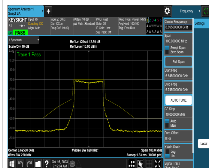
NTNV-11AX20MIMO-Ant1-6695-PASS
