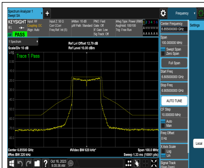
NTNV-11AX20MIMO-Ant1-6855-PASS
