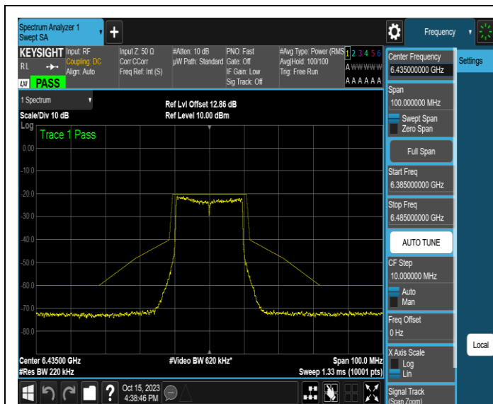
NTNV-11AX20MIMO-Ant3-6435-PASS
