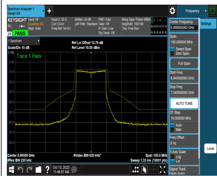
NTNV-11AX20SISO-Ant1-6995-PASS
