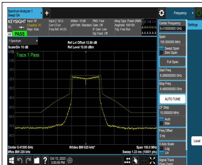
NTNV-11AX20MIMO-Ant1-6415-PASS
