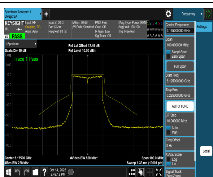
NTNV-11AX20SISO-Ant4-6175-PASS
