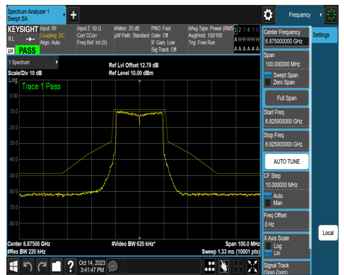
NTNV-11AX20SISO-Ant4-6875-PASS
