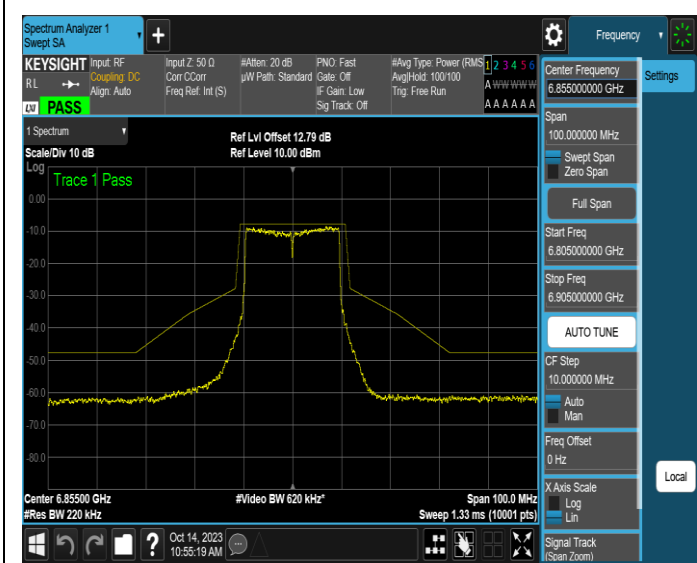
NTNV-11AX20SISO-Ant3-6855-PASS
