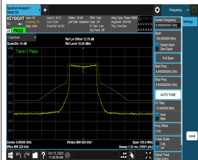
NTNV-11AX20SISO-Ant1-6895-PASS
