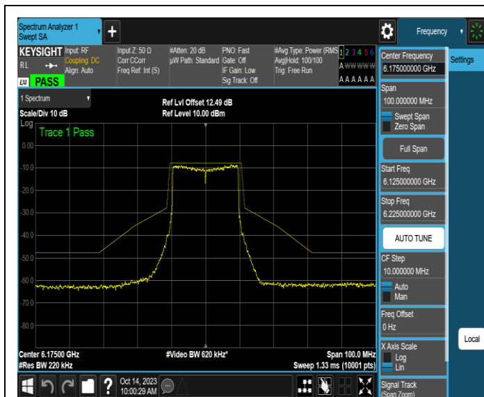
NTNV-11AX20SISO-Ant3-6175-PASS
