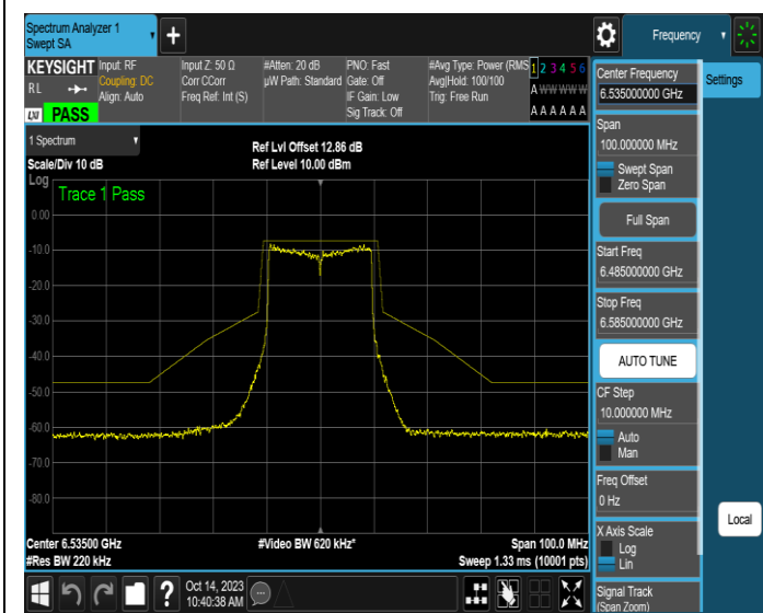
NTNV-11AX20SISO-Ant3-6535-PASS
