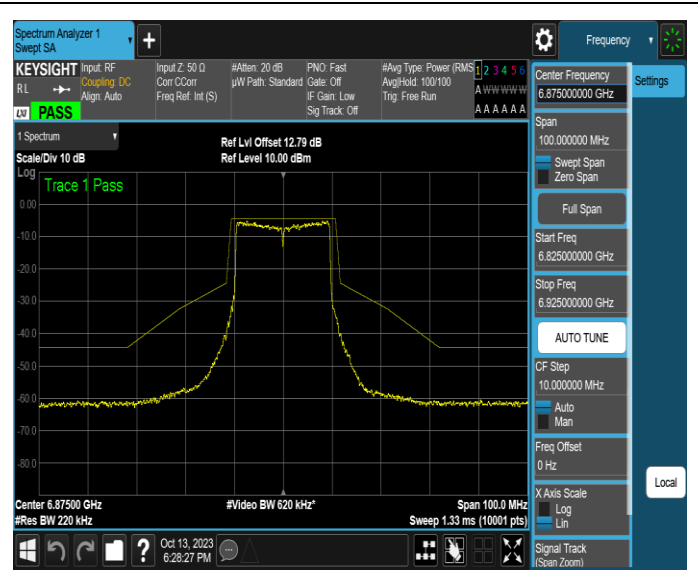
NTNV-11AX20SISO-Ant2-6875-PASS
