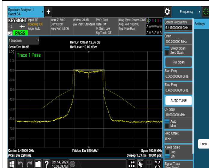
NTNV-11AX20SISO-Ant3-6415-PASS
