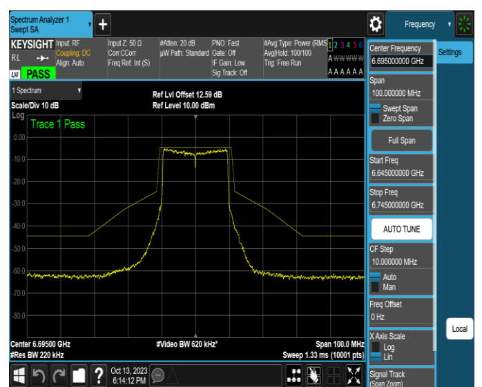
NTNV-11AX20SISO-Ant2-6695-PASS
