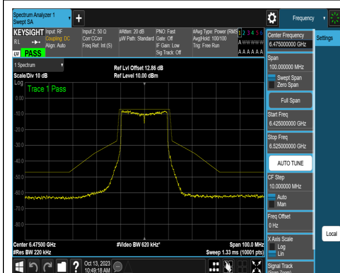
NTNV-11AX20SISO-Ant1-6475-PASS
