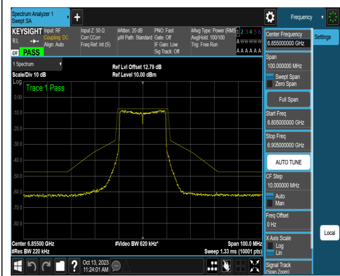
NTNV-11AX20SISO-Ant1-6855-PASS
