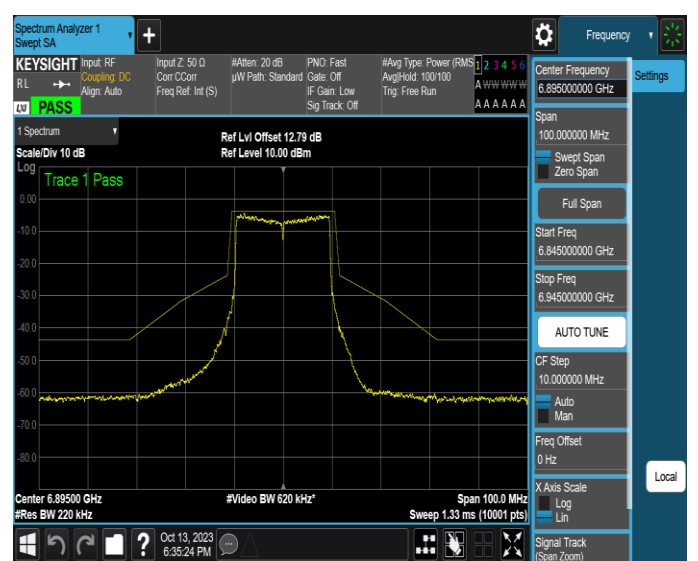
NTNV-11AX20SISO-Ant2-6895-PASS
