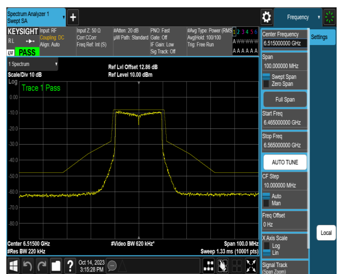
NTNV-11AX20SISO-Ant4-6515-PASS
