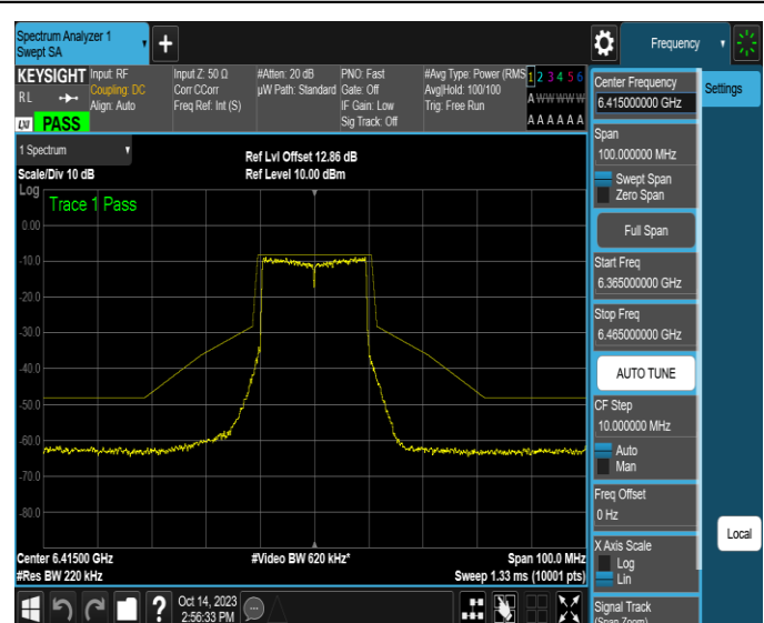
NTNV-11AX20SISO-Ant4-6415-PASS
