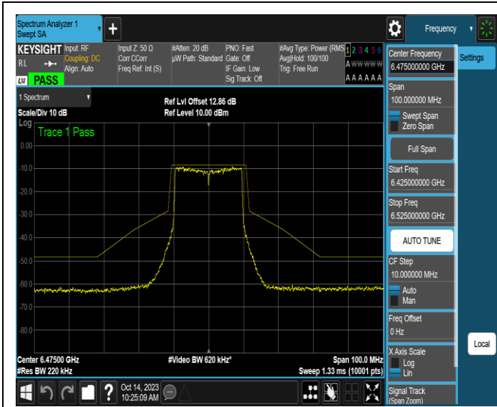
NTNV-11AX20SISO-Ant3-6475-PASS
