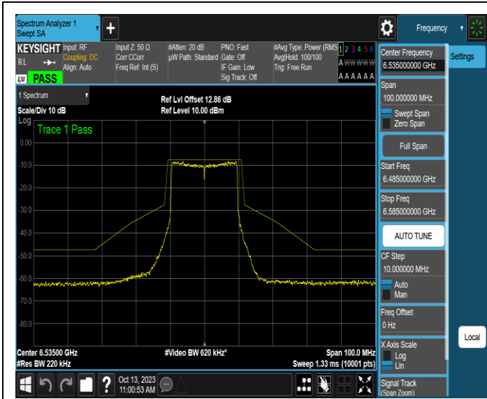
NTNV-11AX20SISO-Ant1-6535-PASS
