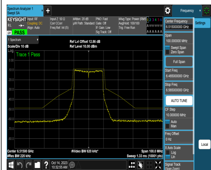
NTNV-11AX20SISO-Ant3-6515-PASS
