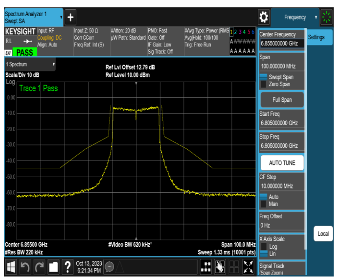
NTNV-11AX20SISO-Ant2-6855-PASS
