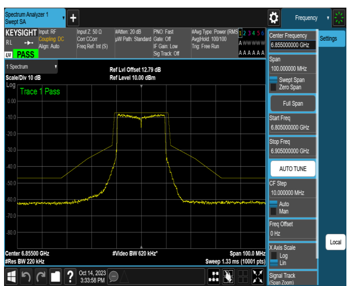
NTNV-11AX20SISO-Ant4-6855-PASS
