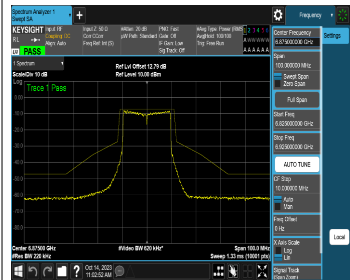
NTNV-11AX20SISO-Ant3-6875-PASS
