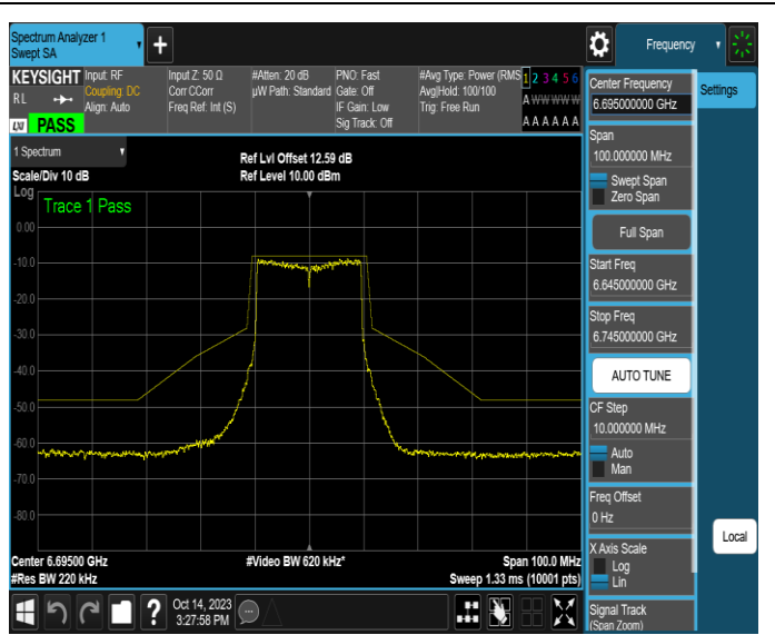
NTNV-11AX20SISO-Ant4-6695-PASS
