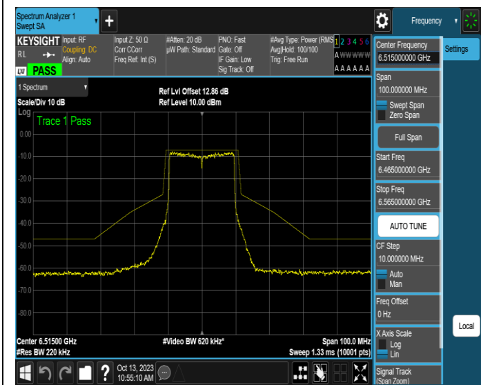
NTNV-11AX20SISO-Ant1-6515-PASS
