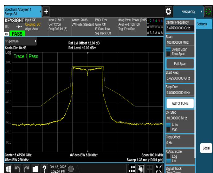
NTNV-11AX20SISO-Ant2-6475-PASS
