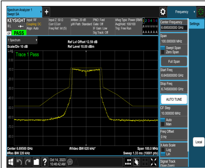
NTNV-11AX20SISO-Ant3-6695-PASS
