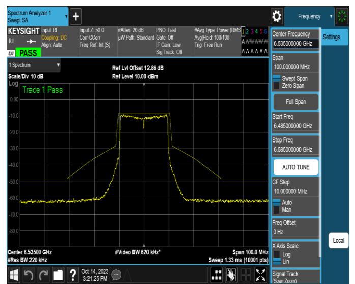
NTNV-11AX20SISO-Ant4-6535-PASS
