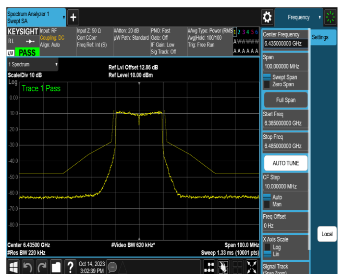
NTNV-11AX20SISO-Ant4-6435-PASS
