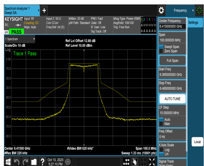
NTNV-11AX20SISO-Ant2-6415-PASS
