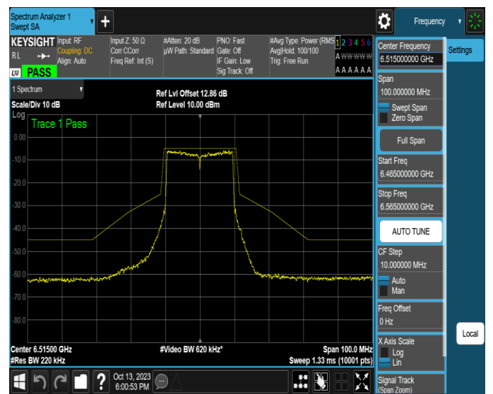
NTNV-11AX20SISO-Ant2-6515-PASS
