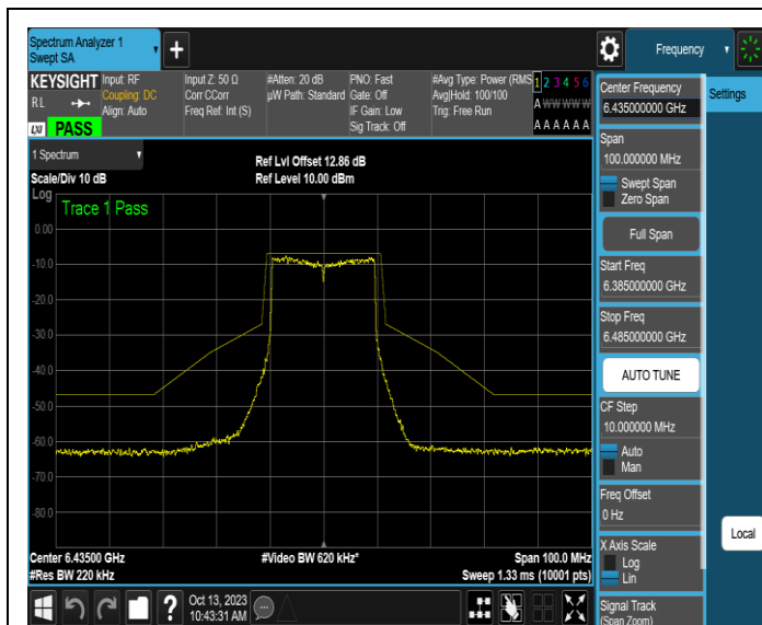
NTNV-11AX20SISO-Ant1-6435-PASS
