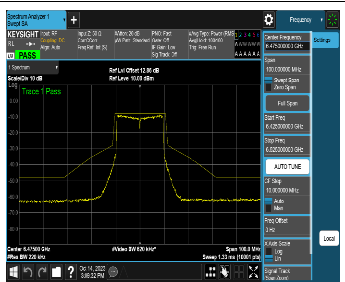
NTNV-11AX20SISO-Ant4-6475-PASS
