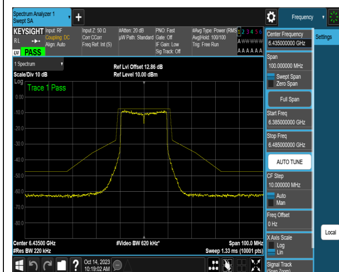
NTNV-11AX20SISO-Ant3-6435-PASS
