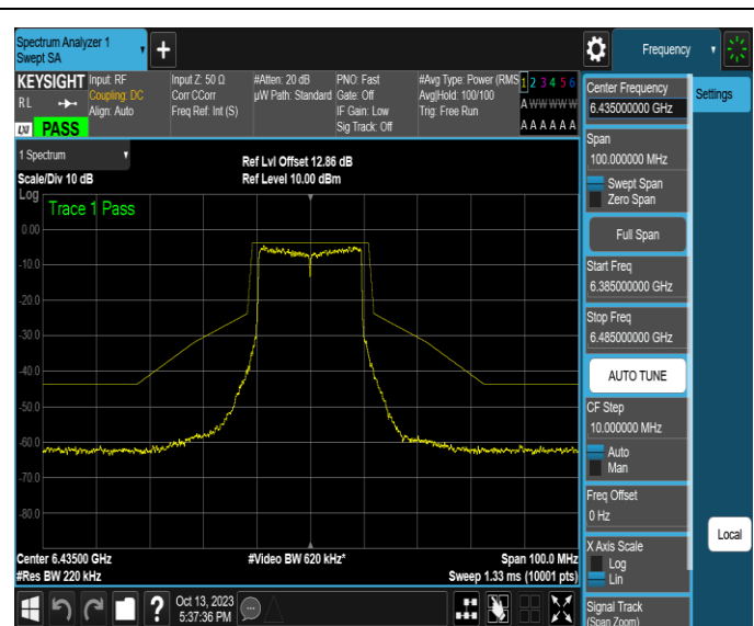
NTNV-11AX20SISO-Ant2-6435-PASS
