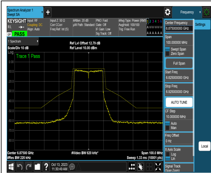
NTNV-11AX20SISO-Ant1-6875-PASS
