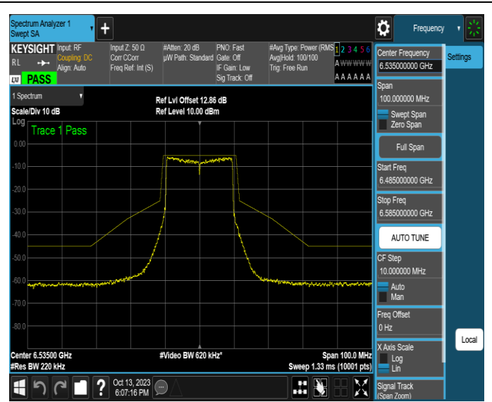
NTNV-11AX20SISO-Ant2-6535-PASS
