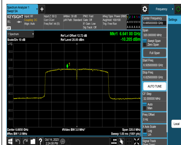
11AX160SISO-Ant3-6665-PASS
