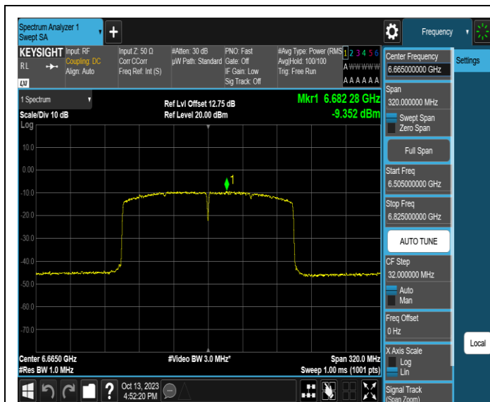
11AX160SISO-Ant1-6665-PASS
