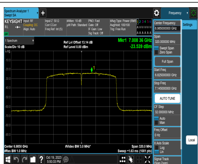
11AX160MIMO-Ant2-6985-PASS
