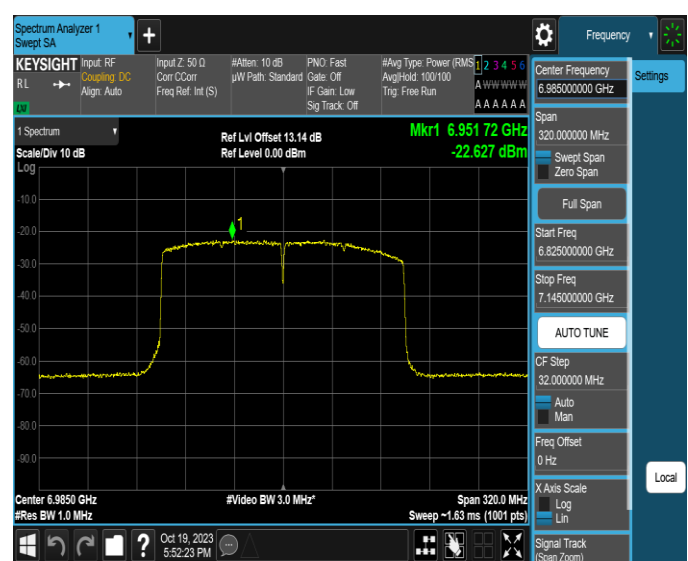
11AX160MIMO-Ant4-6985-PASS
