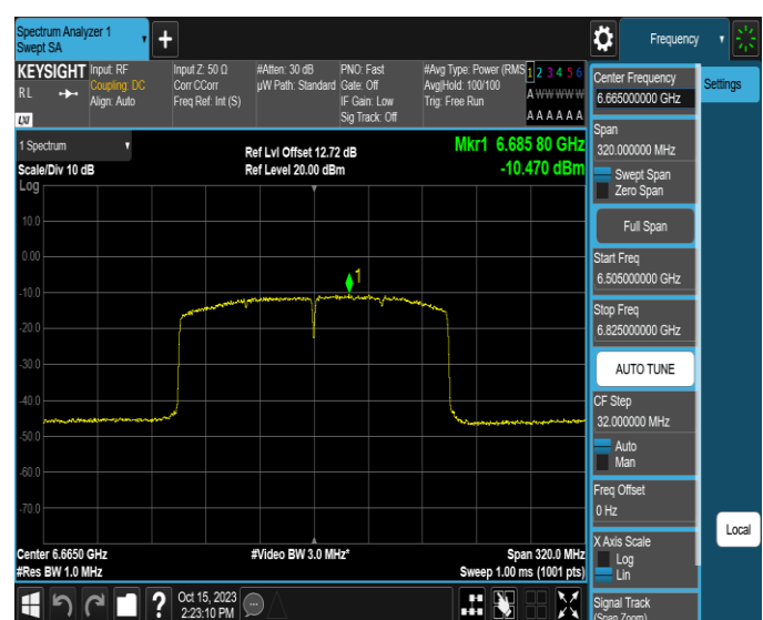
11AX160SISO-Ant4-6665-PASS
