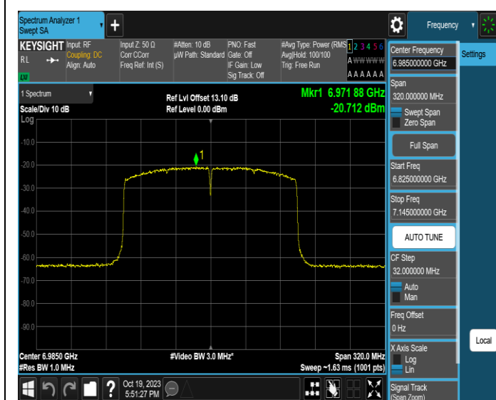
11AX160MIMO-Ant3-6985-PASS
