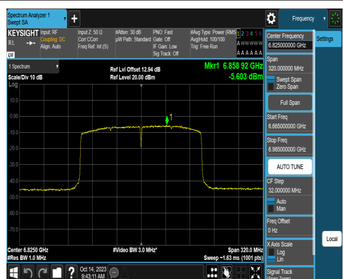
11AX160SISO-Ant2-6825-PASS
