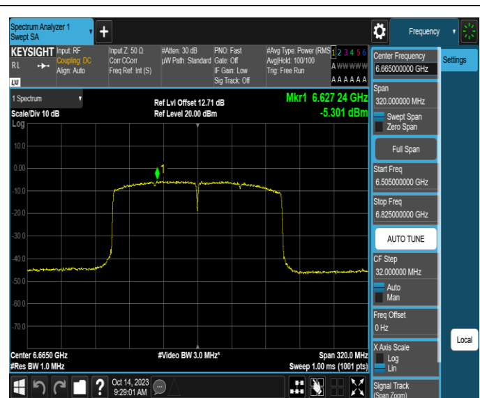
11AX160SISO-Ant2-6665-PASS
