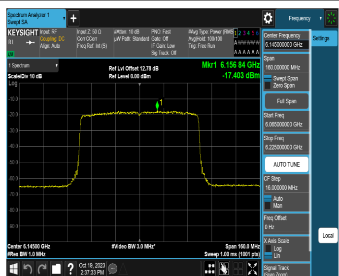
11AX80MIMO-Ant2-6145-PASS
