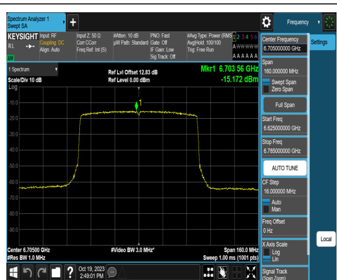
11AX80MIMO-Ant2-6705-PASS
