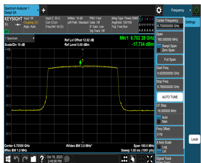
11AX80MIMO-Ant4-6705-PASS
