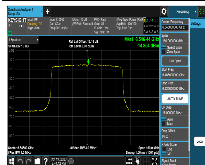
11AX80MIMO-Ant1-6545-PASS
