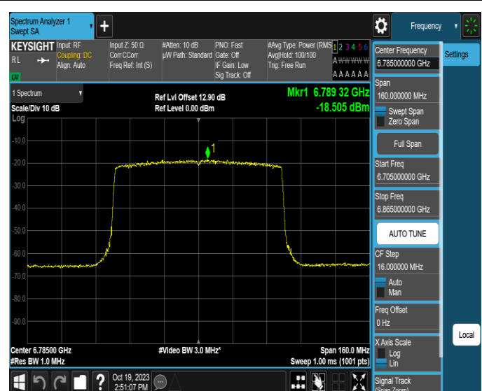
11AX80MIMO-Ant2-6785-PASS
