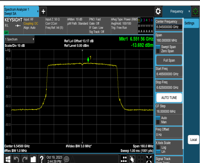
11AX80MIMO-Ant2-6545-PASS
