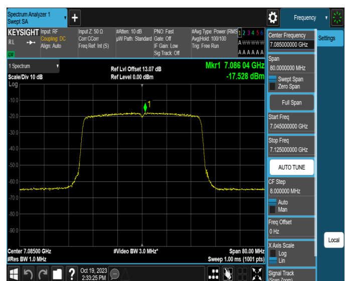
11AX40MIMO-Ant4-7085-PASS
