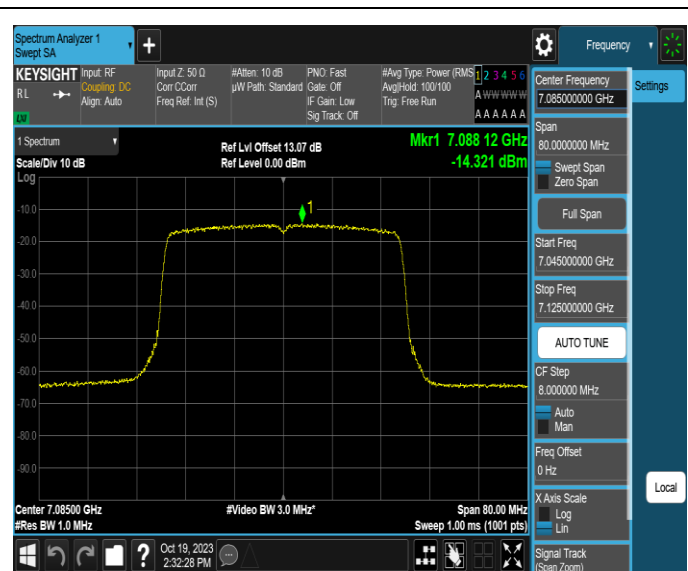
11AX40MIMO-Ant2-7085-PASS
