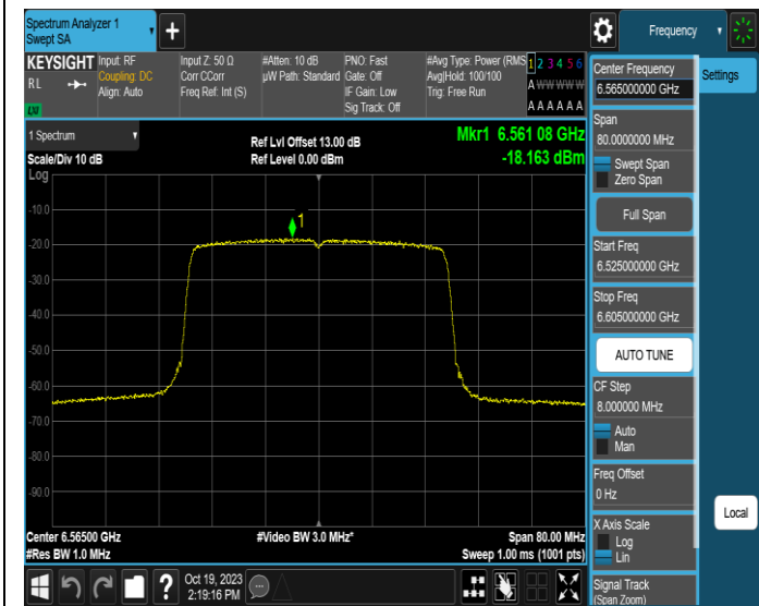
11AX40MIMO-Ant3-6565-PASS
