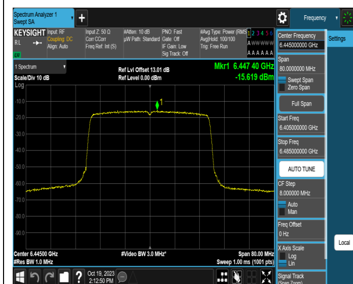
11AX40MIMO-Ant3-6445-PASS
