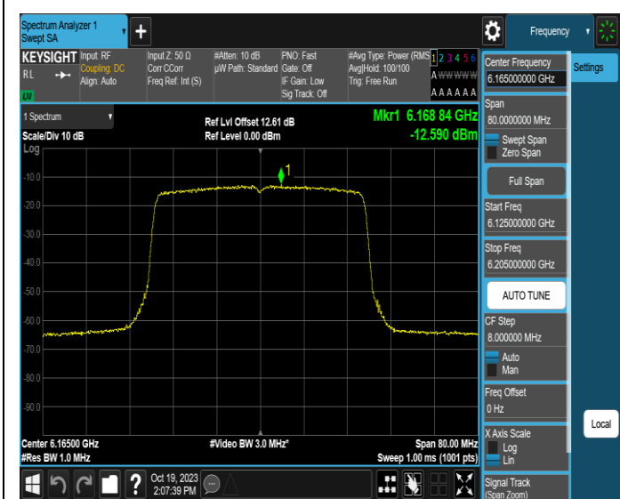
11AX40MIMO-Ant1-6165-PASS
