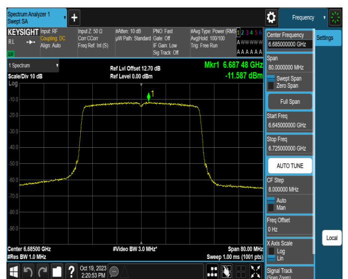
11AX40MIMO-Ant2-6685-PASS
