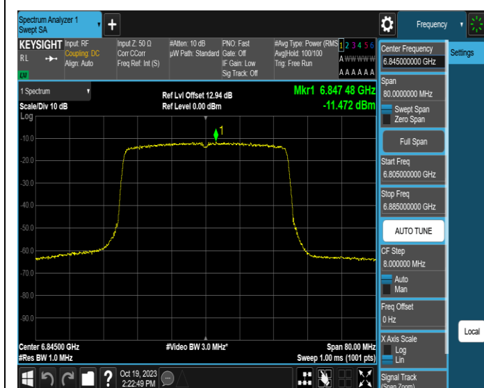
11AX40MIMO-Ant1-6845-PASS
