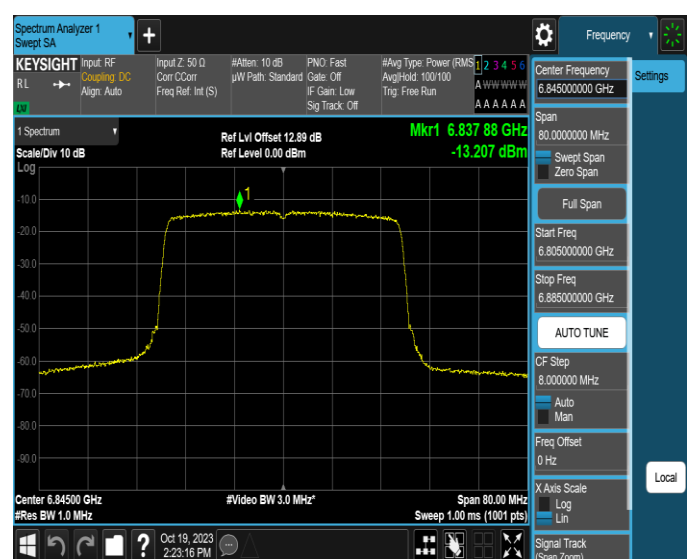
11AX40MIMO-Ant2-6845-PASS
