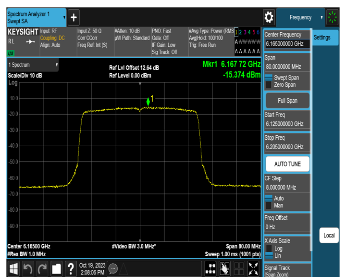
11AX40MIMO-Ant2-6165-PASS
