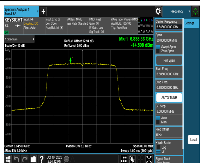
11AX40MIMO-Ant4-6845-PASS
