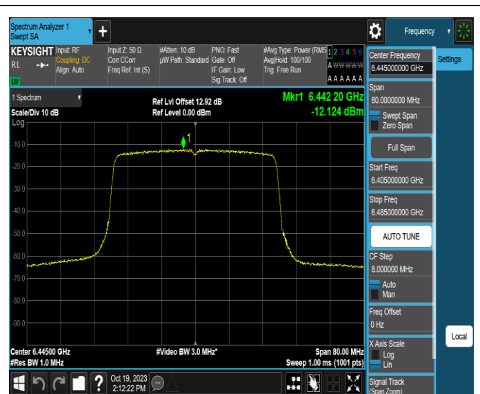
11AX40MIMO-Ant2-6445-PASS
