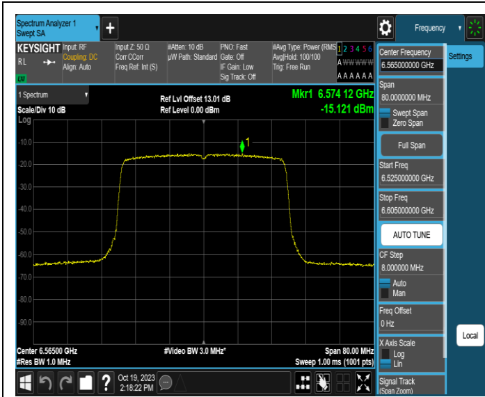
11AX40MIMO-Ant1-6565-PASS
