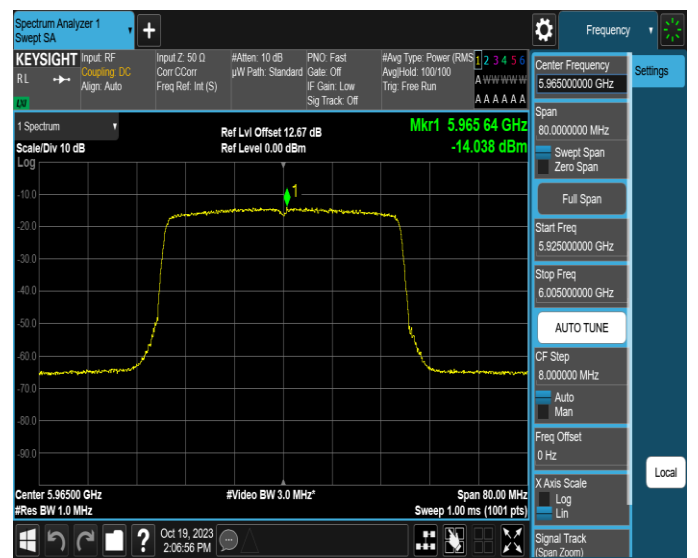
11AX40MIMO-Ant4-5965-PASS
