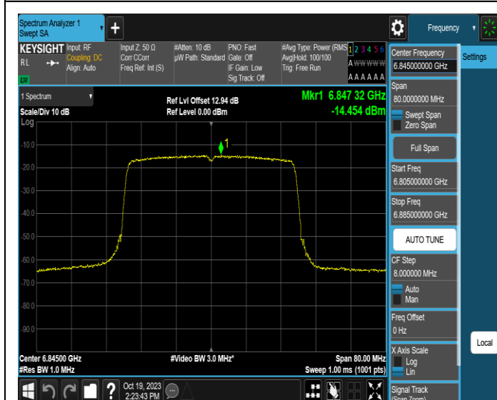
11AX40MIMO-Ant3-6845-PASS
