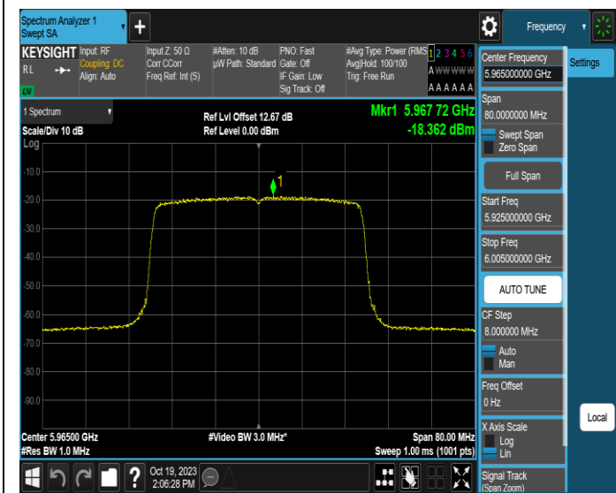
11AX40MIMO-Ant3-5965-PASS
