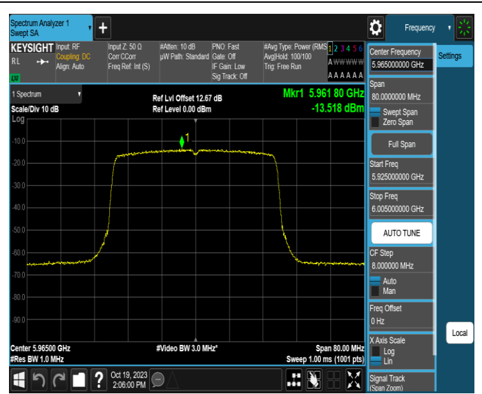
11AX40MIMO-Ant2-5965-PASS
