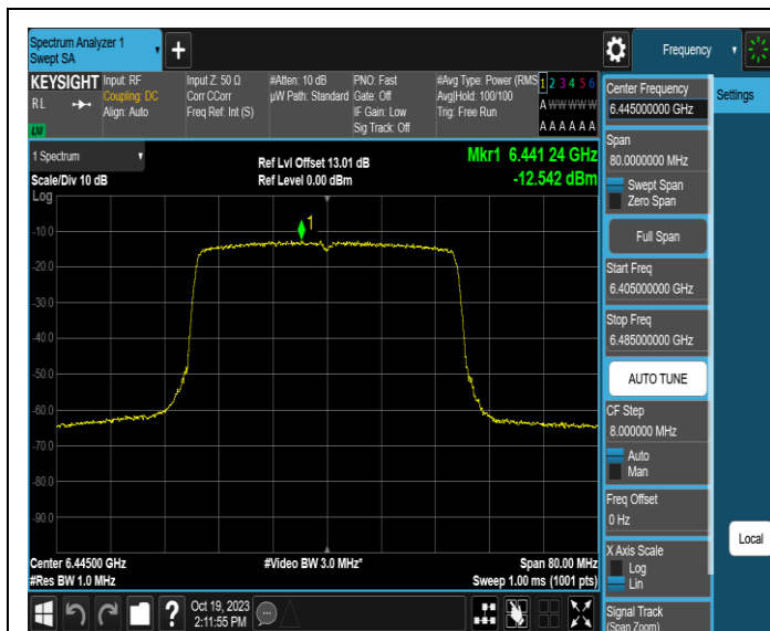
11AX40MIMO-Ant1-6445-PASS
