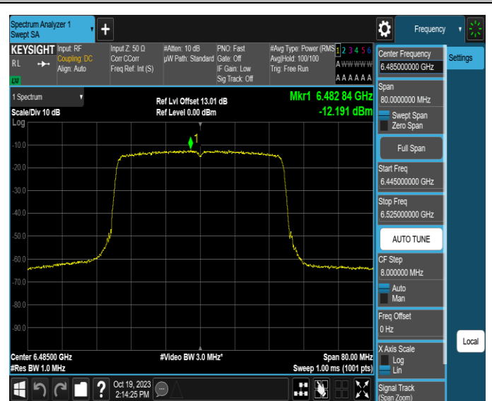
11AX40MIMO-Ant2-6485-PASS
