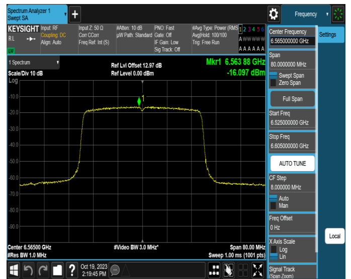
11AX40MIMO-Ant4-6565-PASS
