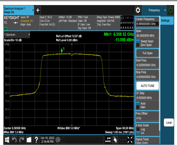
11AX40MIMO-Ant2-6565-PASS
