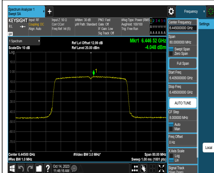
11AX40SISO-Ant3-6445-PASS
