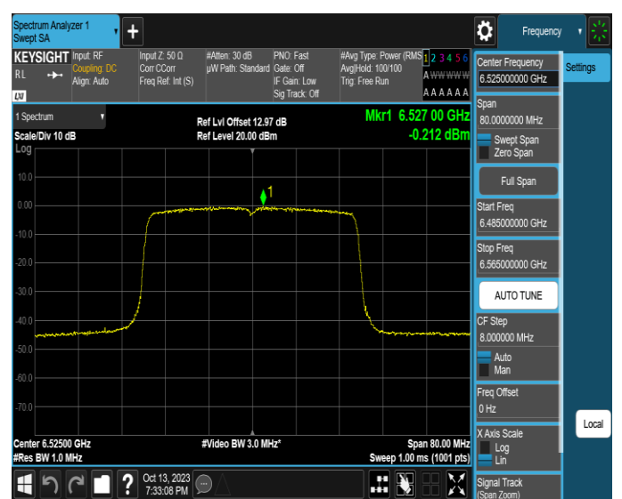
11AX40SISO-Ant2-6525-PASS
