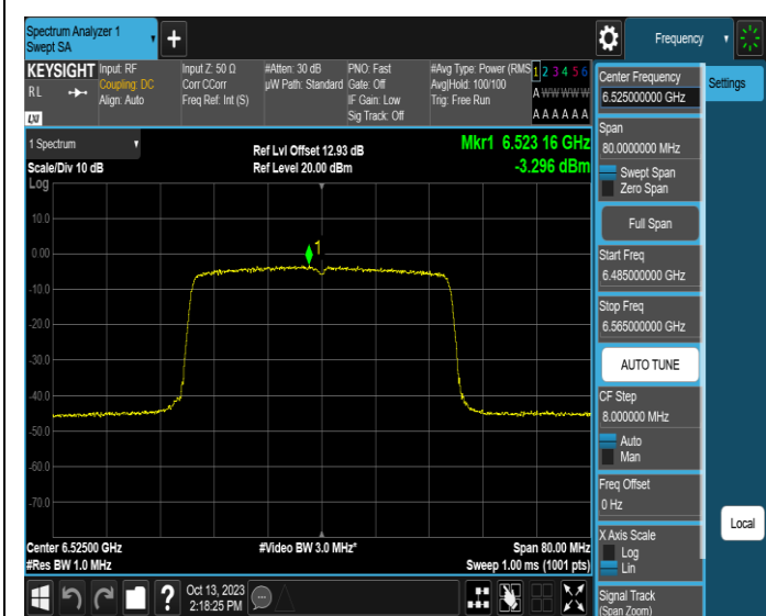
11AX40SISO-Ant1-6525-PASS
