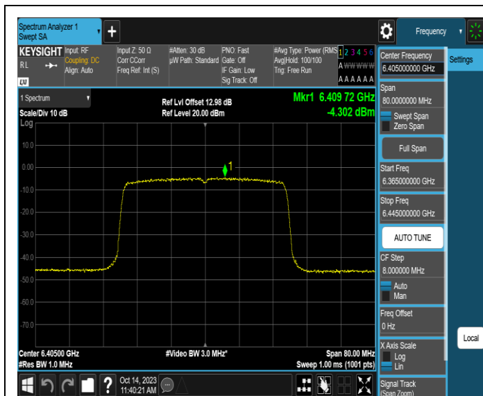
11AX40SISO-Ant3-6405-PASS
