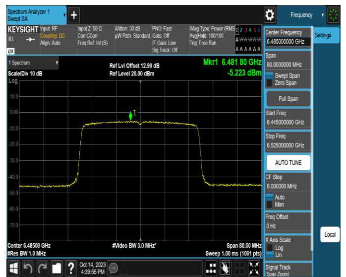
11AX40SISO-Ant4-6485-PASS
