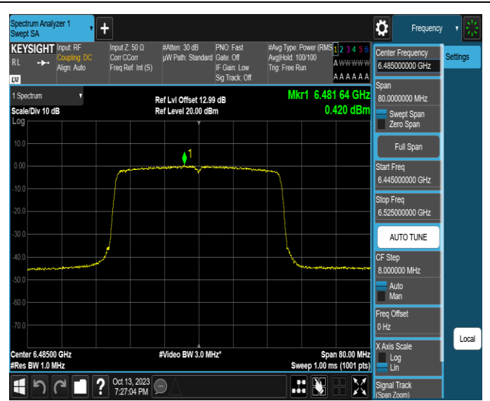
11AX40SISO-Ant2-6485-PASS
