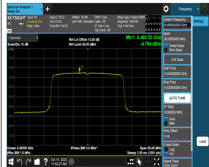
11AX40SISO-Ant3-6485-PASS
