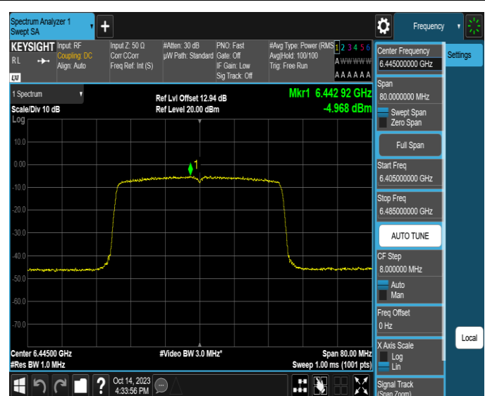
11AX40SISO-Ant4-6445-PASS
