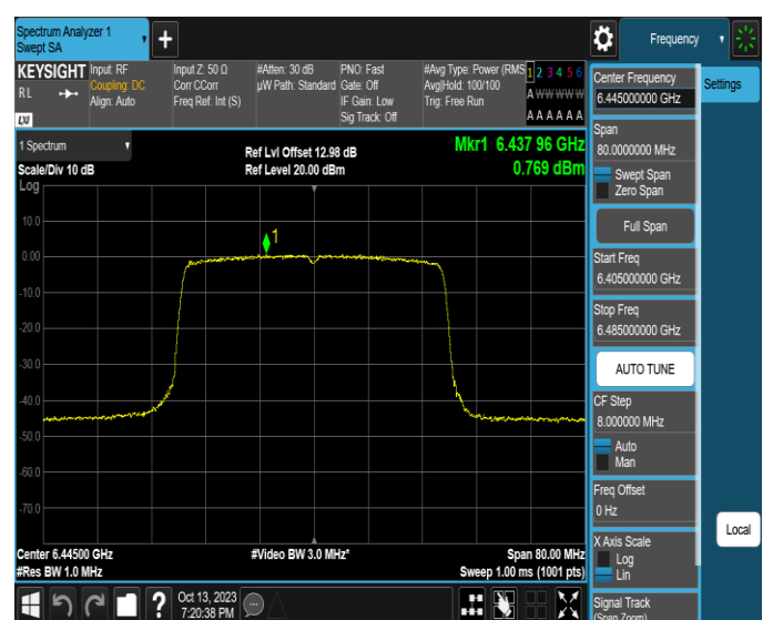
11AX40SISO-Ant2-6445-PASS
