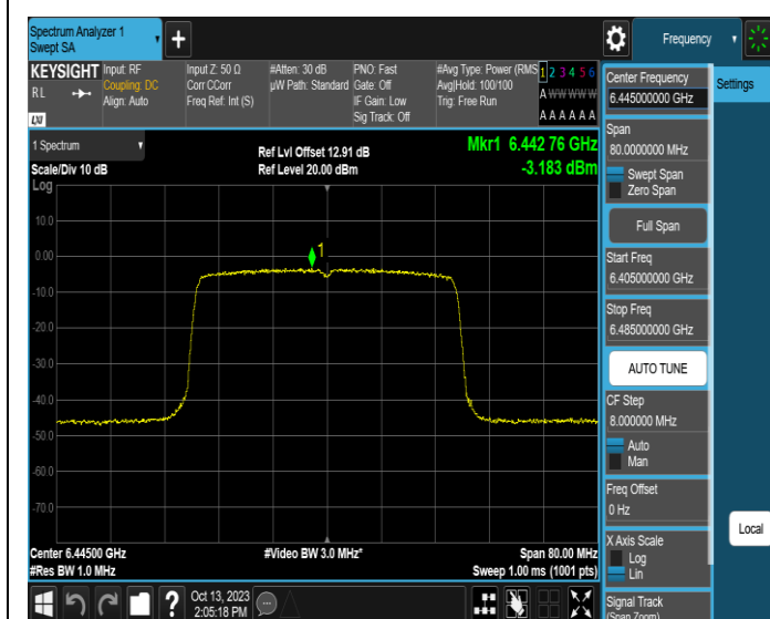
11AX40SISO-Ant1-6445-PASS
