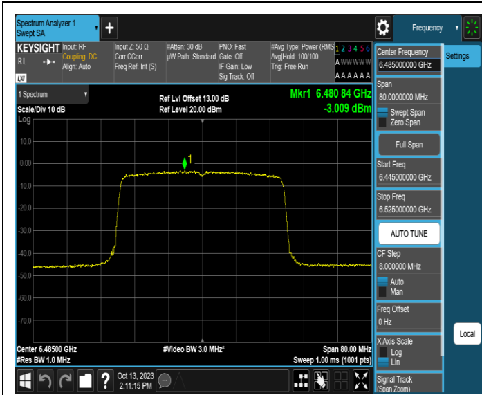
11AX40SISO-Ant1-6485-PASS
