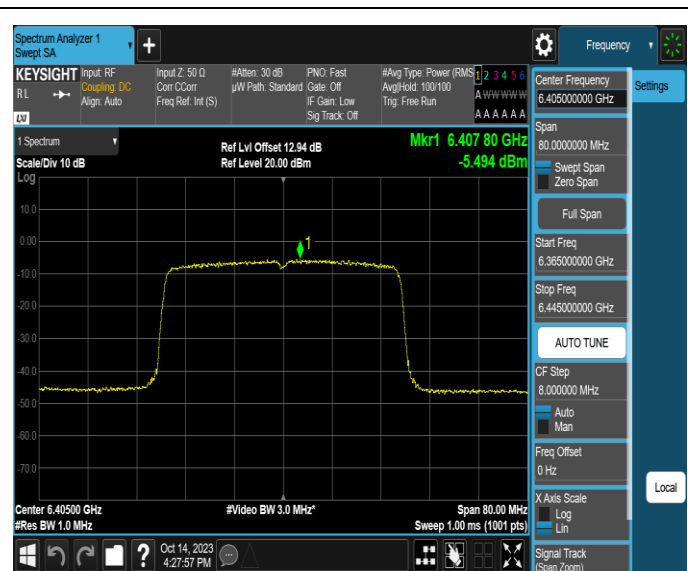
11AX40SISO-Ant4-6405-PASS
