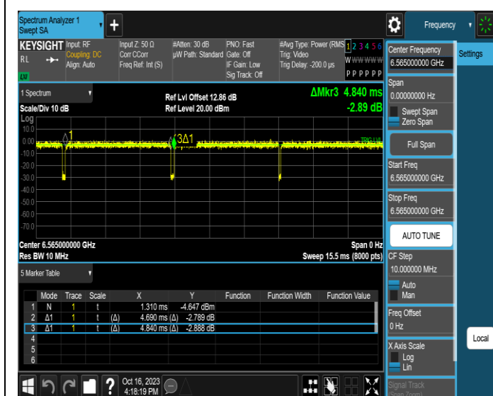
NTNV-11AX40MIMO-Ant3-6565
