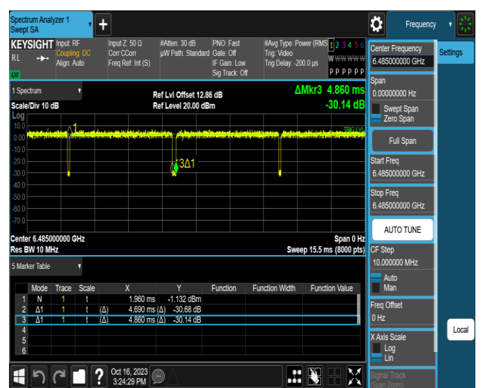
NTNV-11AX40MIMO-Ant2-6485
