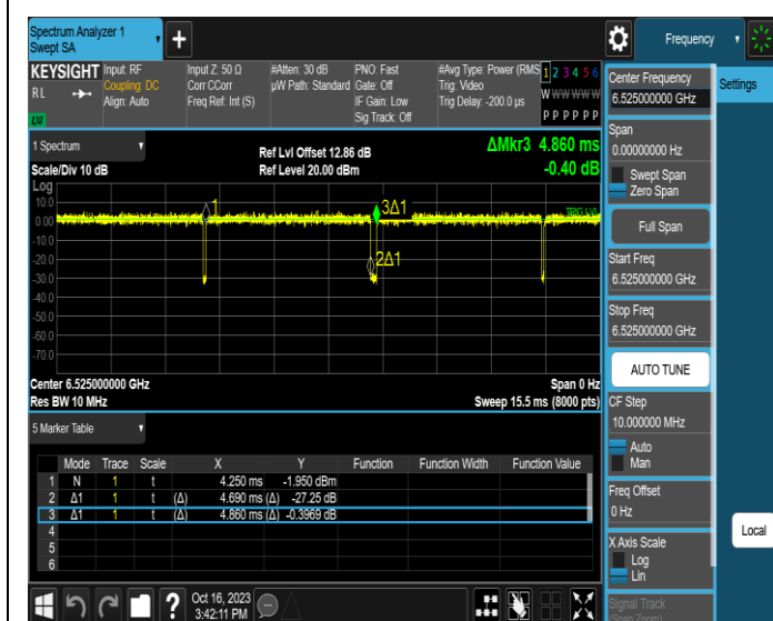
NTNV-11AX40MIMO-Ant3-6525
