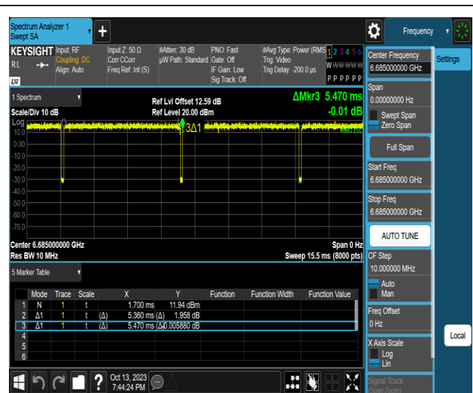
NTNV-11AX40SISO-Ant2-6685
