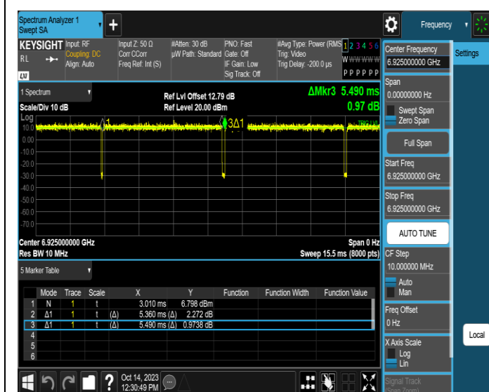
NTNV-11AX40SISO-Ant3-6925
