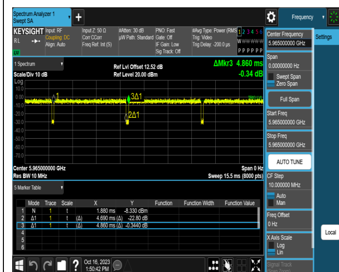
NTNV-11AX40MIMO-Ant3-5965
