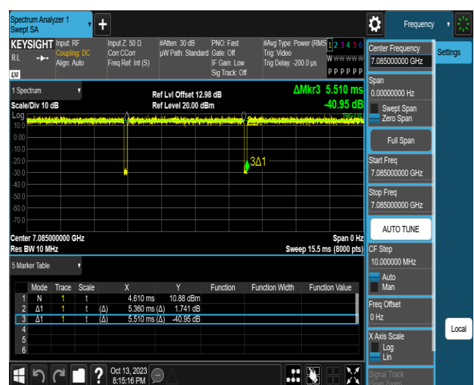
NTNV-11AX40SISO-Ant2-7085
