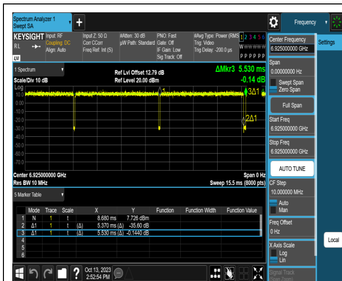
NTNV-11AX40SISO-Ant1-6925
