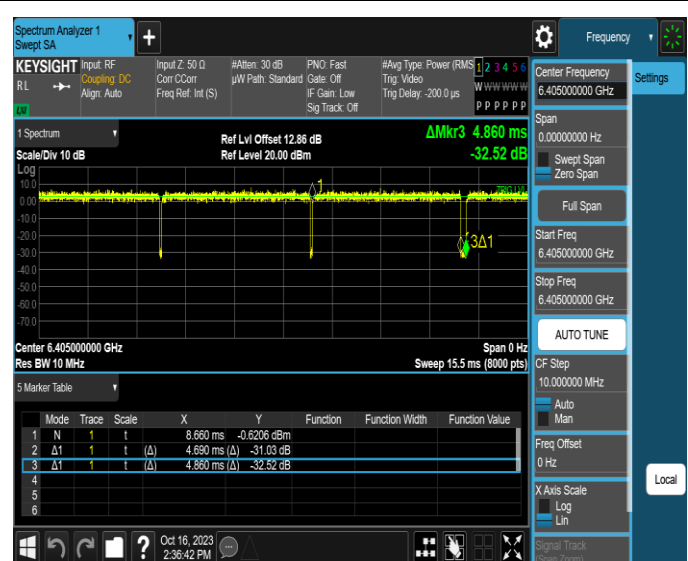
NTNV-11AX40MIMO-Ant2-6405
