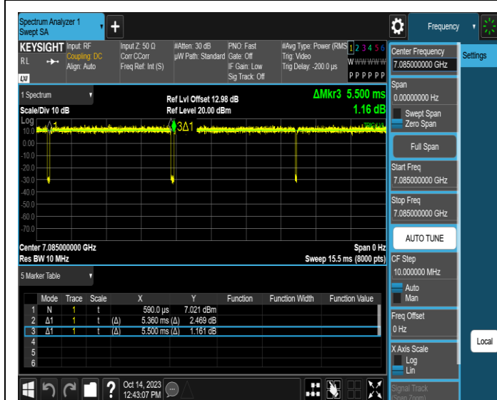
NTNV-11AX40SISO-Ant3-7085
