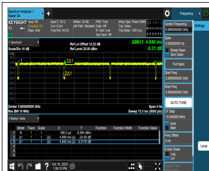
NTNV-11AX40MIMO-Ant1-5965
