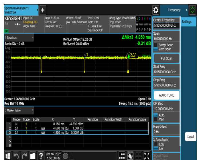
NTNV-11AX40MIMO-Ant4-5965
