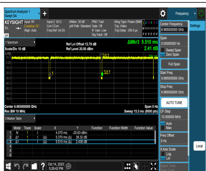
NTNV-11AX40SISO-Ant4-6965
