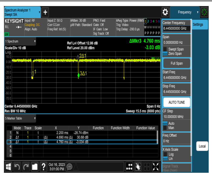
NTNV-11AX40MIMO-Ant2-6445
