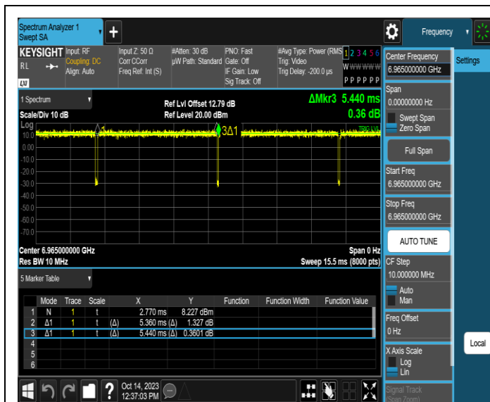
NTNV-11AX40SISO-Ant3-6965
