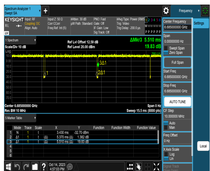
NTNV-11AX40SISO-Ant4-6685
