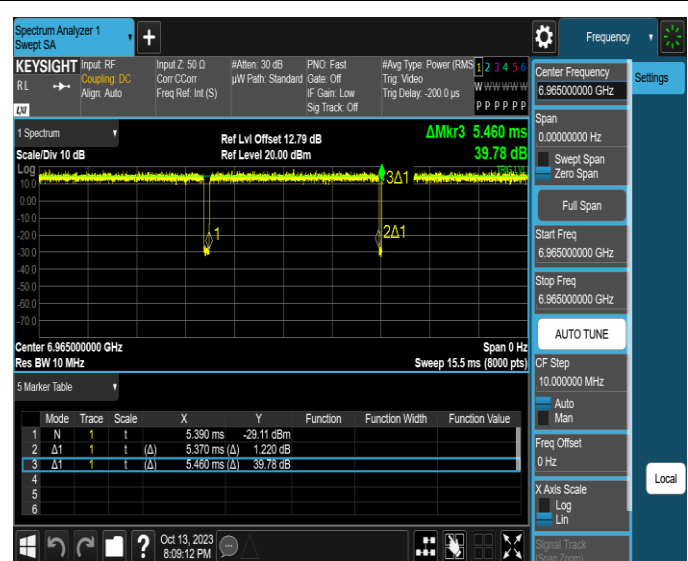
NTNV-11AX40SISO-Ant2-6965
