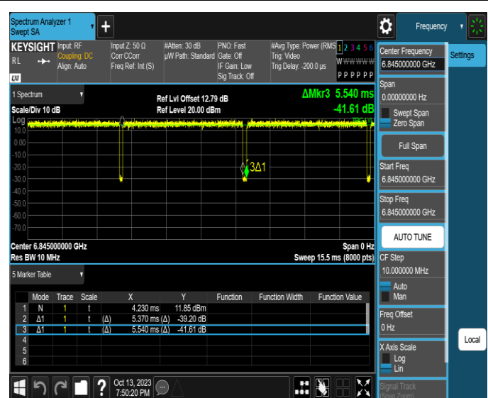
NTNV-11AX40SISO-Ant2-6845
