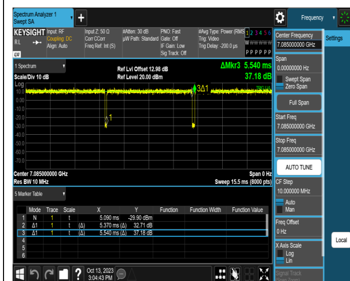
NTNV-11AX40SISO-Ant1-7085
