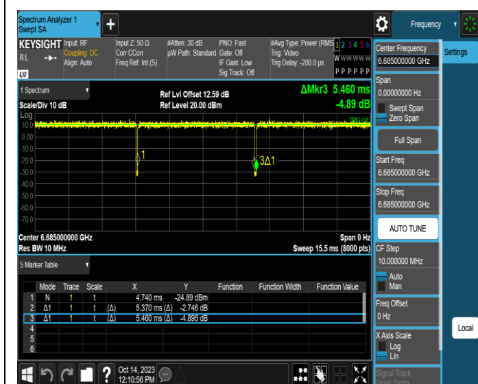
NTNV-11AX40SISO-Ant3-6685
