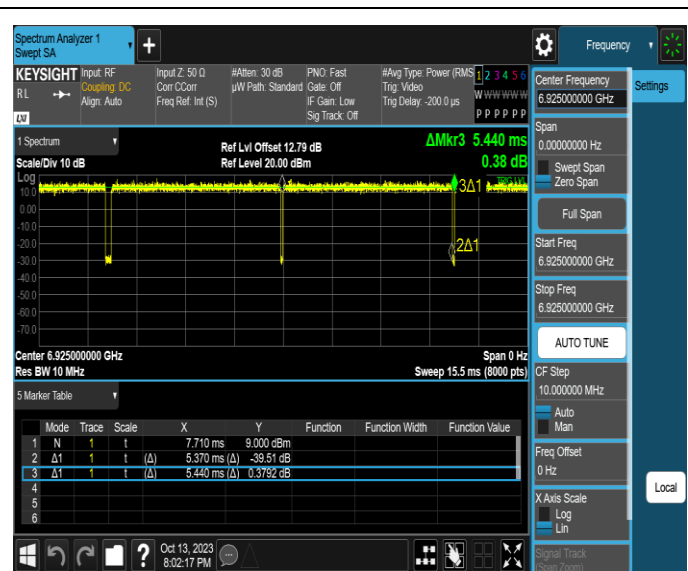
NTNV-11AX40SISO-Ant2-6925
