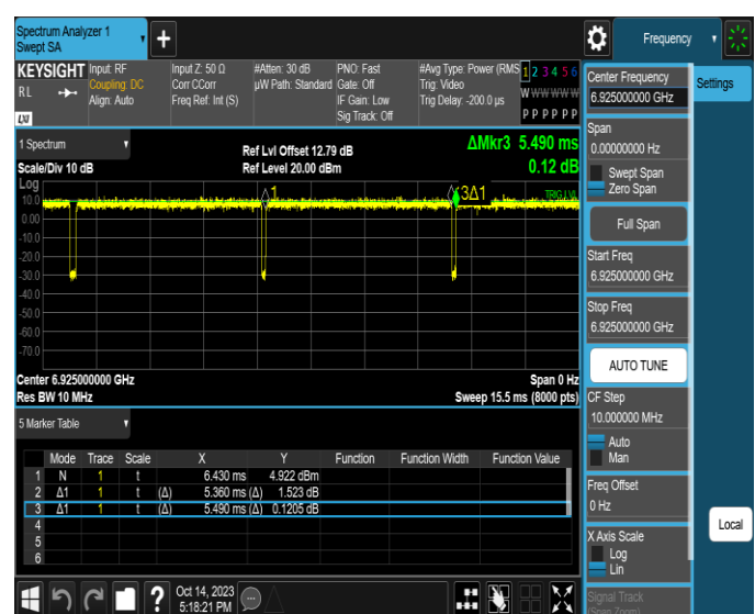
NTNV-11AX40SISO-Ant4-6925
