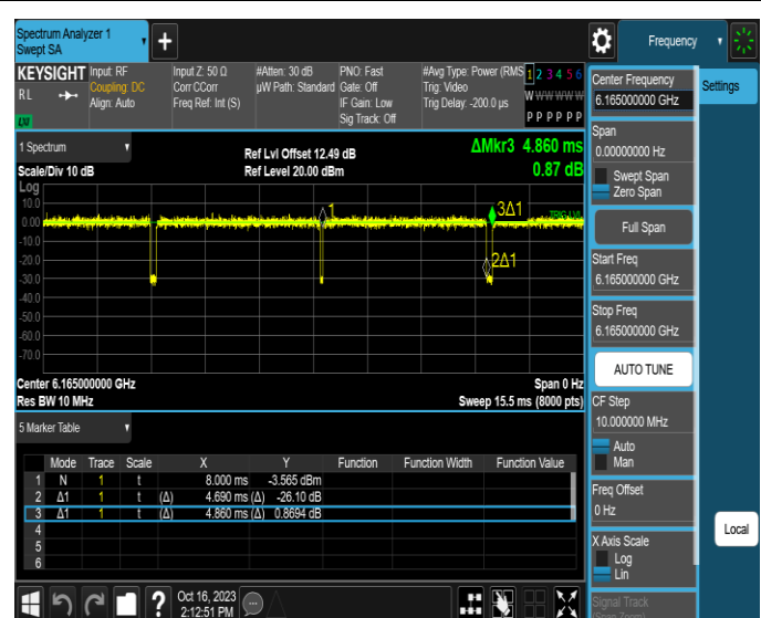
NTNV-11AX40MIMO-Ant2-6165
