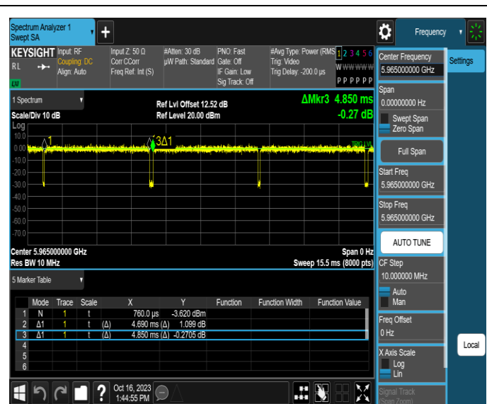
NTNV-11AX40MIMO-Ant2-5965
