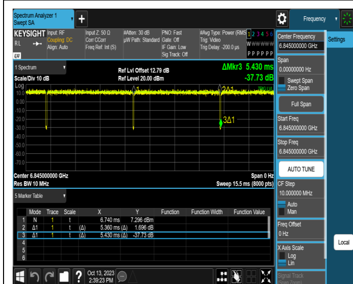
NTNV-11AX40SISO-Ant1-6845
