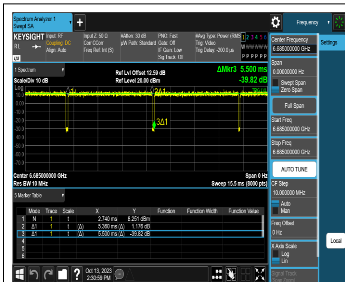
NTNV-11AX40SISO-Ant1-6685
