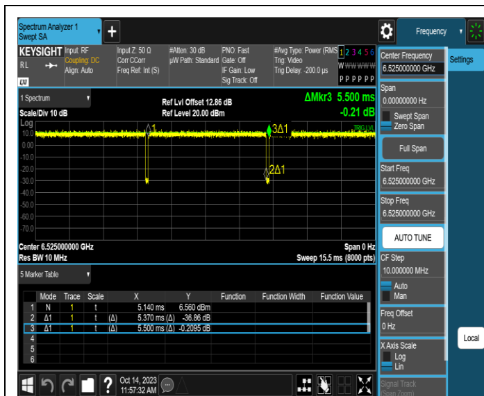
NTNV-11AX40SISO-Ant3-6525
