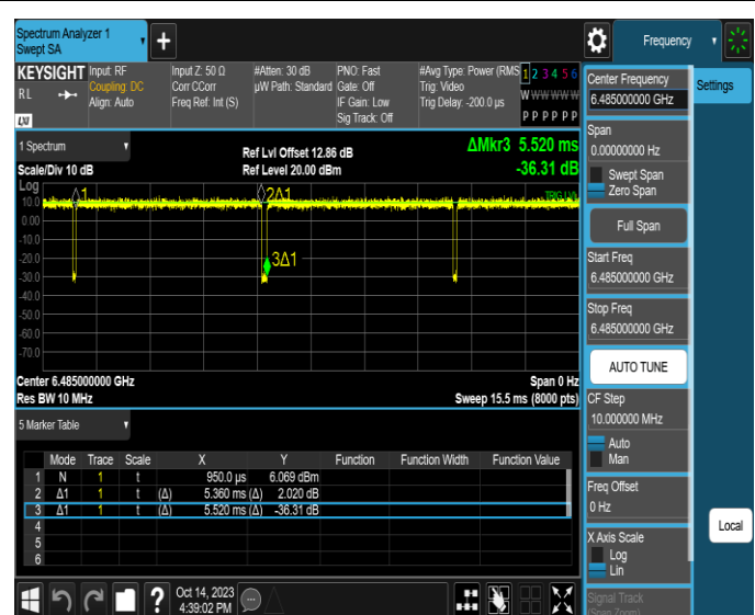
NTNV-11AX40SISO-Ant4-6485
