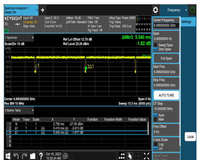
NTNV-11AX20MIMO-Ant2-6895
