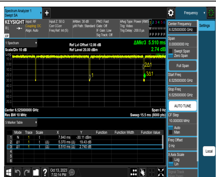
NTNV-11AX40SISO-Ant2-6525
