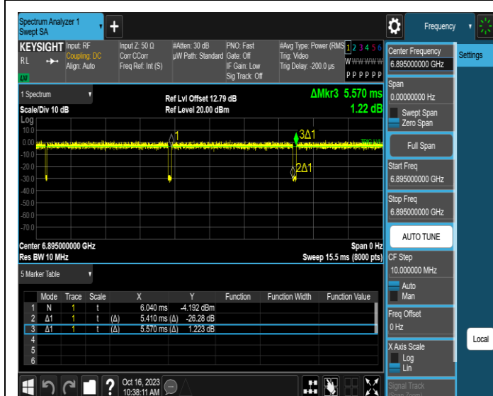
NTNV-11AX20MIMO-Ant3-6895
