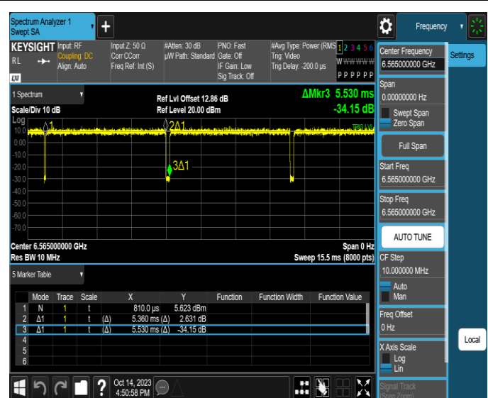
NTNV-11AX40SISO-Ant4-6565
