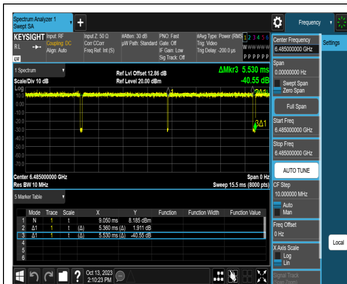
NTNV-11AX40SISO-Ant1-6485
