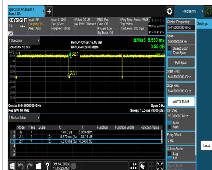
NTNV-11AX40SISO-Ant3-6445
