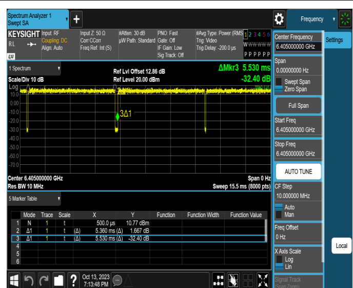
NTNV-11AX40SISO-Ant2-6405
