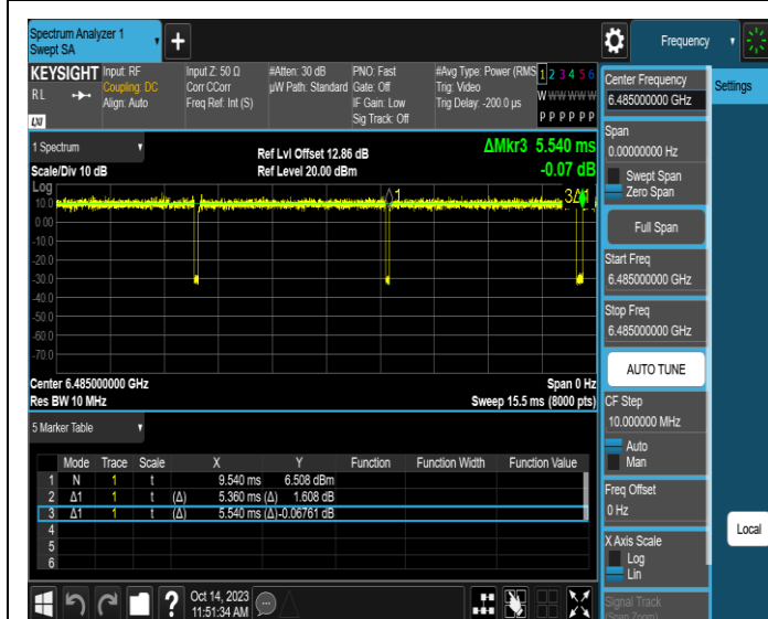
NTNV-11AX40SISO-Ant3-6485
