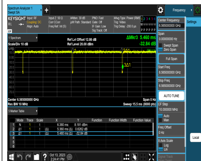
NTNV-11AX40SISO-Ant1-6565
