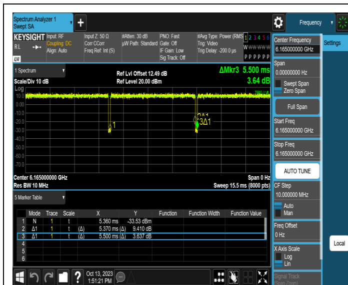
NTNV-11AX40SISO-Ant1-6165
