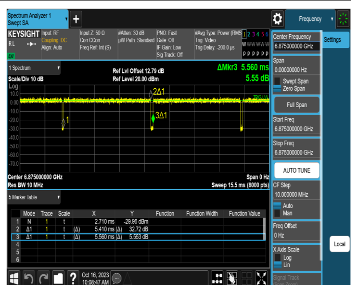
NTNV-11AX20MIMO-Ant2-6875
