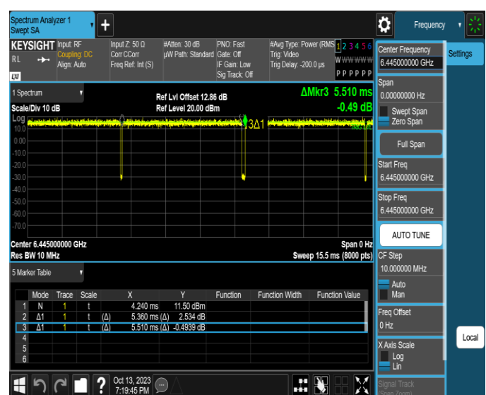
NTNV-11AX40SISO-Ant2-6445
