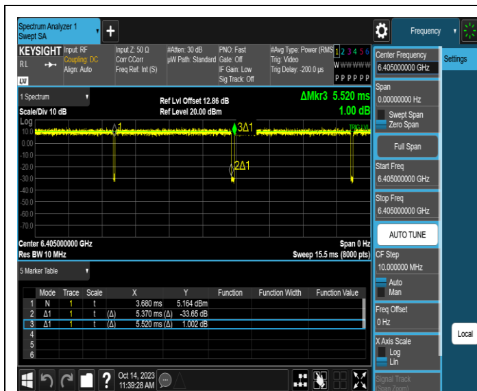
NTNV-11AX40SISO-Ant3-6405
