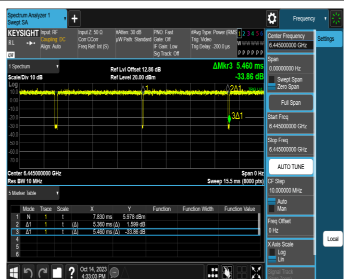
NTNV-11AX40SISO-Ant4-6445
