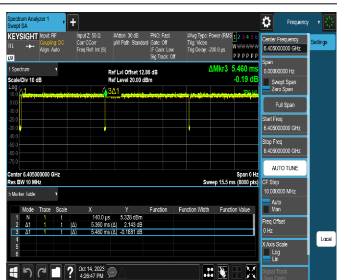
NTNV-11AX40SISO-Ant4-6405
