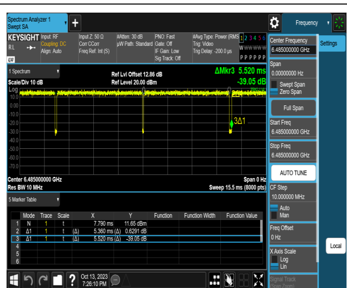
NTNV-11AX40SISO-Ant2-6485
