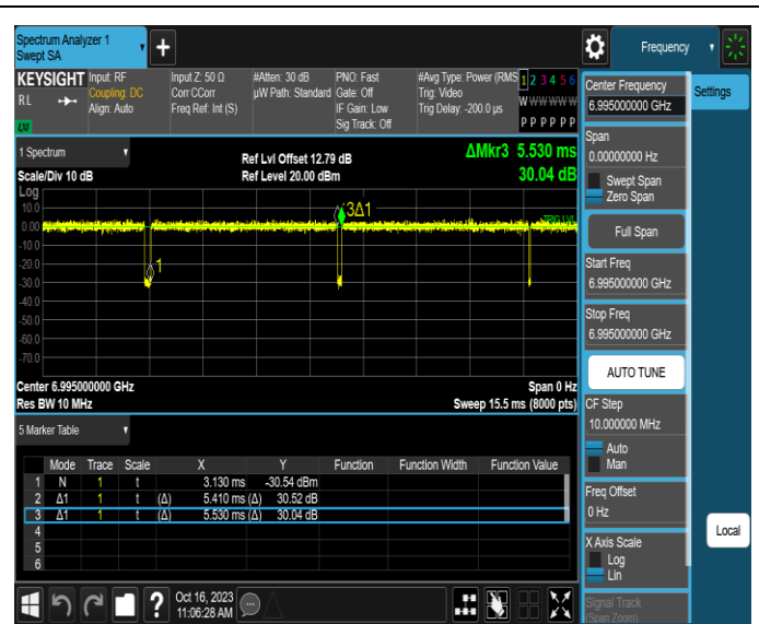
NTNV-11AX20MIMO-Ant2-6995
