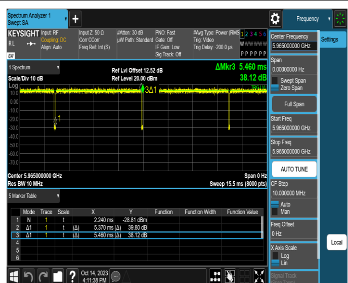
NTNV-11AX40SISO-Ant4-5965
