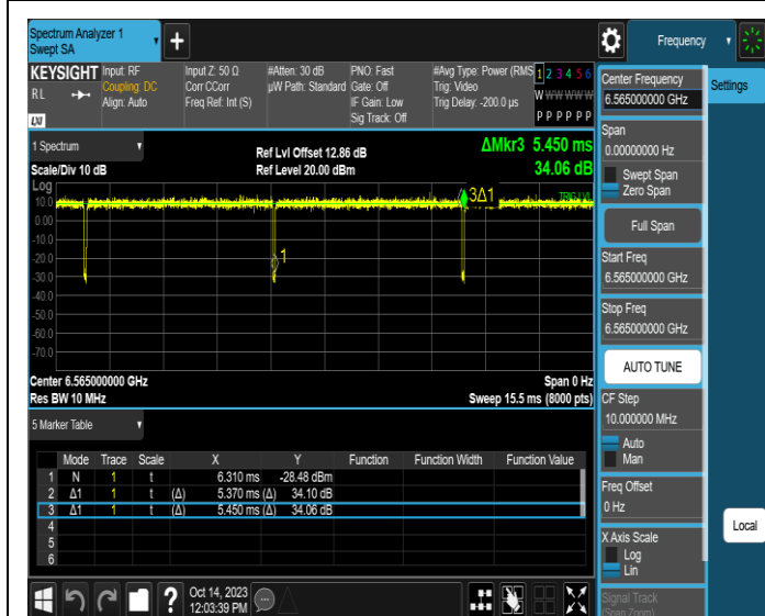
NTNV-11AX40SISO-Ant3-6565
