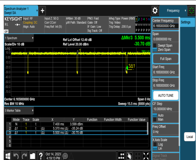
NTNV-11AX40SISO-Ant4-6165
