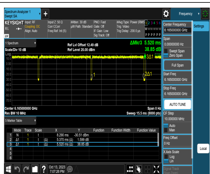
NTNV-11AX40SISO-Ant2-6165
