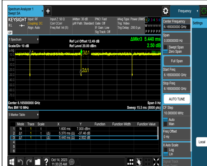
NTNV-11AX40SISO-Ant3-6165
