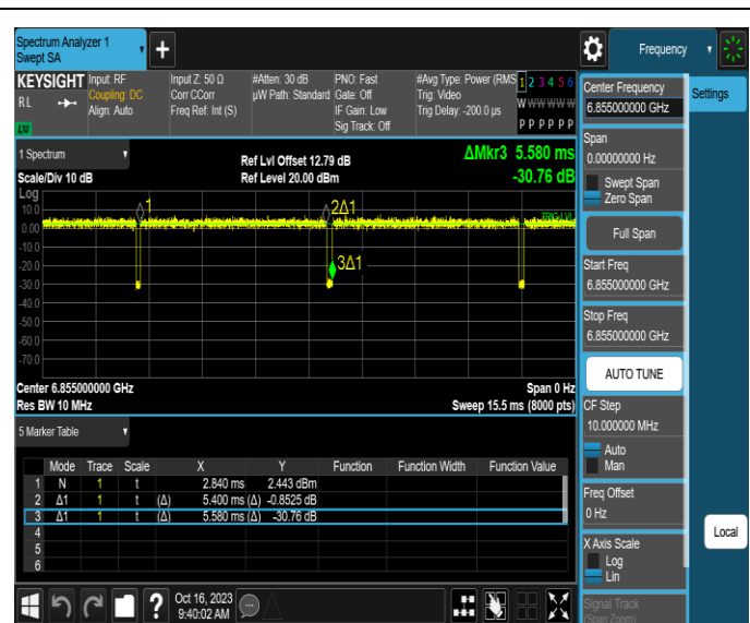
NTNV-11AX20MIMO-Ant2-6855
