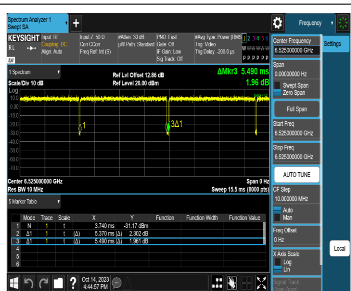
NTNV-11AX40SISO-Ant4-6525
