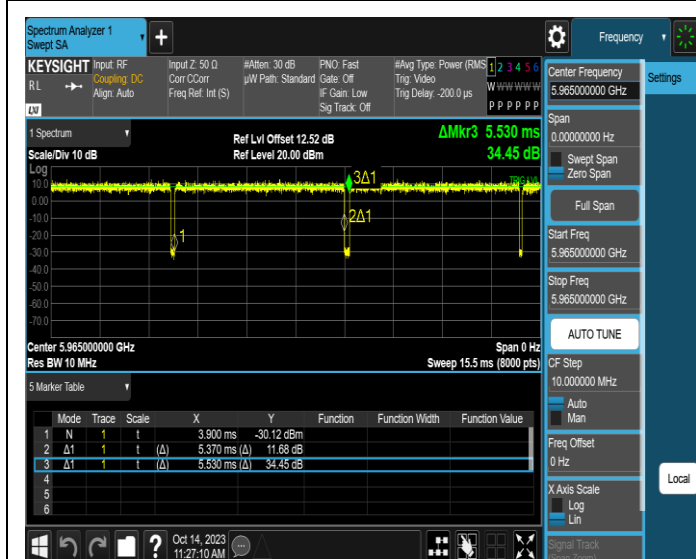
NTNV-11AX40SISO-Ant3-5965
