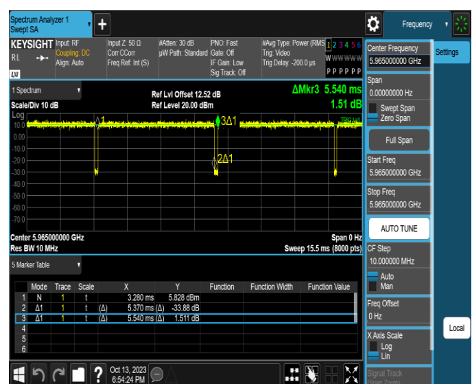
NTNV-11AX40SISO-Ant2-5965
