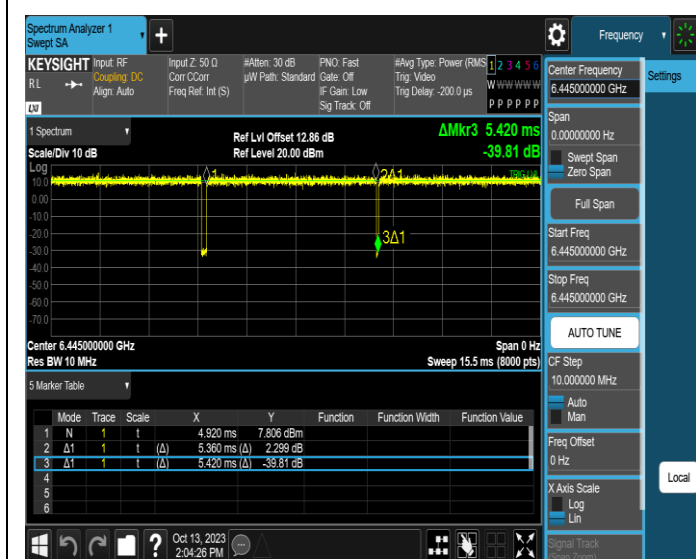
NTNV-11AX40SISO-Ant1-6445
