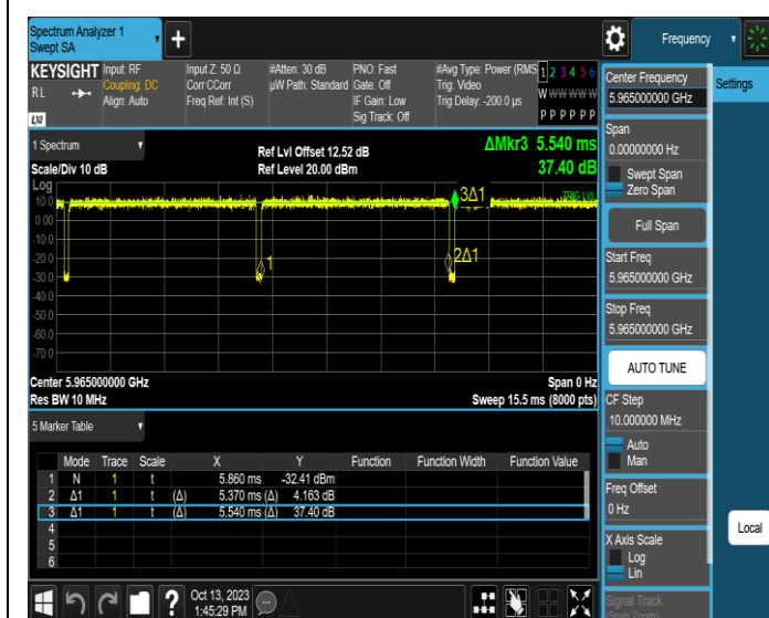
NTNV-11AX40SISO-Ant1-5965
