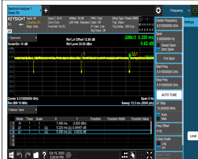
NTNV-11AX20MIMO-Ant3-6515
