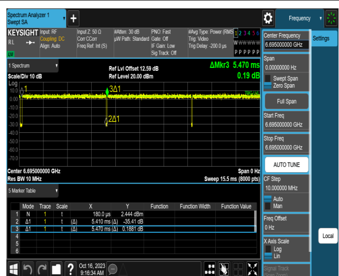
NTNV-11AX20MIMO-Ant2-6695
