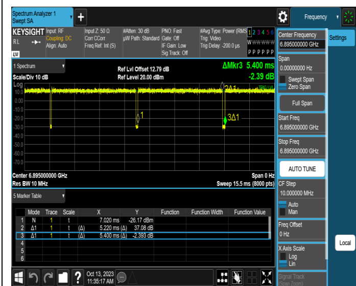
NTNV-11AX20SISO-Ant1-6895
