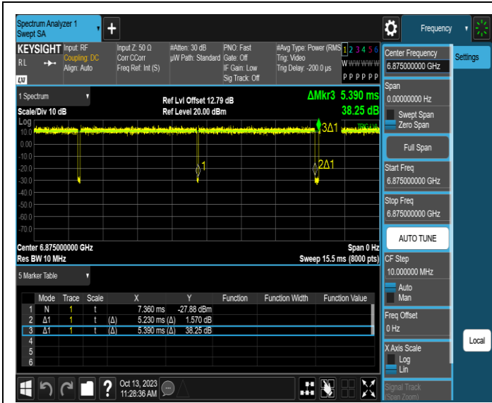
NTNV-11AX20SISO-Ant1-6875
