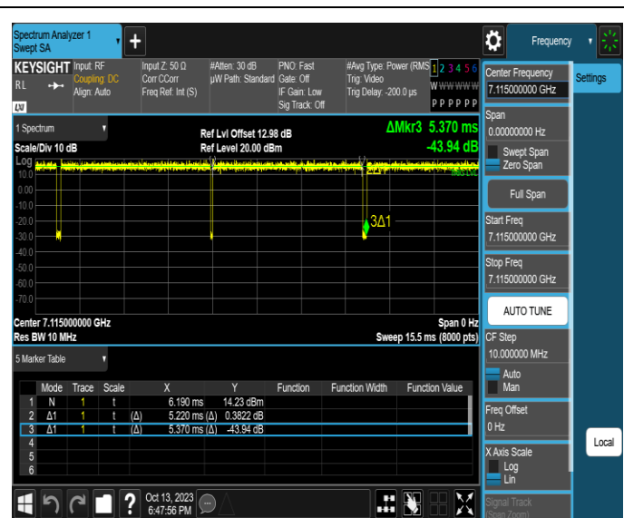
NTNV-11AX20SISO-Ant2-7115
