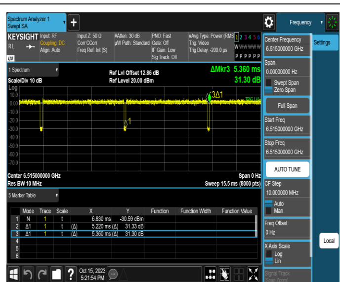
NTNV-11AX20MIMO-Ant2-6515
