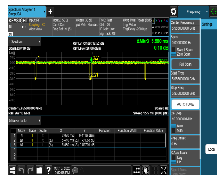
NTNV-11AX20MIMO-Ant1-5955
