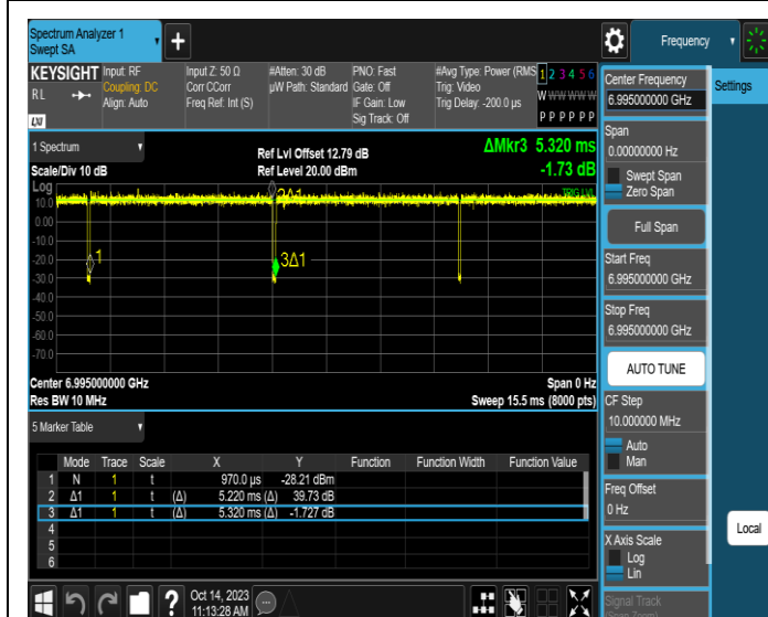
NTNV-11AX20SISO-Ant3-6995
