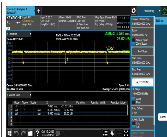
NTNV-11AX20MIMO-Ant3-5955
