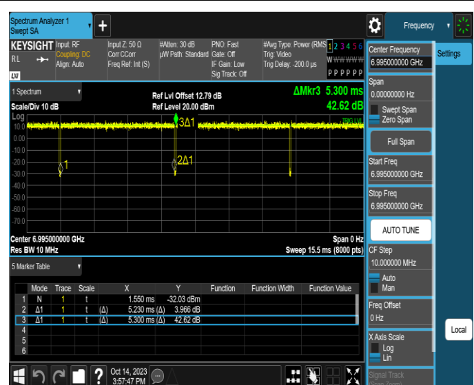
NTNV-11AX20SISO-Ant4-6995
