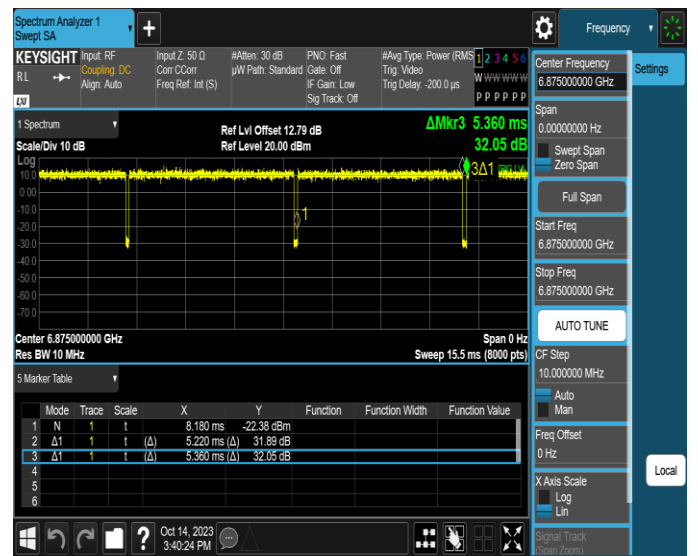
NTNV-11AX20SISO-Ant4-6875
