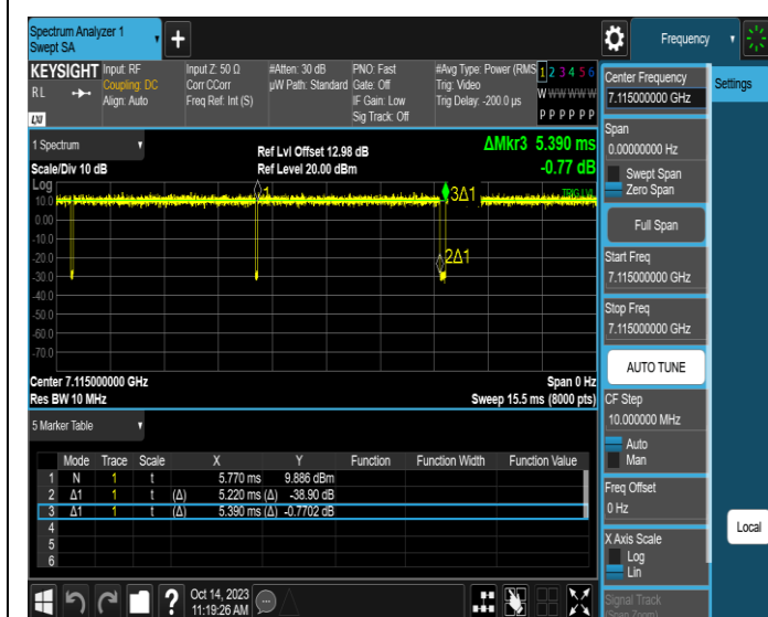
NTNV-11AX20SISO-Ant3-7115
