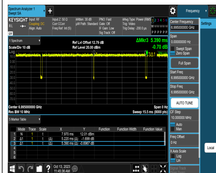
NTNV-11AX20SISO-Ant1-6995
