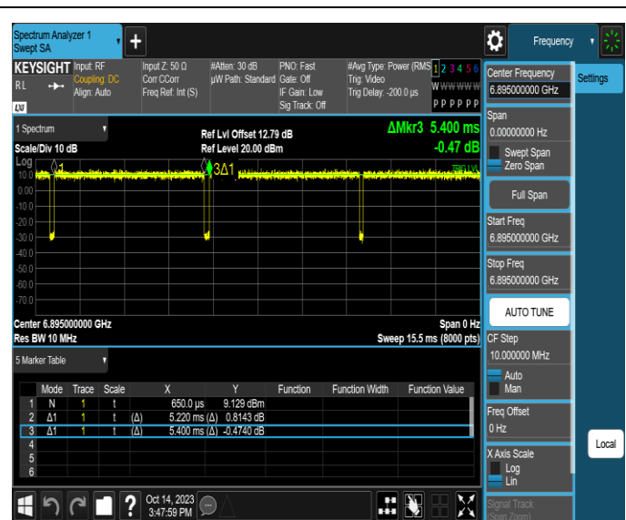
NTNV-11AX20SISO-Ant4-6895
