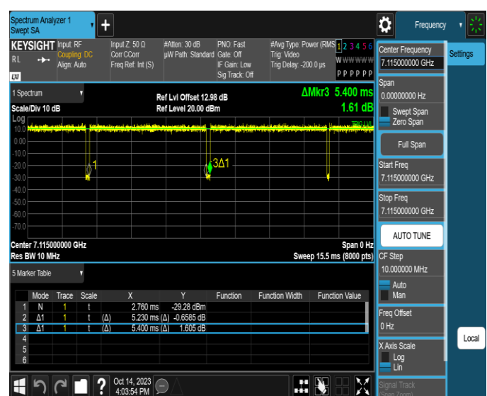
NTNV-11AX20SISO-Ant4-7115
