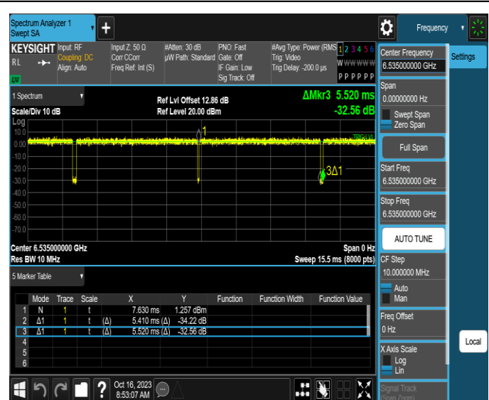
NTNV-11AX20MIMO-Ant2-6535
