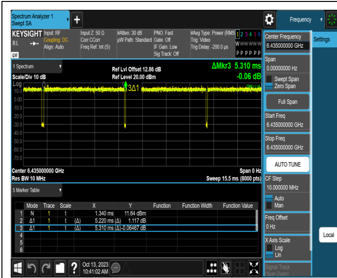
NTNV-11AX20SISO-Ant1-6435
