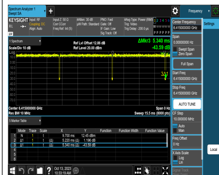
NTNV-11AX20SISO-Ant1-6415
