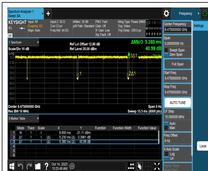
NTNV-11AX20SISO-Ant3-6475
