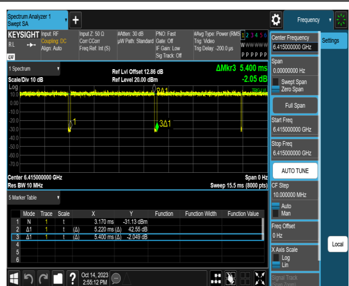
NTNV-11AX20SISO-Ant4-6415
