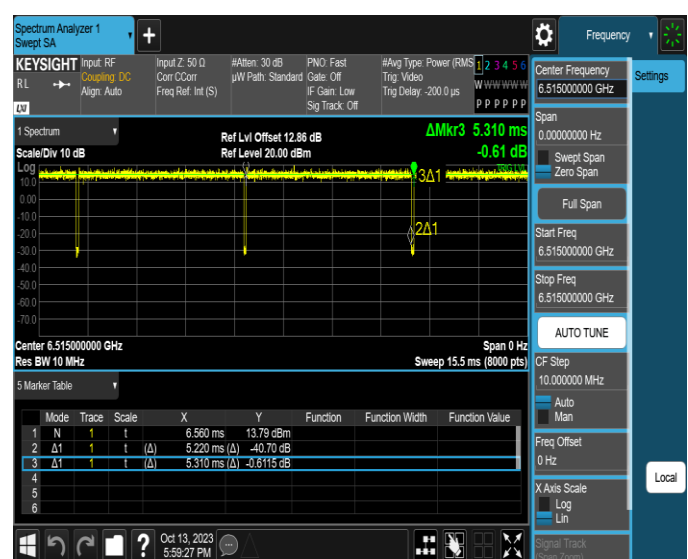
NTNV-11AX20SISO-Ant2-6515
