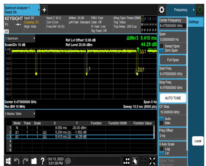
NTNV-11AX20SISO-Ant2-6475
