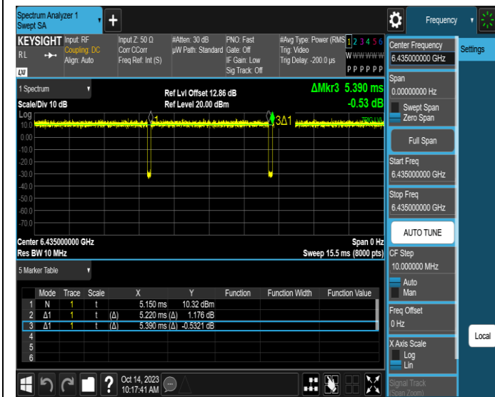
NTNV-11AX20SISO-Ant3-6435
