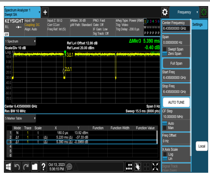
NTNV-11AX20SISO-Ant2-6435
