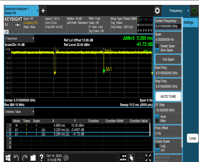
NTNV-11AX20SISO-Ant4-6515
