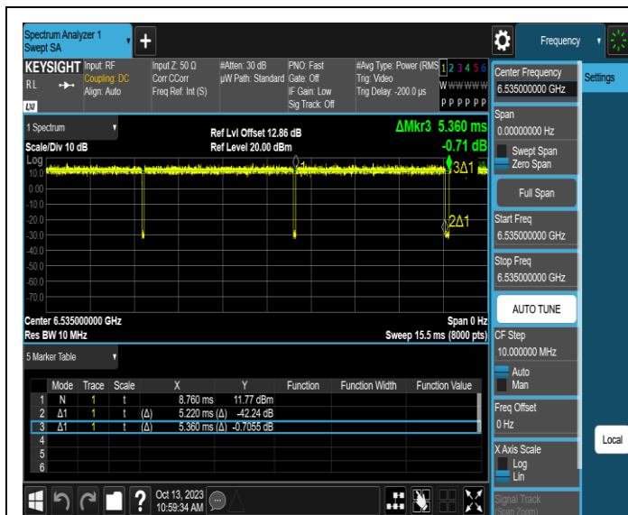
NTNV-11AX20SISO-Ant1-6535
