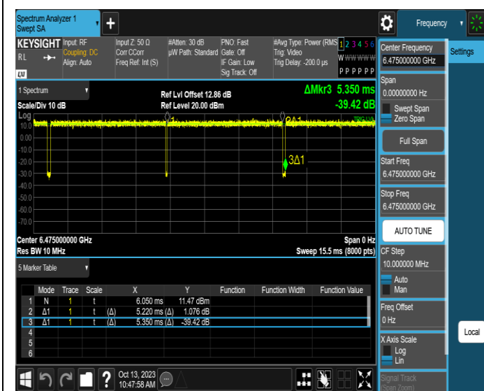
NTNV-11AX20SISO-Ant1-6475
