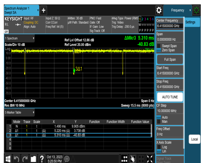
NTNV-11AX20SISO-Ant2-6415
