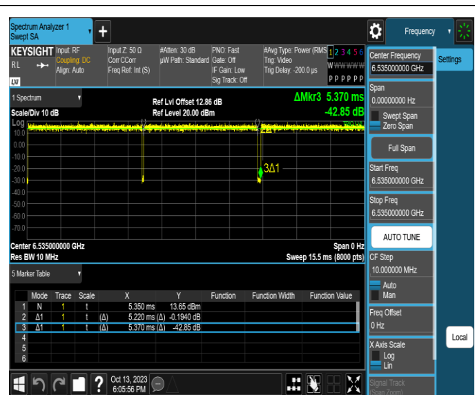
NTNV-11AX20SISO-Ant2-6535
