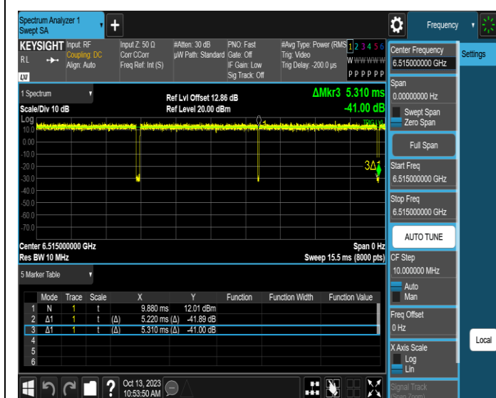
NTNV-11AX20SISO-Ant1-6515
