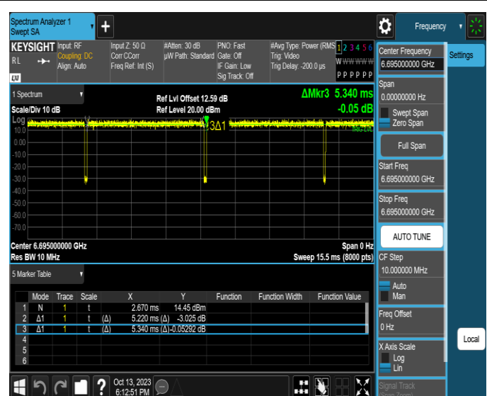
NTNV-11AX20SISO-Ant2-6695
