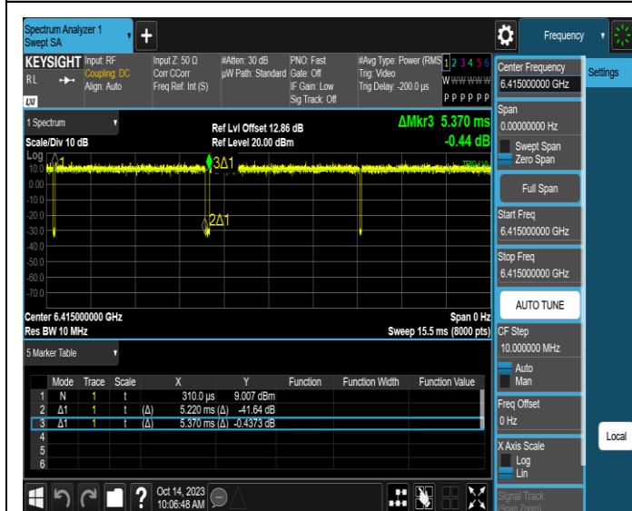
NTNV-11AX20SISO-Ant3-6415
