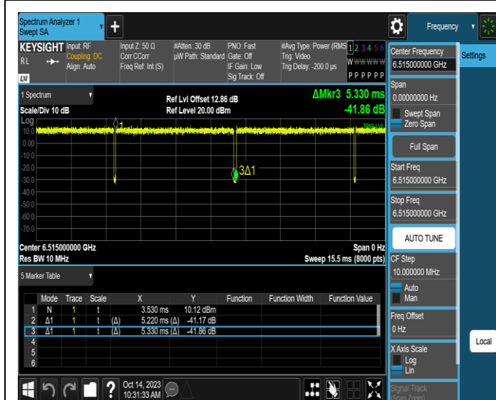
NTNV-11AX20SISO-Ant3-6515
