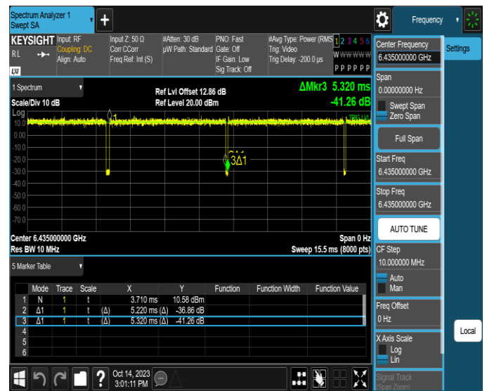
NTNV-11AX20SISO-Ant4-6435
