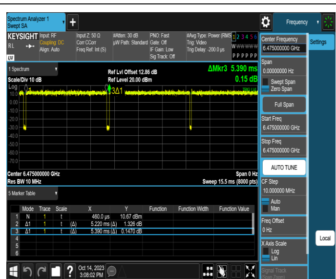
NTNV-11AX20SISO-Ant4-6475
