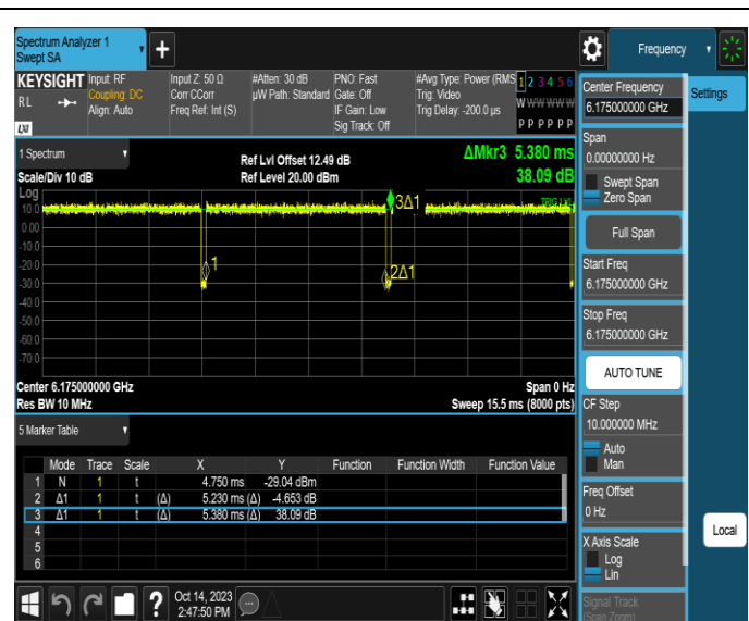
NTNV-11AX20SISO-Ant4-6175
