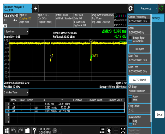
NTNV-11AX20SISO-Ant4-6535
