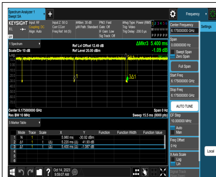
NTNV-11AX20SISO-Ant3-6175
