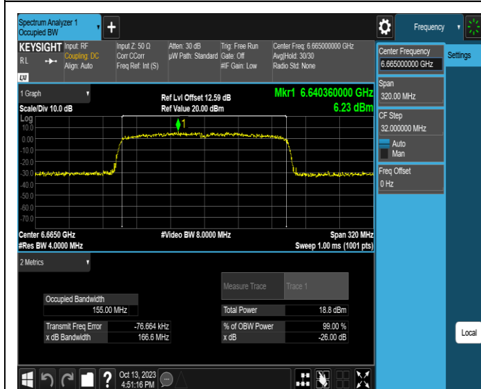
11AX160SISO-Ant1-6665
