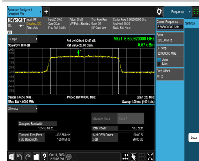
11AX160SISO-Ant3-6665
