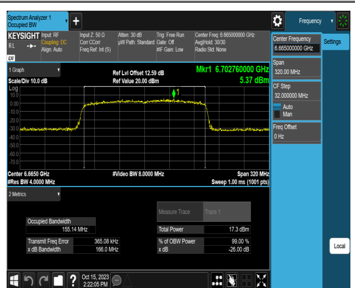
11AX160SISO-Ant4-6665
