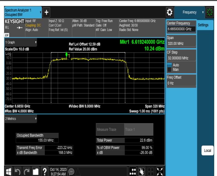
11AX160SISO-Ant2-6665
