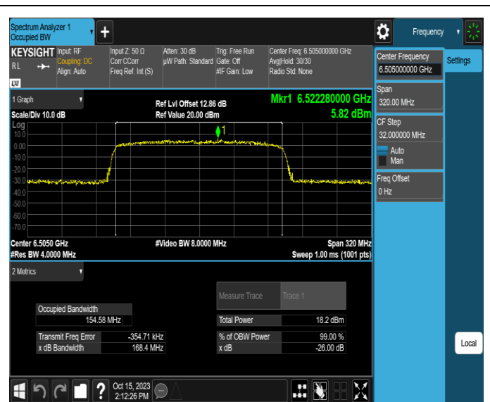
11AX160SISO-Ant4-6505
