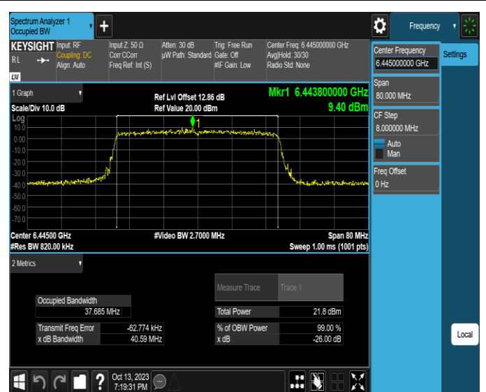
11AX40SISO-Ant2-6445
