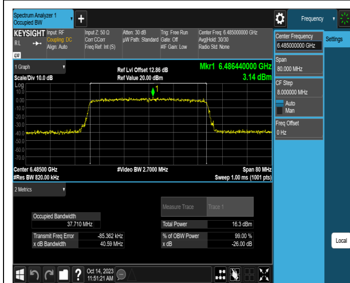
11AX40SISO-Ant3-6485
