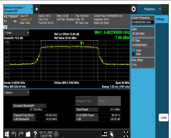
11AX40SISO-Ant2-6485
