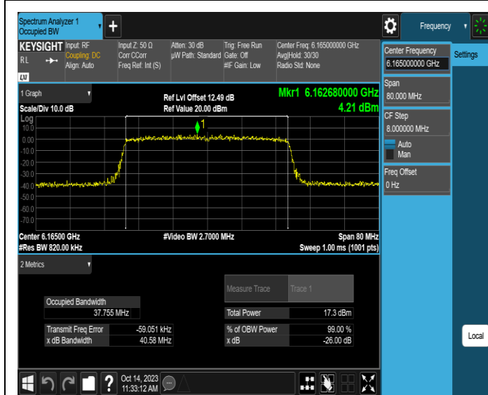
11AX40SISO-Ant3-6165
