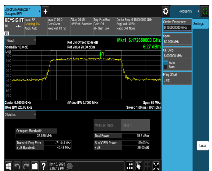
11AX40SISO-Ant2-6165
