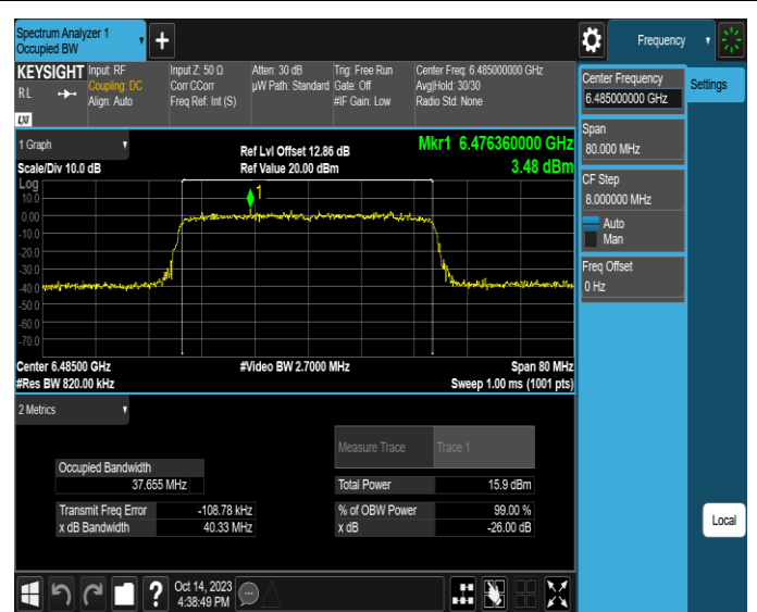
11AX40SISO-Ant4-6485
