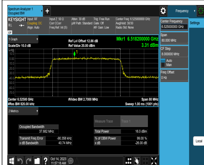
11AX40ISO-Ant3-6525
