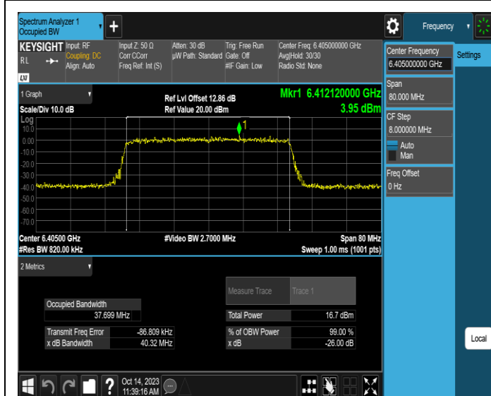
11AX40SISO-Ant3-6405
