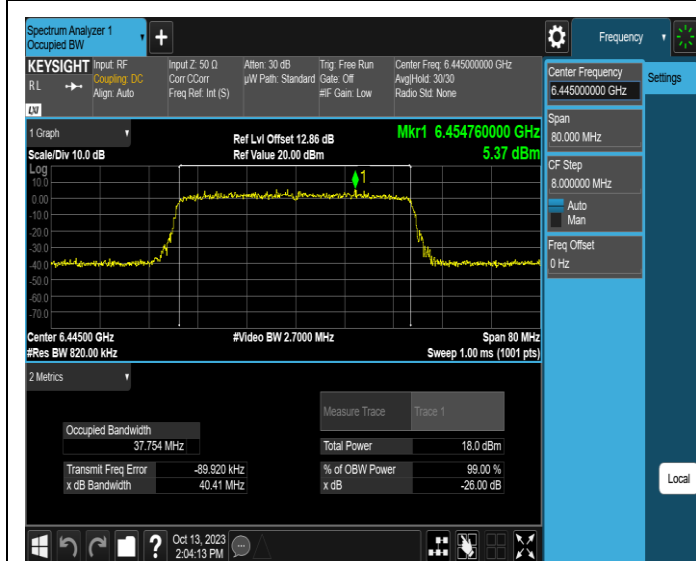
11AX40SISO-Ant1-6445
