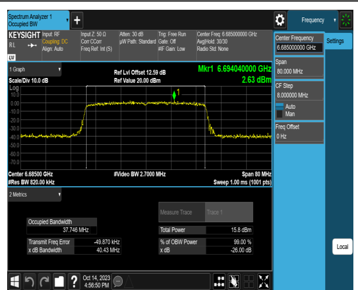
11AX40SISO-Ant4-6685
