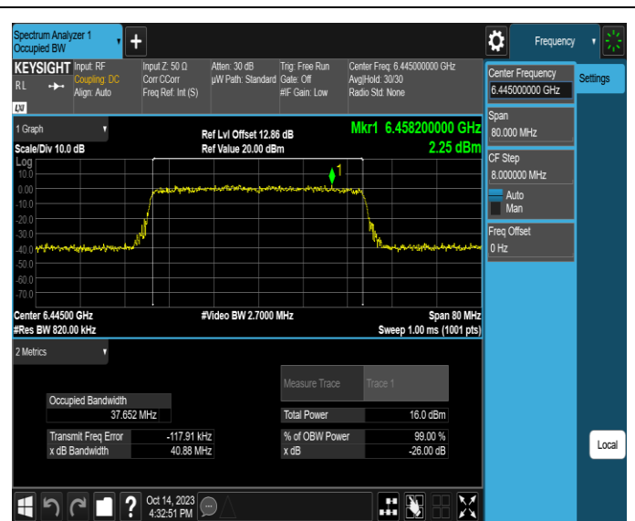
11AX40SISO-Ant4-6445
