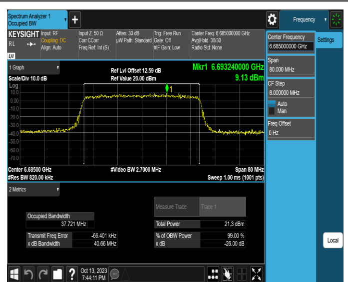
11AX40SISO-Ant2-6685
