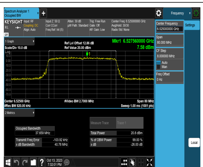
11AX40ISO-Ant2-6525
