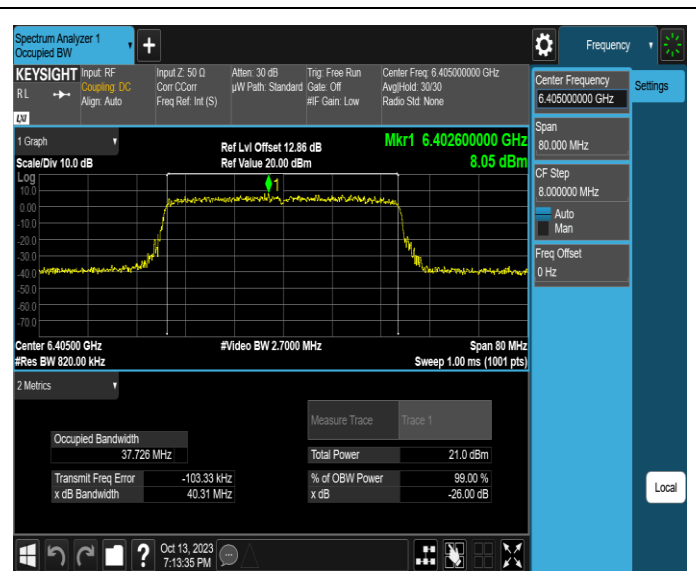
11AX40SISO-Ant2-6405
