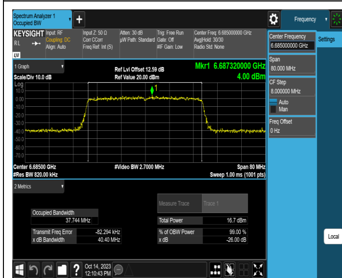
11AX40SISO-Ant3-6685
