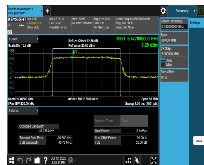
11AX40SISO-Ant1-6485
