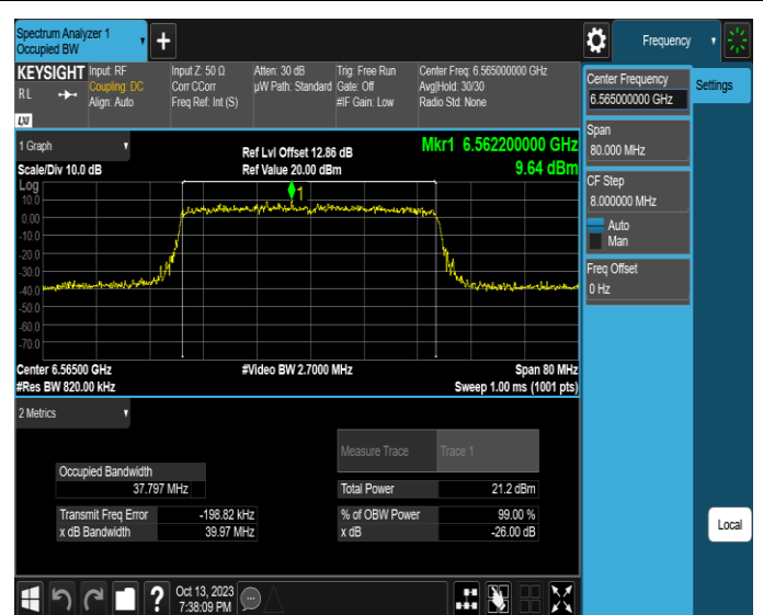
11AX40ISO-Ant2-6565
