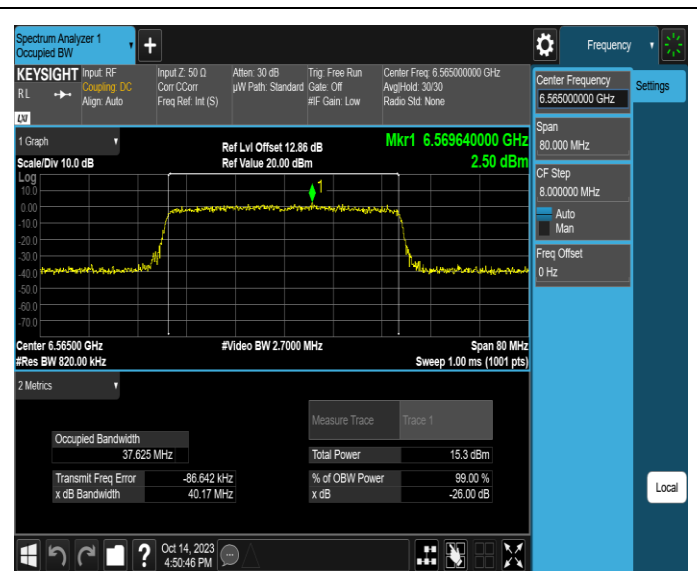
11AX40SISO-Ant4-6565
