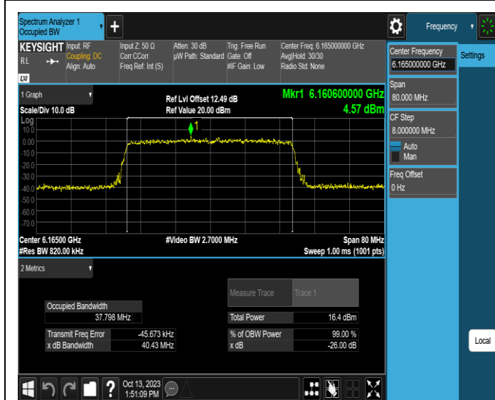
11AX40SISO-Ant1-6165
