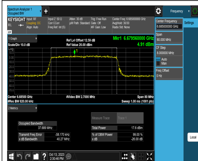
11AX40SISO-Ant1-6685
