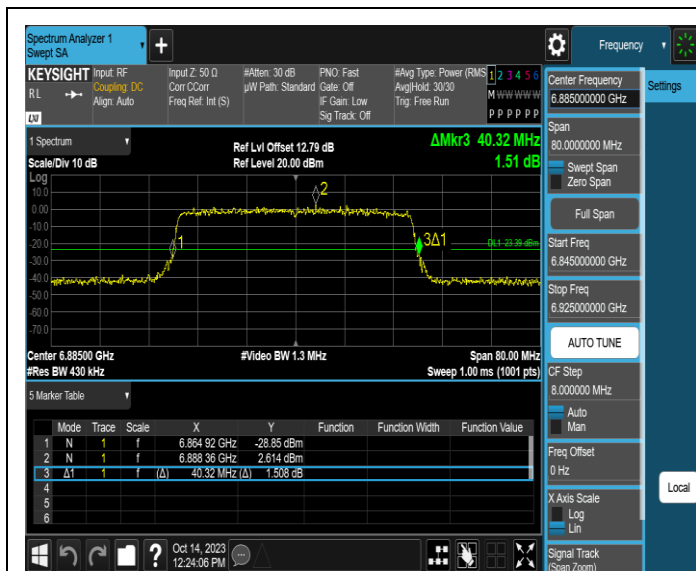
11AX40SISO-Ant3-6885
