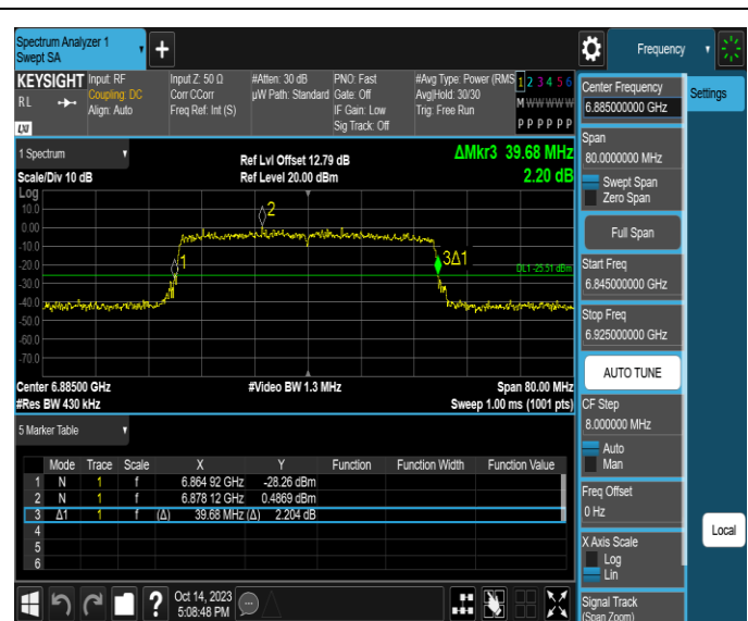
11AX40SISO-Ant4-6885
