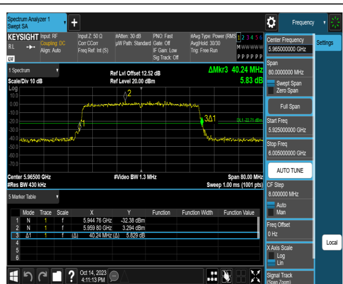
11AX40SISO-Ant4-5965
