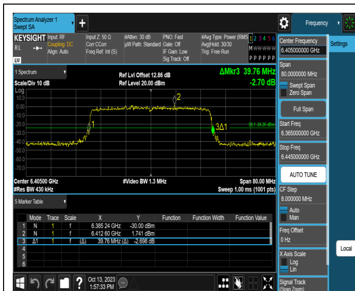
11AX40SISO-Ant1-6405
