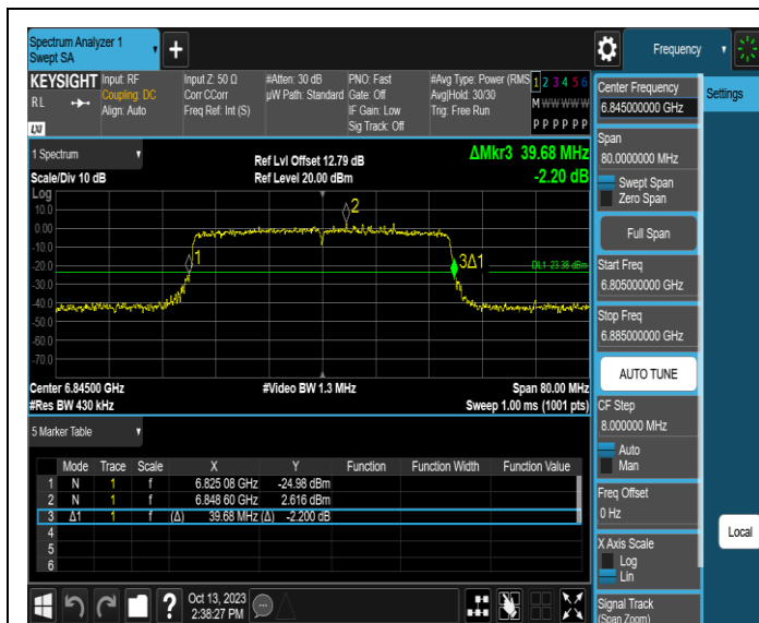
11AX40SISO-Ant1-6845
