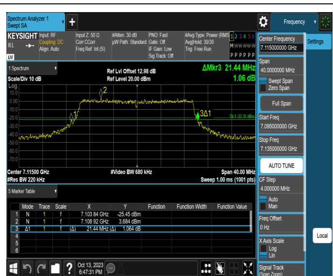
11AX20SISO-Ant2-7115
