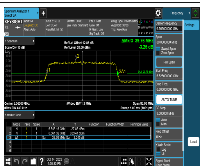
11AX40SISO-Ant4-6565
