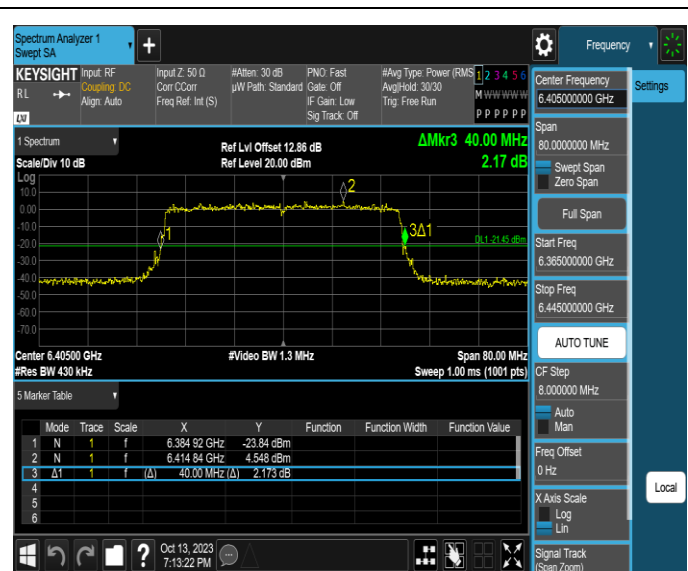
11AX40SISO-Ant2-6405
