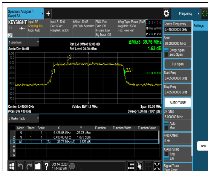
11AX40SISO-Ant3-6445
