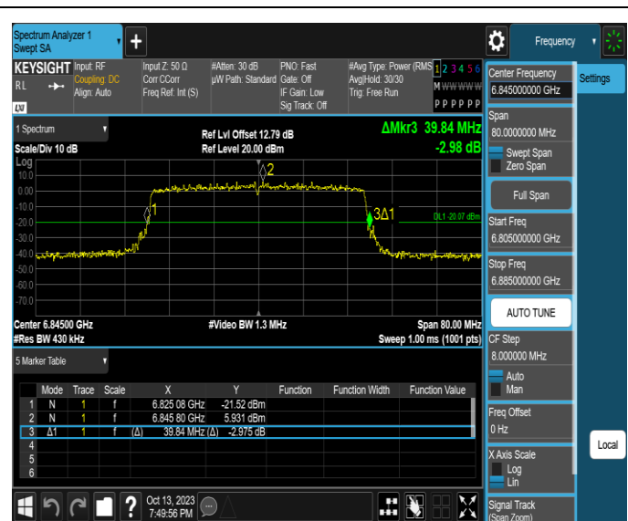
11AX40SISO-Ant2-6845
