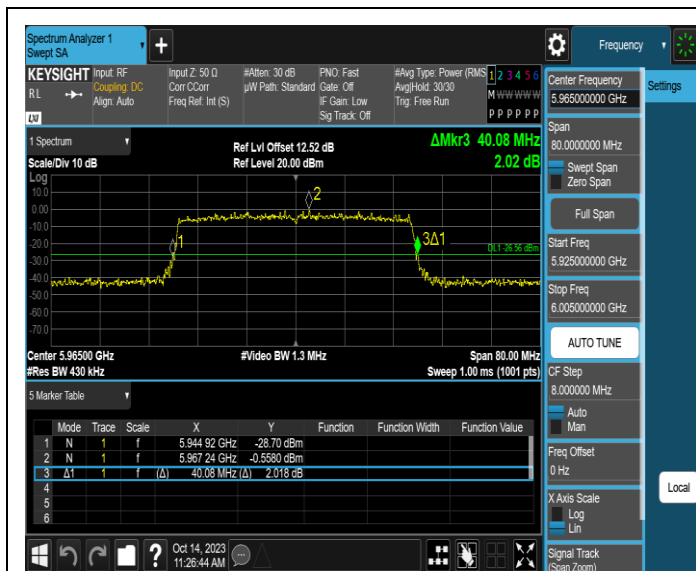
11AX40SISO-Ant3-5965
