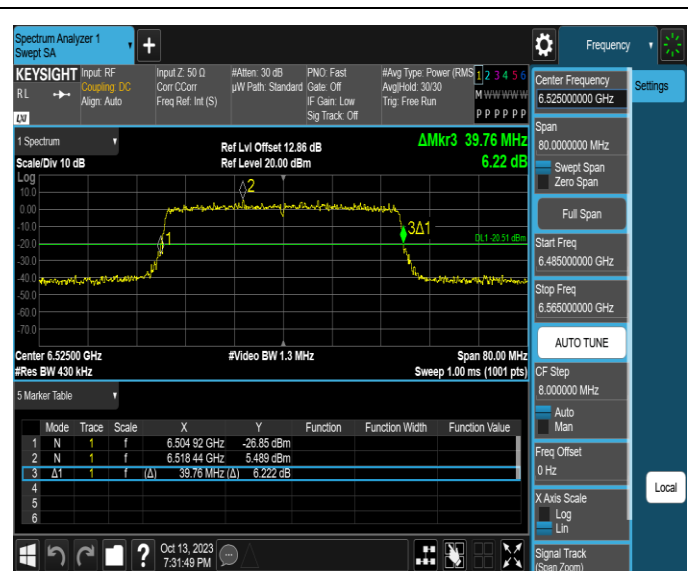
11AX40ISO-Ant2-6525
