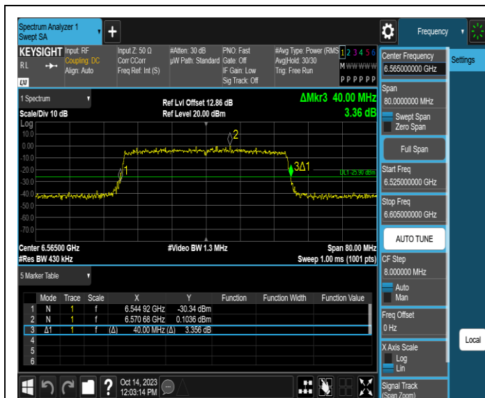
11AX40SISO-Ant3-6565
