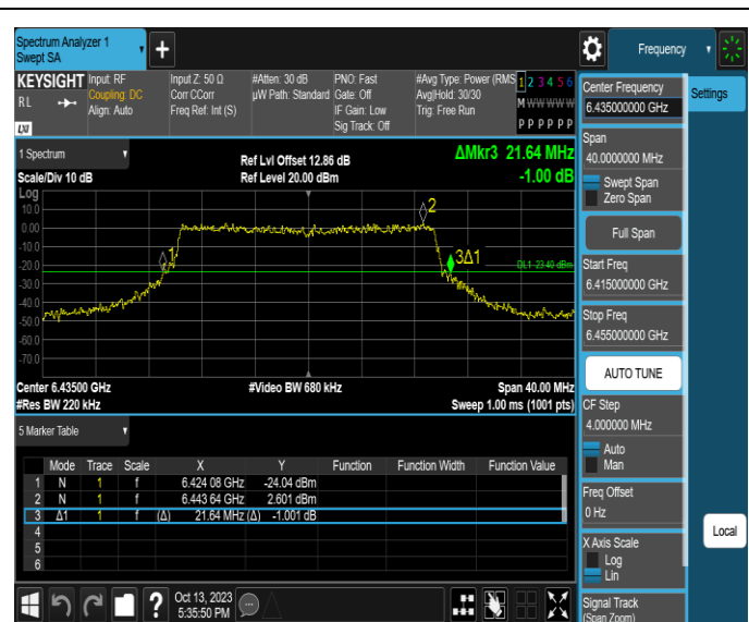
11AX20SISO-Ant2-6435
