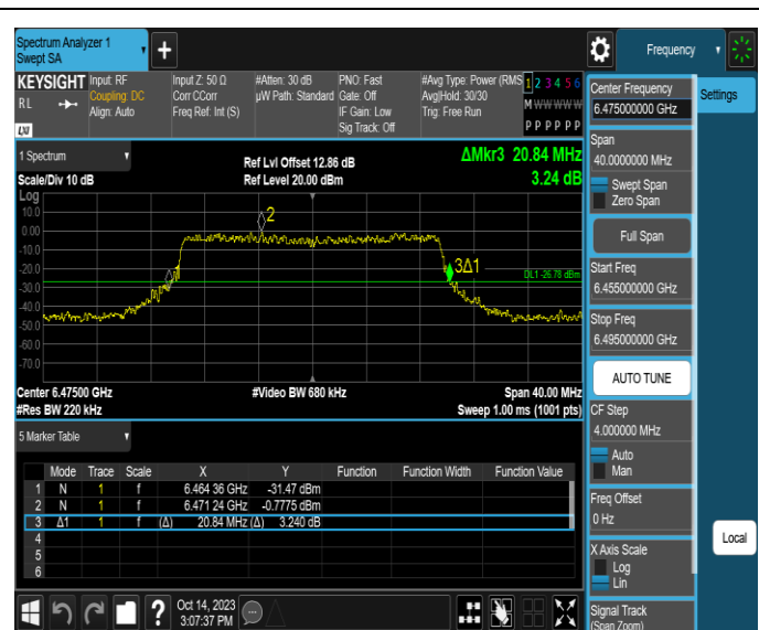
11AX20SISO-Ant4-6475
