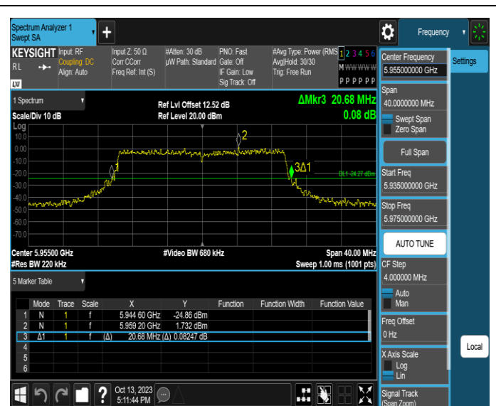
11AX20SISO-Ant2-5955
