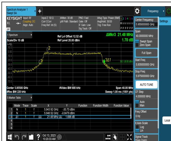
11AX20SISO-Ant1-5955
