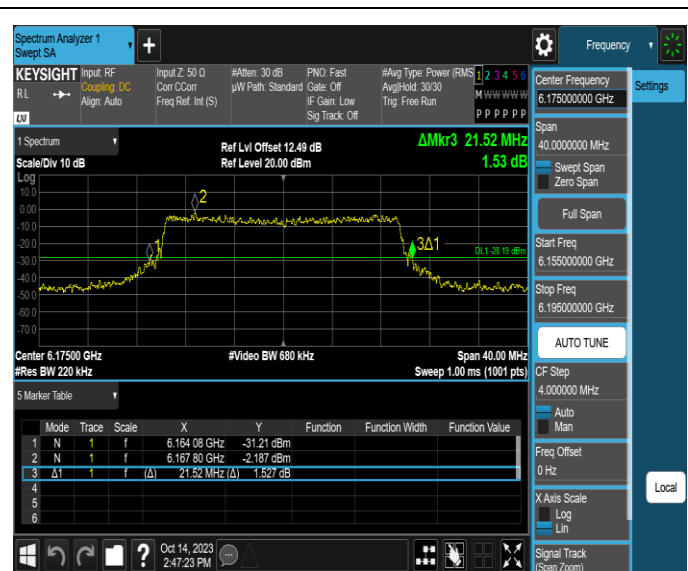
11AX20SISO-Ant4-6175
