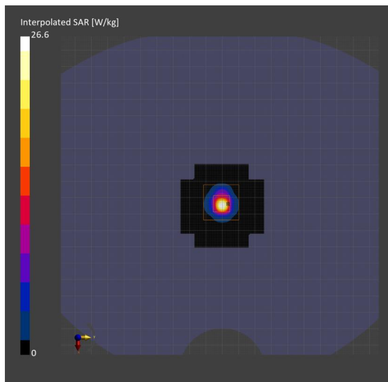
Fig.B.1. Validation 6500MHz 25mW
