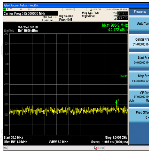
Band4-3MHz-16QAM-20385-15RB#0-Range1:30~1000MHz
