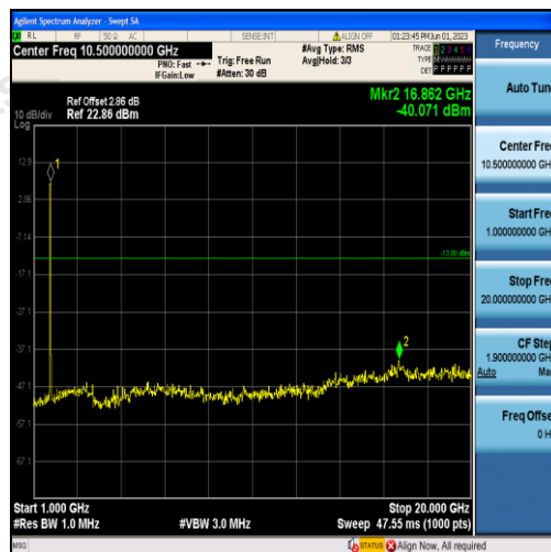
Band4-15MHz-16QAM-20175-75RB#0-Range2:1000~20000MHz
