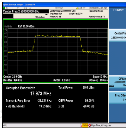
Band7-20MHz-QPSK-21350-100RB#0-17.973
