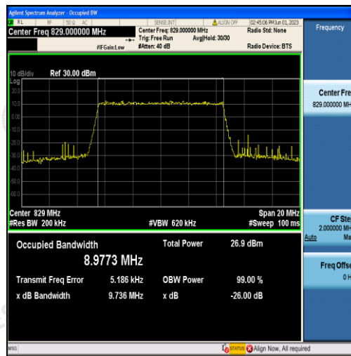
Band5-10MHz-16QAM-20450-50RB#0-8.9773
