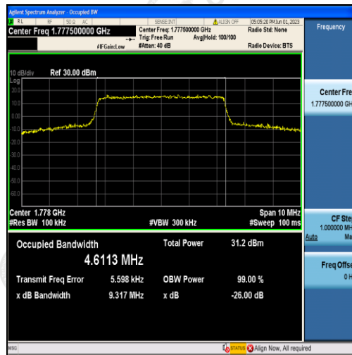
Band66-5MHz-16QAM-132647-25RB#0-4.6113
