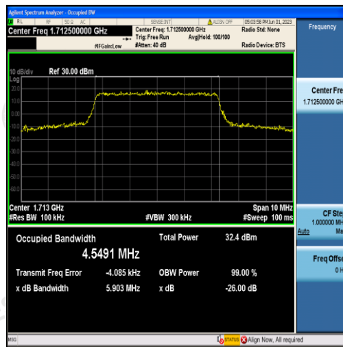
Band66-5MHz-16QAM-131997-25RB#0-4.5491
