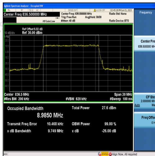
Band5-10MHz-16QAM-20525-50RB#0-8.9850
