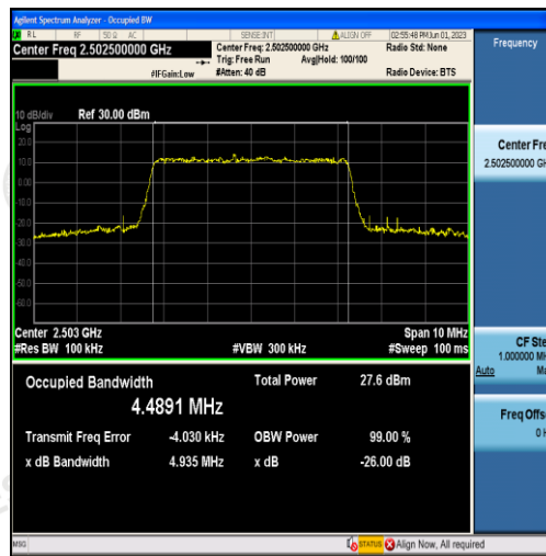
Band7-5MHz-16QAM-20775-25RB#0-4.4891
