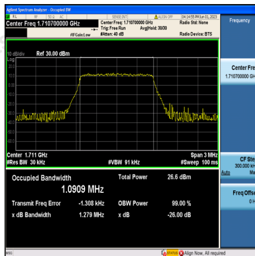
Band66-1.4MHz-QPSK-131979-6RB#0-1.0909
