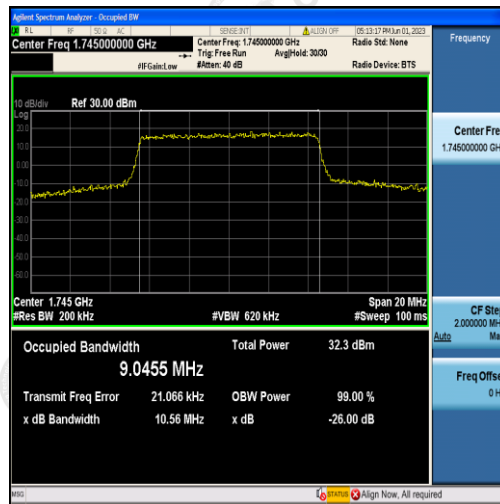
Band66-10MHz-QPSK-132322-50RB#0-9.0455
