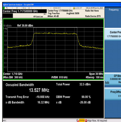
Band66-15MHz-QPSK-132047-75RB#0-13.527
