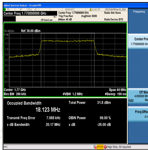
Band66-20MHz-QPSK-132572-100RB#0-18.123
