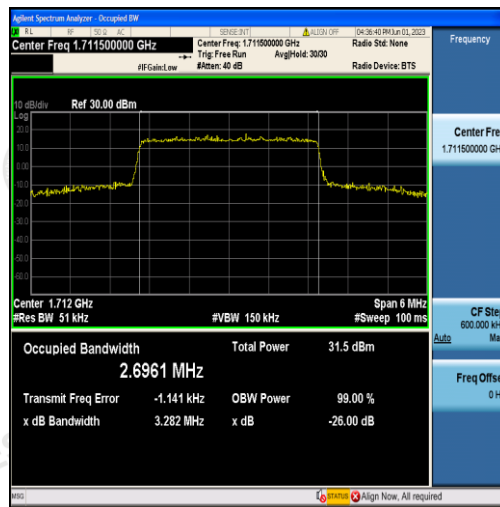
Band66-3MHz-16QAM-131987-15RB#0-2.6961
