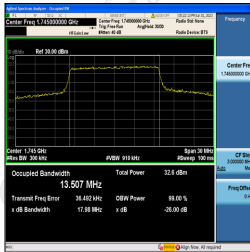
Band66-15MHz-QPSK-132322-75RB#0-13.507
