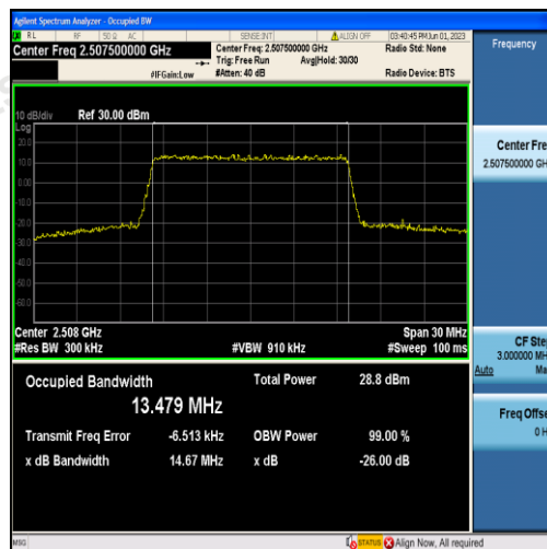
Band7-15MHz-QPSK-20825-75RB#0-13.479
