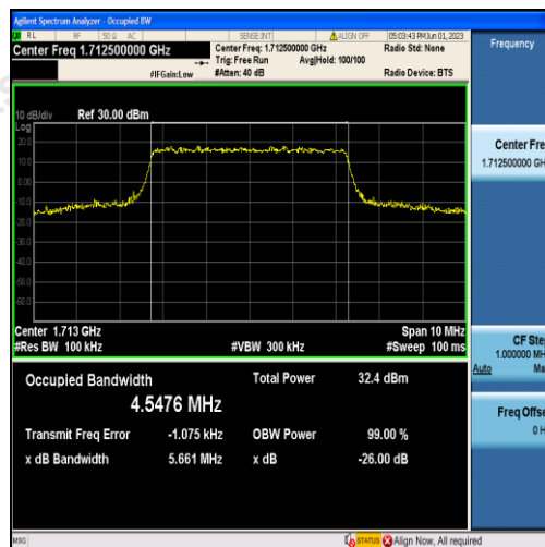
Band66-5MHz-QPSK-131997-25RB#0-4.5476
