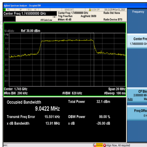
Band66-10MHz-16QAM-132322-50RB#0-9.0422
