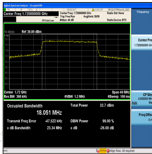
Band66-20MHz-16QAM-132072-100RB#0-18.051
