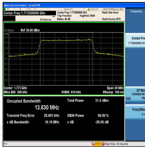
Band66-15MHz-QPSK-132597-75RB#0-13.630
