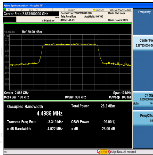
Band7-5MHz-QPSK-21425-25RB#0-4.4986
