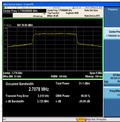
Band66-3MHz-QPSK-132657-15RB#0-2.7078
