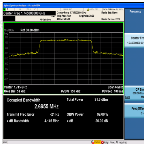
Band66-3MHz-16QAM-132322-15RB#0-2.6955
