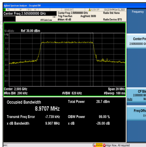
Band7-10MHz-QPSK-20800-50RB#0-8.9707
