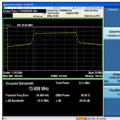
Band66-15MHz-16QAM-132322-75RB#0-13.608
