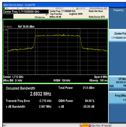
Band66-3MHz-QPSK-131987-15RB#0-2.6932
