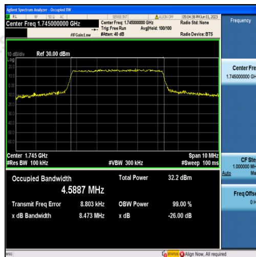
Band66-5MHz-16QAM-132322-25RB#0-4.5887
