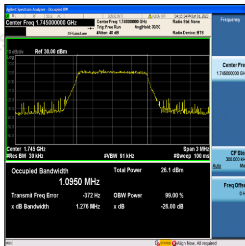
Band66-1.4MHz-16QAM-132322-6RB#0-1.0950
