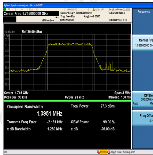
Band66-1.4MHz-QPSK-132322-6RB#0-1.0951
