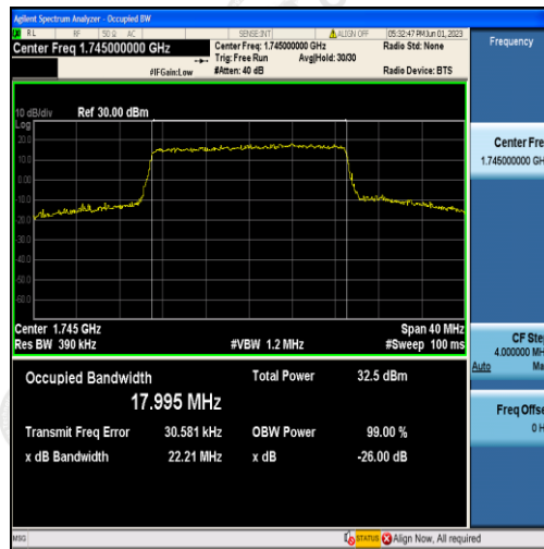
Band66-20MHz-QPSK-132322-100RB#0-17.995
