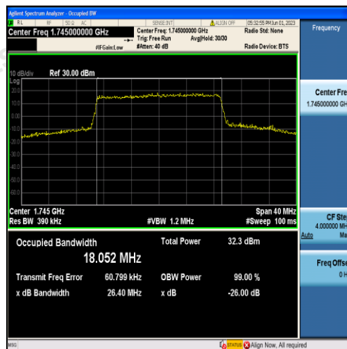
Band66-20MHz-16QAM-132322-100RB#0-18.052
