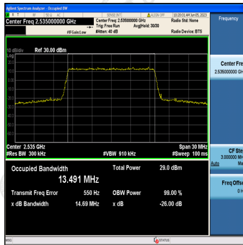
Band7-15MHz-QPSK-21100-75RB#0-13.491
