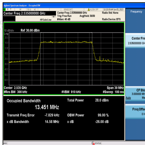
Band7-15MHz-16QAM-21100-75RB#0-13.451
