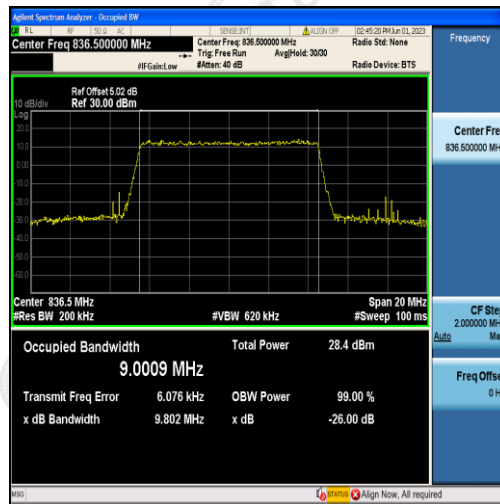
Band5-10MHz-QPSK-20525-50RB#0-9.0009
