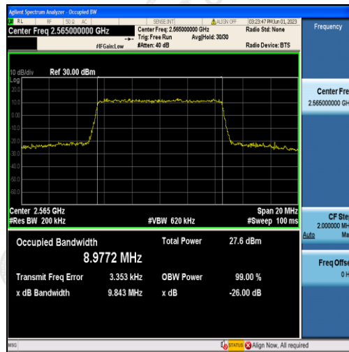
Band7-10MHz-16QAM-21400-50RB#0-8.9772
