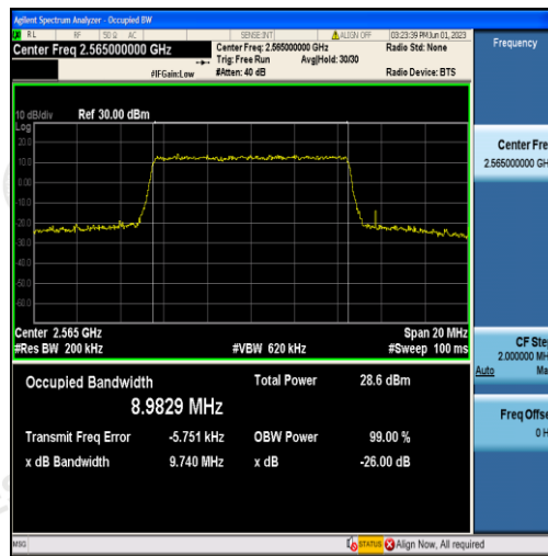
Band7-10MHz-QPSK-21400-50RB#0-8.9829
