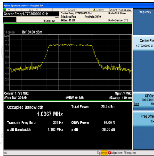
Band66-1.4MHz-QPSK-132665-6RB#0-1.0967
