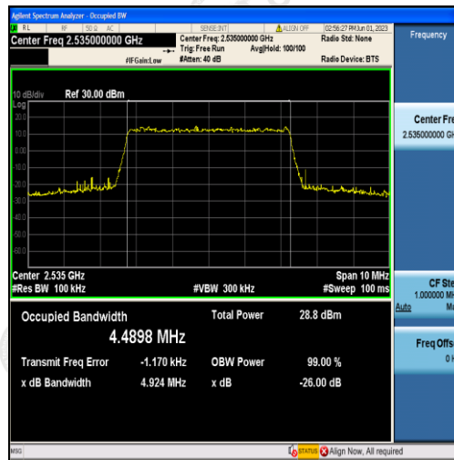
Band7-5MHz-QPSK-21100-25RB#0-4.4898
