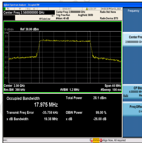
Band7-20MHz-16QAM-21350-100RB#0-17.975
