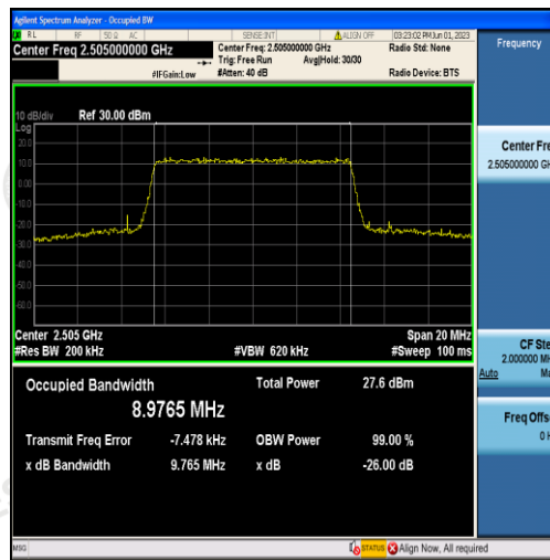
Band7-10MHz-16QAM-20800-50RB#0-8.9765
