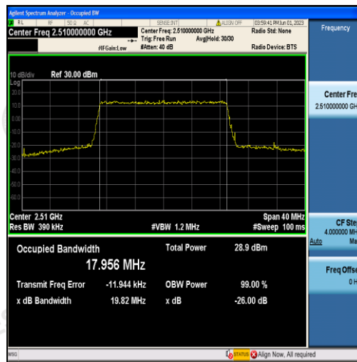
Band7-20MHz-QPSK-20850-100RB#0-17.956
