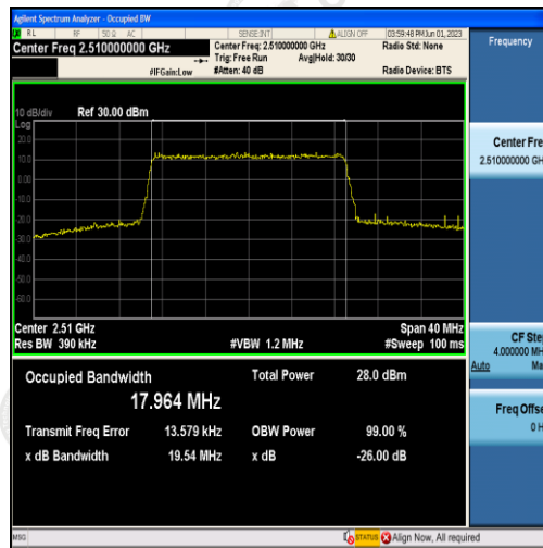
Band7-20MHz-16QAM-20850-100RB#0-17.964
