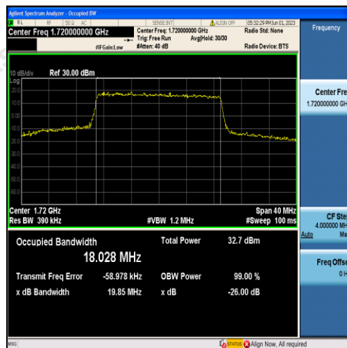
Band66-20MHz-QPSK-132072-100RB#0-18.028
