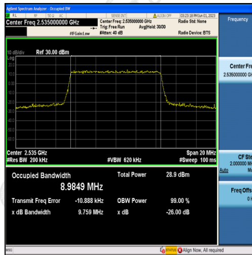
Band7-10MHz-QPSK-21100-50RB#0-8.9849
