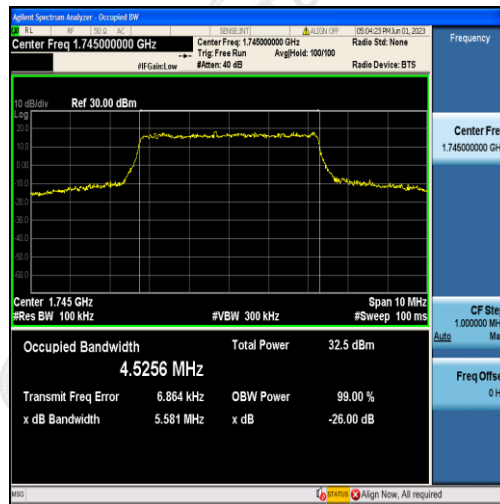
Band66-5MHz-QPSK-132322-25RB#0-4.5256
