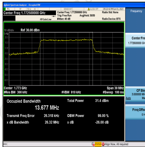
Band66-15MHz-16QAM-132597-75RB#0-13.677
