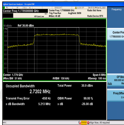
Band66-3MHz-16QAM-132657-15RB#0-2.7202
