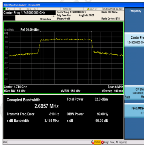
Band66-3MHz-QPSK-132322-15RB#0-2.6957
