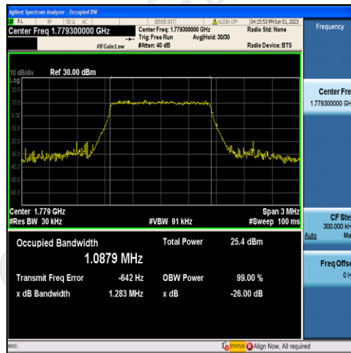
Band66-1.4MHz-16QAM-132665-6RB#0-1.0879
