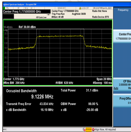
Band66-10MHz-16QAM-132622-50RB#0-9.1226
