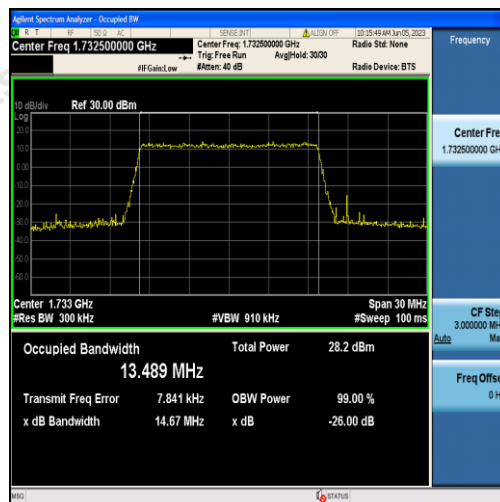
Band4-15MHz-QPSK-20175-75RB#0-13.489
