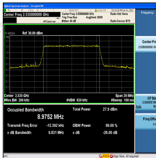
Band7-10MHz-16QAM-21100-50RB#0-8.9752
