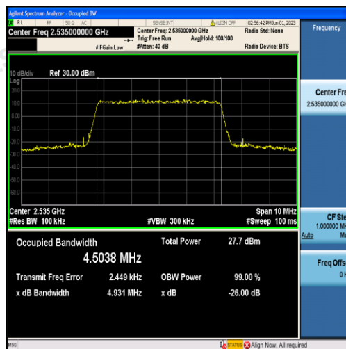
Band7-5MHz-16QAM-21100-25RB#0-4.5038
