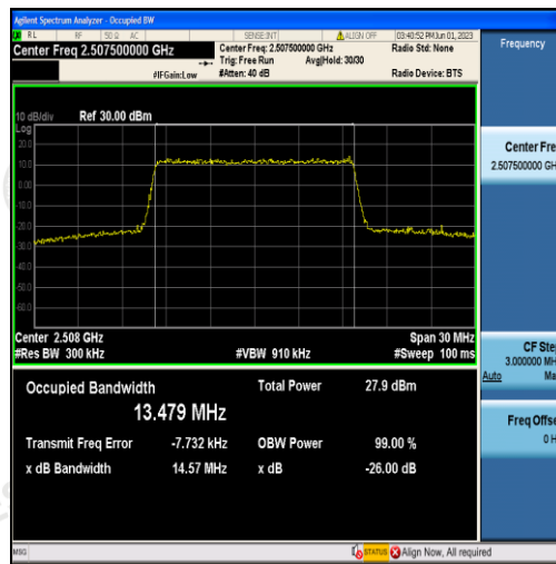
Band7-15MHz-16QAM-20825-75RB#0-13.479
