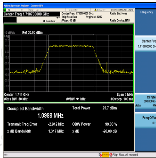
Band66-1.4MHz-16QAM-131979-6RB#0-1.0988
