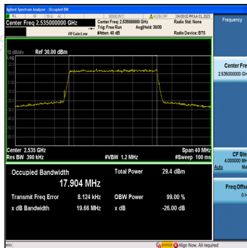
Band7-20MHz-QPSK-21100-100RB#0-17.904
