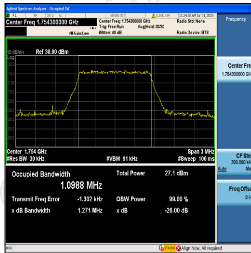
Band4-1.4MHz-QPSK-20393-6RB#0-1.0988
