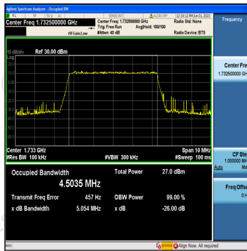
Band4-5MHz-16QAM-20175-25RB#0-4.5035
