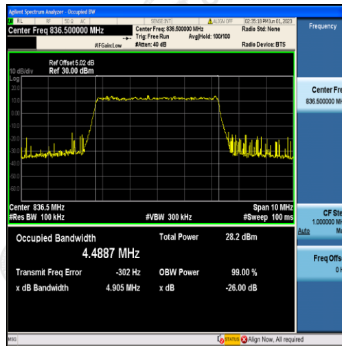
Band5-5MHz-QPSK-20525-25RB#0-4.4887
