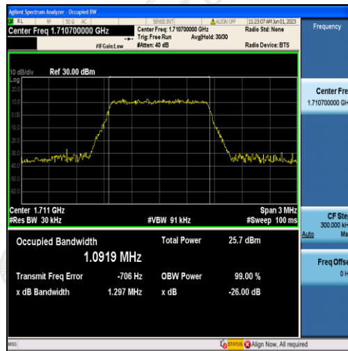
Band4-1.4MHz-16QAM-19957-6RB#0-1.0919
