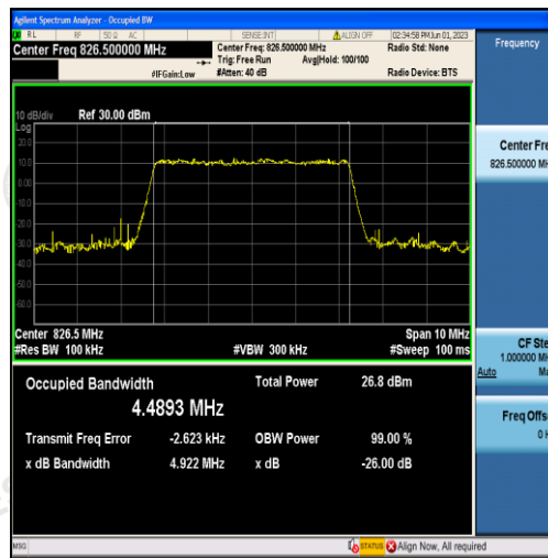
Band5-5MHz-16QAM-20425-25RB#0-4.4893
