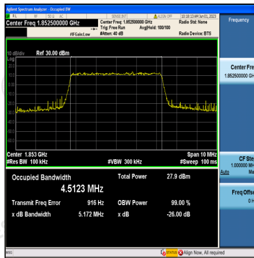
Band2-5MHz-QPSK-18625-25RB#0-4.5123
