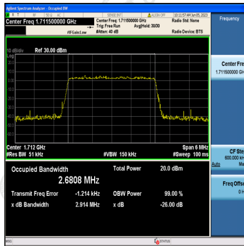
Band4-3MHz-16QAM-19965-15RB#0-2.6808
