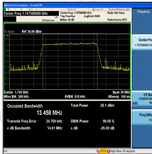
Band4-15MHz-QPSK-20325-75RB#0-13.458
