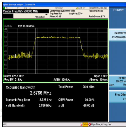
Band5-3MHz-16QAM-20415-15RB#0-2.6766
