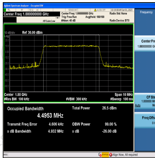
Band2-5MHz-16QAM-18900-25RB#0-4.4953
