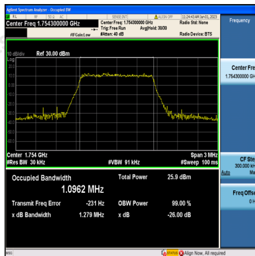
Band4-1.4MHz-16QAM-20393-6RB#0-1.0962
