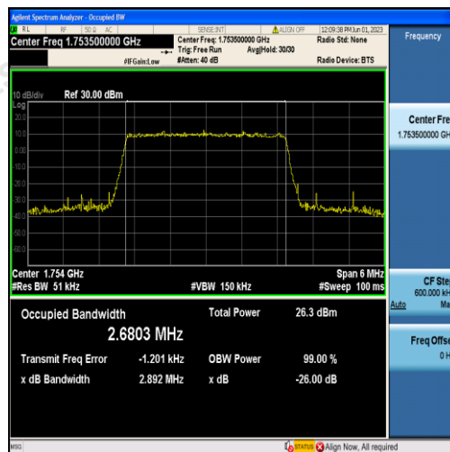
Band4-3MHz-16QAM-20385-15RB#0-2.6803
