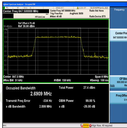
Band5-3MHz-QPSK-20635-15RB#0-2.6909
