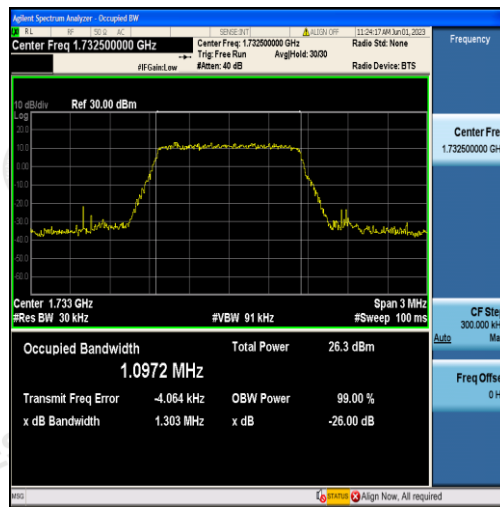
Band4-1.4MHz-16QAM-20175-6RB#0-1.0972
