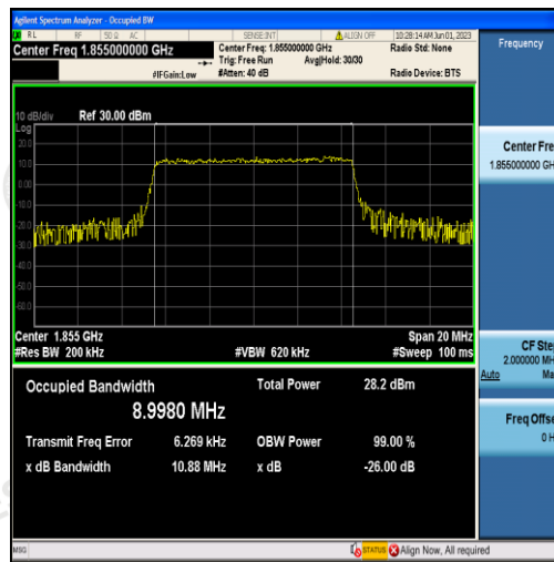
Band2-10MHz-QPSK-18650-50RB#0-8.9980
