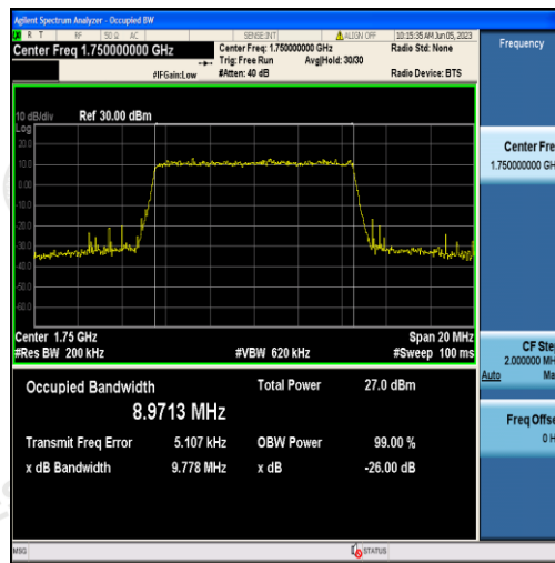
Band4-10MHz-16QAM-20350-50RB#0-8.9713
