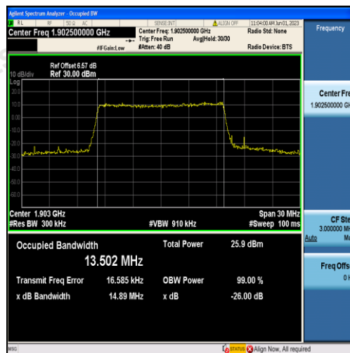
Band2-15MHz-16QAM-19125-75RB#0-13.502
