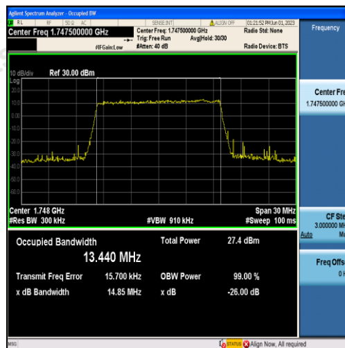
Band4-15MHz-16QAM-20325-75RB#0-13.440
