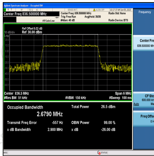
Band5-3MHz-16QAM-20525-15RB#0-2.6790
