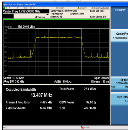
Band4-15MHz-16QAM-20175-75RB#0-13.487
