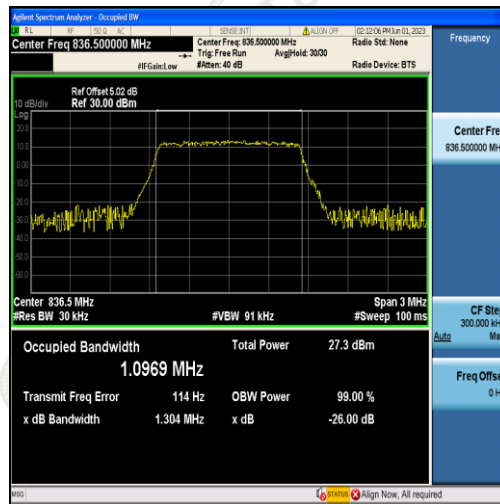
Band5-1.4MHz-QPSK-20525-6RB#0-1.0969
