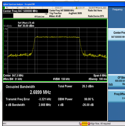
Band5-3MHz-16QAM-20635-15RB#0-2.6899
