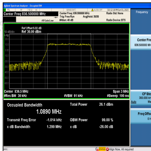
Band5-1.4MHz-16QAM-20525-6RB#0-1.0890
