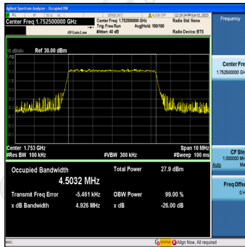
Band4-5MHz-QPSK-20375-25RB#0-4.5032
