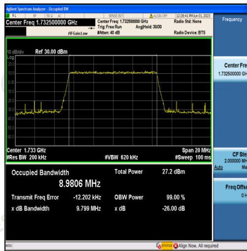
Band4-10MHz-16QAM-20175-50RB#0-8.9806
