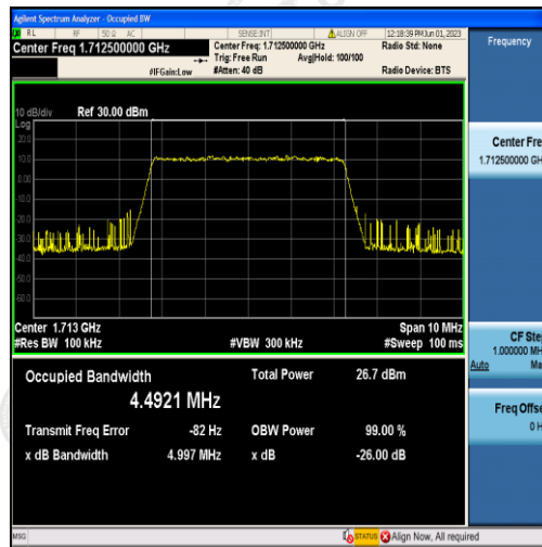
Band4-5MHz-16QAM-19975-25RB#0-4.4921
