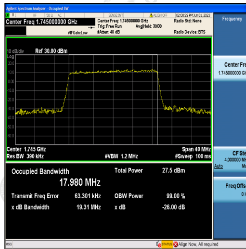
Band4-20MHz-16QAM-20300-100RB#0-17.980
