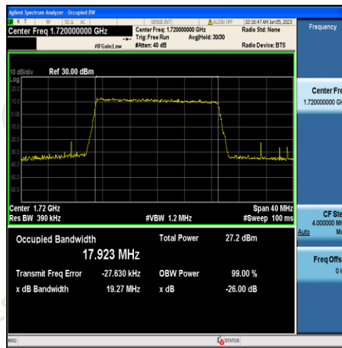
Band4-20MHz-16QAM-20050-100RB#0-17.923
