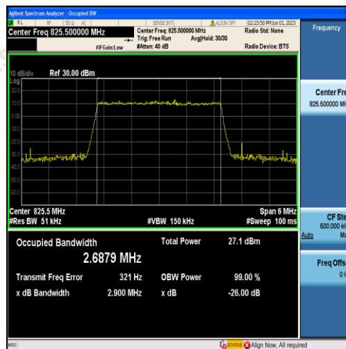
Band5-3MHz-QPSK-20415-15RB#0-2.6879
