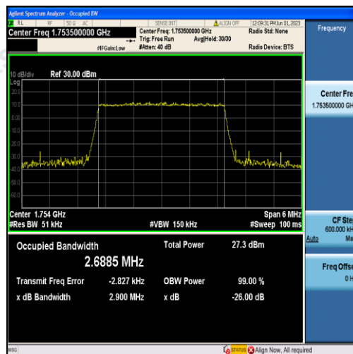
Band4-3MHz-QPSK-20385-15RB#0-2.6885
