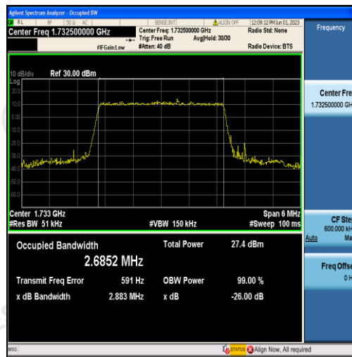
Band4-3MHz-QPSK-20175-15RB#0-2.6852
