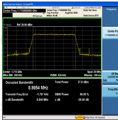
Band4-10MHz-QPSK-20000-50RB#0-8.9854
