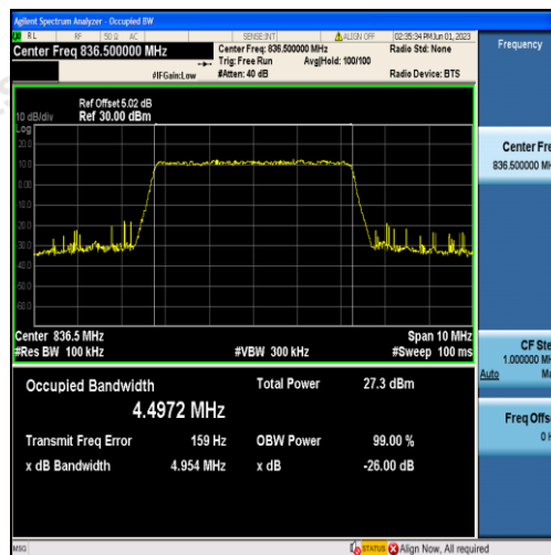
Band5-5MHz-16QAM-20525-25RB#0-4.4972
