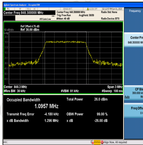
Band5-1.4MHz-16QAM-20643-6RB#0-1.0957
