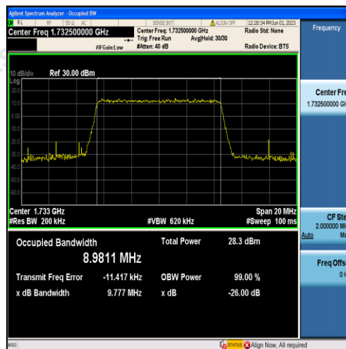
Band4-10MHz-QPSK-20175-50RB#0-8.9811
