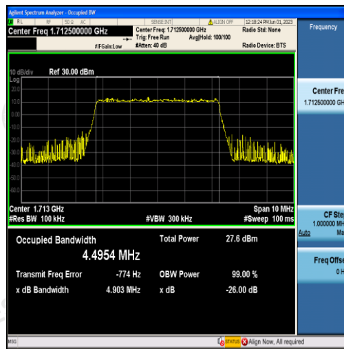
Band4-5MHz-QPSK-19975-25RB#0-4.4954
