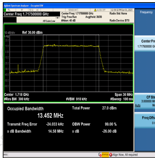
Band4-15MHz-16QAM-20025-75RB#0-13.452
