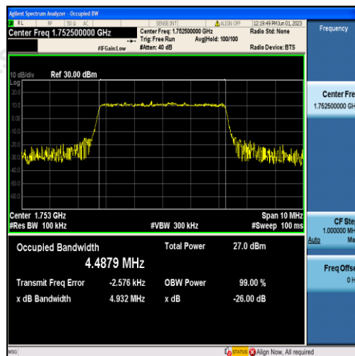
Band4-5MHz-16QAM-20375-25RB#0-4.4879
