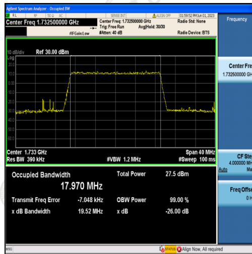
Band4-20MHz-16QAM-20175-100RB#0-17.970
