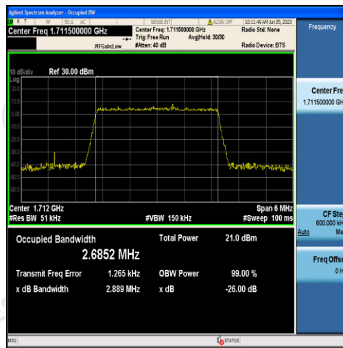
Band4-3MHz-QPSK-19965-15RB#0-2.6852
