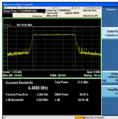
Band4-5MHz-QPSK-20175-25RB#0-4.4968
