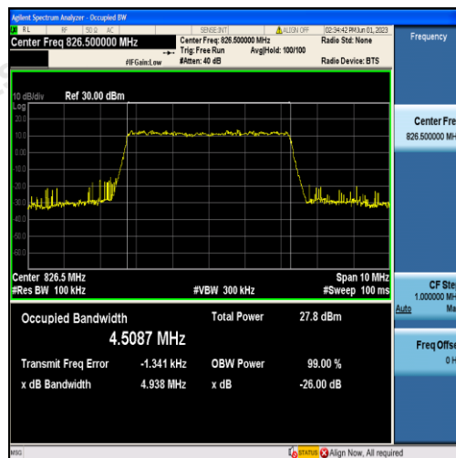
Band5-5MHz-QPSK-20425-25RB#0-4.5087
