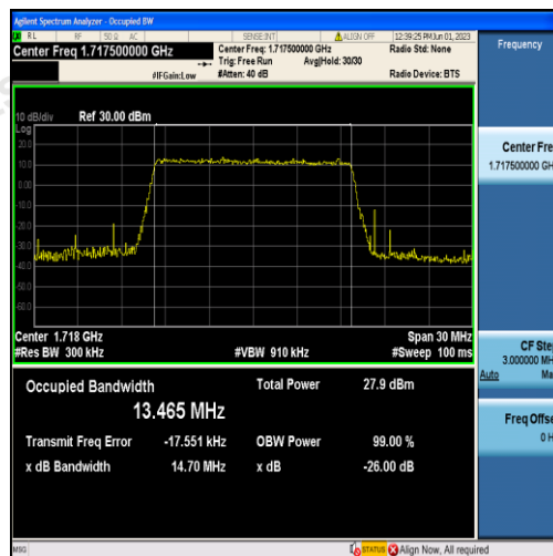
Band4-15MHz-QPSK-20025-75RB#0-13.465
