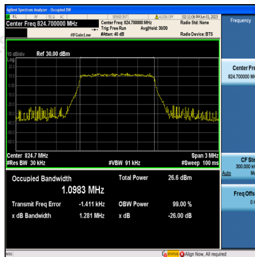
Band5-1.4MHz-QPSK-20407-6RB#0-1.0983
