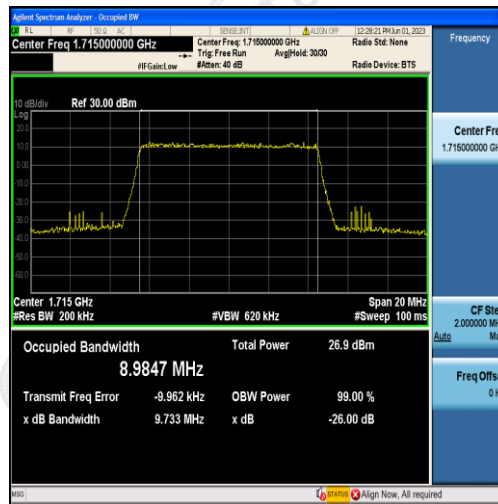
Band4-10MHz-16QAM-20000-50RB#0-8.9847
