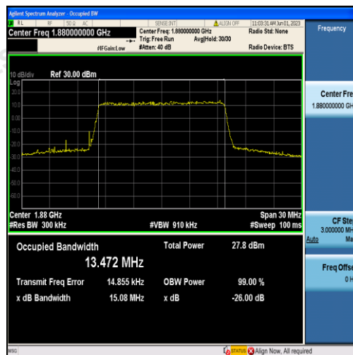
Band2-15MHz-QPSK-18900-75RB#0-13.472
