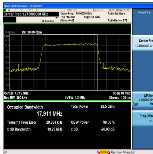
Band4-20MHz-QPSK-20300-100RB#0-17.911
