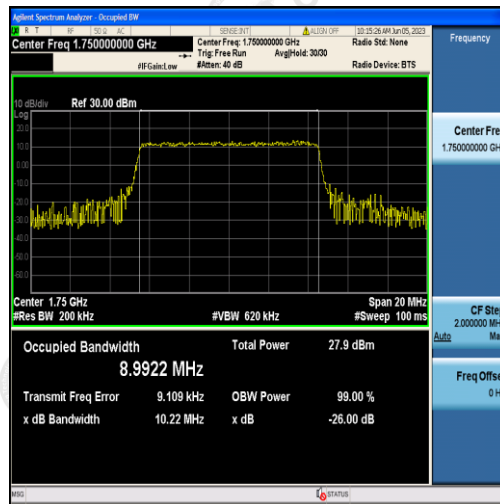
Band4-10MHz-QPSK-20350-50RB#0-8.9922
