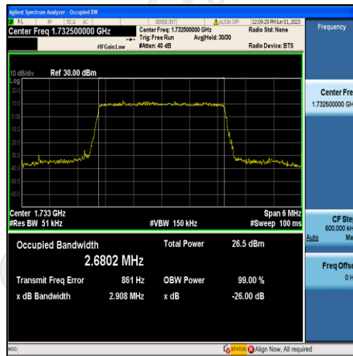
Band4-3MHz-16QAM-20175-15RB#0-2.6802
