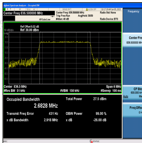
Band5-3MHz-QPSK-20525-15RB#0-2.6828
