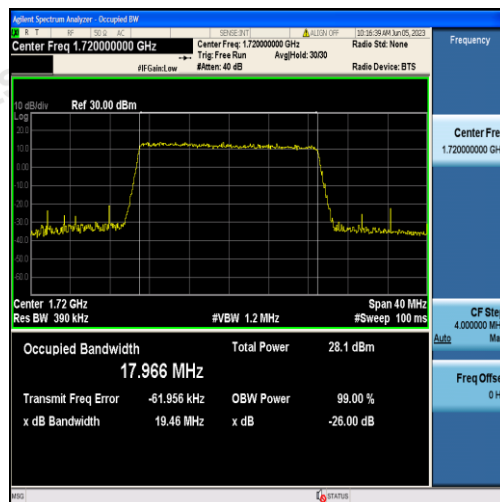
Band4-20MHz-QPSK-20050-100RB#0-17.966
