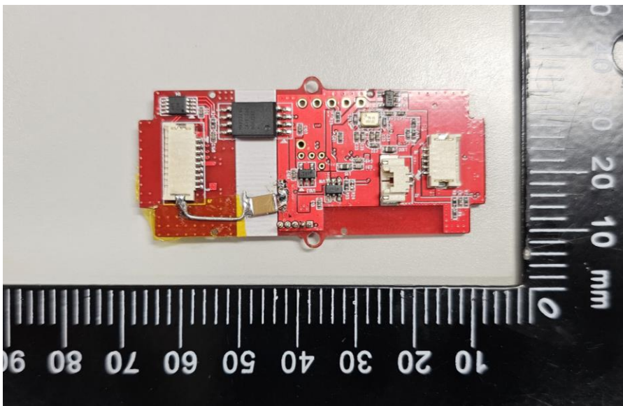
(Internal Photo-Main Board)
