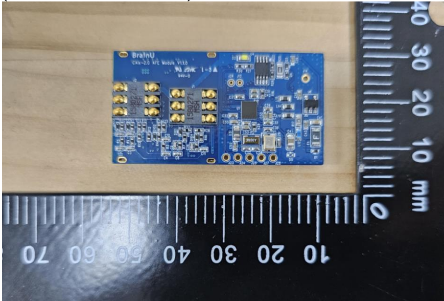
(Internal Photo-AFE Board)
