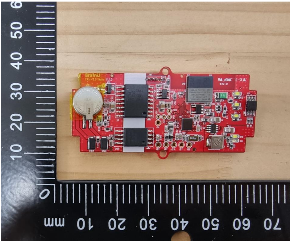
(Internal Photo-Main Board)
