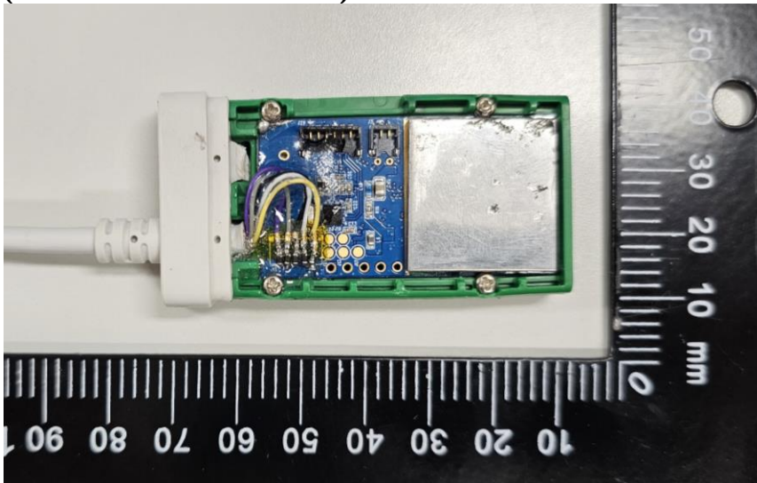
(Internal Photo-AFE Board)
