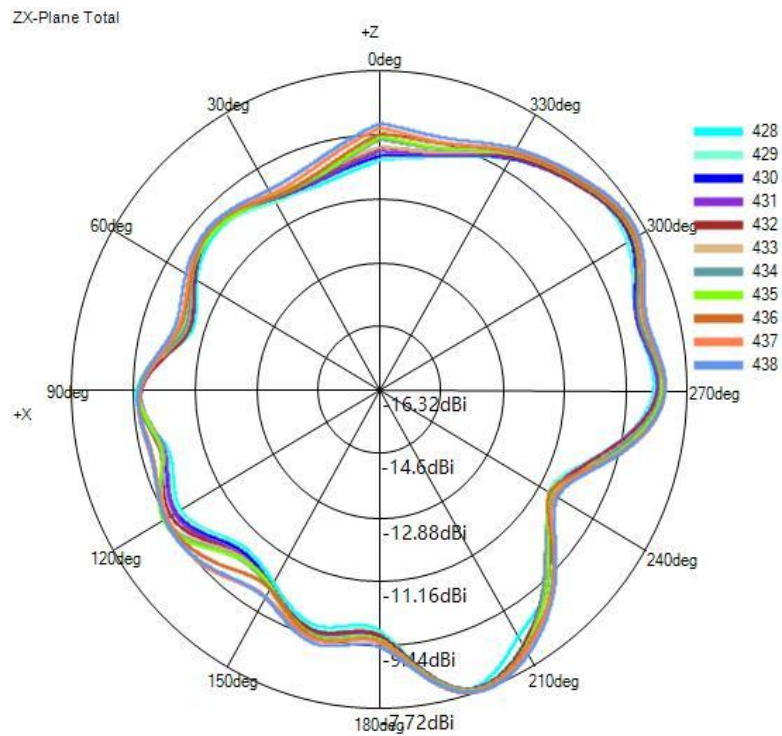
(1) X-Z Plane(unit:dBi):
