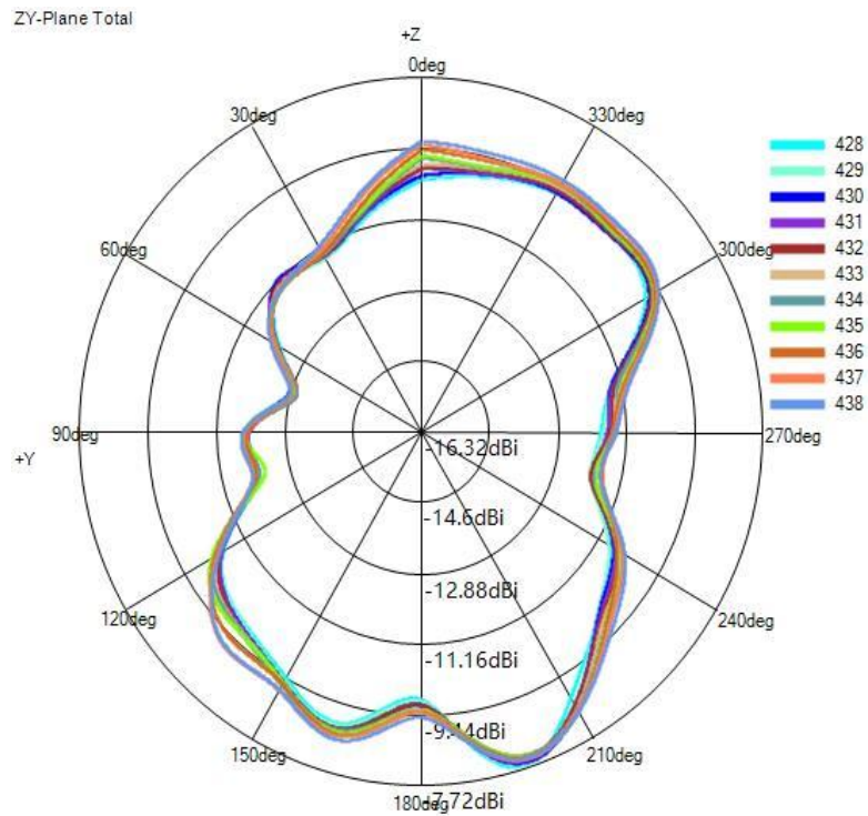
(2) Y-Z Plane(unit:dBi):
