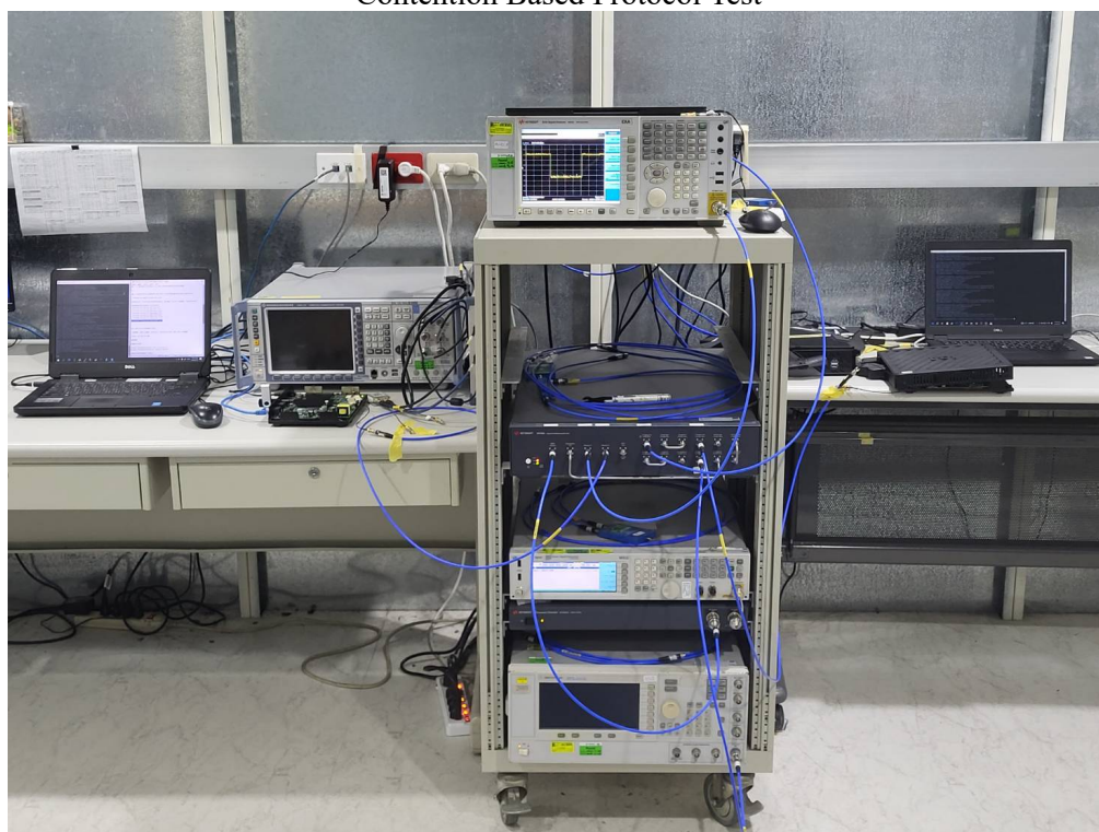
Contention Based Protocol Test
