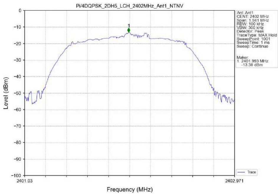
Pi/4DQPSK_2DH5_LCH_2402MHz_Ant1_NTNV
