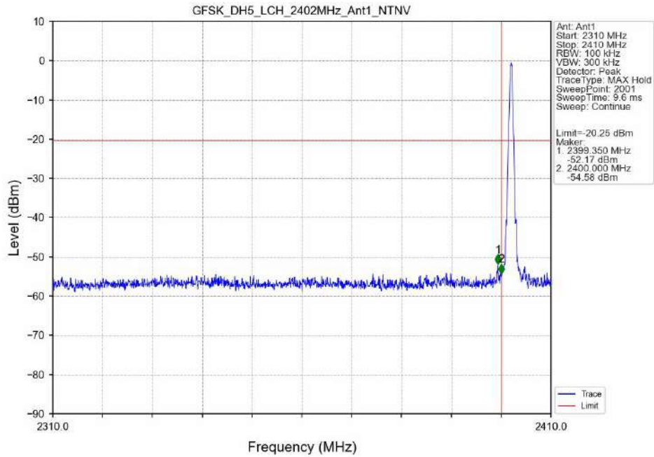
GFSK_DH5_LCH_2402MHz_Ant1_NTNV
