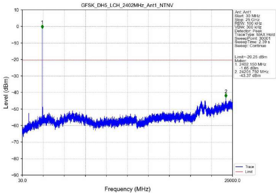
GFSK_DH5_LCH_2402MHz_Ant1_NTNV
