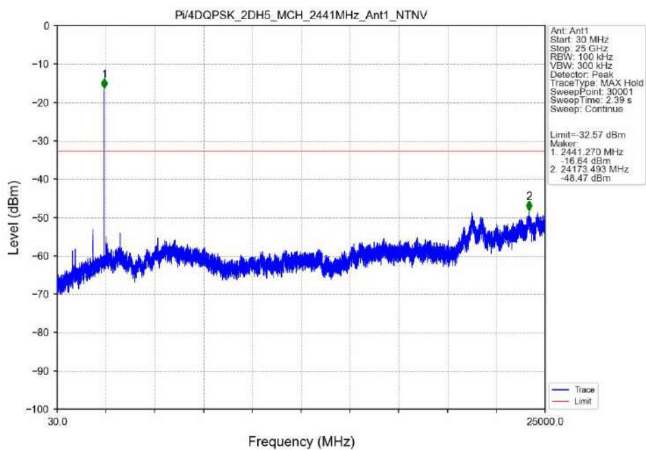
Pi/4DQPSK_2DH5_MCH_2441MHz_Ant1_NTNV
