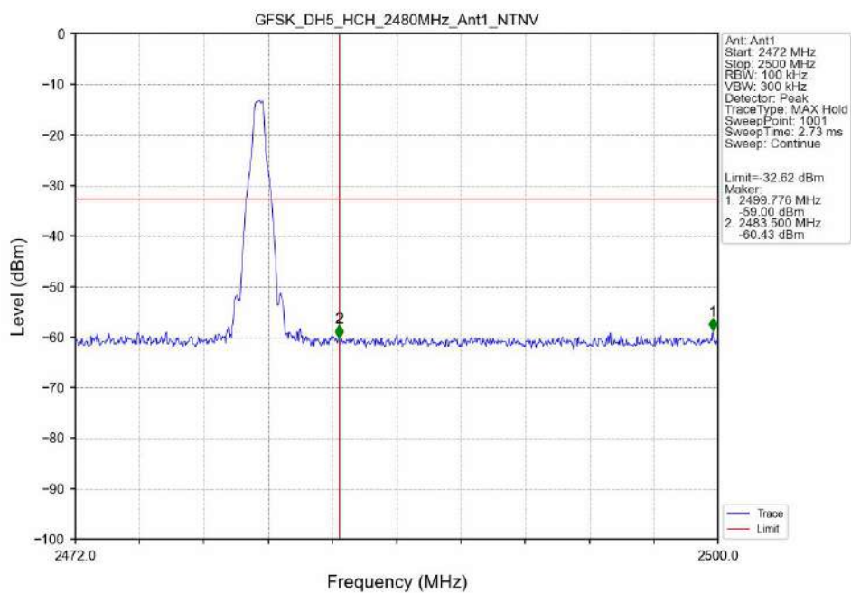
GFSK_DH5_HCH_2480MHz_Ant1_NTNV
