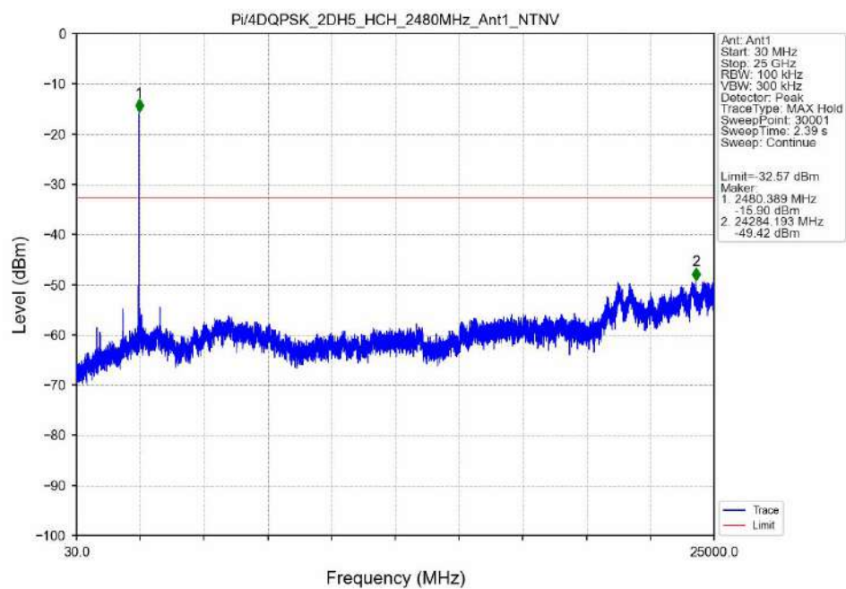
Pi/4DQPSK_2DH5_HCH_2480MHz_Ant1_NTNV
