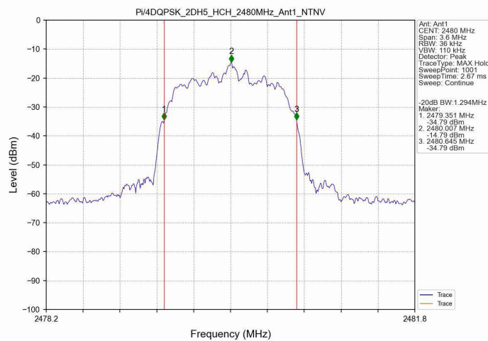
Pi/4DQPSK_2DH5_HCH_2480MHz_Ant1_NTNV
