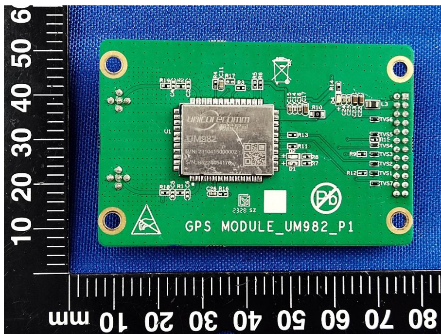
SECONDARY BOARD 3 TOP VIEW (WITH SHIELDING)
