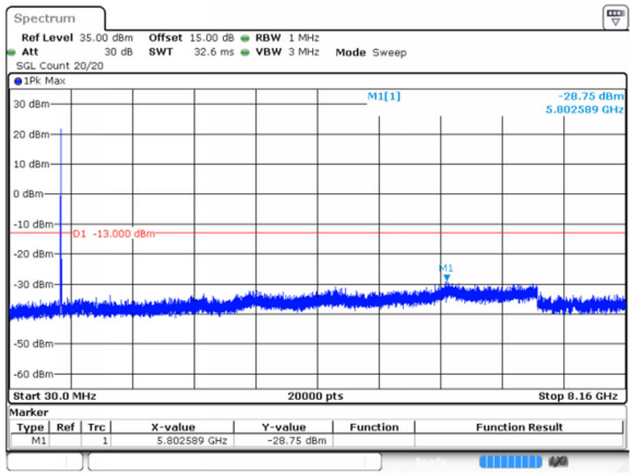
10MHz_Middle_QPSK_1@0(30MHz~8.16GHz)
