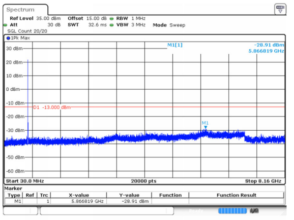
10MHz_High_QPSK_1@0(30MHz~8.16GHz)
