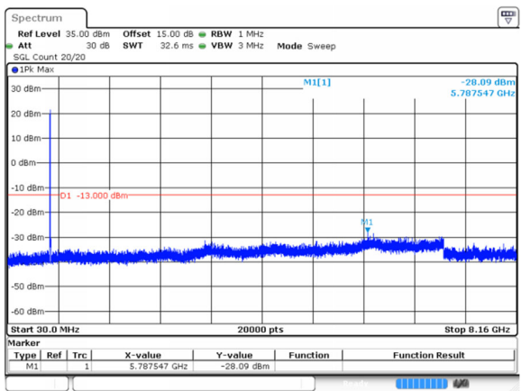
10MHz_Low_QPSK_1@0(30MHz~8.16GHz)
