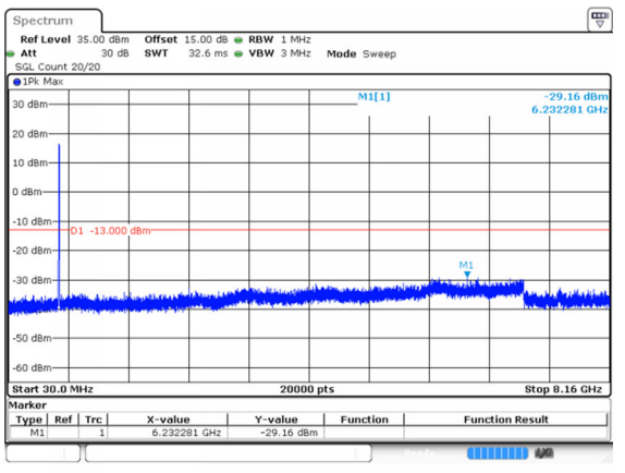
10MHz_High_QPSK_50@0(30MHz~8.16GHz)
