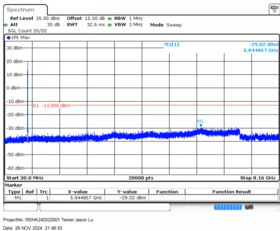
5MHz_Middle_QPSK_25@0(30MHz~8.16GHz)
