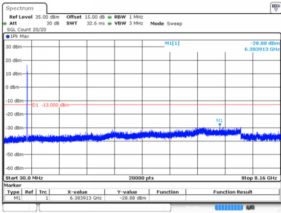
10MHz_Middle_QPSK_50@0(30MHz~8.16GHz)
