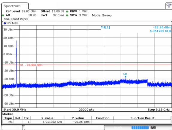
10MHz_Low_QPSK_50@0(30MHz~8.16GHz)
