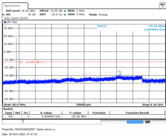
5MHz_High_QPSK_25@0(30MHz~8.16GHz)
