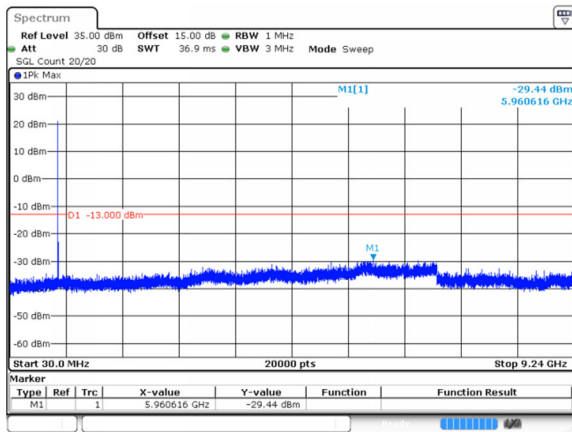
1_10MHz_Low_QPSK_1@0(30MHz~9.24GHz)
