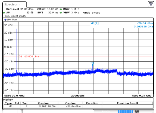
1.4MHz_Cross_QPSK_6@0(30MHz~9.24GHz)
