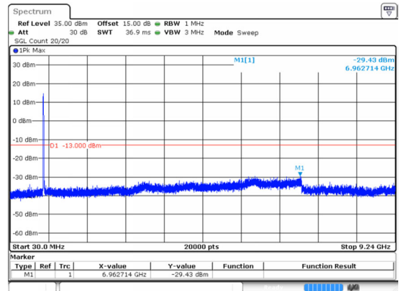
1_15MHz_Low_QPSK_75@0(30MHz~9.24GHz)
