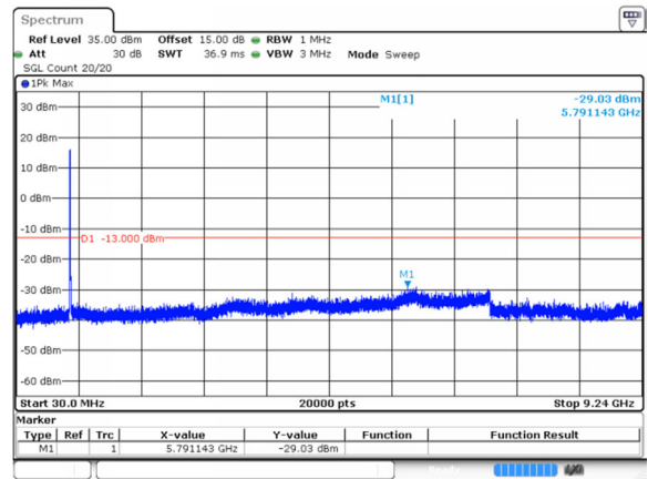
1_10MHz_Low_QPSK_50@0(30MHz~9.24GHz)
