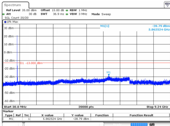
1_15MHz_Low_QPSK_1@0(30MHz~9.24GHz)
