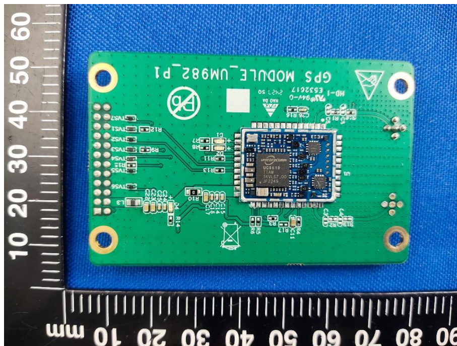
SECONDARY BOARD 1 TOP VIEW (WITHOUT SHIELDING)
