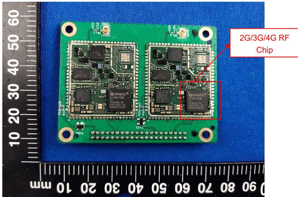
SECONDARY BOARD 1 TOP VIEW (WITHOUT SHIELDING)
