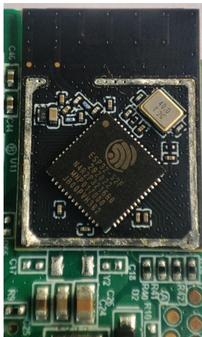
ESP32-S2-MINI-2 (WiFi) Module image without shield
