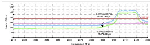
802.11g-Channel 1 Peak+ Average
