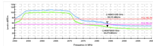
802.11g-Channel 11 Peak+ Average
