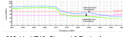
802.11n HT40-Channel 9 Peak+ Average
