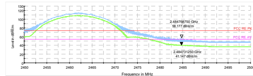
802.11b-Channel 11 Peak+ Average
