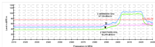
802.11n HT20-Channel 1 Peak+ Average
