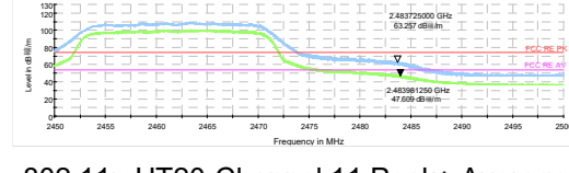
802.11n HT20-Channel 11 Peak+ Average
