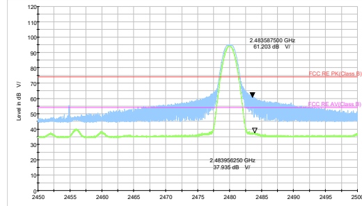
Bluetooth LE (1M) Channel 39 Peak+ Average
