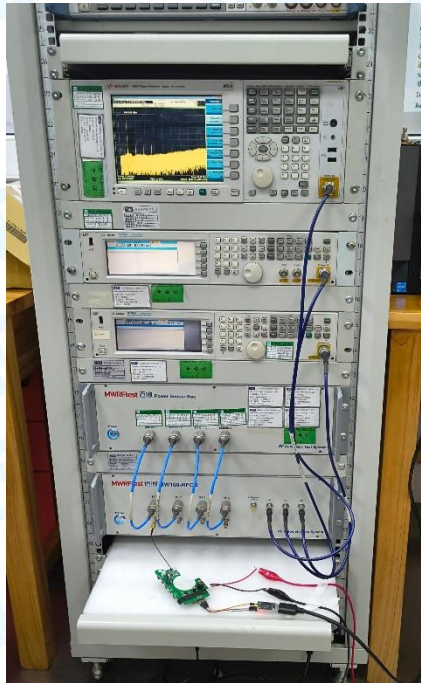
Photo of Setup for Conducted Measurement
